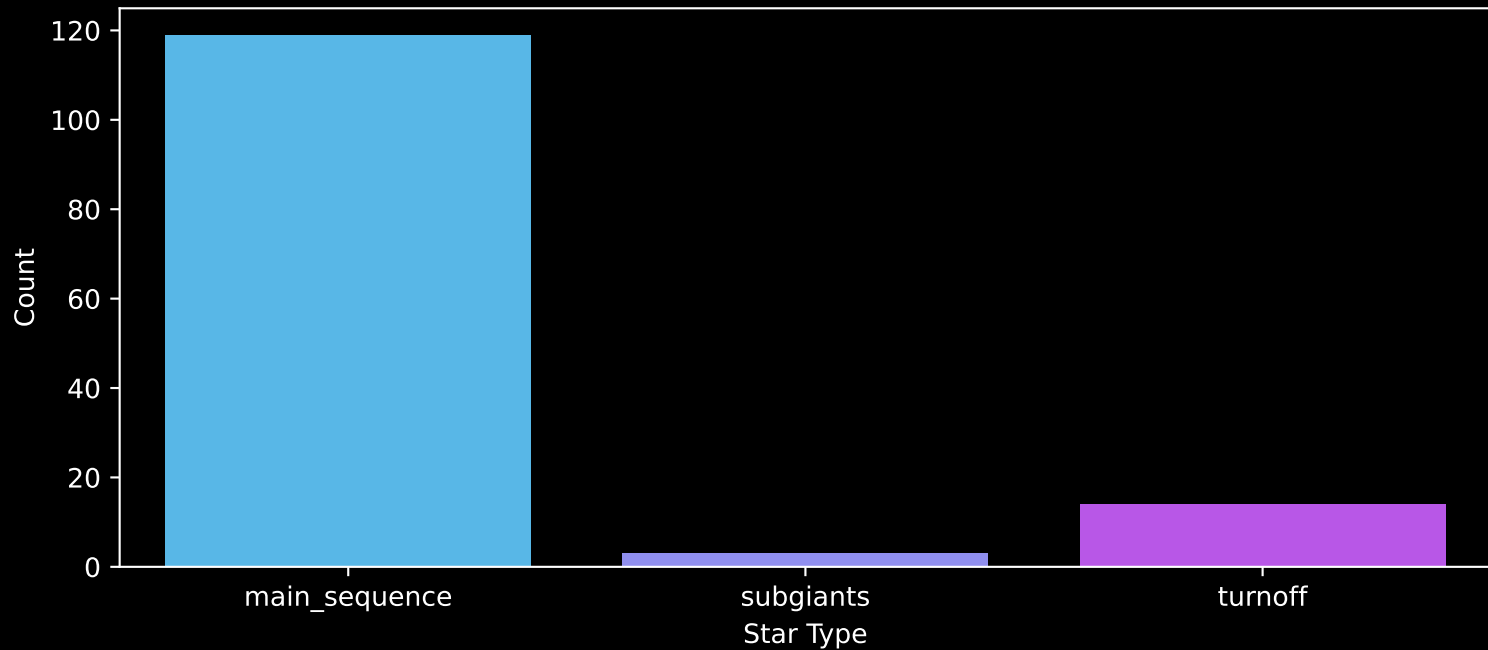
Gaia Cluster: [UPK_579] Count plot of Star Type
