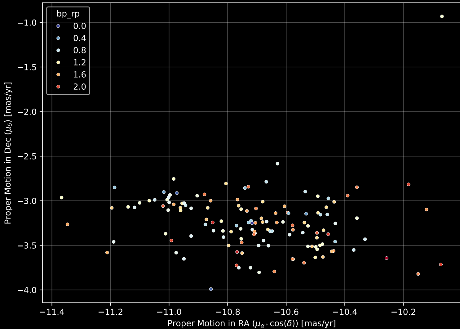
Gaia Cluster: [UPK_579] Proper Motion Diagram (n= 136)
