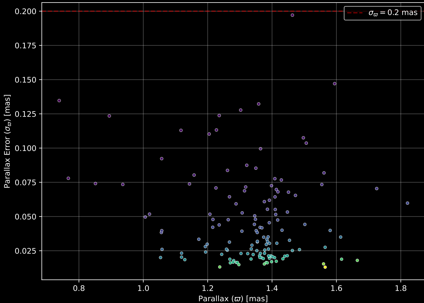
Gaia Cluster: [UPK_579] Parallax Quality (n= 136)
