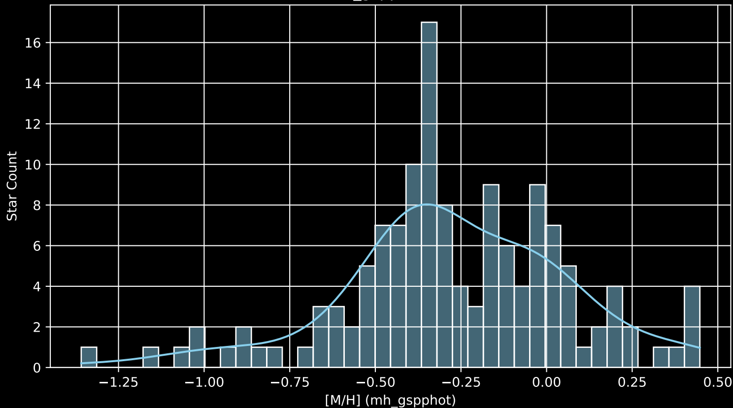
Gaia Cluster: [UPK_579 [M/H] (mh_gspphot) (n= 135)
