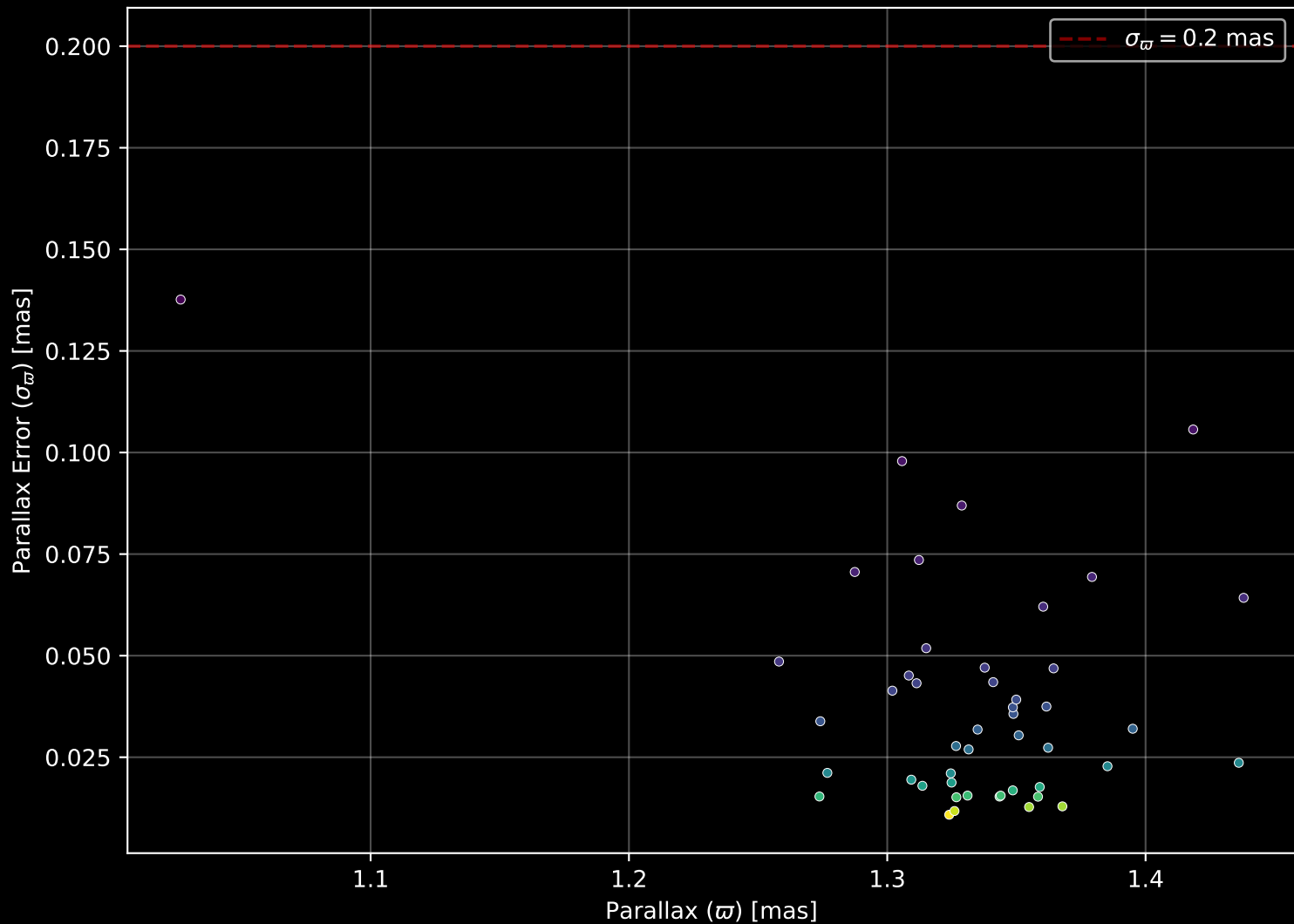
Gaia Cluster: [UPK_605] Parallax Quality (n= 47)
