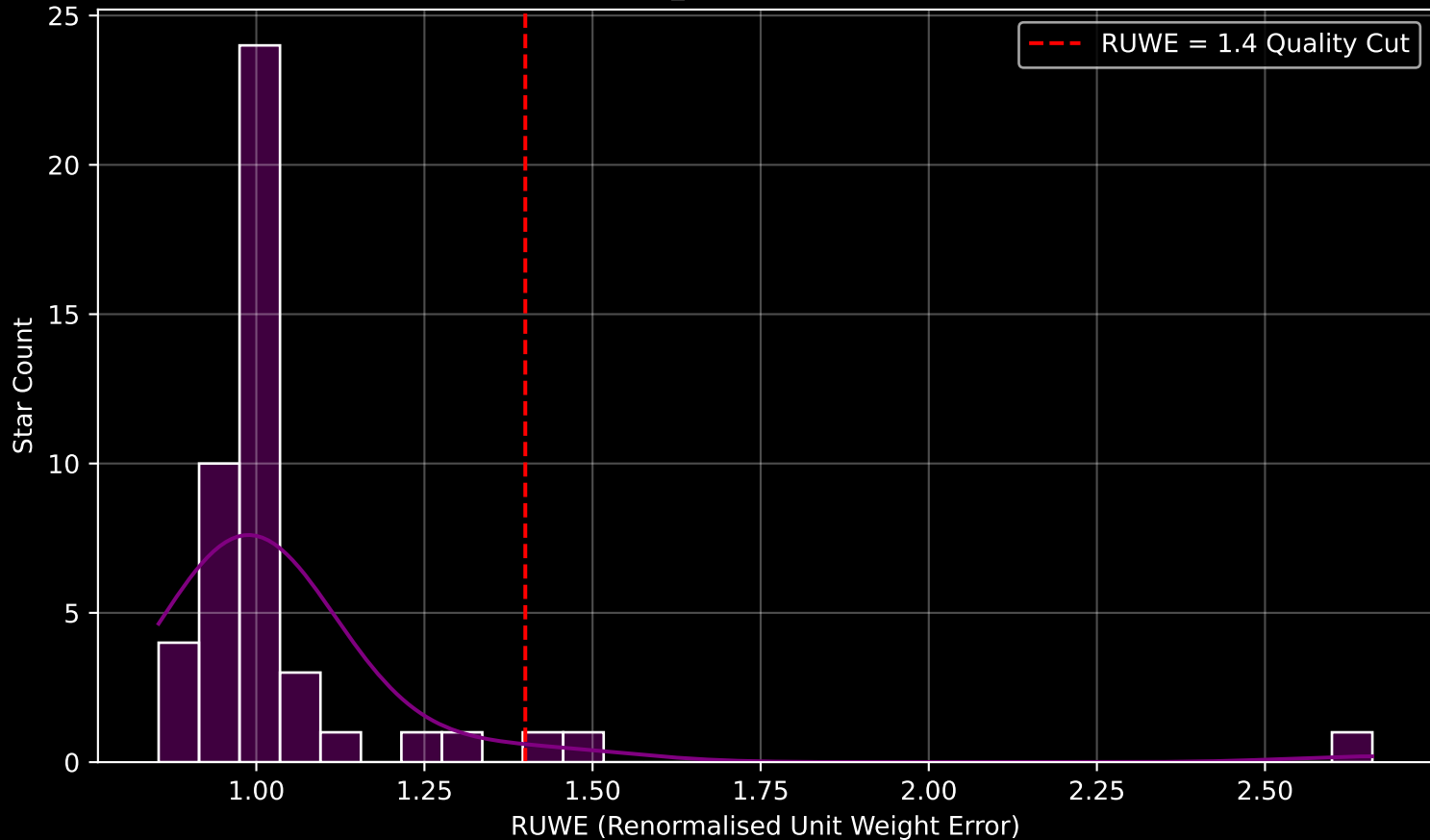
Gaia Cluster: [UPK_605] RUWE Distribution (n= 47)
