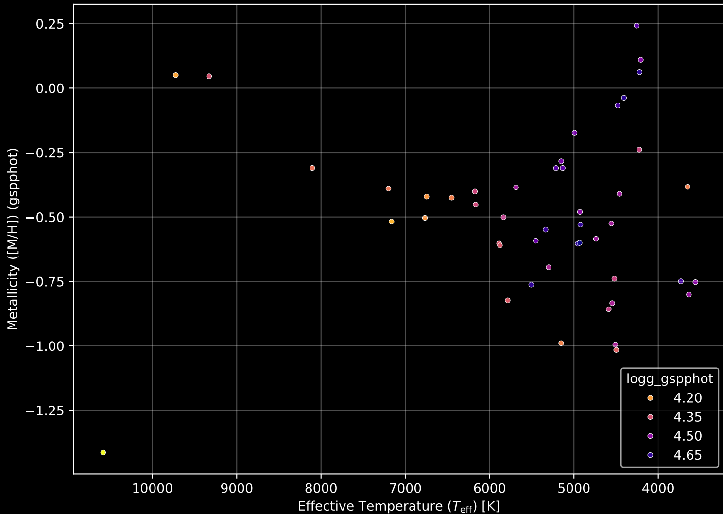
Gaia Cluster: [UPK_605] Stellar Population Parameters (n= 47)
