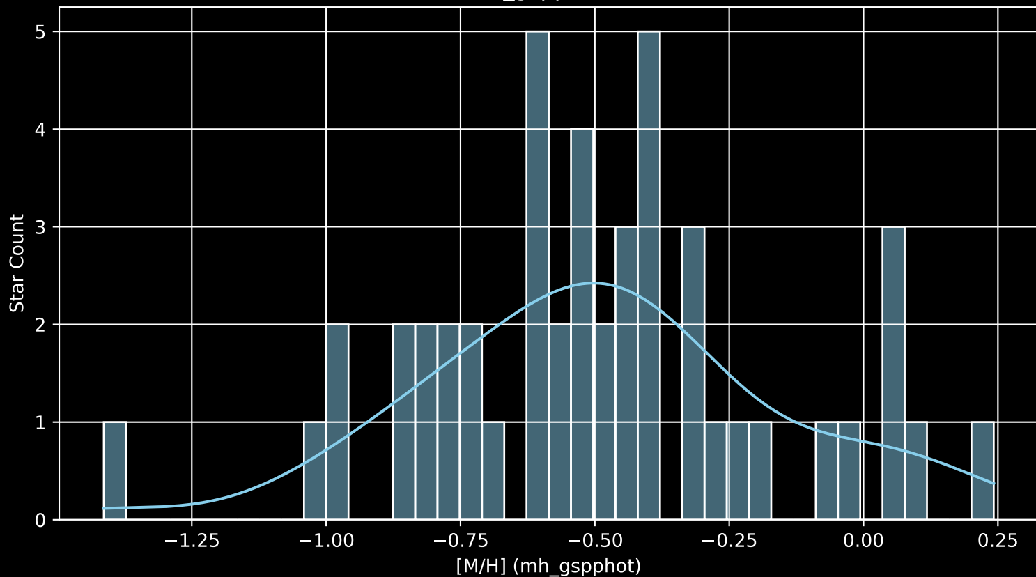
Gaia Cluster: [UPK_605 [M/H] (mh_gspphot) (n= 47)
