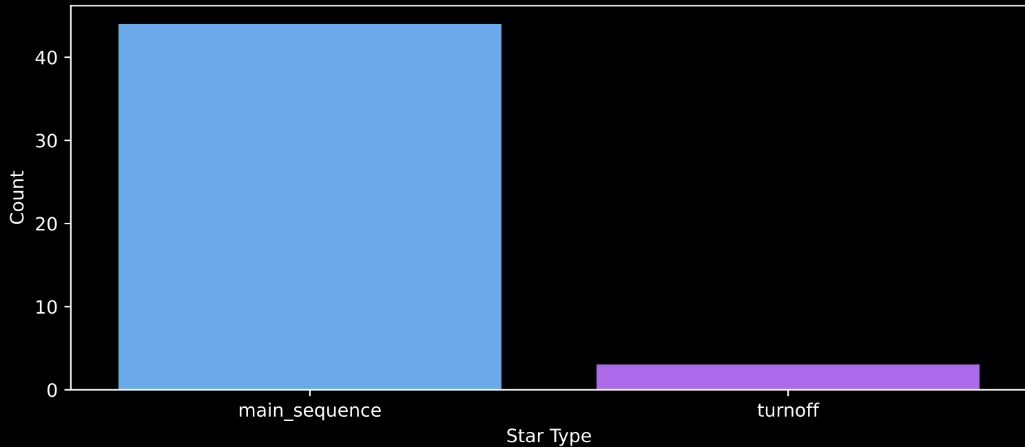
Gaia Cluster: [UPK_605] Count plot of Star Type
