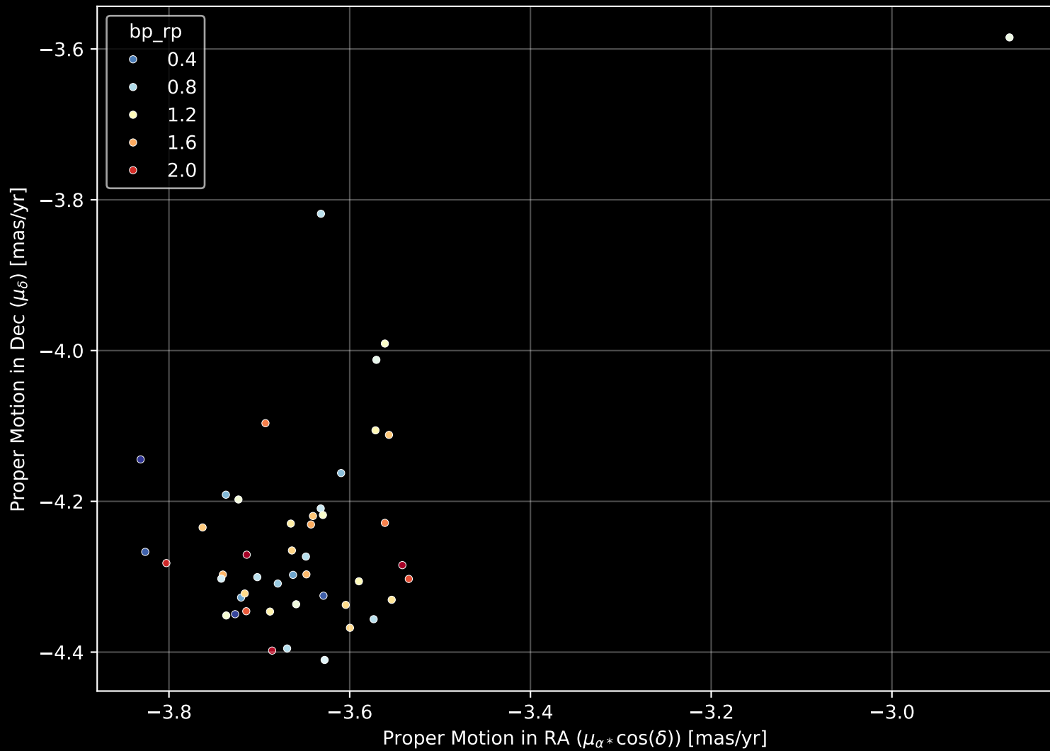
Gaia Cluster: [UPK_605] Proper Motion Diagram (n= 47)
