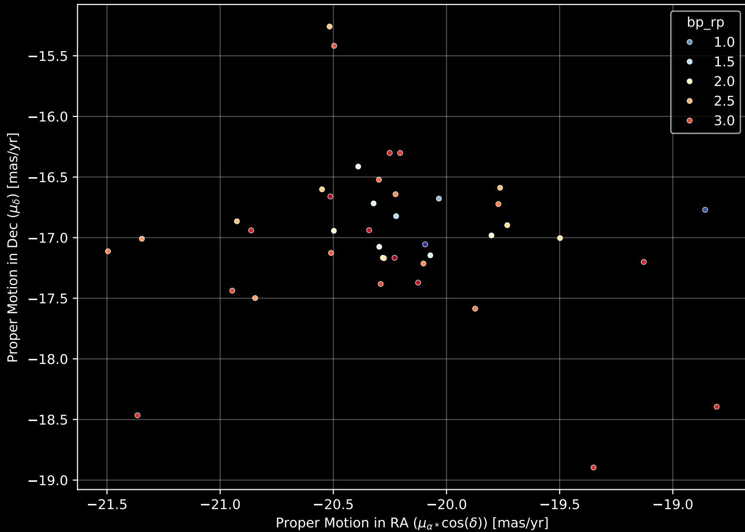
Gaia Cluster: [UPK_606] Proper Motion Diagram (n= 41)
