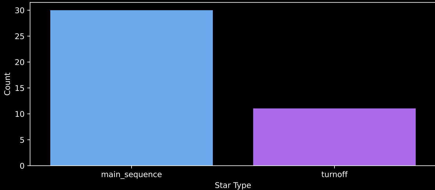
Gaia Cluster: [UPK_606] Count plot of Star Type
