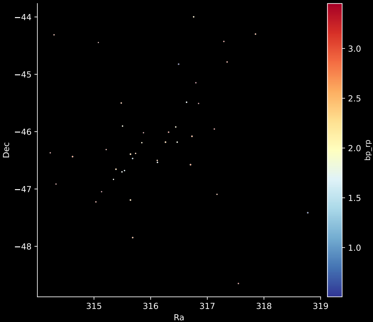
Gaia Cluster: [UPK_606] Stars: 41
