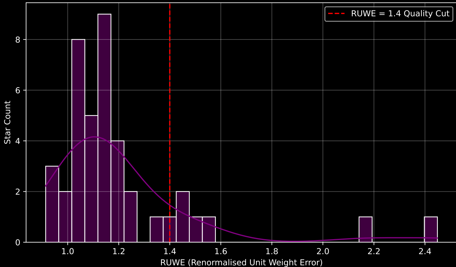
Gaia Cluster: [UPK_606] RUWE Distribution (n= 41)
