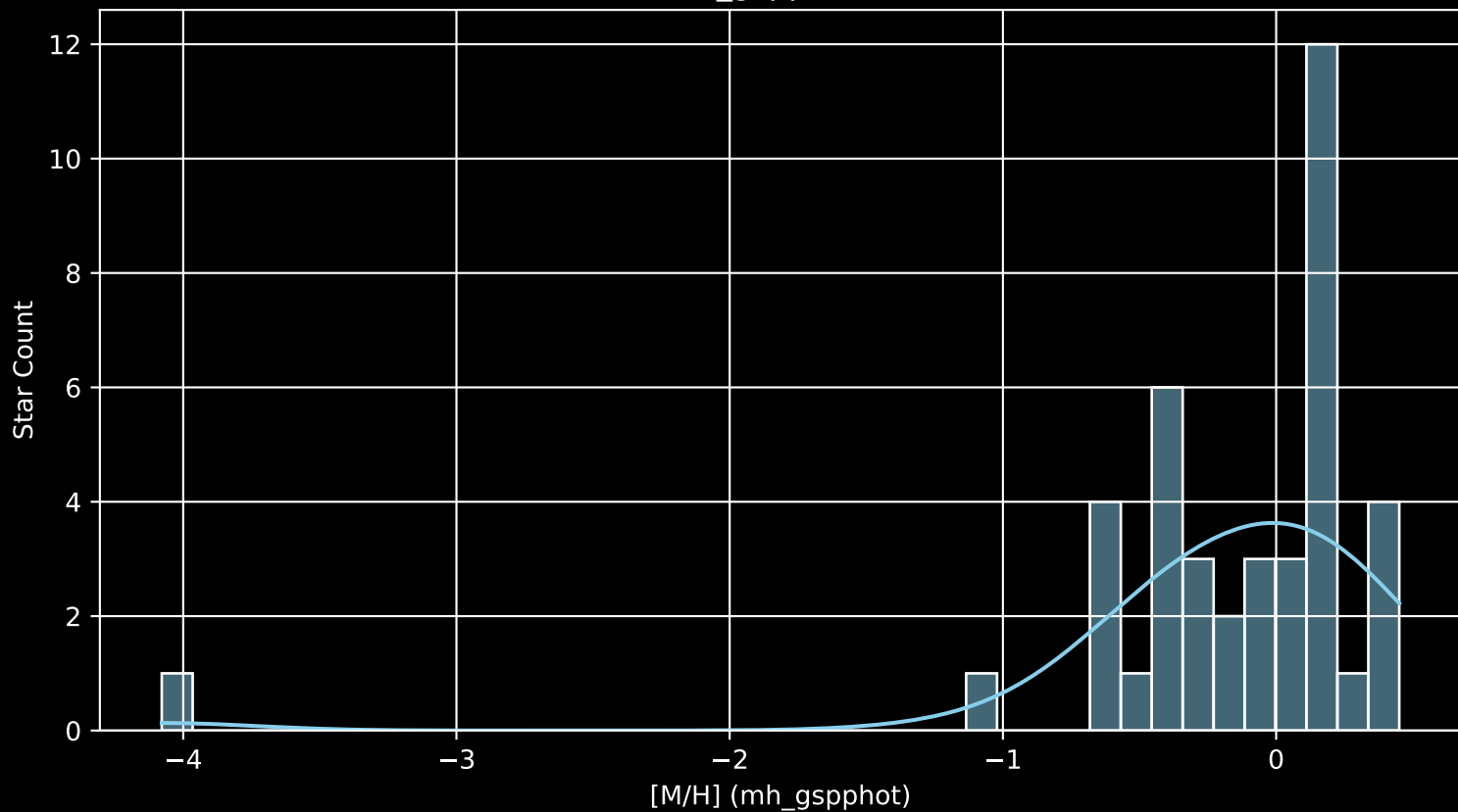
Gaia Cluster: [UPK_606 [M/H] (mh_gspphot) (n= 41)
