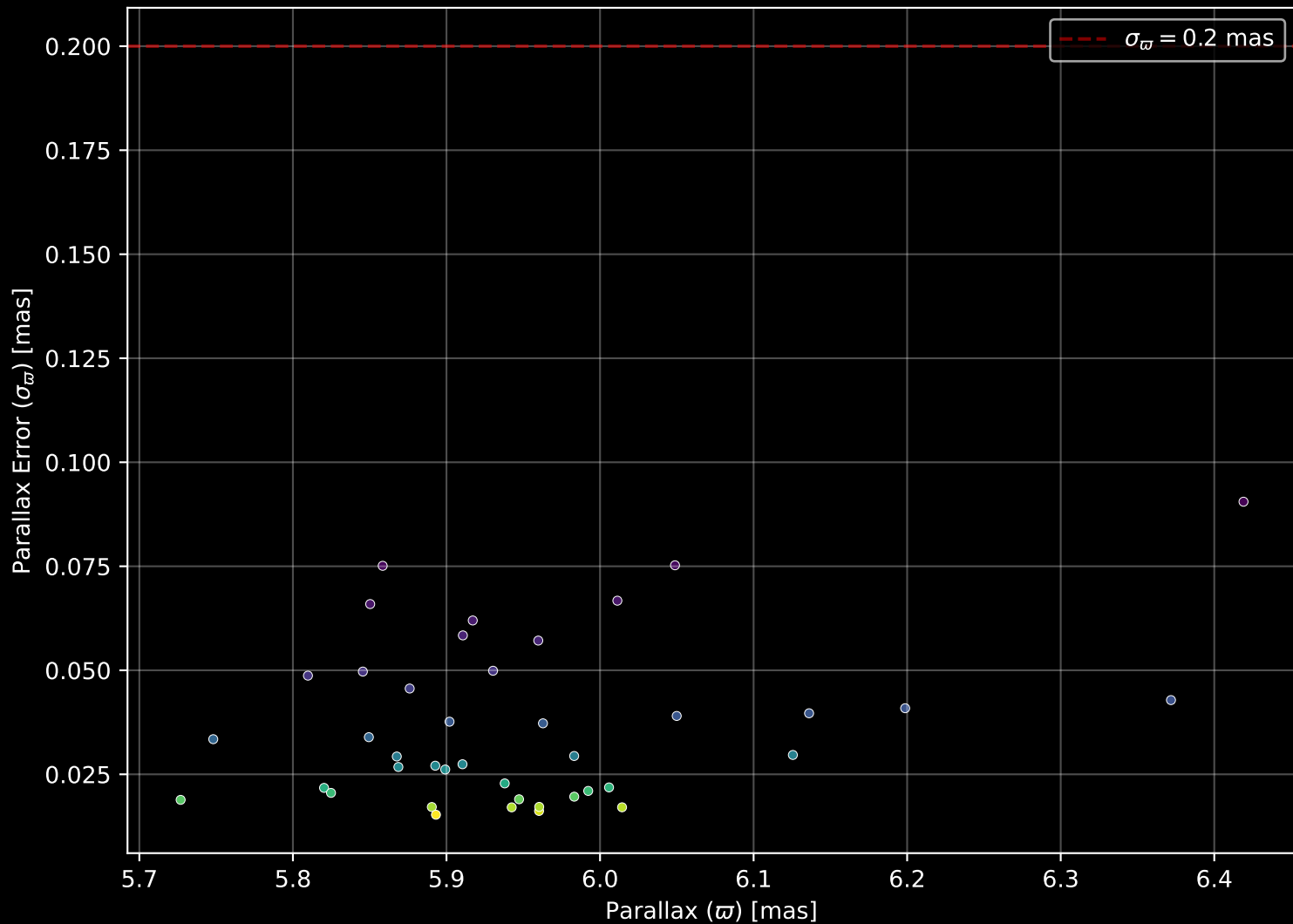
Gaia Cluster: [UPK_606] Parallax Quality (n= 41)
