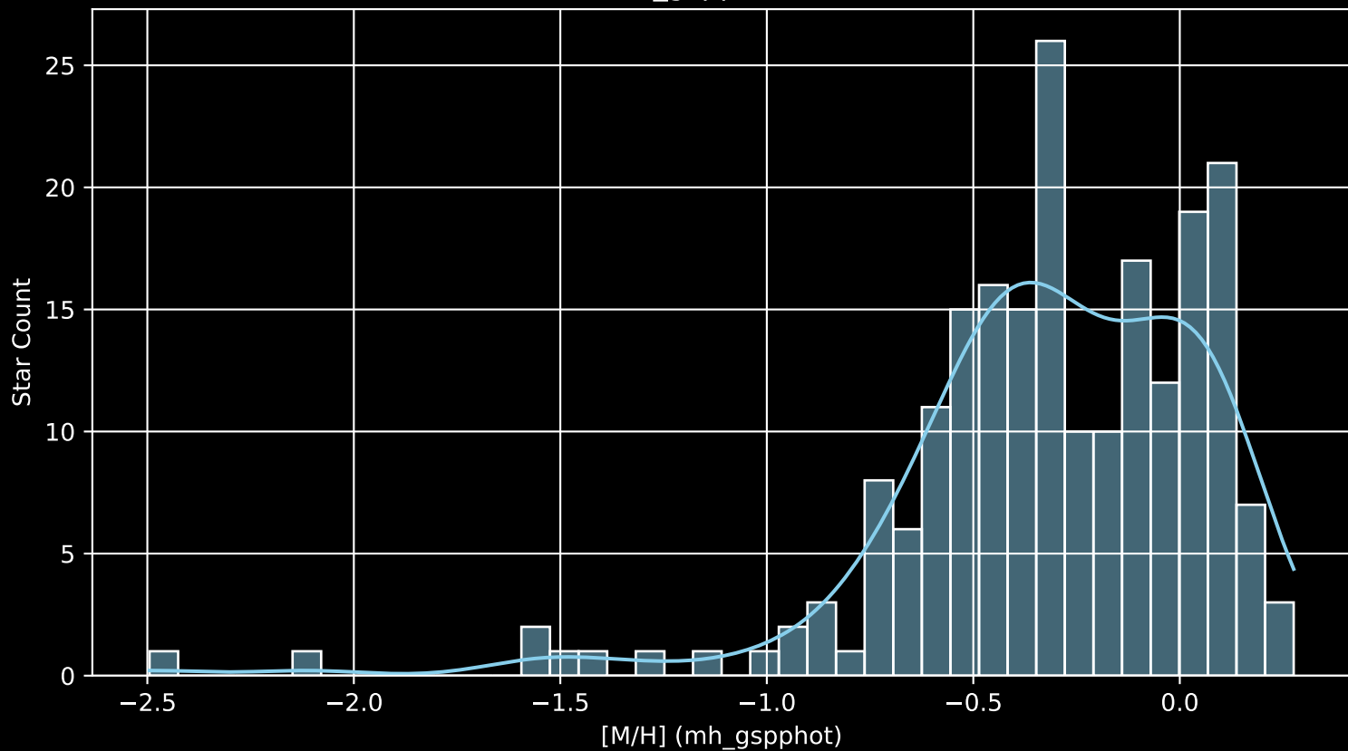
Gaia Cluster: [UPK_612 [M/H] (mh_gspphot) (n= 211)
