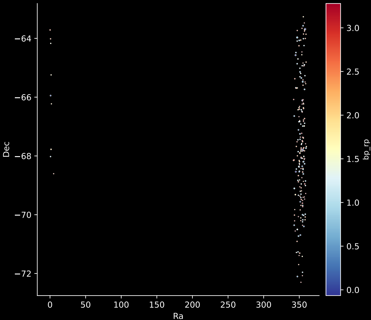
Gaia Cluster: [UPK_612] Stars: 211
