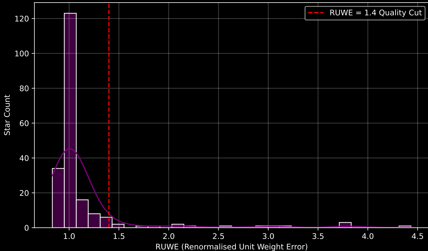
Gaia Cluster: [UPK_612] RUWE Distribution (n= 202)
