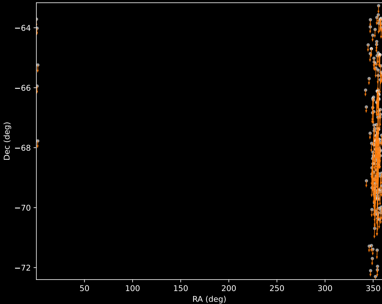
Gaia DR3 Cluster 2 Proper Motion Vectors (n=161)
