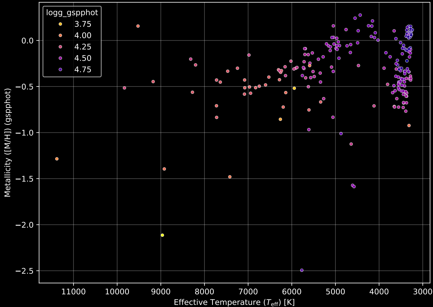
Gaia Cluster: [UPK_612] Stellar Population Parameters (n= 211)
