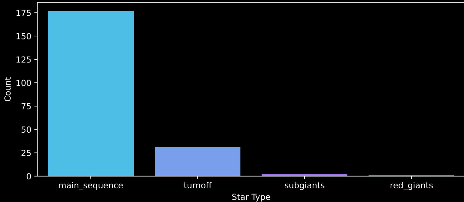
Gaia Cluster: [UPK_612] Count plot of Star Type
