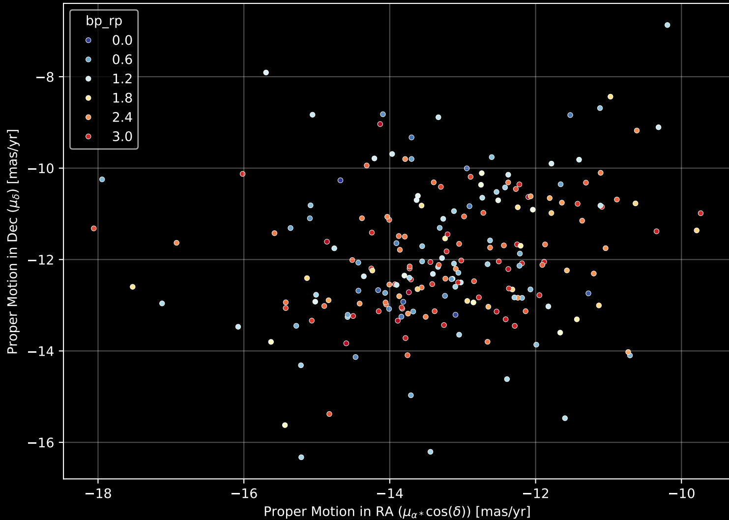
Gaia Cluster: [UPK_612] Proper Motion Diagram (n= 211)
