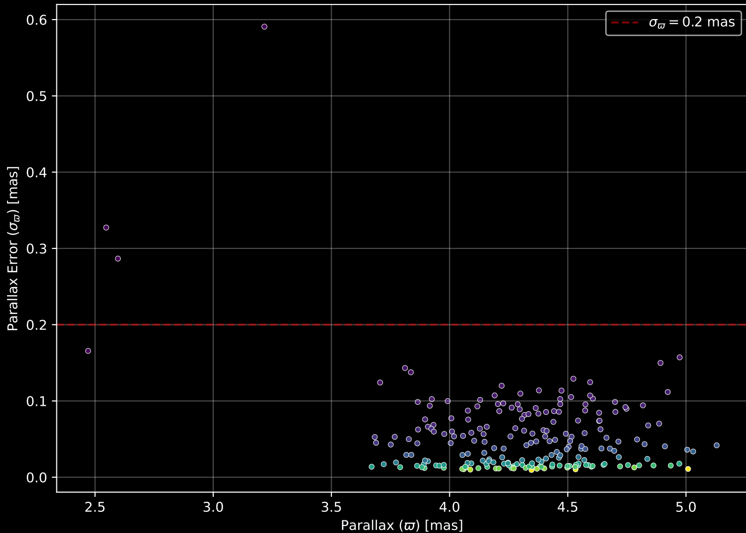
Gaia Cluster: [UPK_612] Parallax Quality (n= 211)
