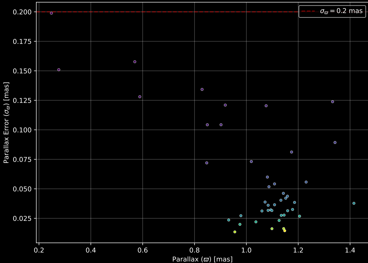
Gaia Cluster: [UPK_613] Parallax Quality (n= 45)
