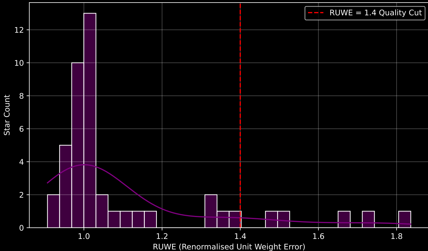
Gaia Cluster: [UPK_613] RUWE Distribution (n= 45)
