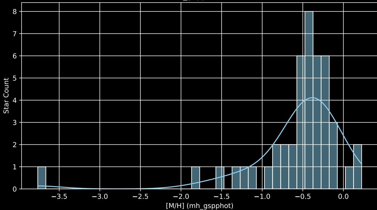
Gaia Cluster: [UPK_613 [M/H] (mh_gspphot) (n= 45)
