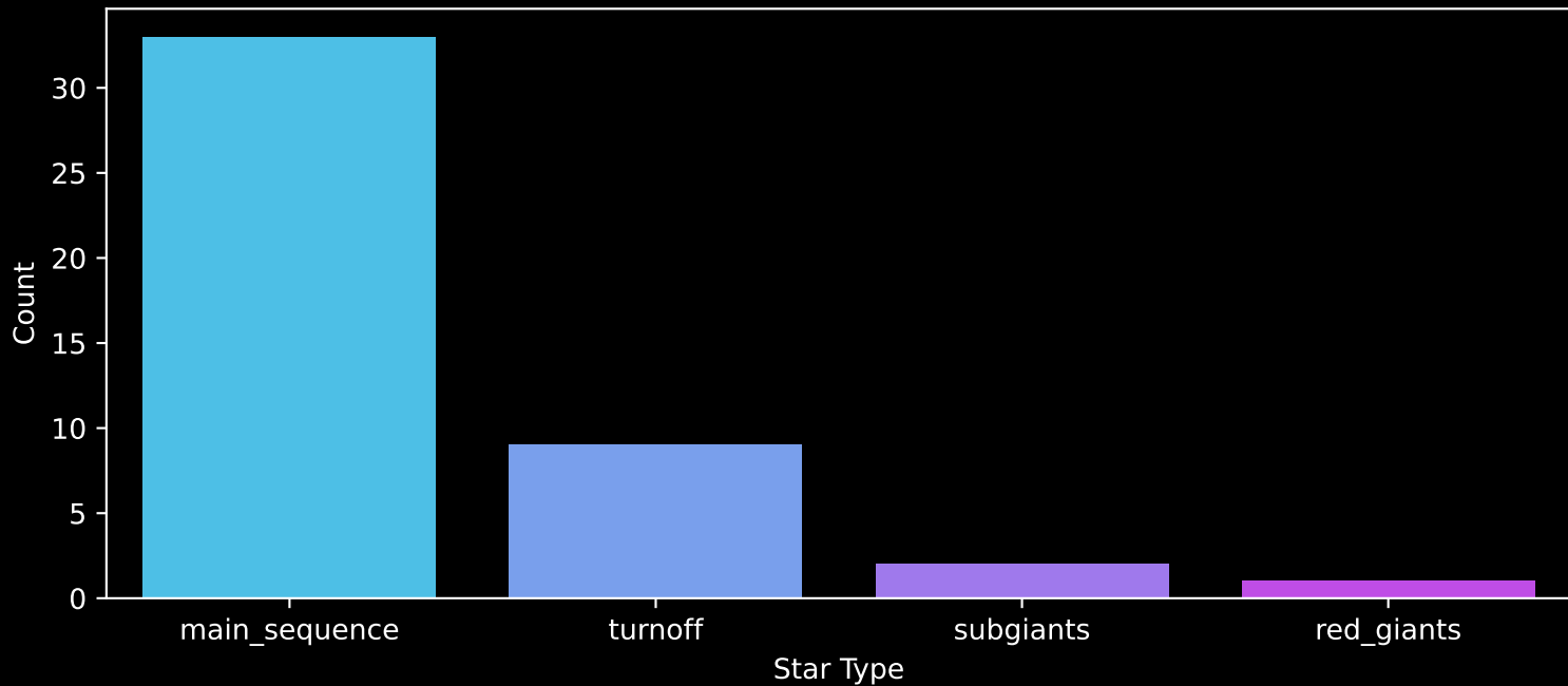
Gaia Cluster: [UPK_613] Count plot of Star Type
