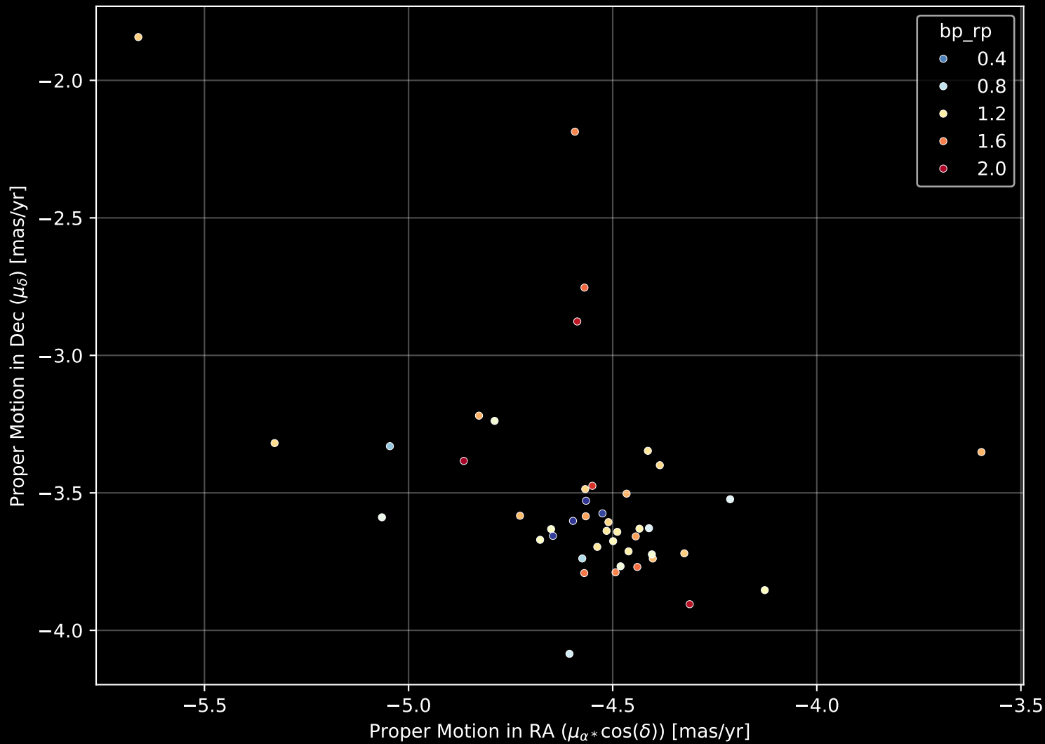
Gaia Cluster: [UPK_613] Proper Motion Diagram (n= 45)
