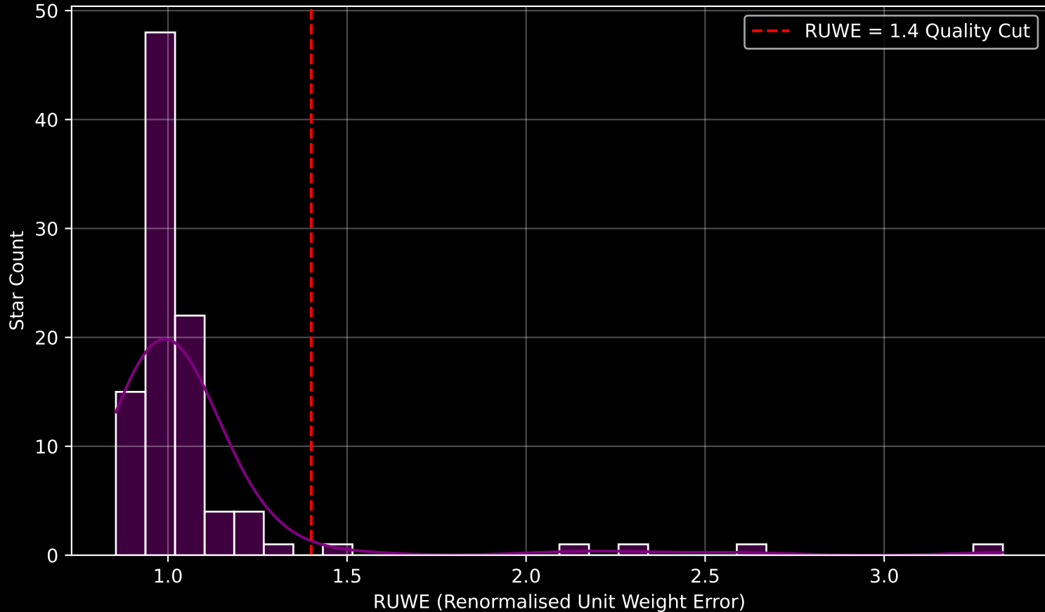
Gaia Cluster: [UPK_614] RUWE Distribution (n= 99)
