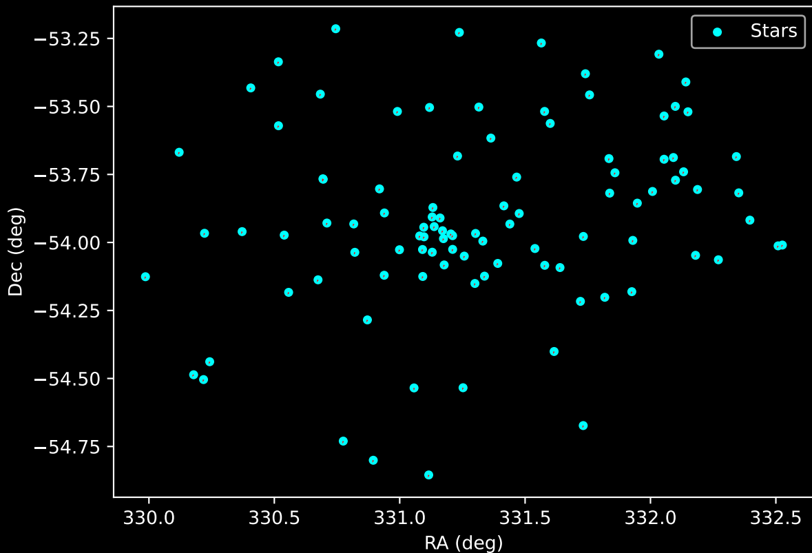
Gaia Cluster: [UPK_614] Proper Motion Vectors for Gaia Star Field (n= 99)
