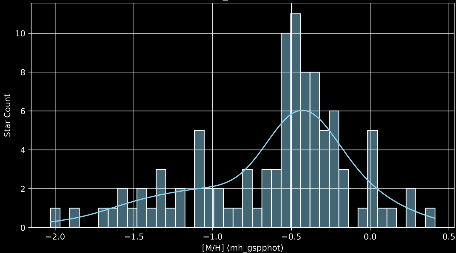
Gaia Cluster: [UPK_614 [M/H] (mh_gspphot) (n= 99)
