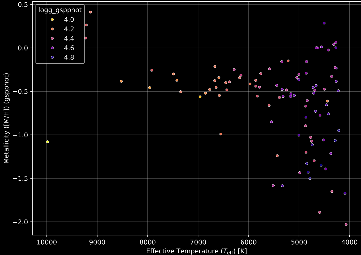
Gaia Cluster: [UPK_614] Stellar Population Parameters (n= 99)
