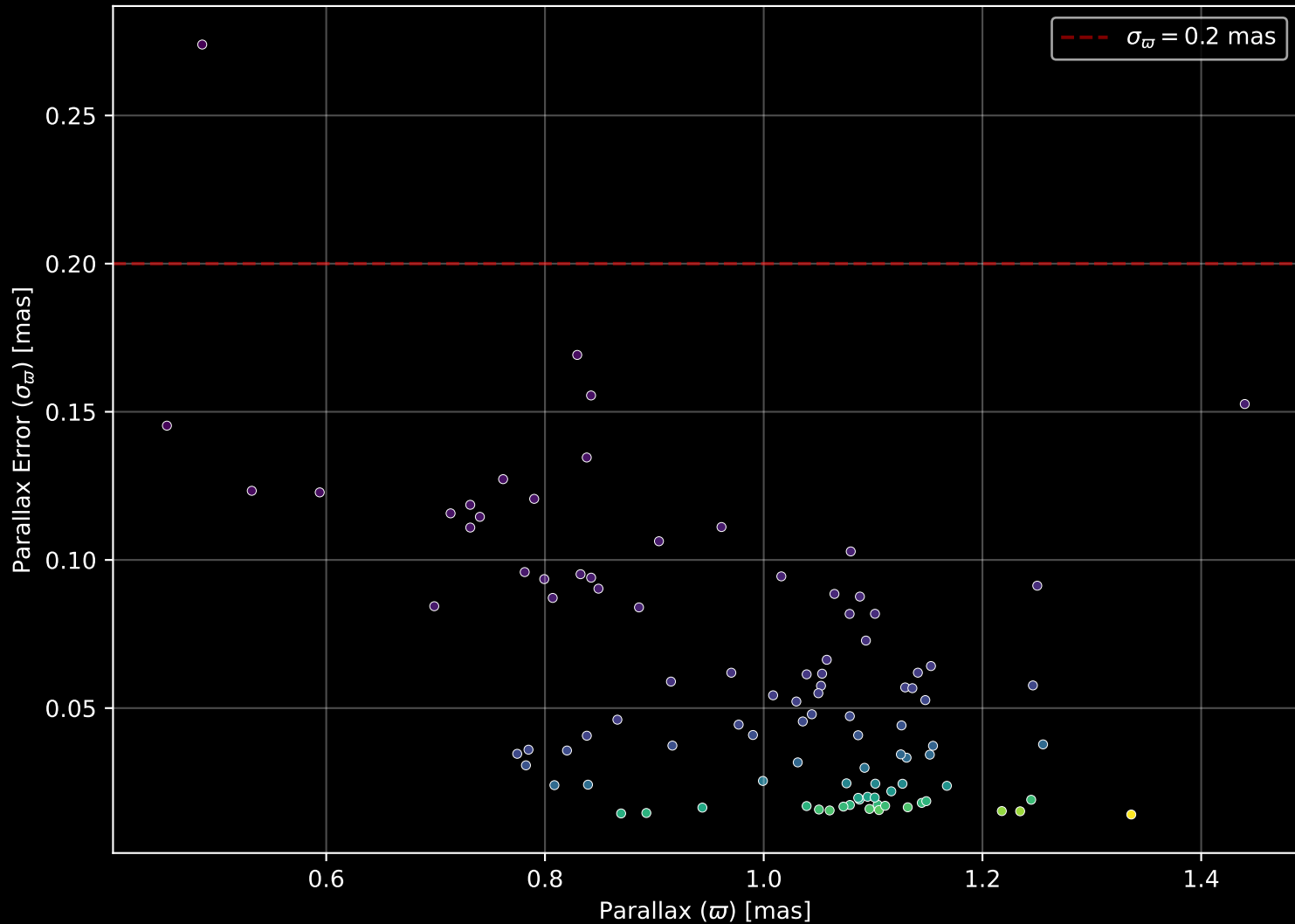
Gaia Cluster: [UPK_614] Parallax Quality (n= 99)
