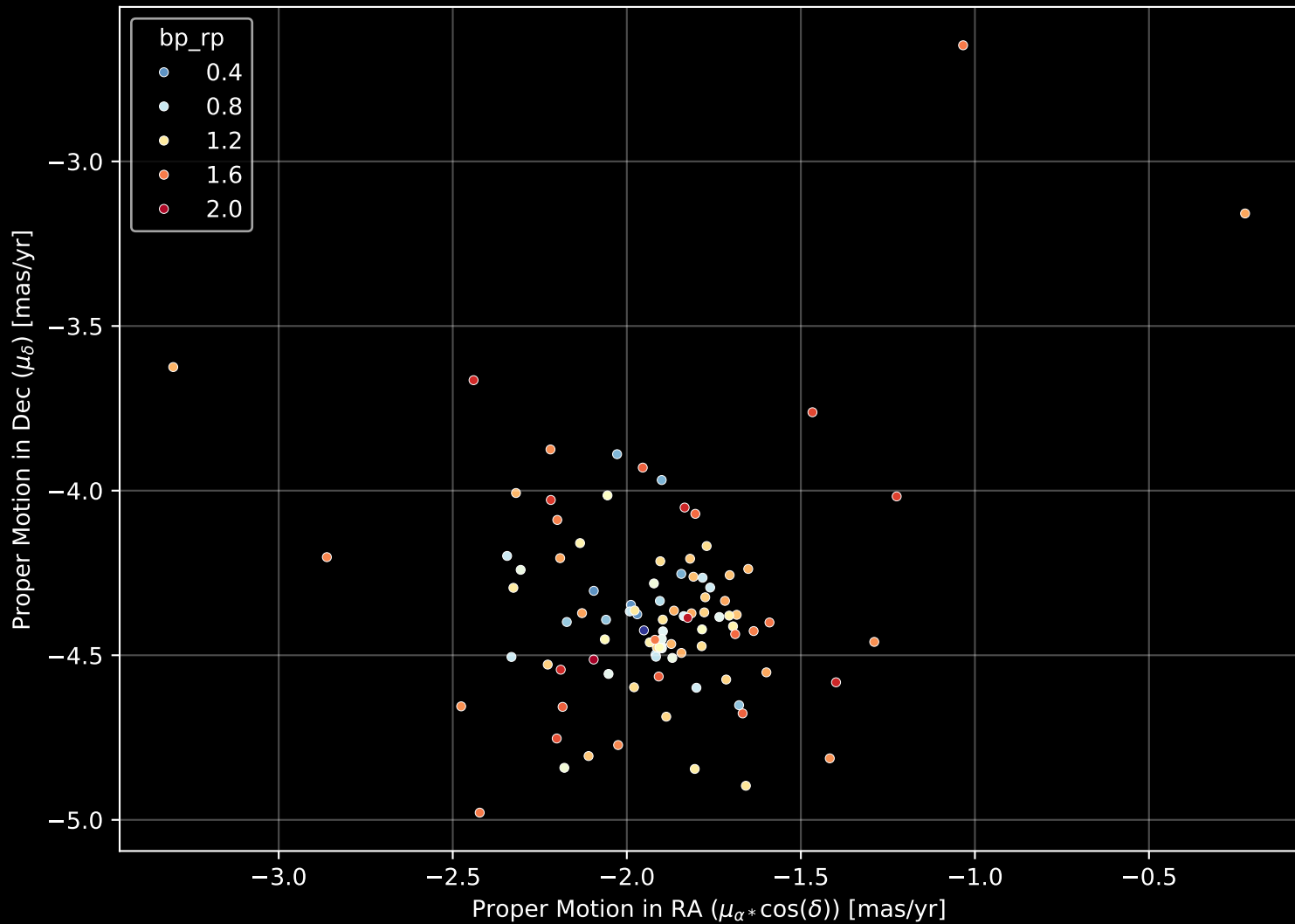
Gaia Cluster: [UPK_614] Proper Motion Diagram (n= 99)
