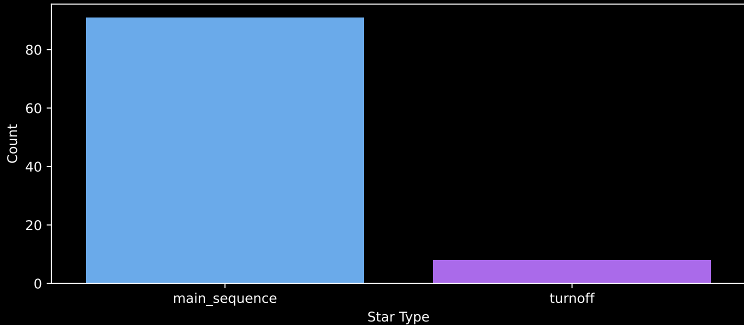
Gaia Cluster: [UPK_614] Count plot of Star Type
