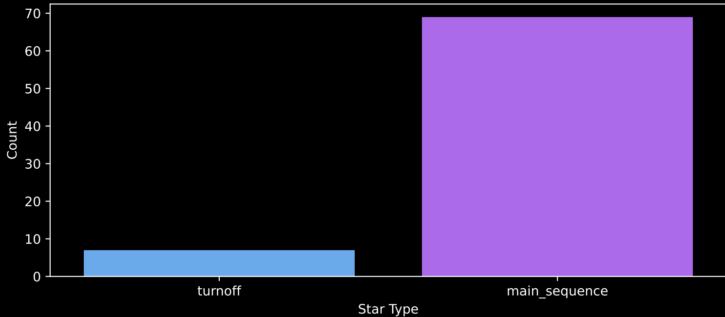
Gaia Cluster: [UPK_617] Count plot of Star Type
