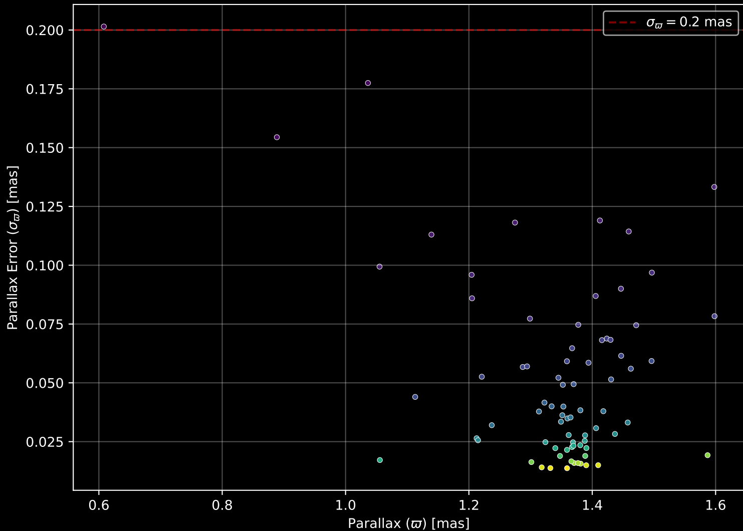
Gaia Cluster: [UPK_617] Parallax Quality (n= 76)
