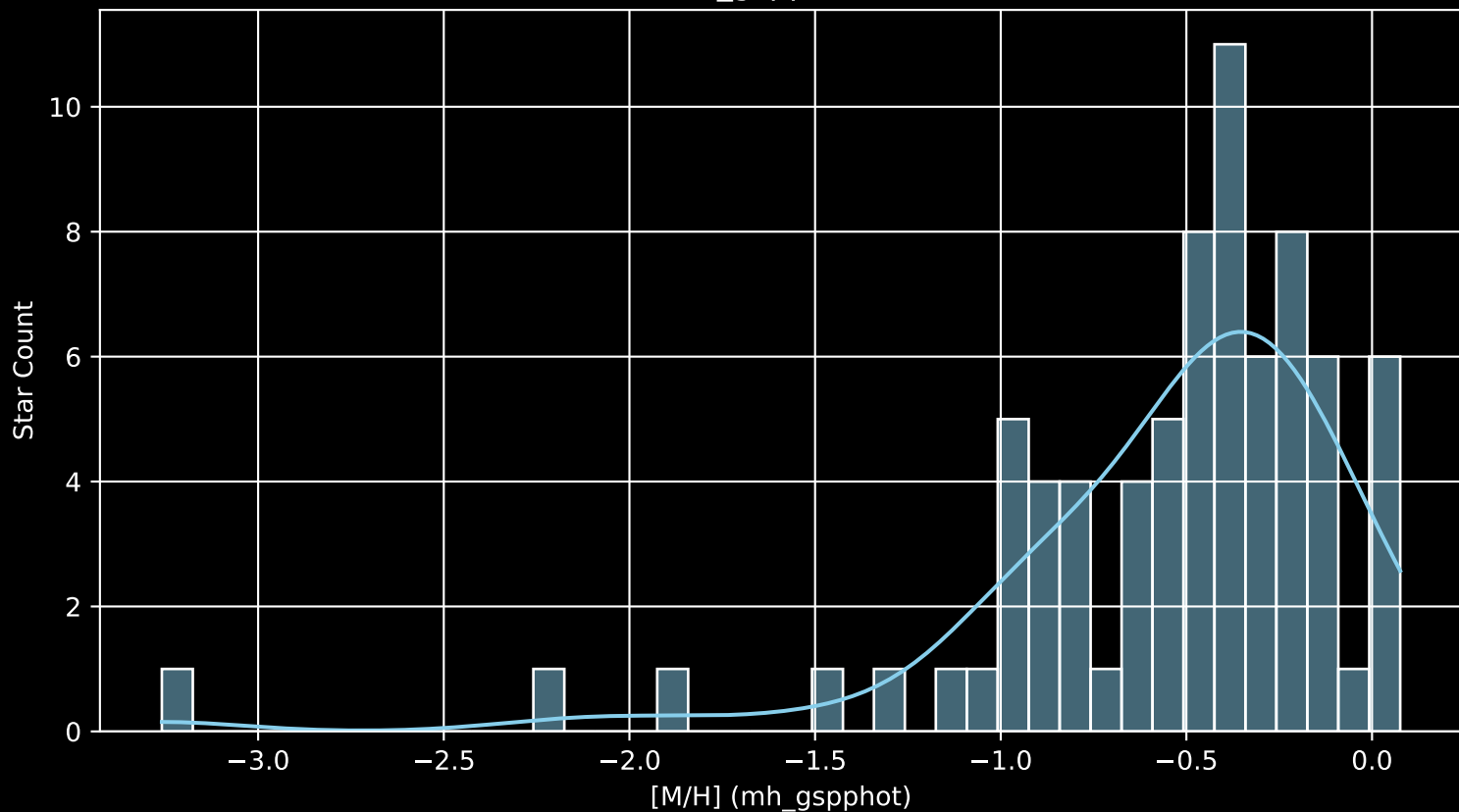
Gaia Cluster: [UPK_617 [M/H] (mh_gspphot) (n= 76)
