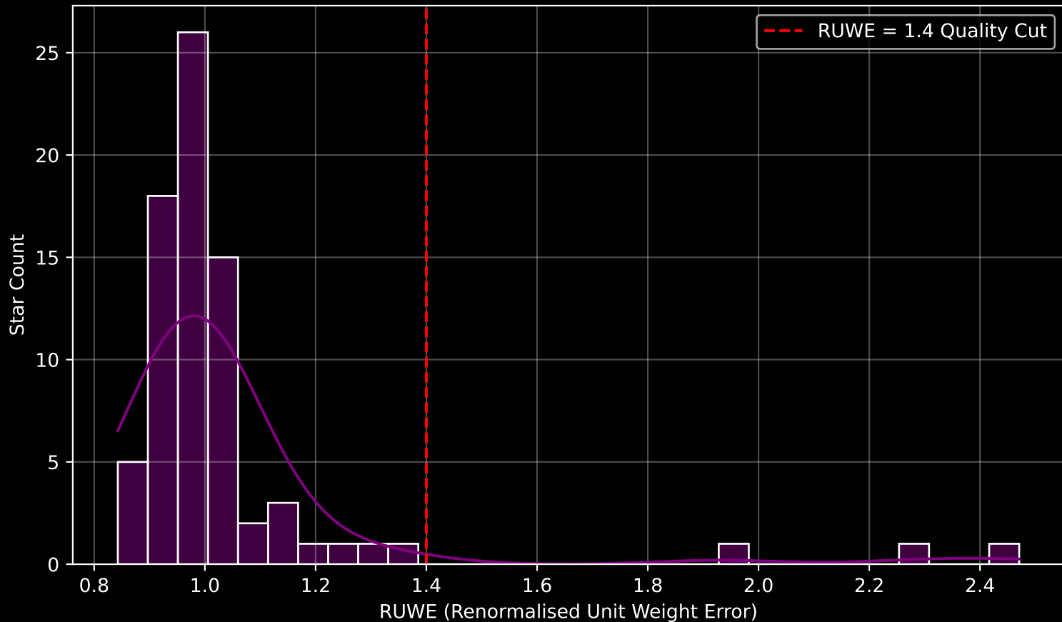
Gaia Cluster: [UPK_617] RUWE Distribution (n= 76)
