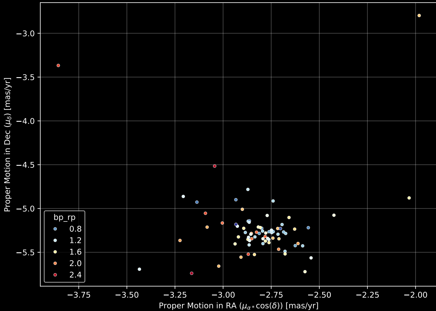
Gaia Cluster: [UPK_617] Proper Motion Diagram (n= 76)
