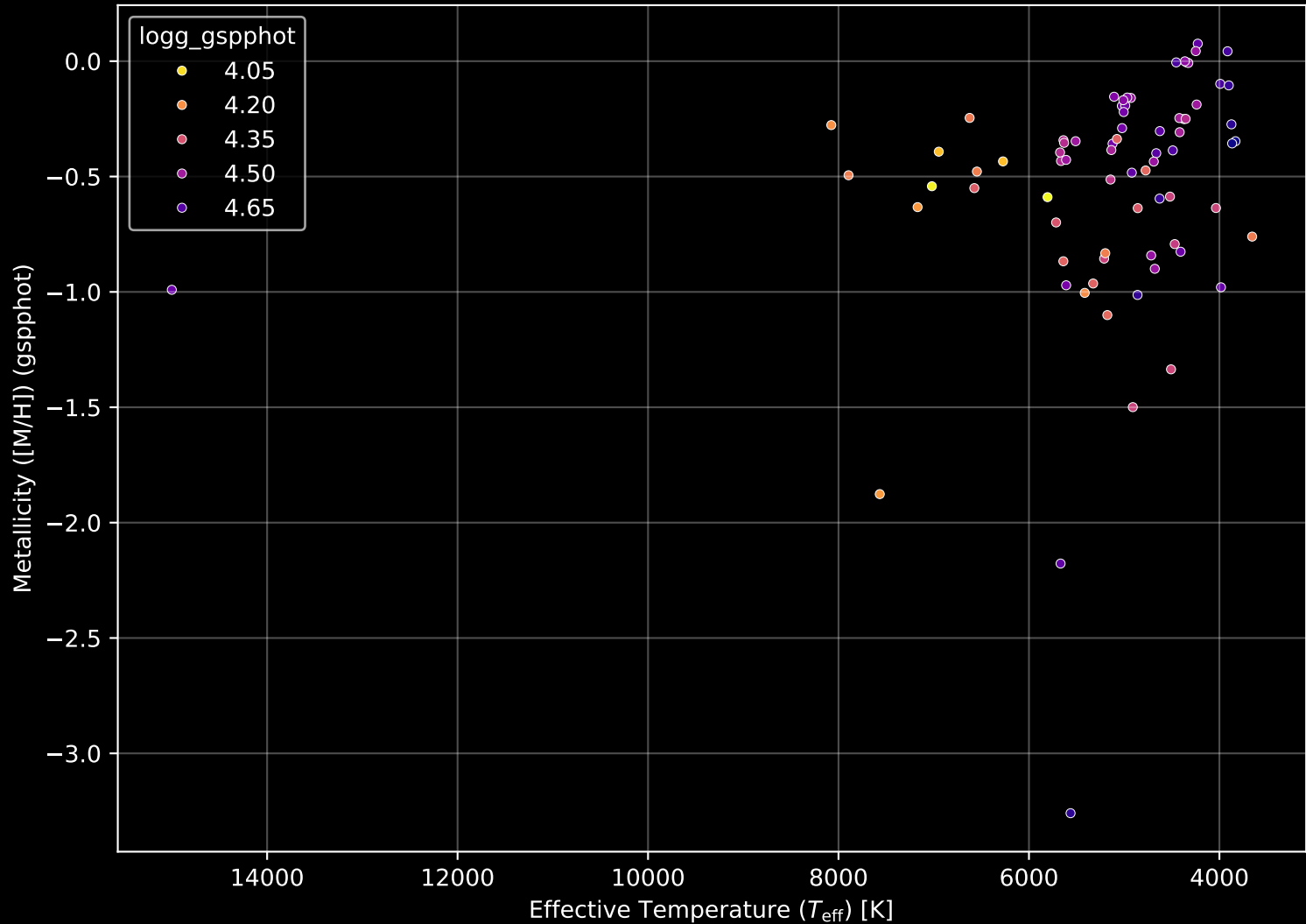
Gaia Cluster: [UPK_617] Stellar Population Parameters (n= 76)
