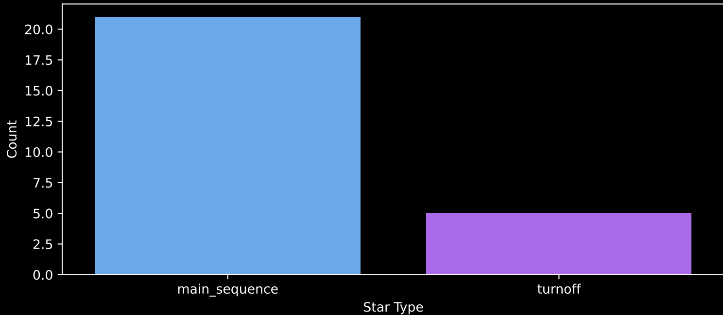
Gaia Cluster: [UPK_624] Count plot of Star Type
