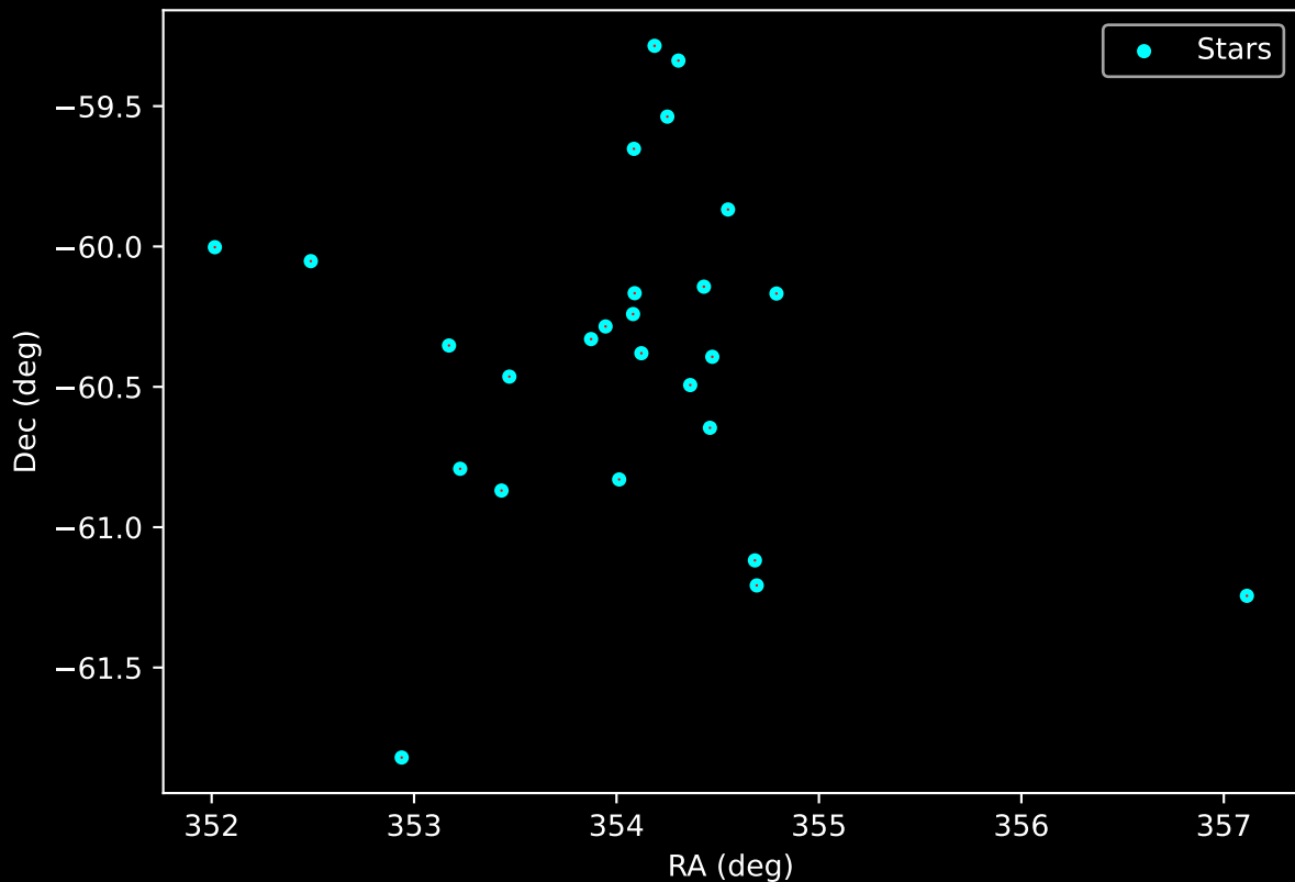
Gaia Cluster: [UPK_624] Proper Motion Vectors for Gaia Star Field (n= 26)
