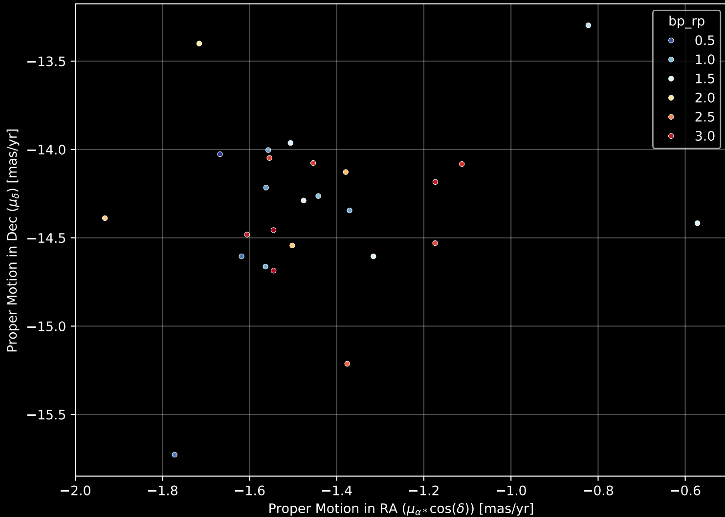
Gaia Cluster: [UPK_624] Proper Motion Diagram (n= 26)
