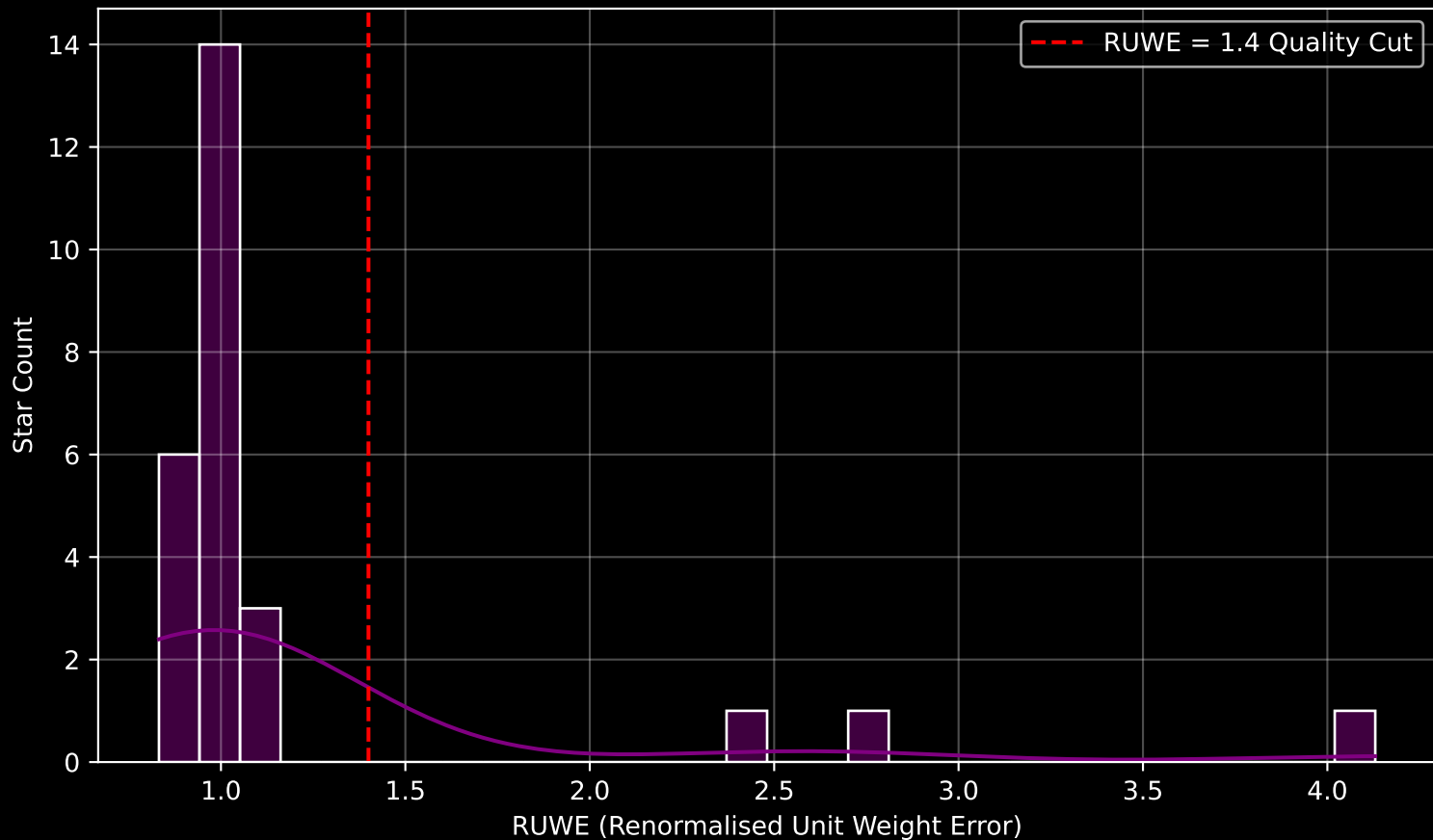
Gaia Cluster: [UPK_624] RUWE Distribution (n= 26)
