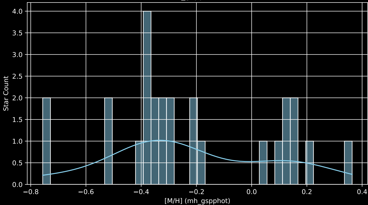
Gaia Cluster: [UPK_624 [M/H] (mh_gspphot) (n= 26)
