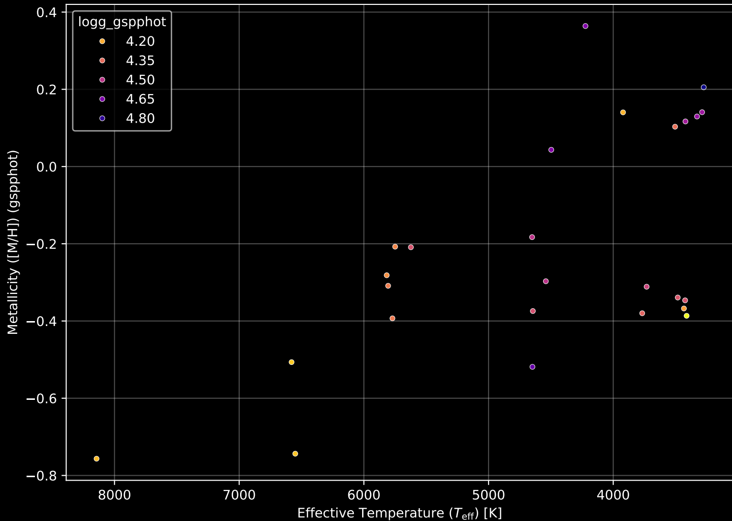
Gaia Cluster: [UPK_624] Stellar Population Parameters (n= 26)
