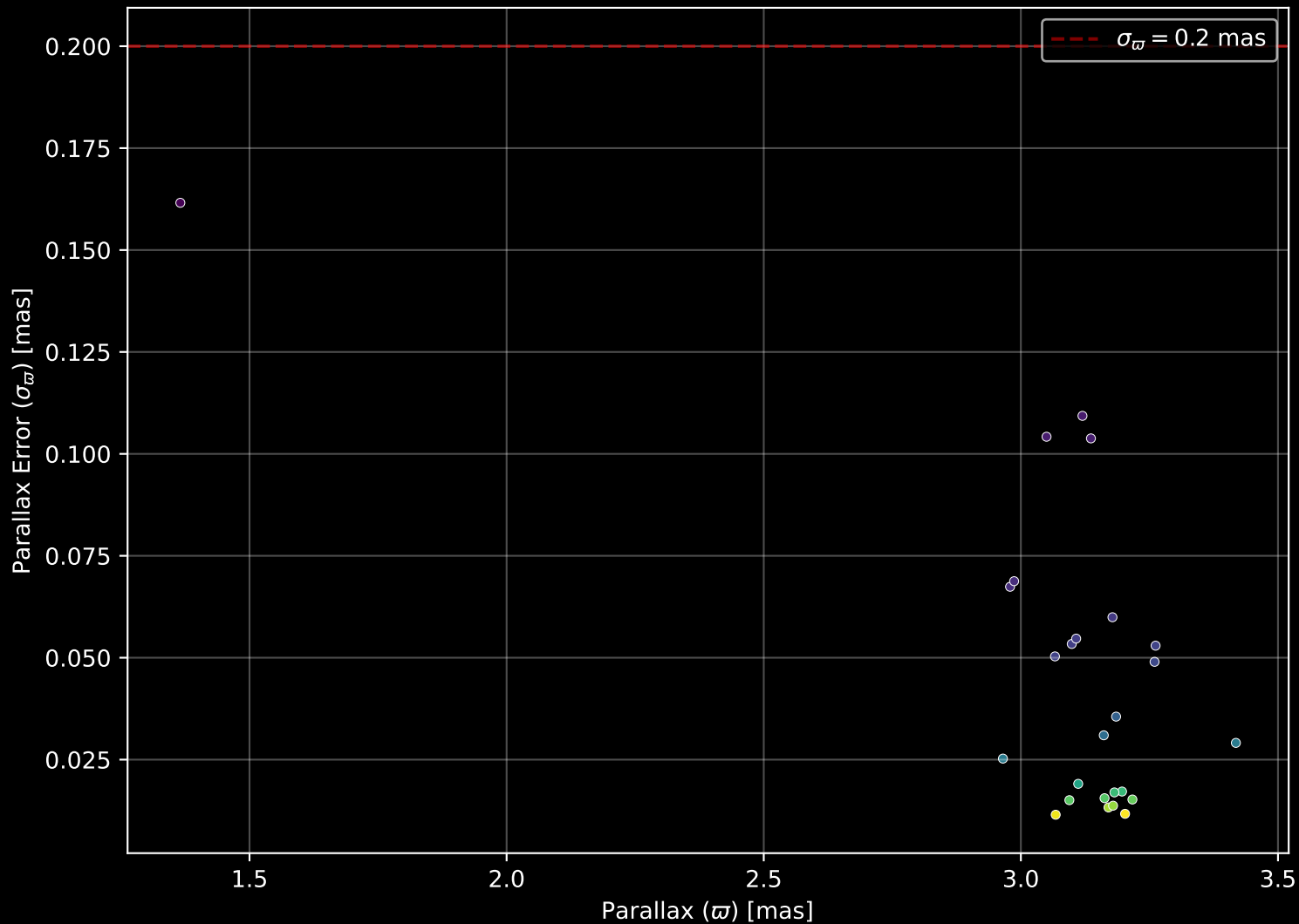
Gaia Cluster: [UPK_624] Parallax Quality (n= 26)
