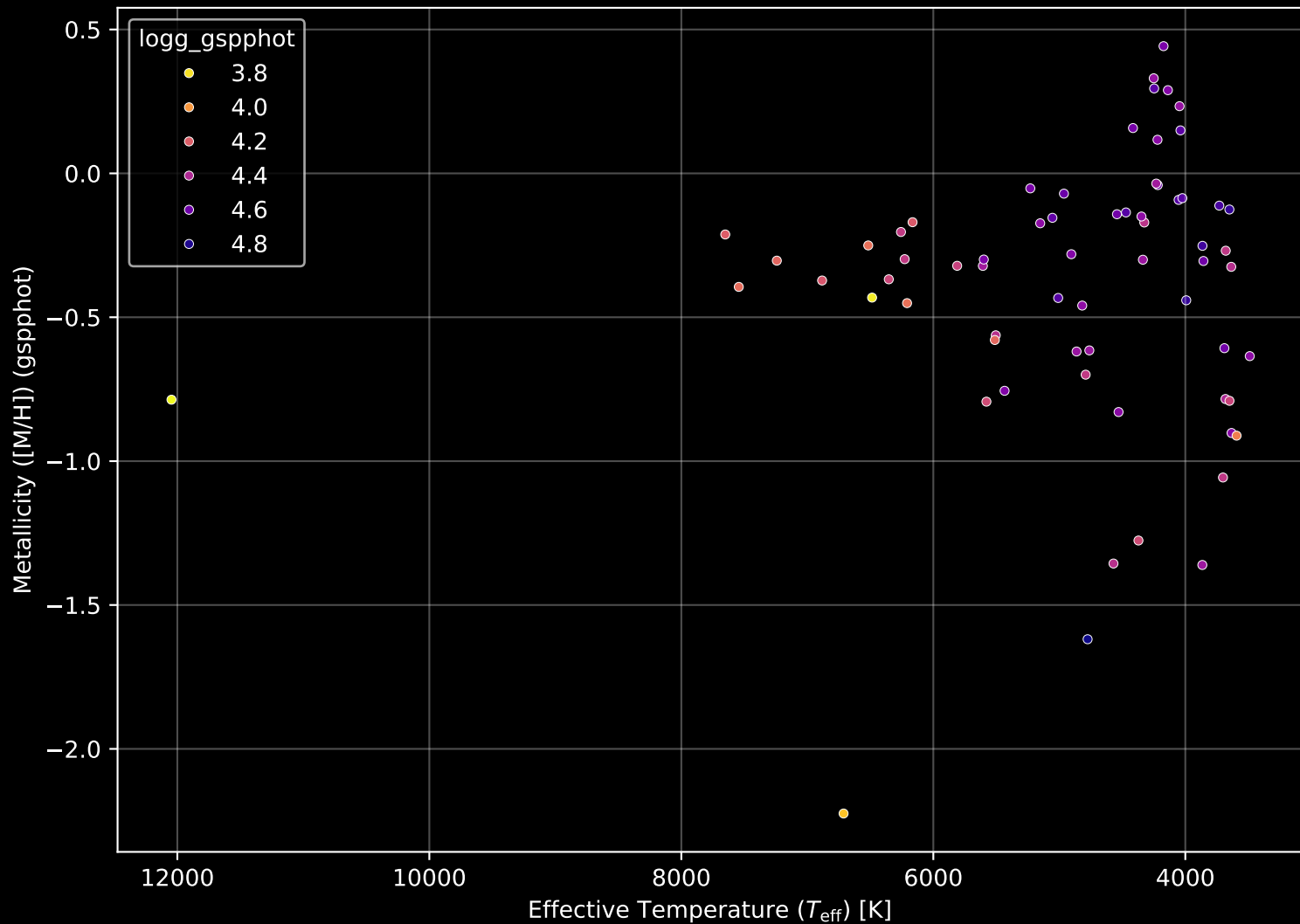
Gaia Cluster: [UPK_627] Stellar Population Parameters (n= 66)
