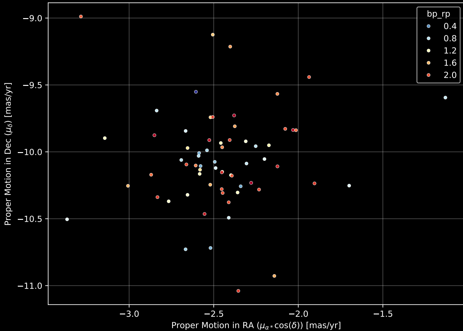
Gaia Cluster: [UPK_627] Proper Motion Diagram (n= 66)
