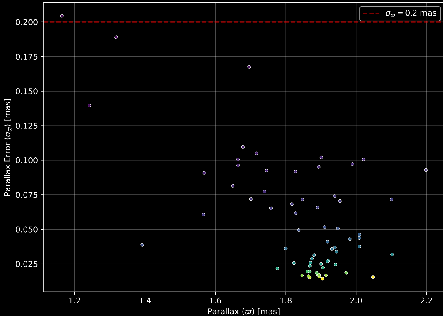
Gaia Cluster: [UPK_627] Parallax Quality (n= 66)
