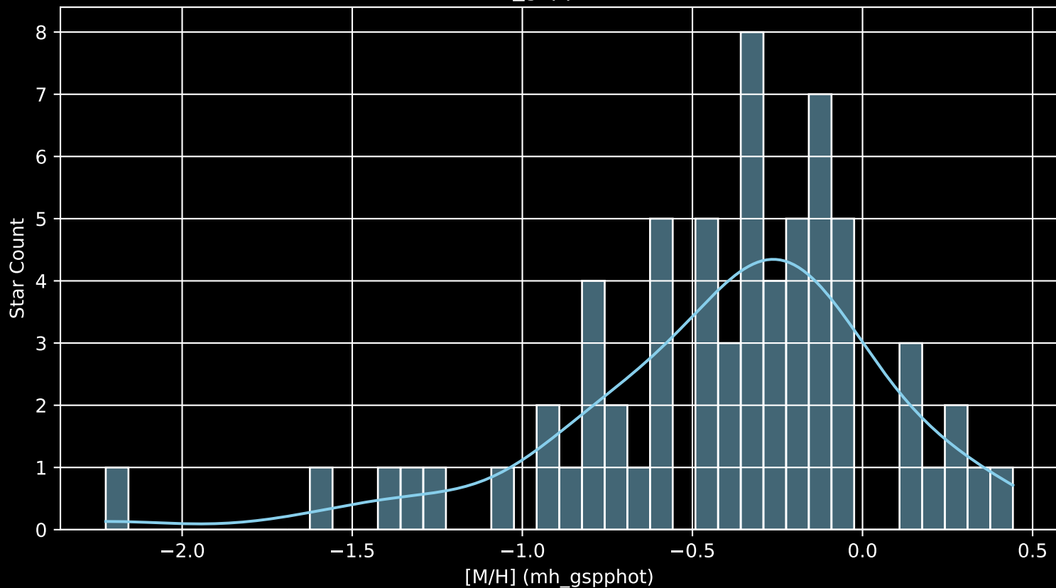
Gaia Cluster: [UPK_627 [M/H] (mh_gspphot) (n= 66)
