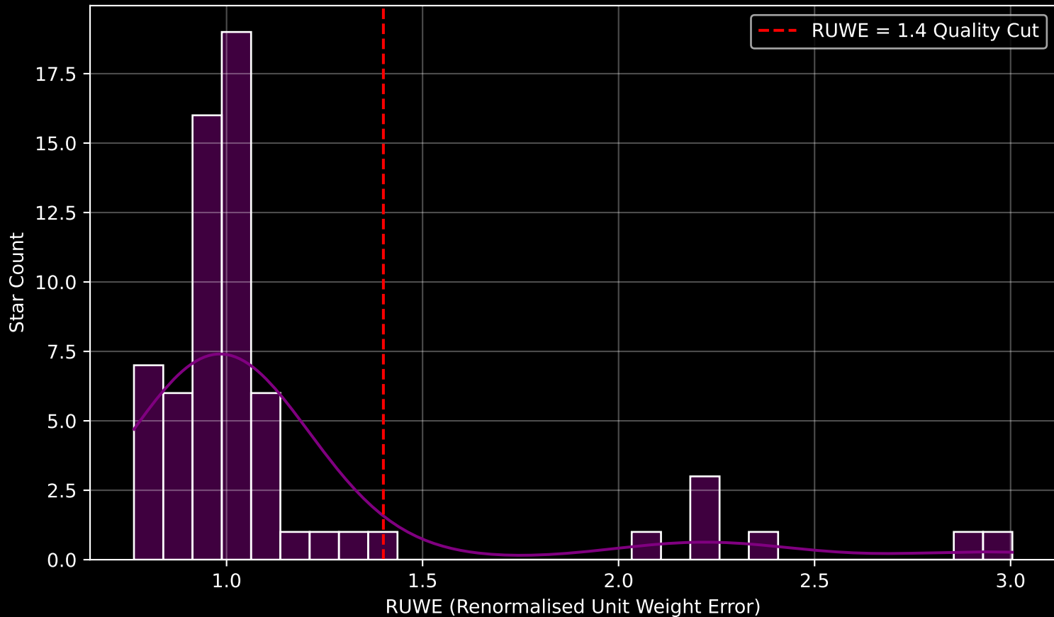
Gaia Cluster: [UPK_627] RUWE Distribution (n= 65)
