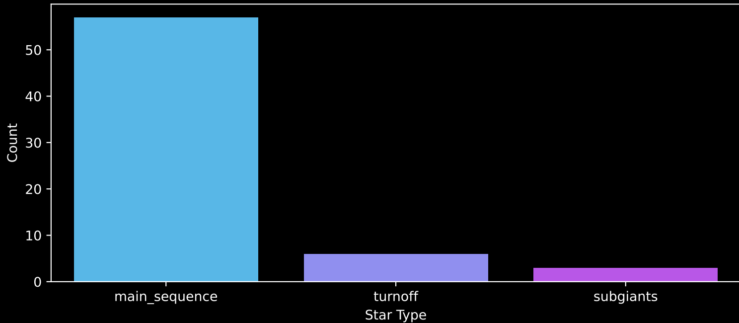
Gaia Cluster: [UPK_627] Count plot of Star Type
