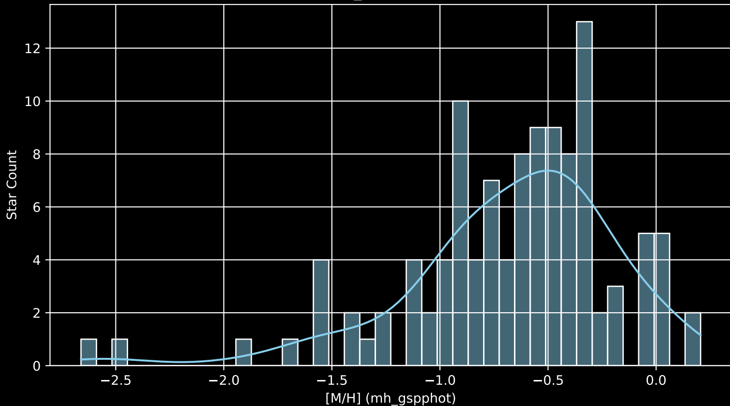
Gaia Cluster: [UPK_629 [M/H] (mh_gspphot) (n= 112)
