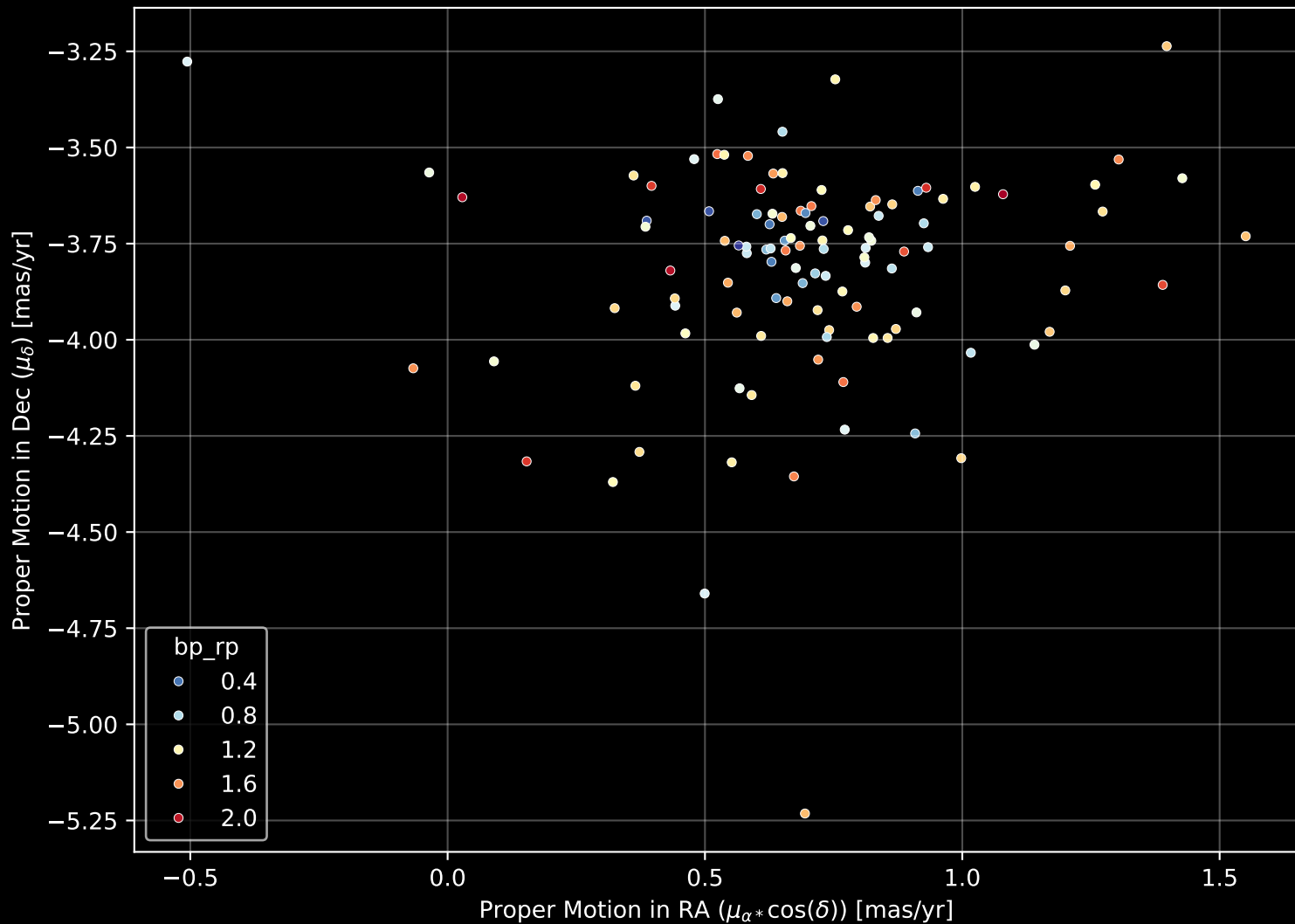
Gaia Cluster: [UPK_629] Proper Motion Diagram (n= 112)
