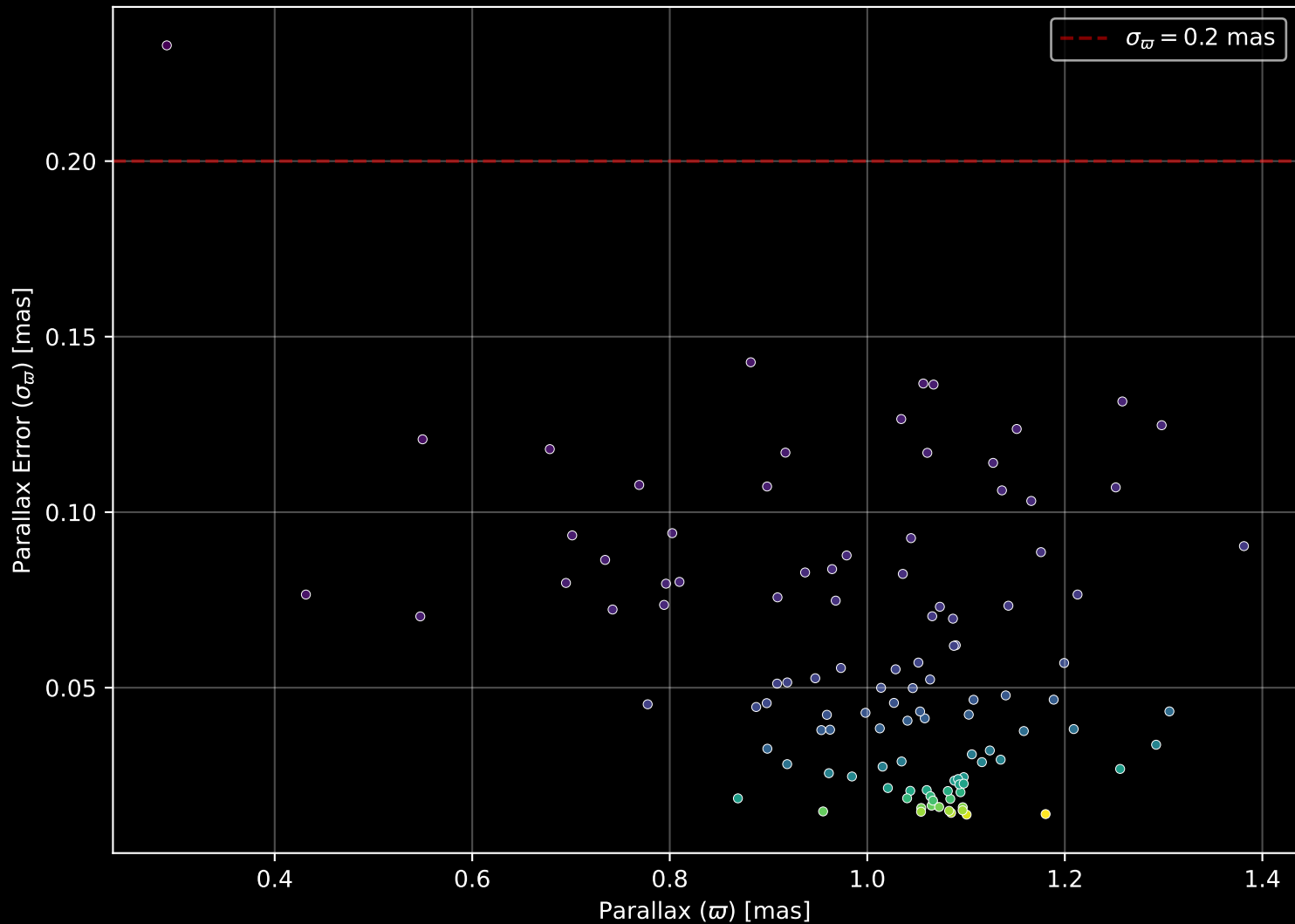
Gaia Cluster: [UPK_629] Parallax Quality (n= 112)
