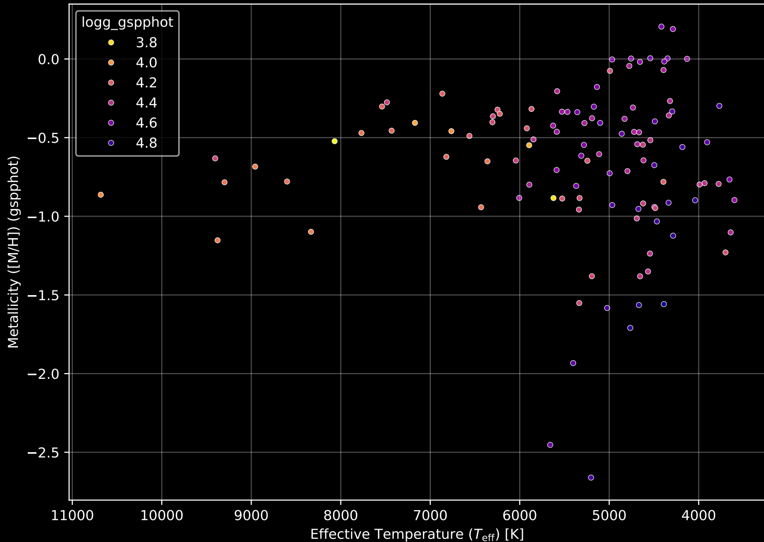
Gaia Cluster: [UPK_629] Stellar Population Parameters (n= 112)
