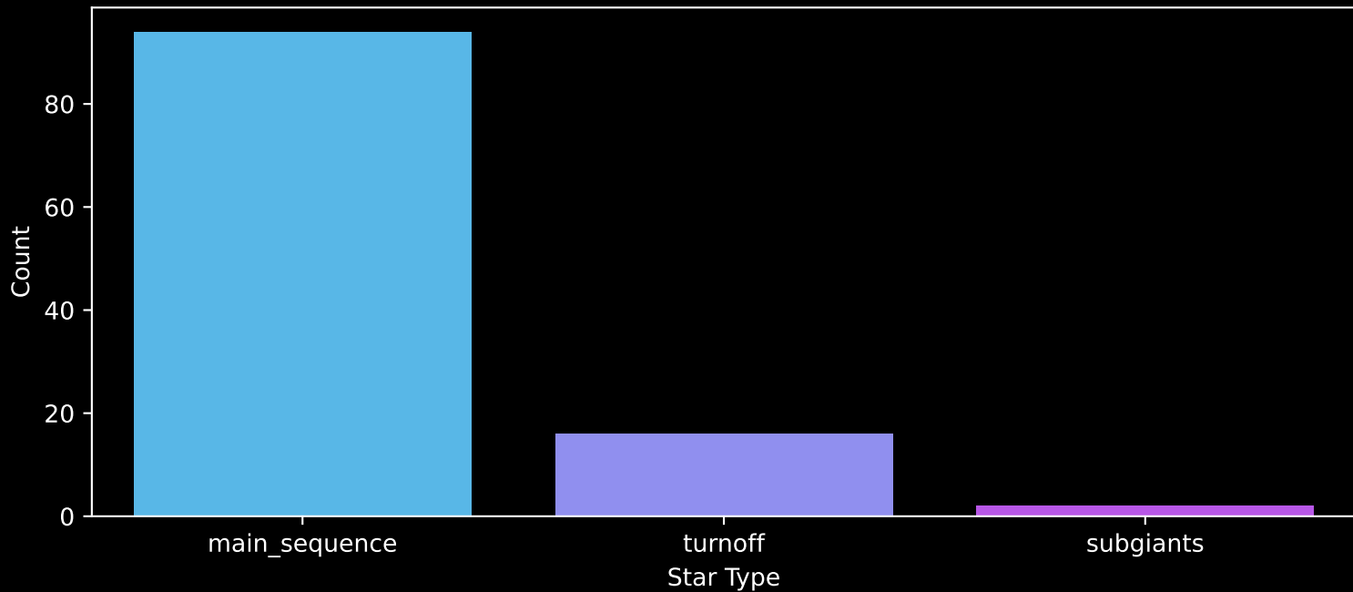
Gaia Cluster: [UPK_629] Count plot of Star Type
