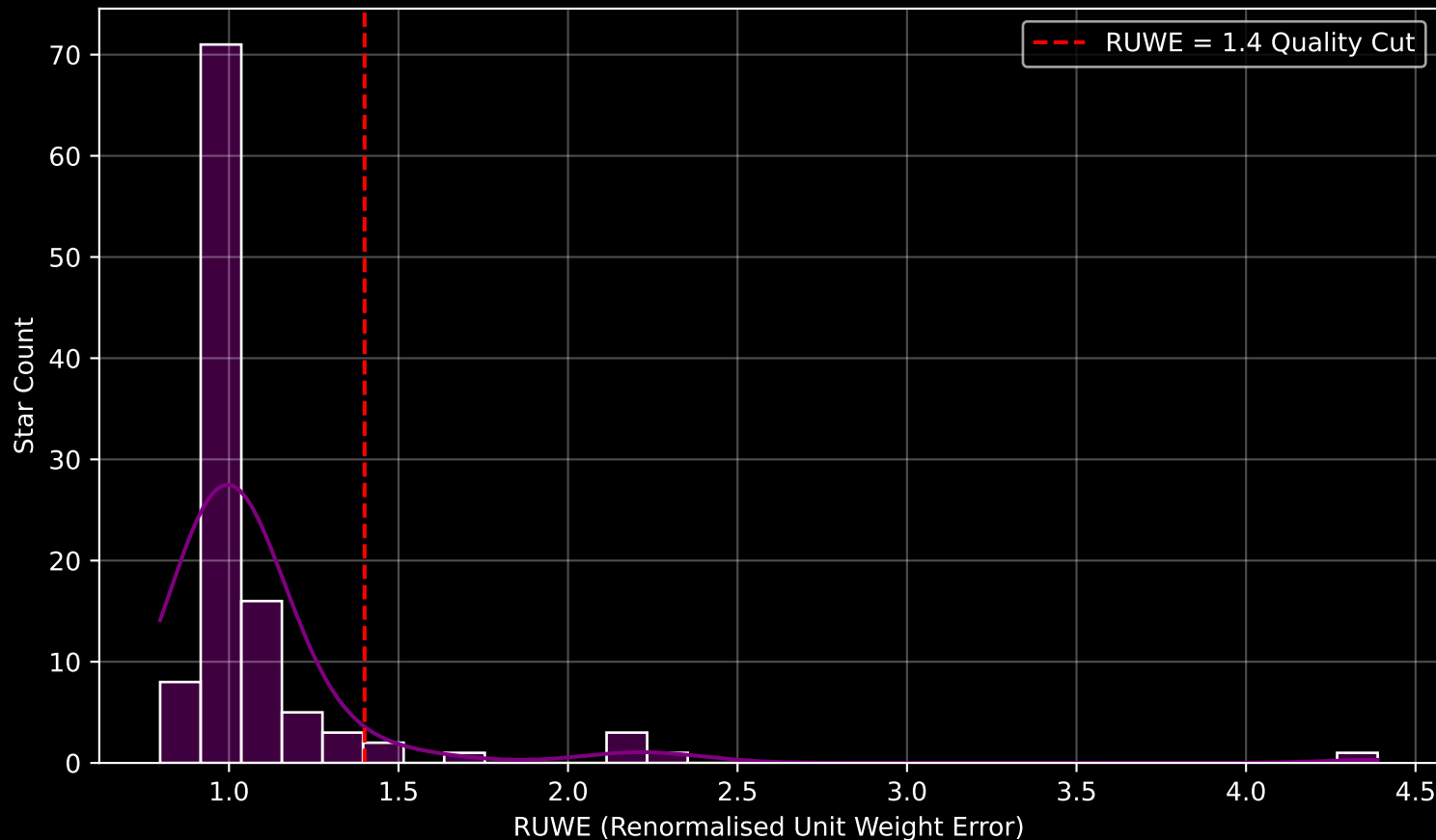
Gaia Cluster: [UPK_629] RUWE Distribution (n= 111)
