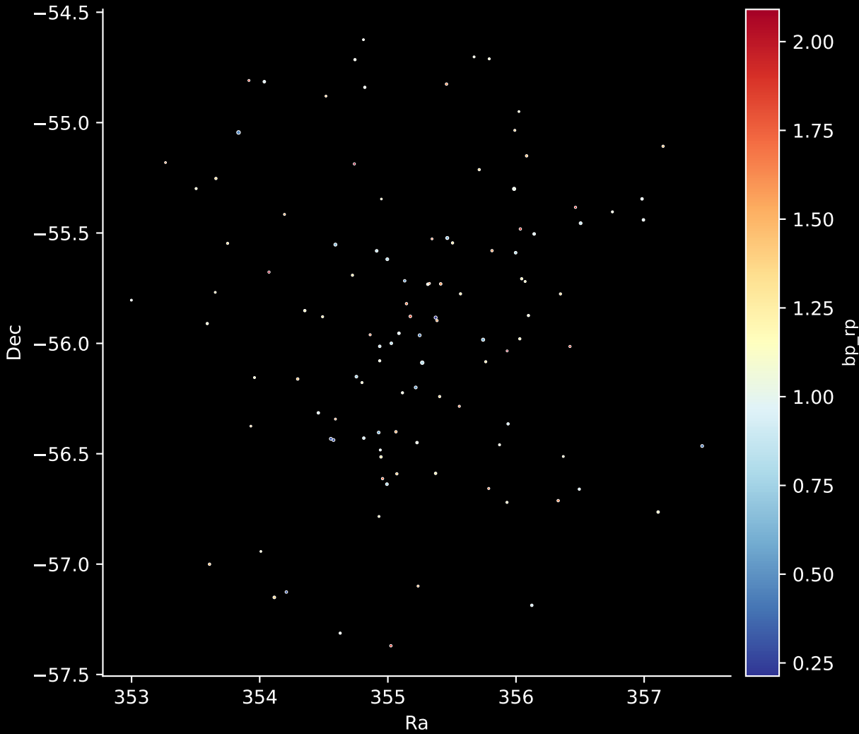
Gaia Cluster: [UPK_629] Stars: 112
