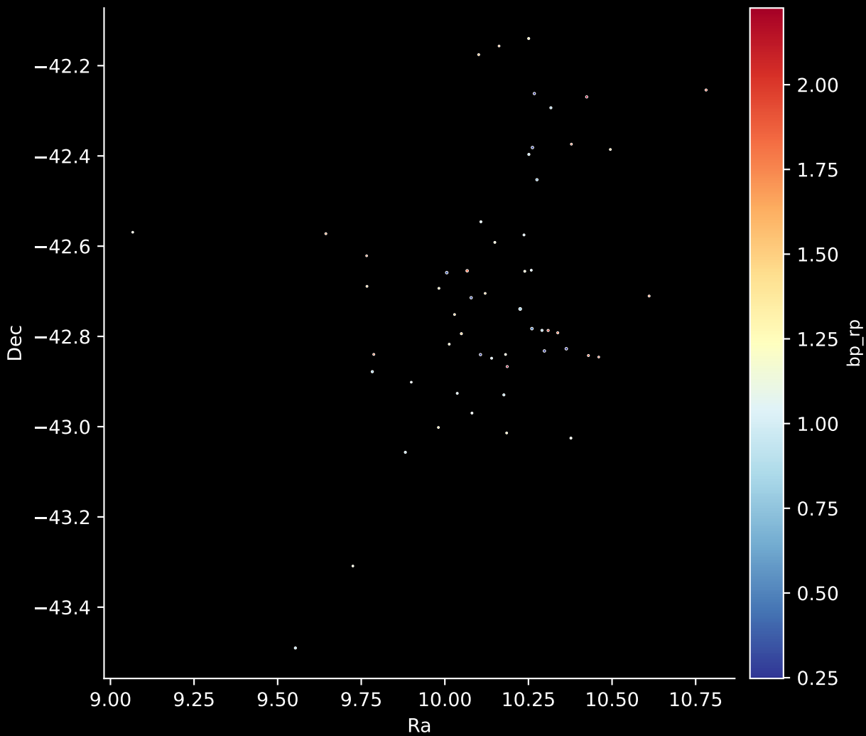
Gaia Cluster: [UPK_645] Stars: 55
