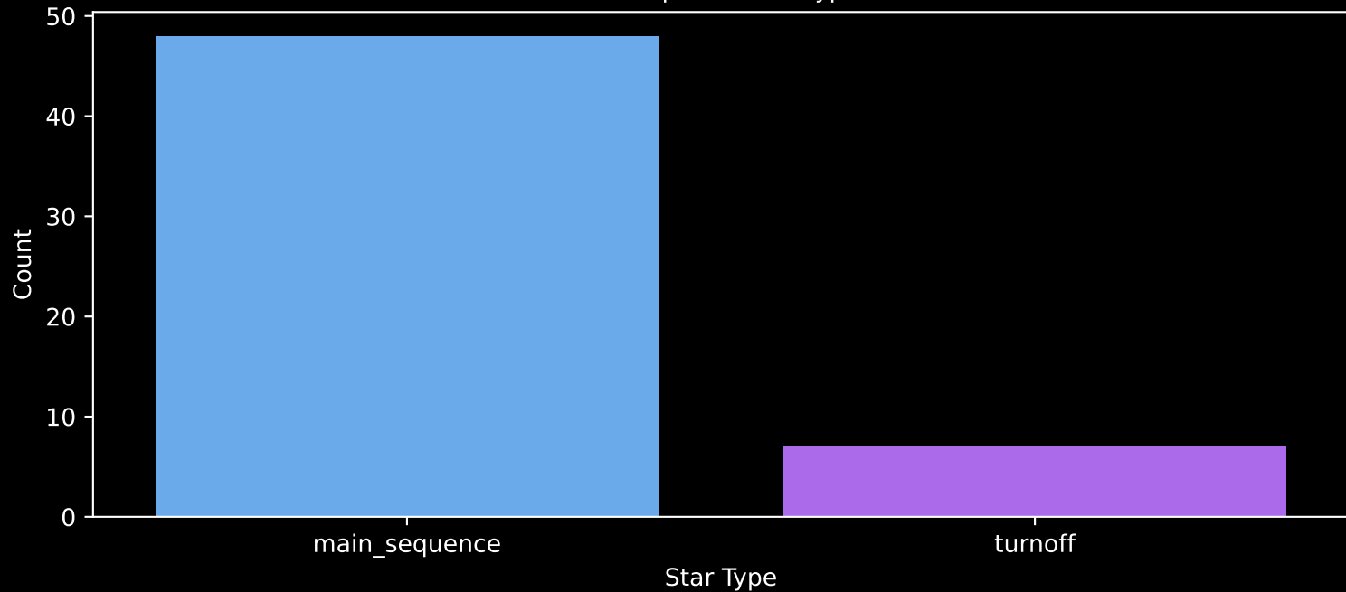
Gaia Cluster: [UPK_645] Count plot of Star Type
