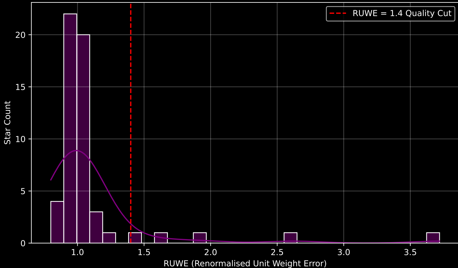
Gaia Cluster: [UPK_645] RUWE Distribution (n= 55)
