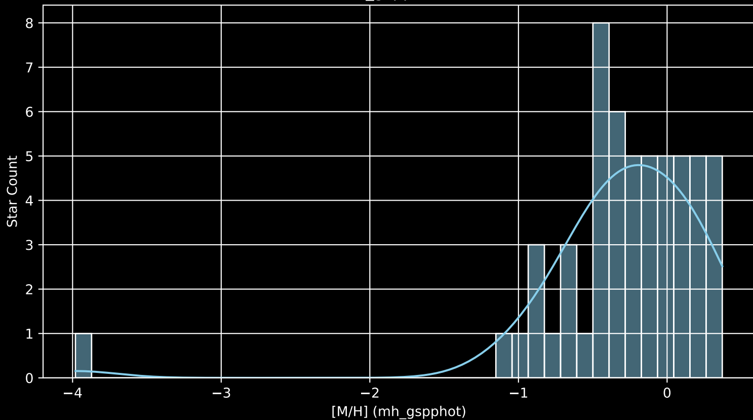
Gaia Cluster: [UPK_645 [M/H] (mh_gspphot) (n= 55)
