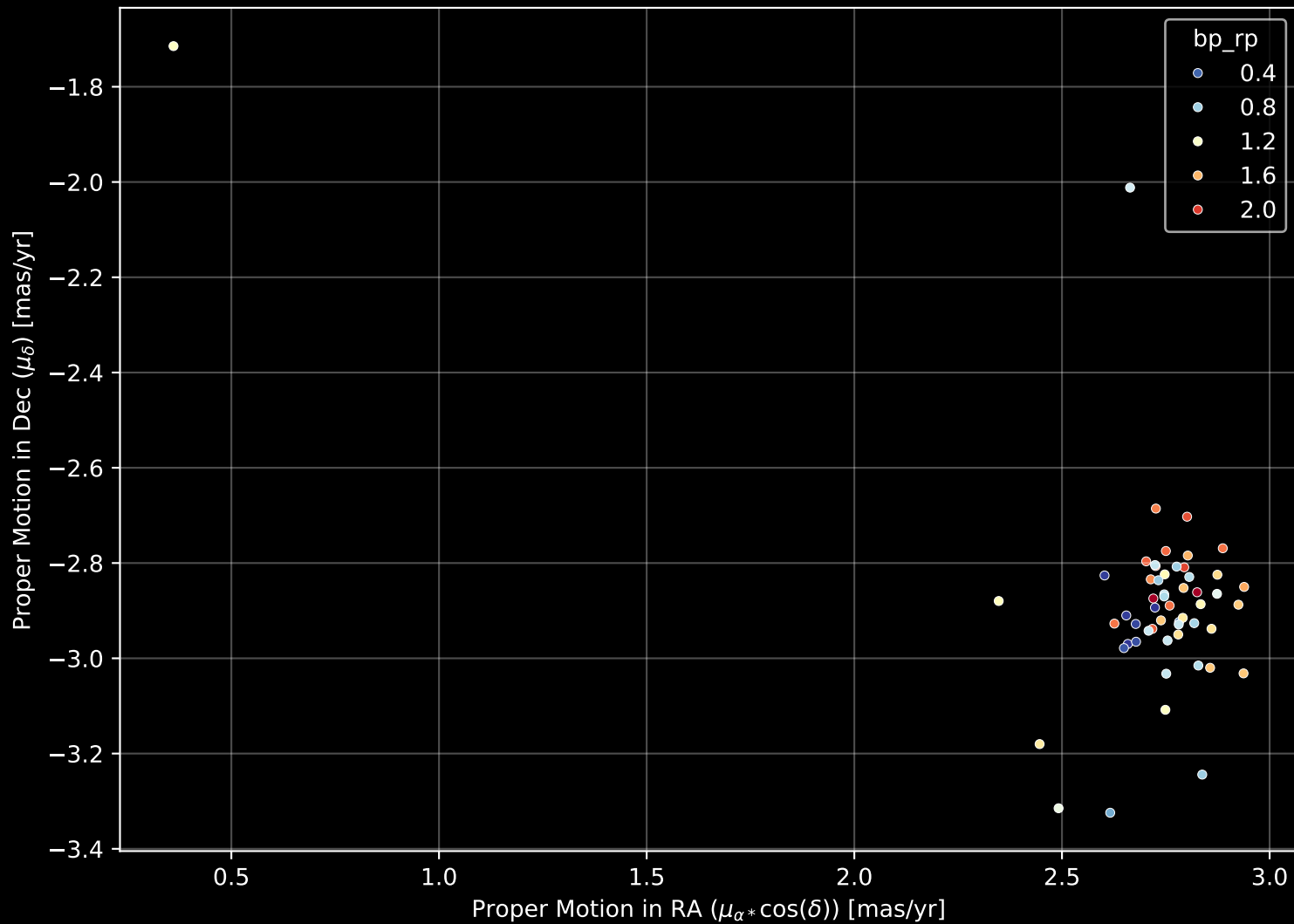
Gaia Cluster: [UPK_645] Proper Motion Diagram (n= 55)
