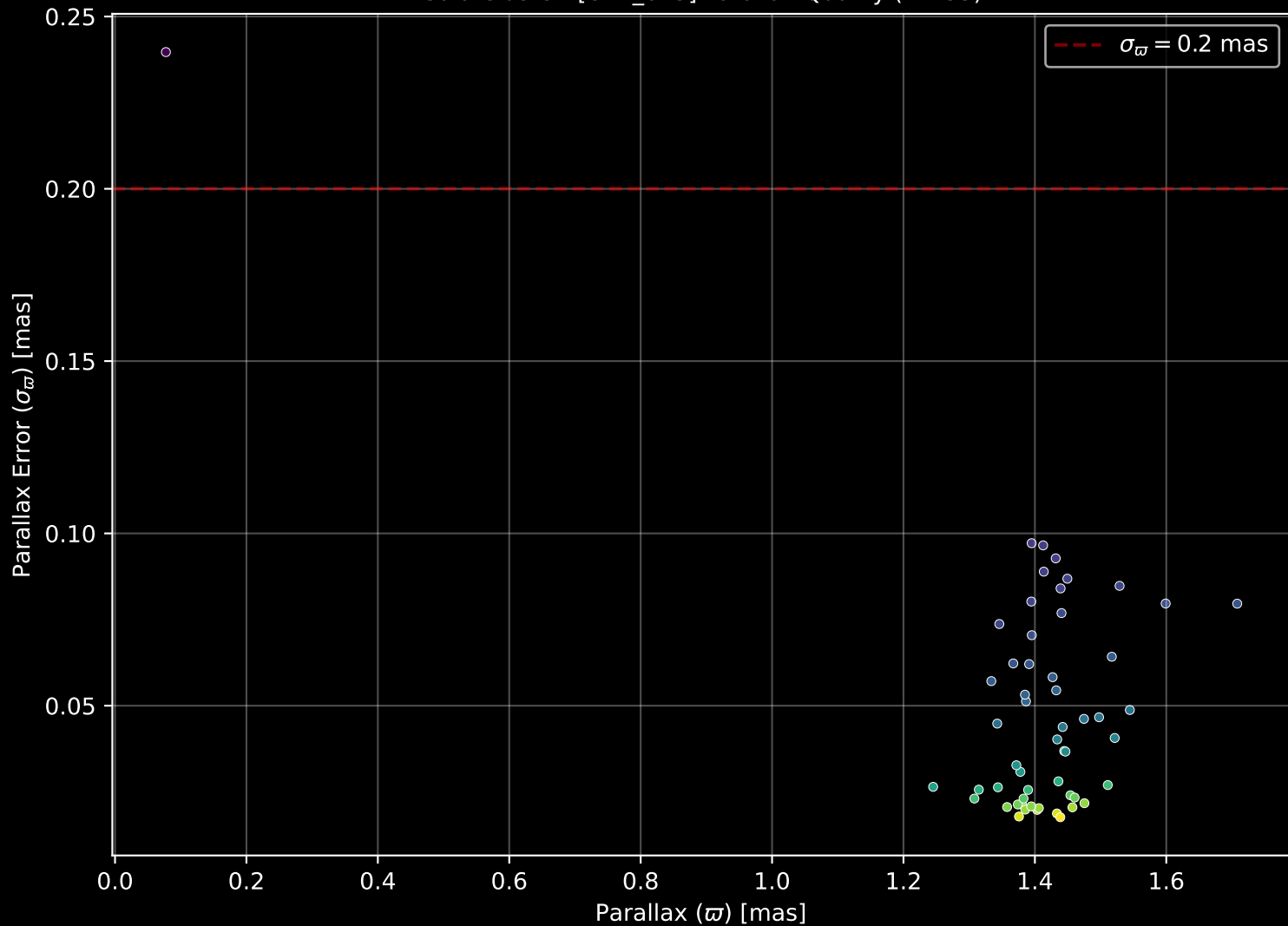
Gaia Cluster: [UPK_645] Parallax Quality (n= 55)
