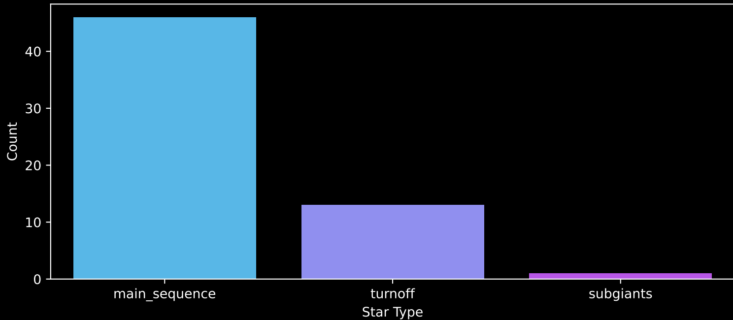
Gaia Cluster: [UPK_7] Count plot of Star Type
