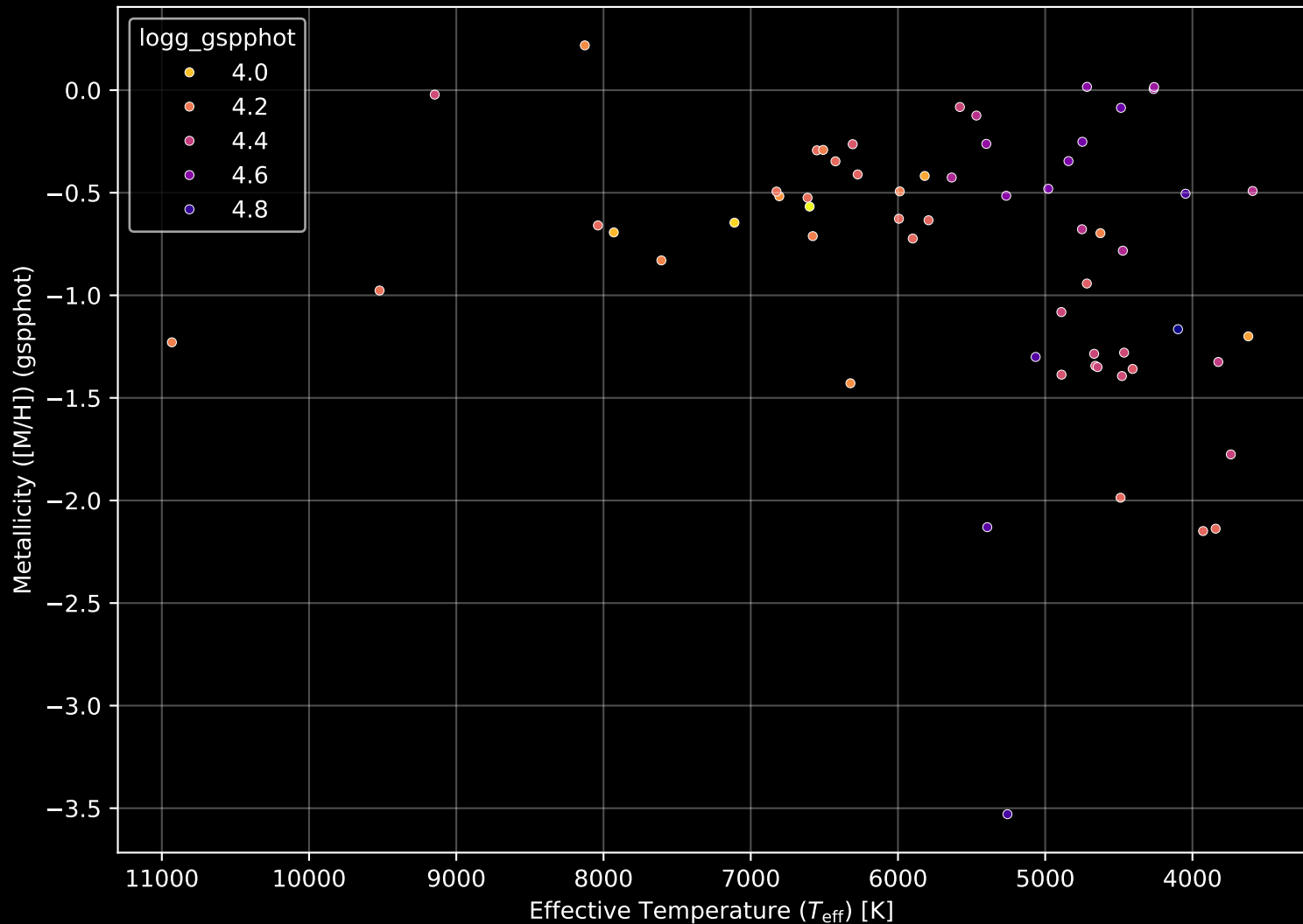
Gaia Cluster: [UPK_7] Stellar Population Parameters (n= 60)
