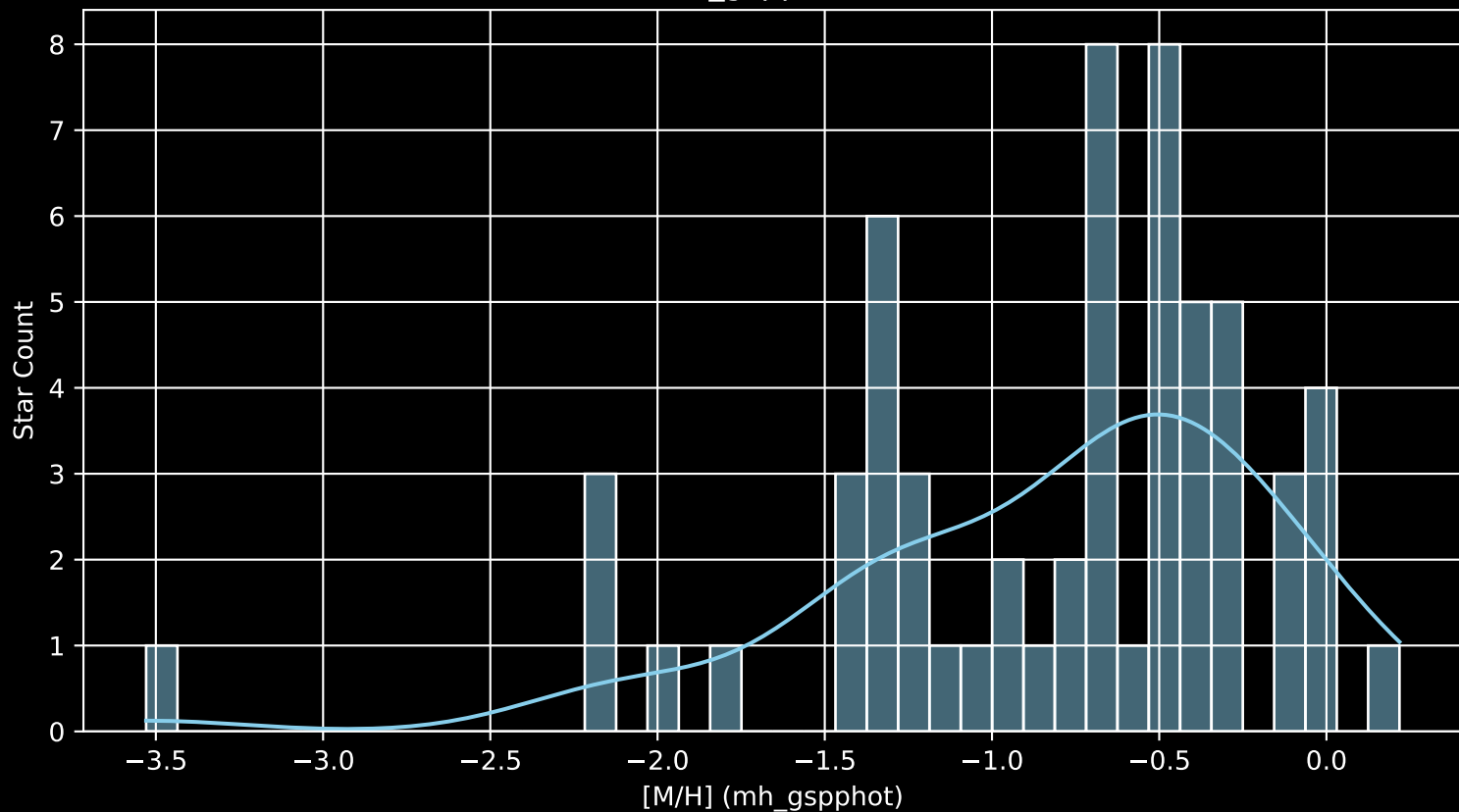
Gaia Cluster: [UPK_7 [M/H] (mh_gspphot) (n= 60)
