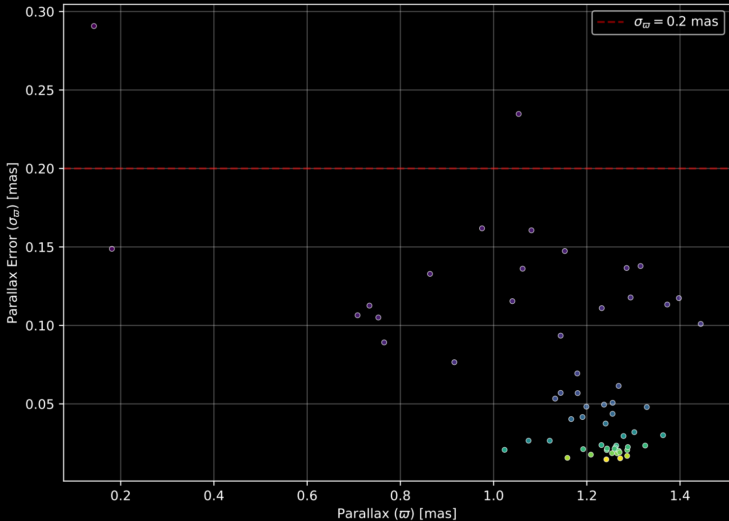
Gaia Cluster: [UPK_7] Parallax Quality (n= 60)
