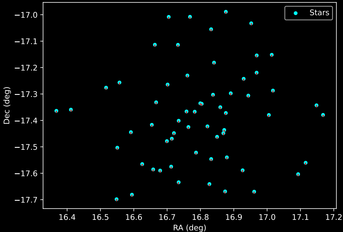
Gaia Cluster: [UPK_7] Proper Motion Vectors for Gaia Star Field (n= 60)
