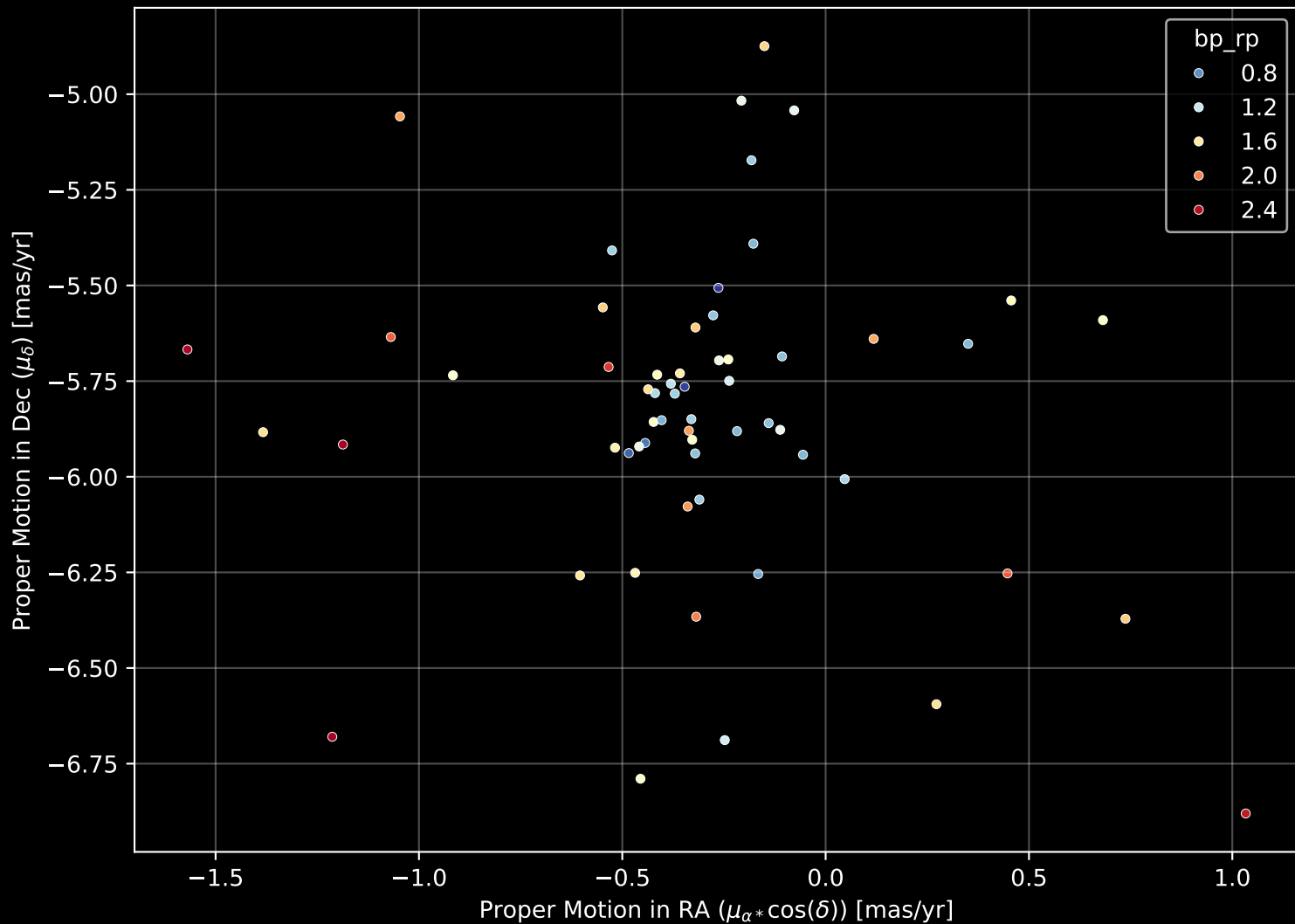
Gaia Cluster: [UPK_7] Proper Motion Diagram (n= 60)
