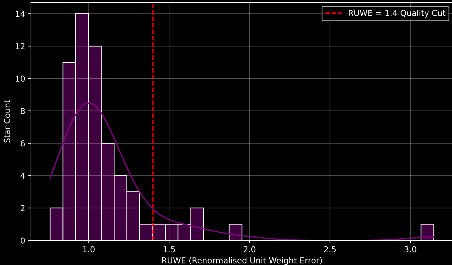
Gaia Cluster: [UPK_7] RUWE Distribution (n= 60)
