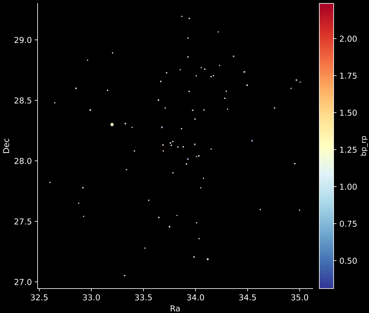
Gaia Cluster: [UPK_80] Stars: 77
