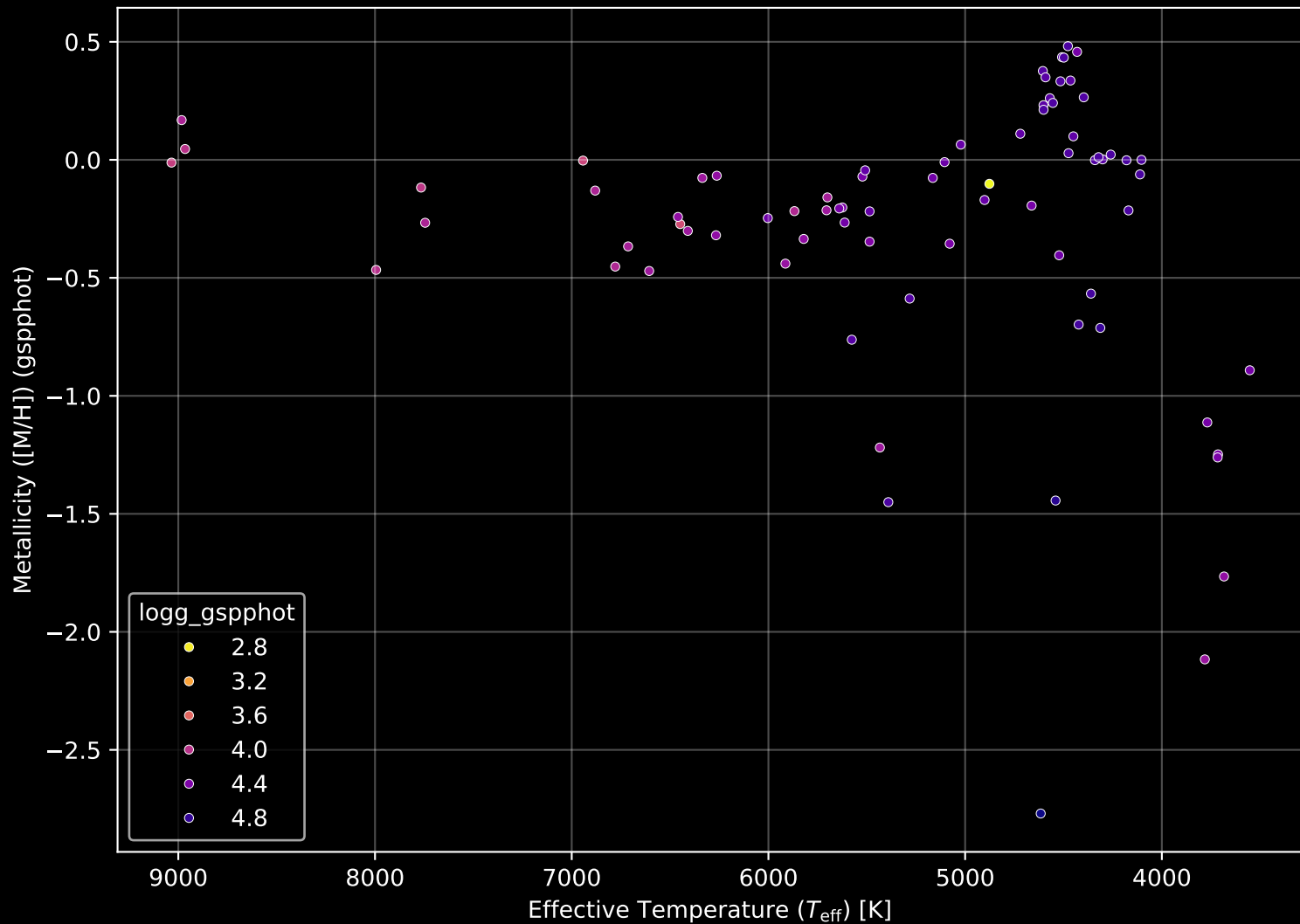
Gaia Cluster: [UPK_80] Stellar Population Parameters (n= 77)
