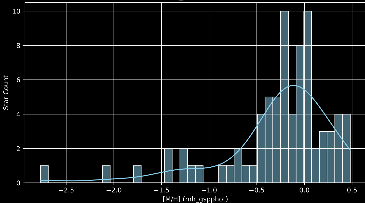
Gaia Cluster: [UPK_80 [M/H] (mh_gspphot) (n= 77)
