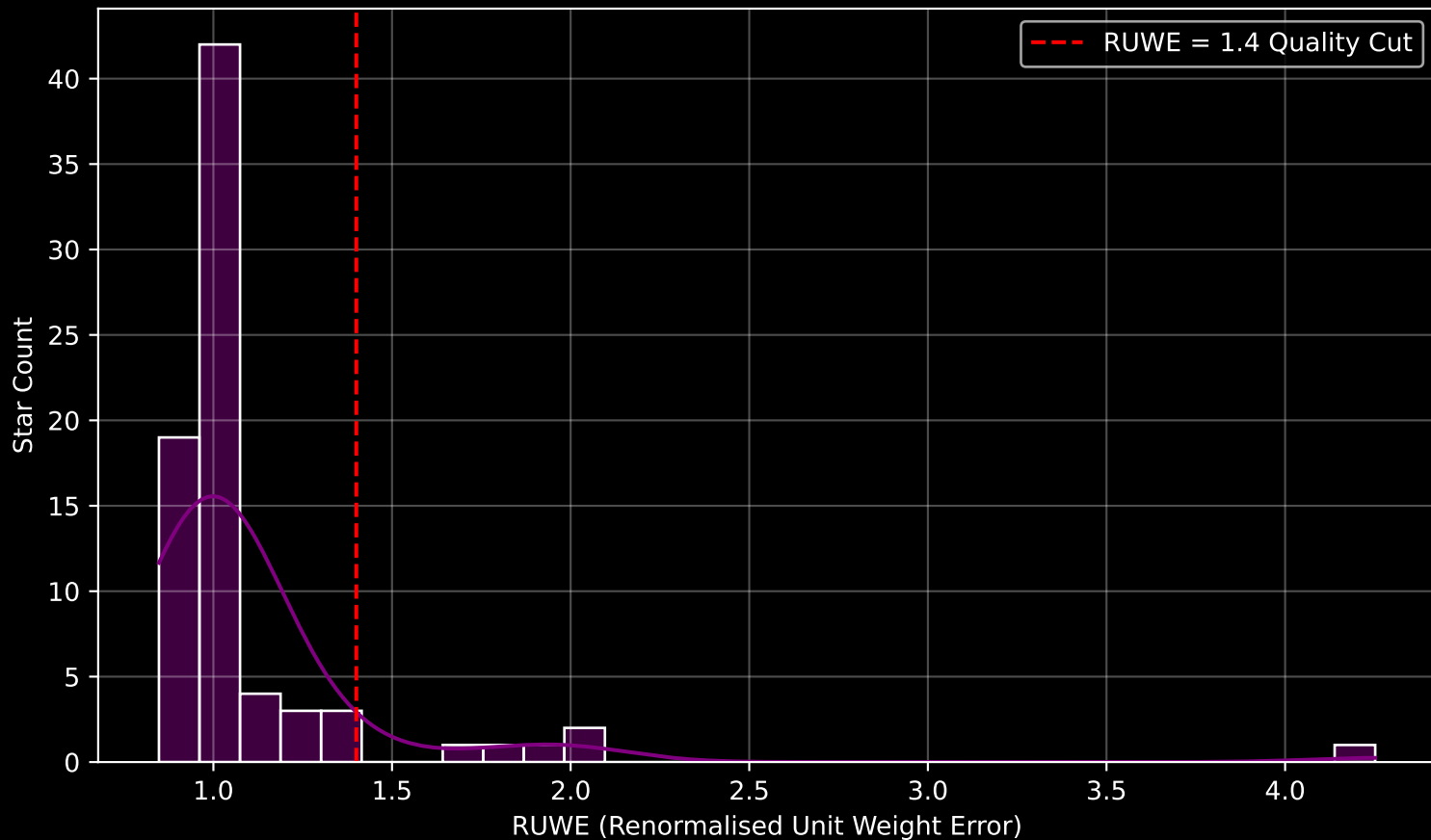
Gaia Cluster: [UPK_80] RUWE Distribution (n= 77)
