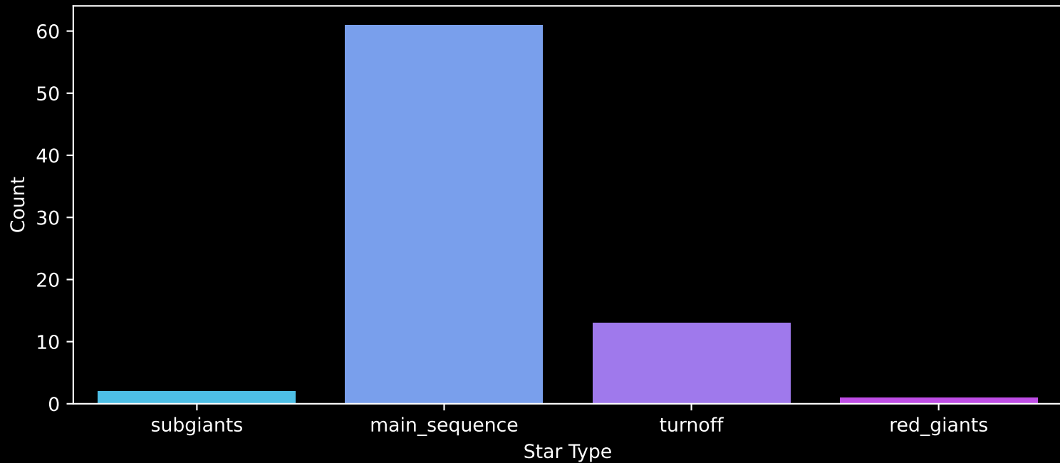
Gaia Cluster: [UPK_80] Count plot of Star Type
