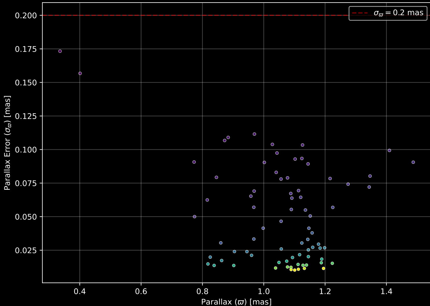
Gaia Cluster: [UPK_80] Parallax Quality (n= 77)
