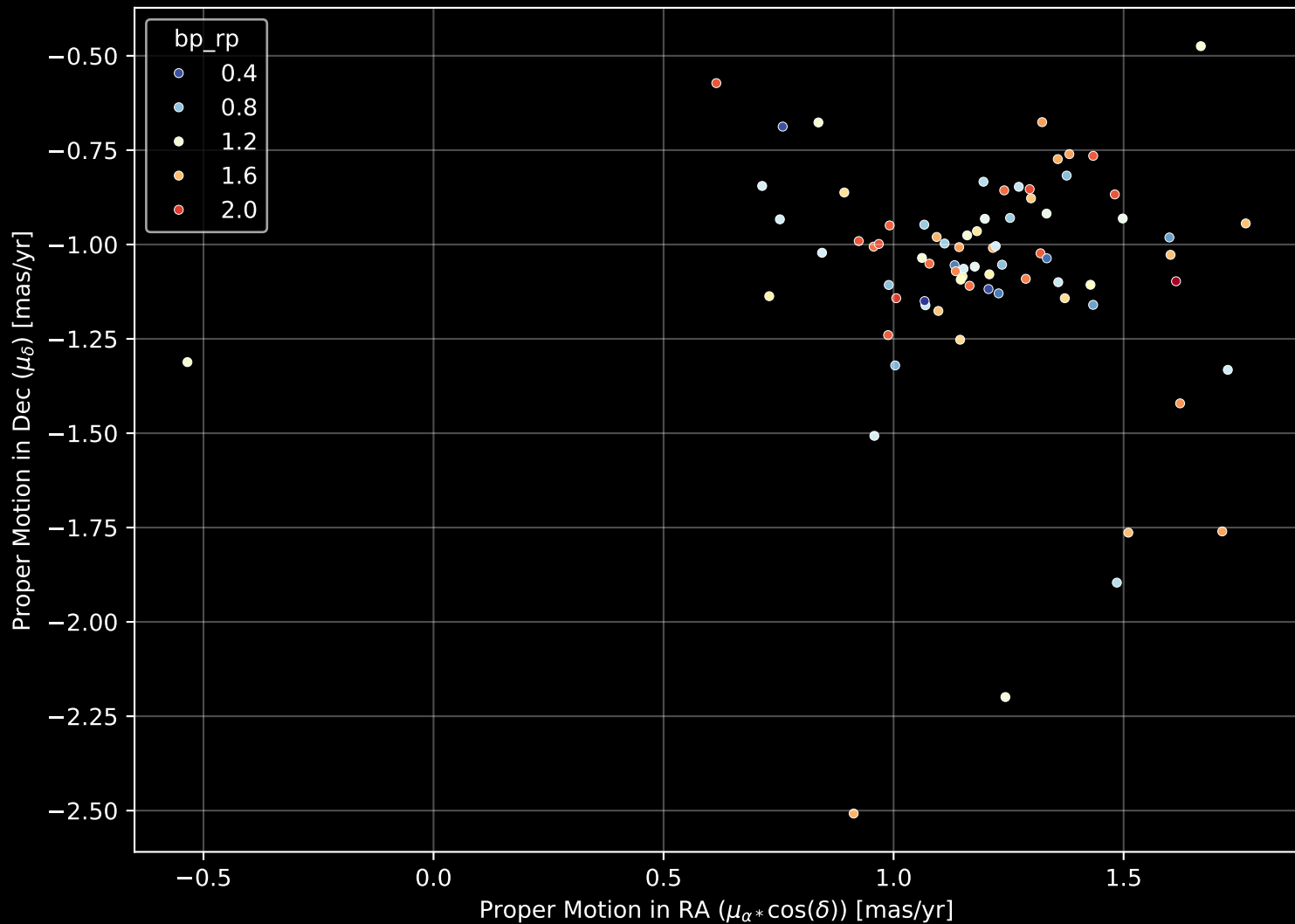
Gaia Cluster: [UPK_80] Proper Motion Diagram (n= 77)
