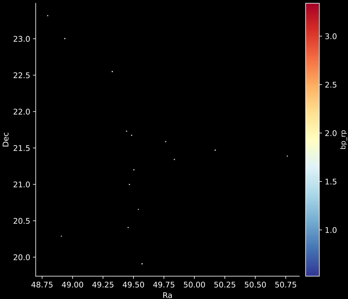
Gaia Cluster: [UPK_88] Stars: 16
