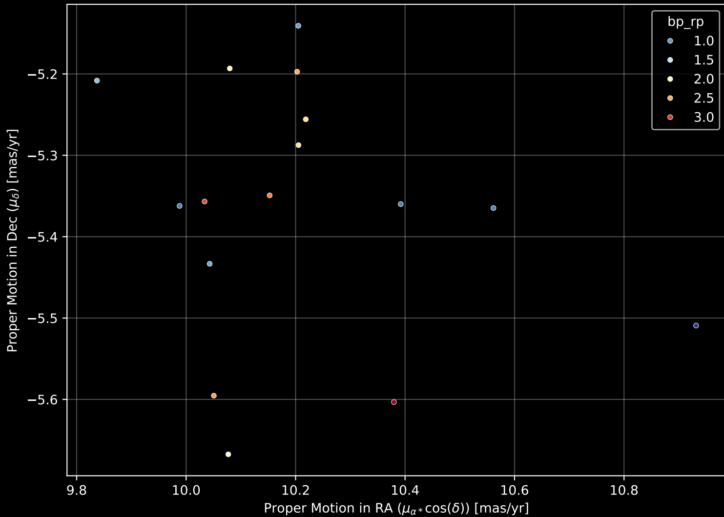
Gaia Cluster: [UPK_88] Proper Motion Diagram (n= 16)
