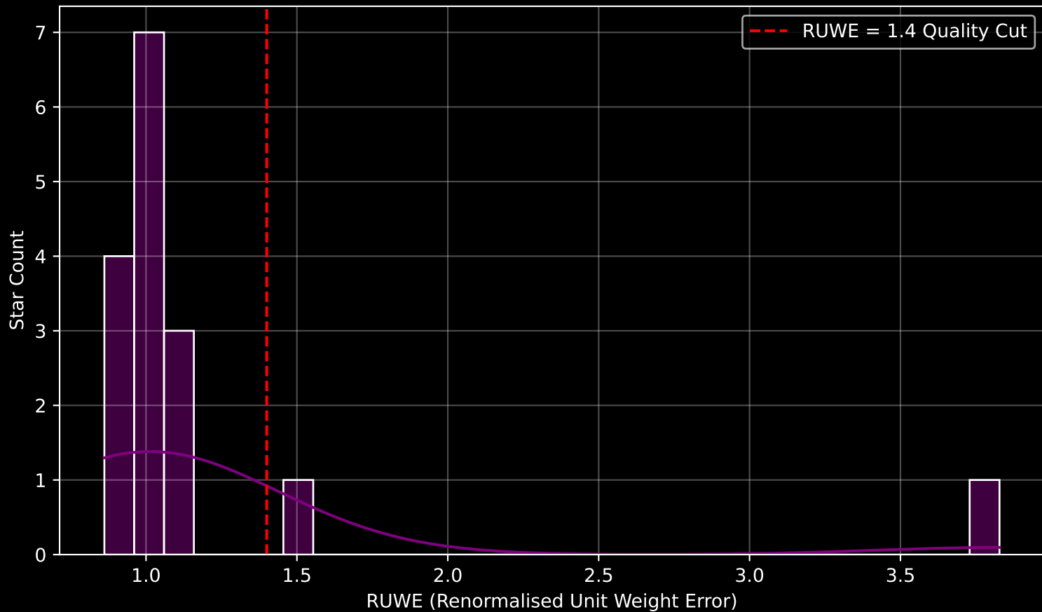
Gaia Cluster: [UPK_88] RUWE Distribution (n= 16)
