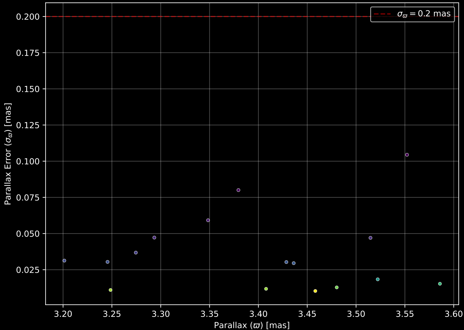
Gaia Cluster: [UPK_88] Parallax Quality (n= 16)
