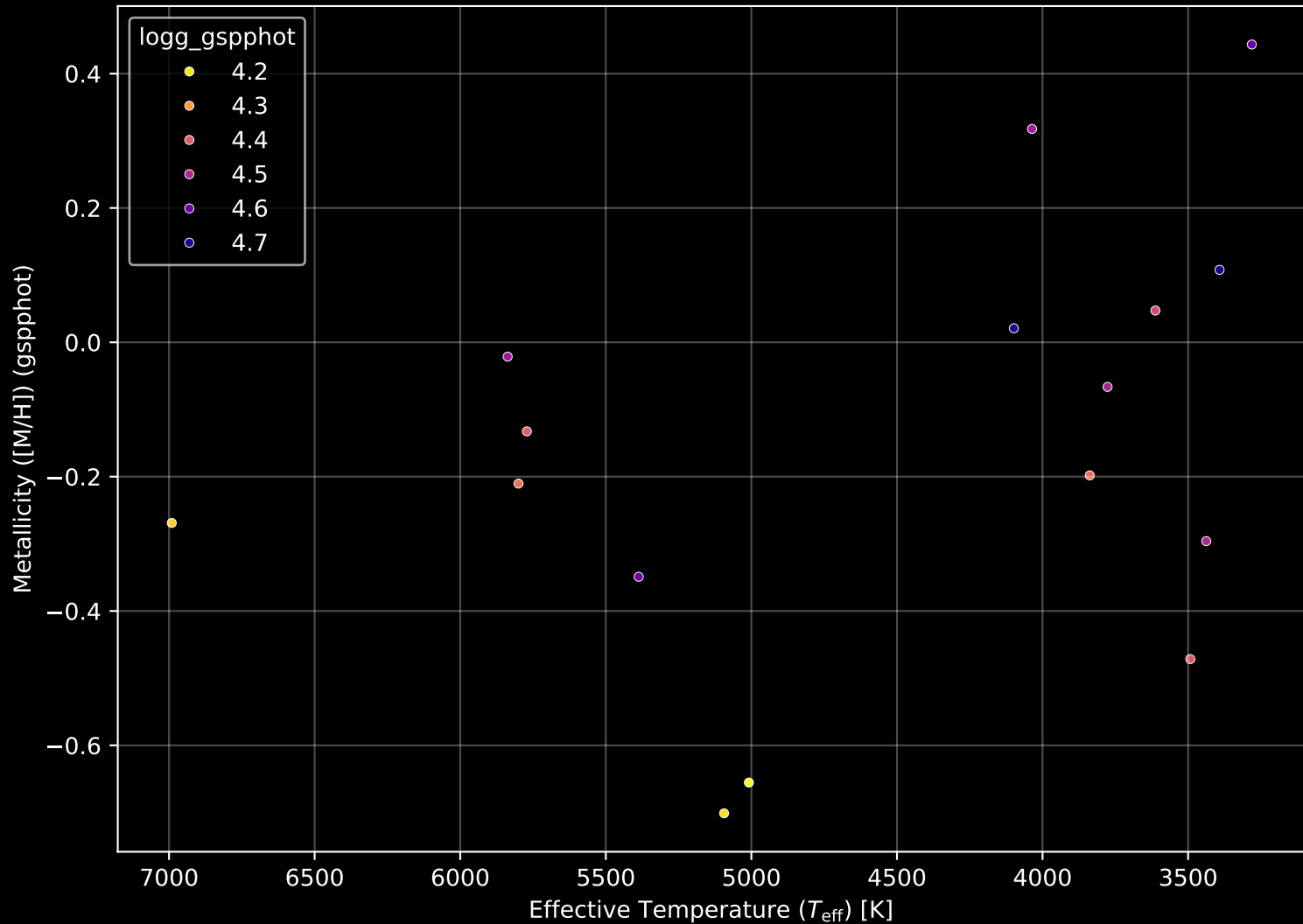
Gaia Cluster: [UPK_88] Stellar Population Parameters (n= 16)
