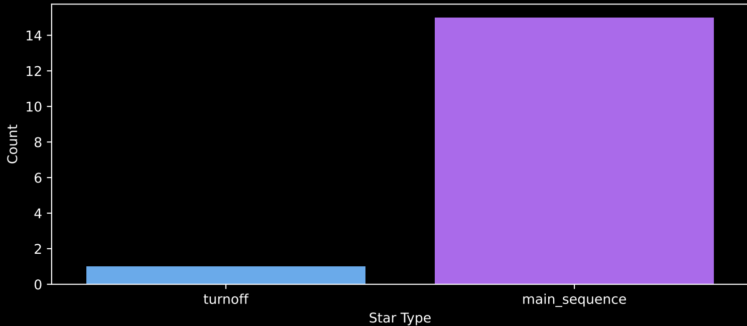
Gaia Cluster: [UPK_88] Count plot of Star Type
