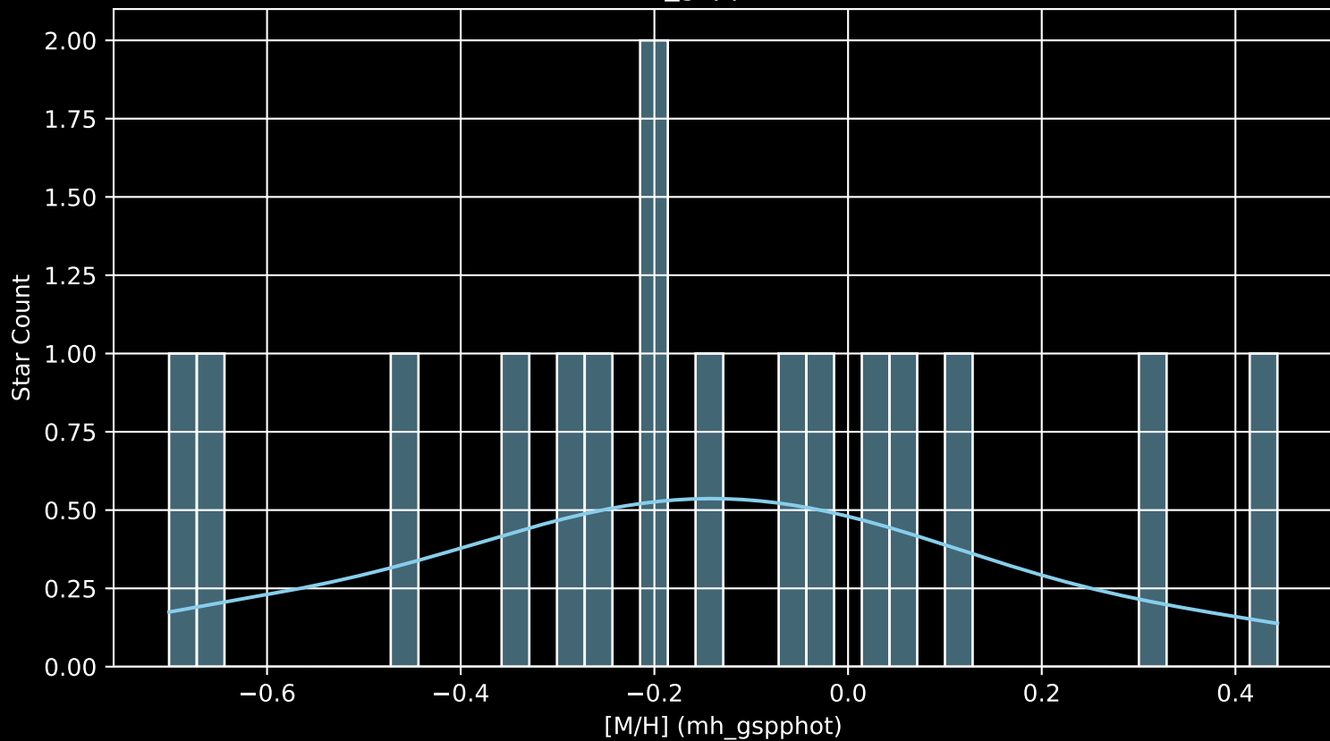
Gaia Cluster: [UPK_88 [M/H] (mh_gspphot) ( \bar{n}= 16 )
