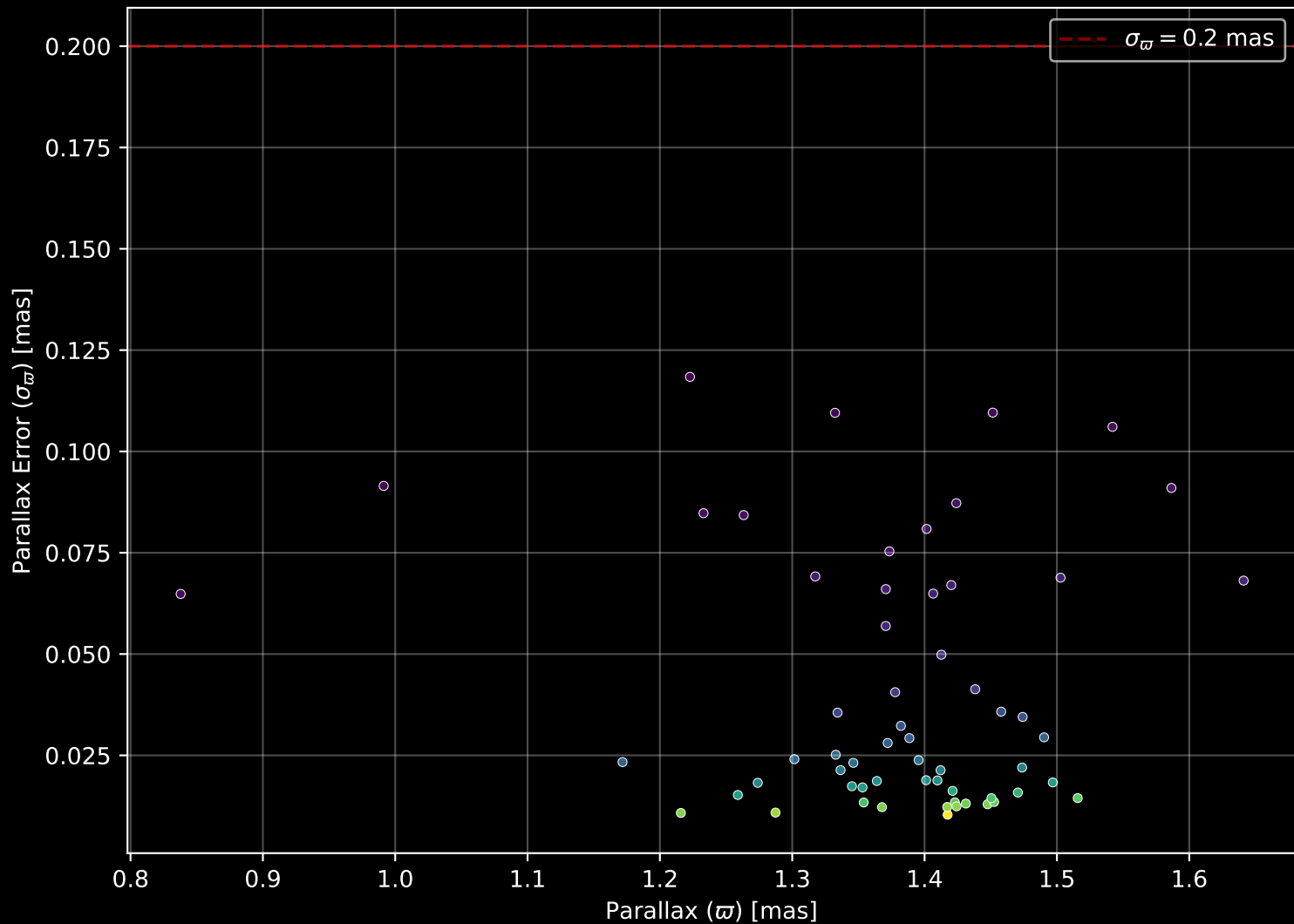
Gaia Cluster: [UPK_93] Parallax Quality (n= 60)
