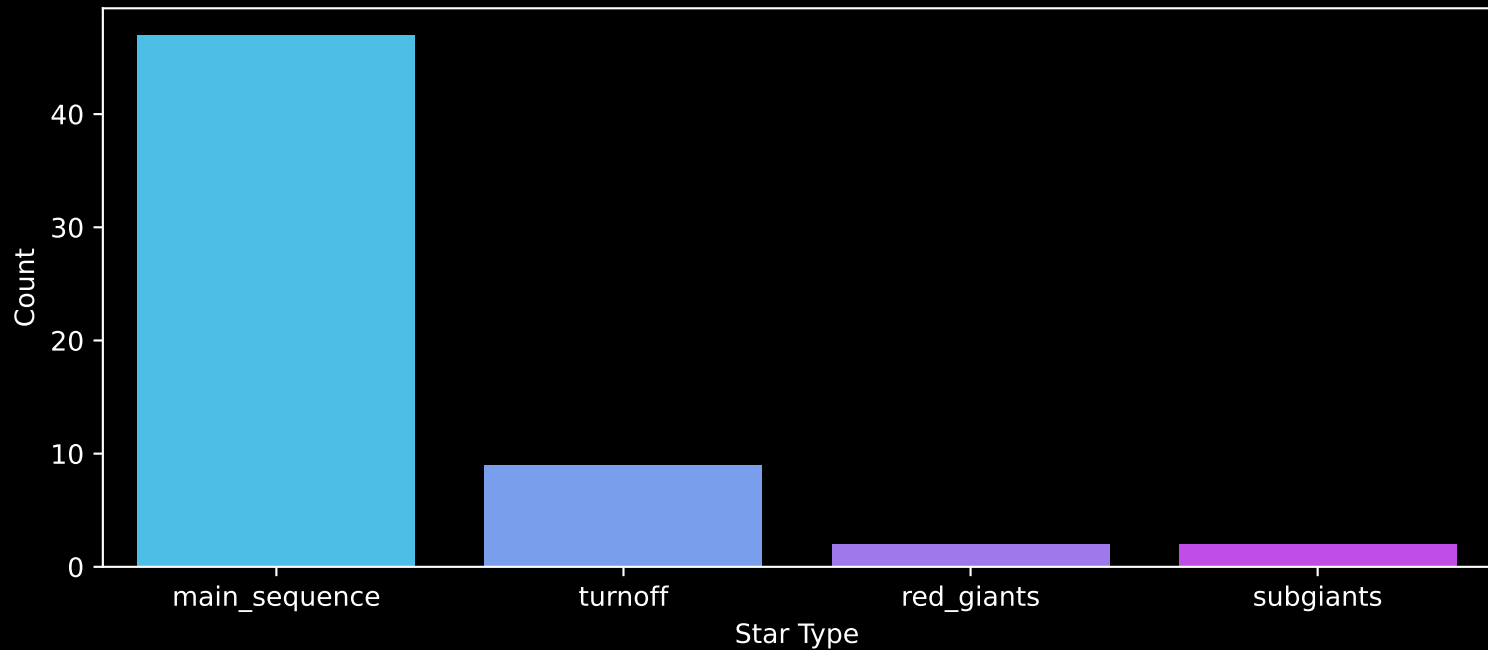
Gaia Cluster: [UPK_93] Count plot of Star Type
