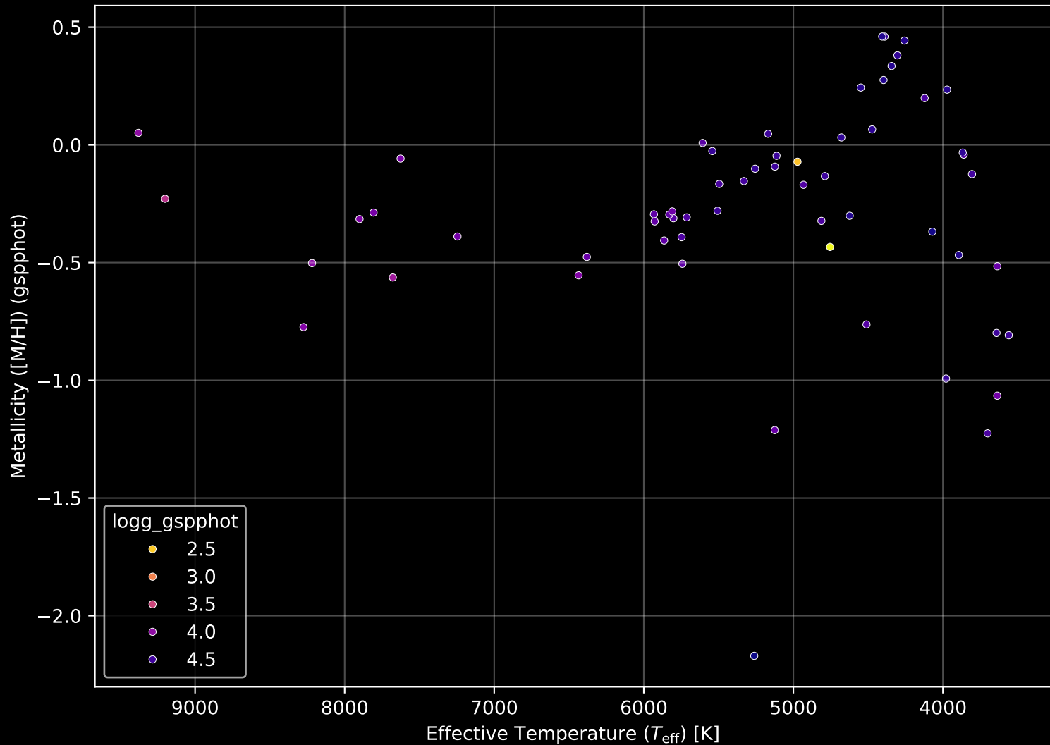
Gaia Cluster: [UPK_93] Stellar Population Parameters (n= 60)
