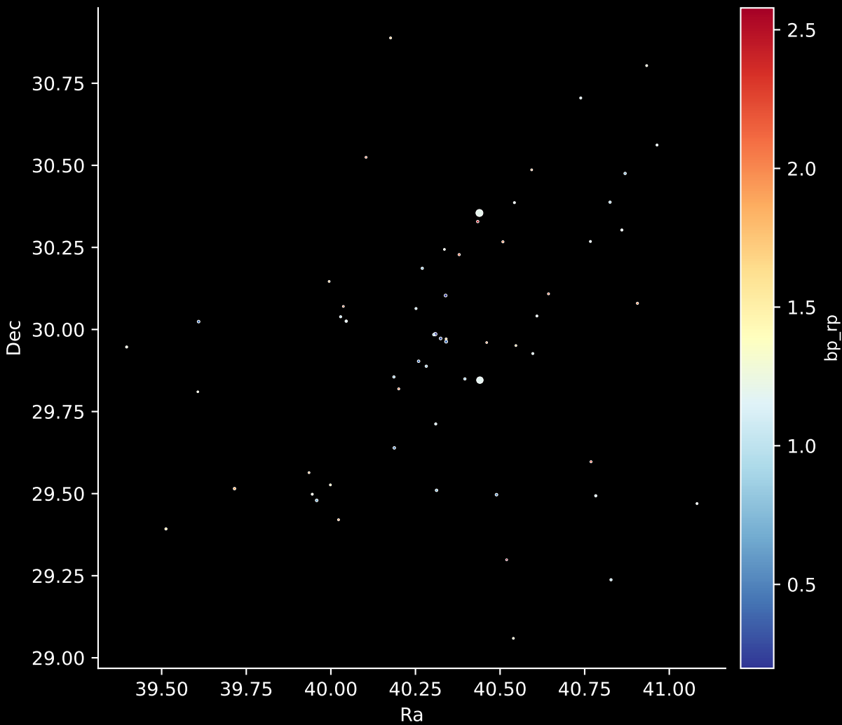
Gaia Cluster: [UPK_93] Stars: 60
