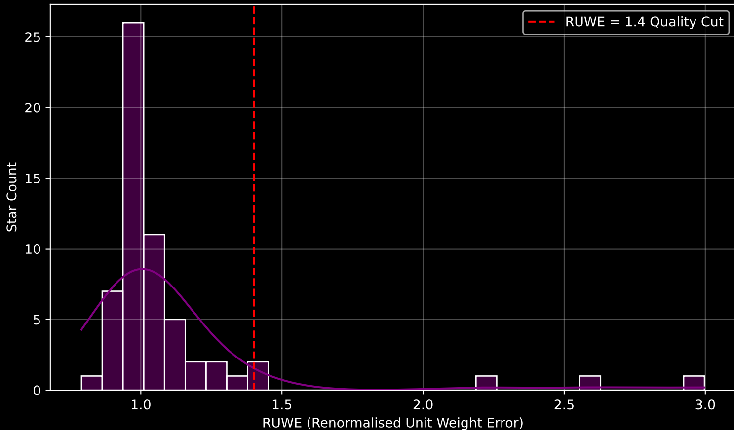
Gaia Cluster: [UPK_93] RUWE Distribution (n= 60)
