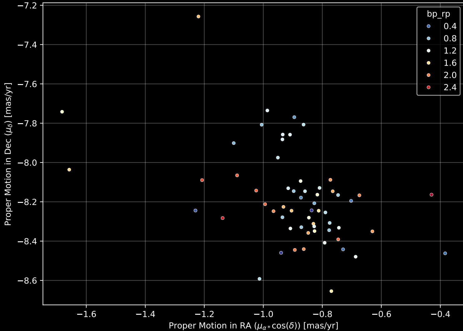
Gaia Cluster: [UPK_93] Proper Motion Diagram (n= 60)
