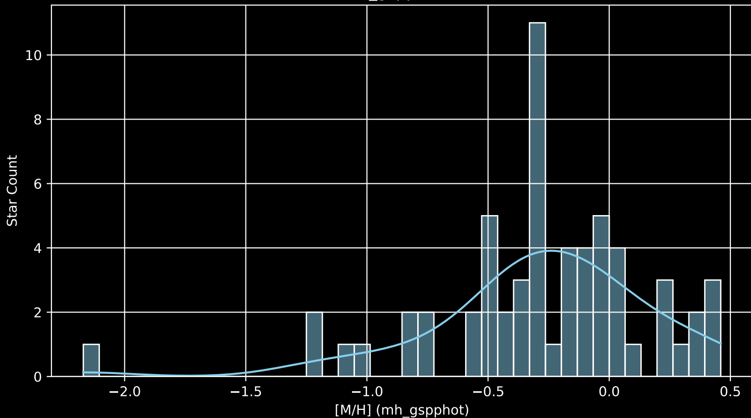
Gaia Cluster: [UPK_93 [M/H] (mh_gspphot) ( \bar{n}=60 )
