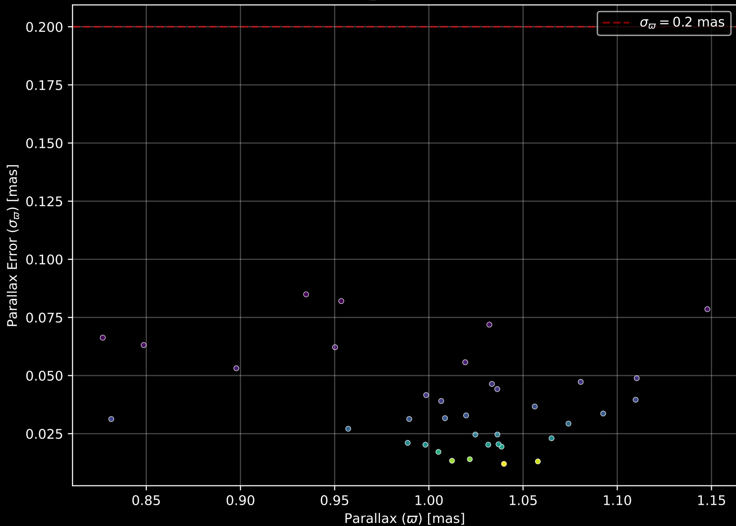
Gaia Cluster: [UPK_94] Parallax Quality (n= 37)
