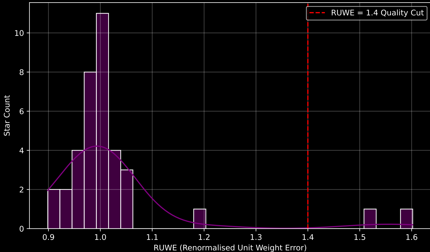
Gaia Cluster: [UPK_94] RUWE Distribution (n= 37)
