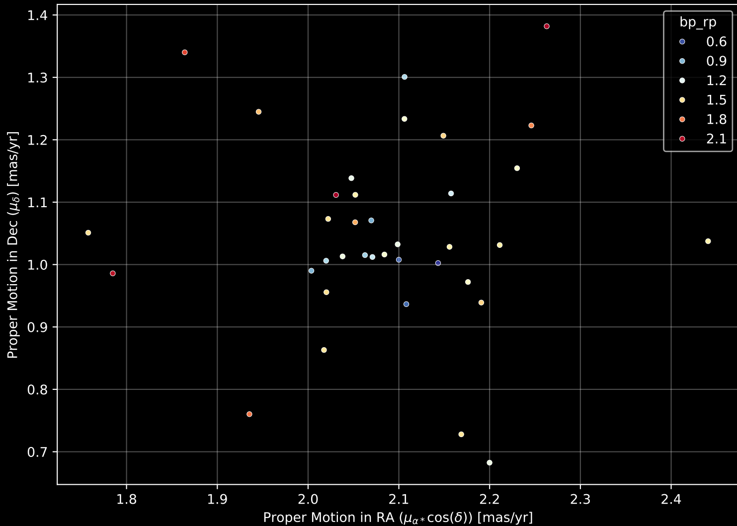
Gaia Cluster: [UPK_94] Proper Motion Diagram (n= 37)
