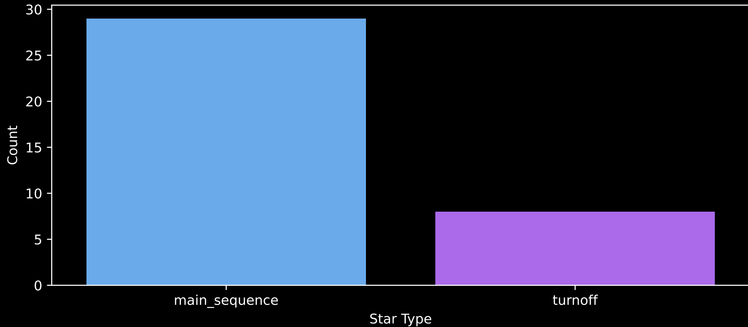
Gaia Cluster: [UPK_94] Count plot of Star Type
