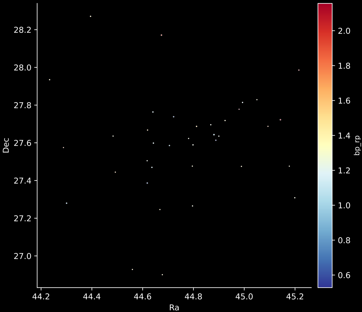
Gaia Cluster: [UPK_94] Stars: 37
