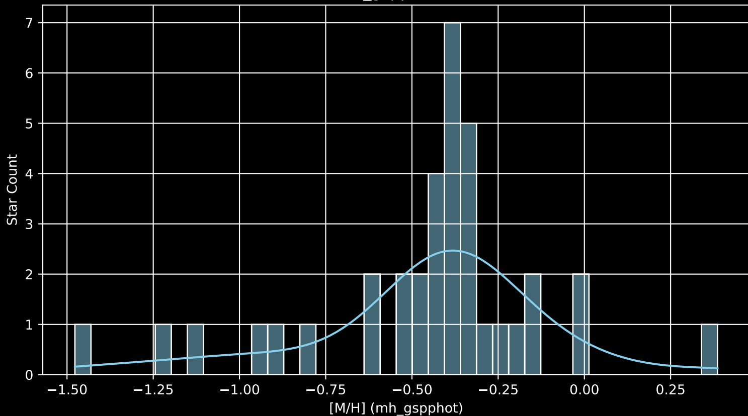
Gaia Cluster: [UPK_94 [M/H] (mh_gspphot) (n= 36)
