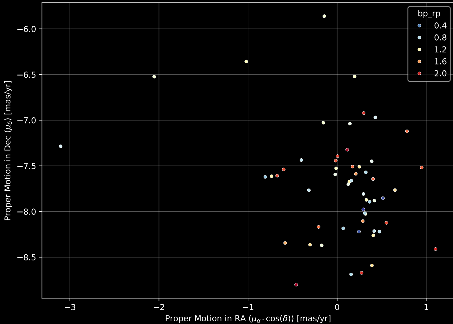
Gaia Cluster: [UPK_99] Proper Motion Diagram (n= 56)
