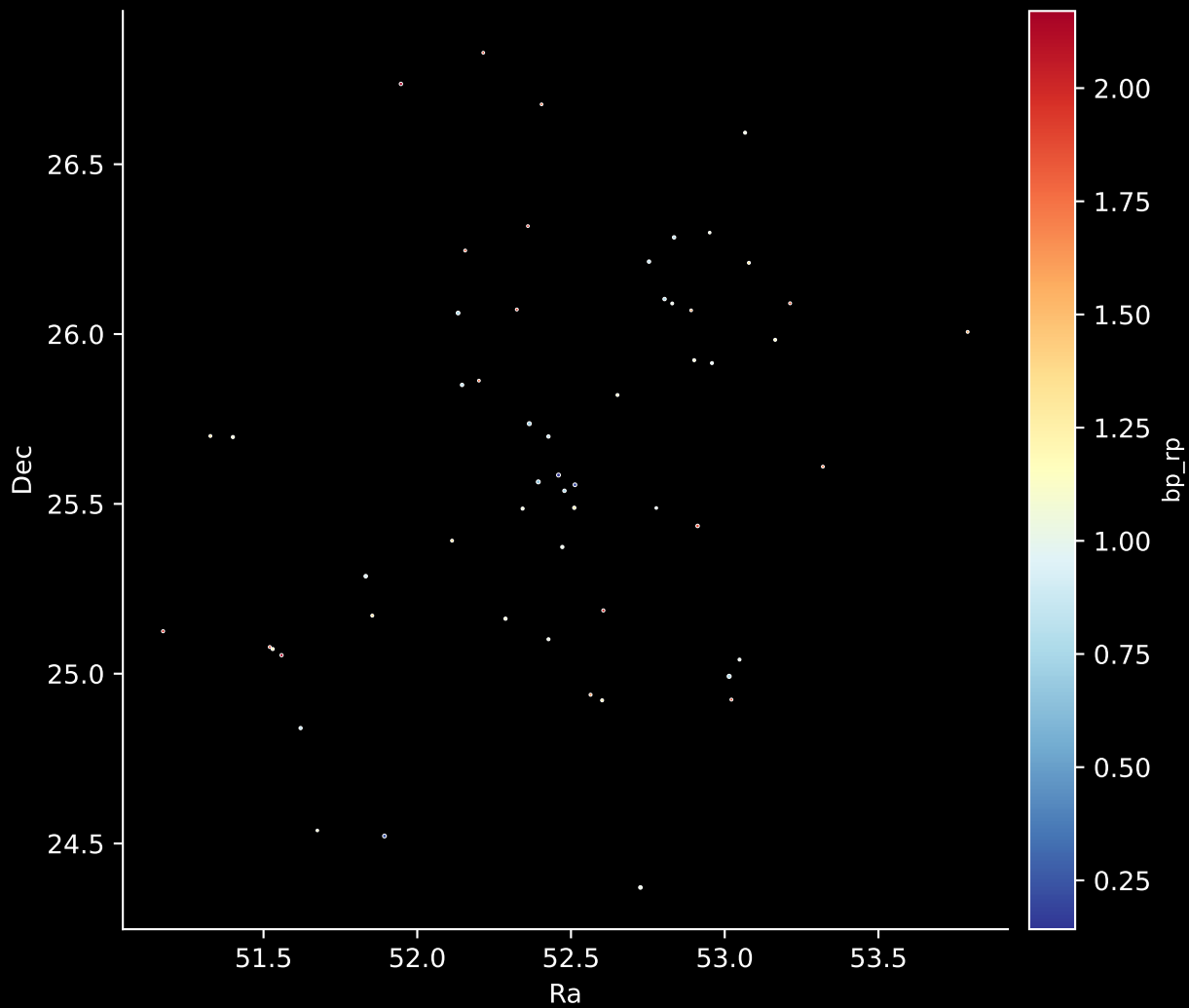
Gaia Cluster: [UPK_99] Stars: 56
