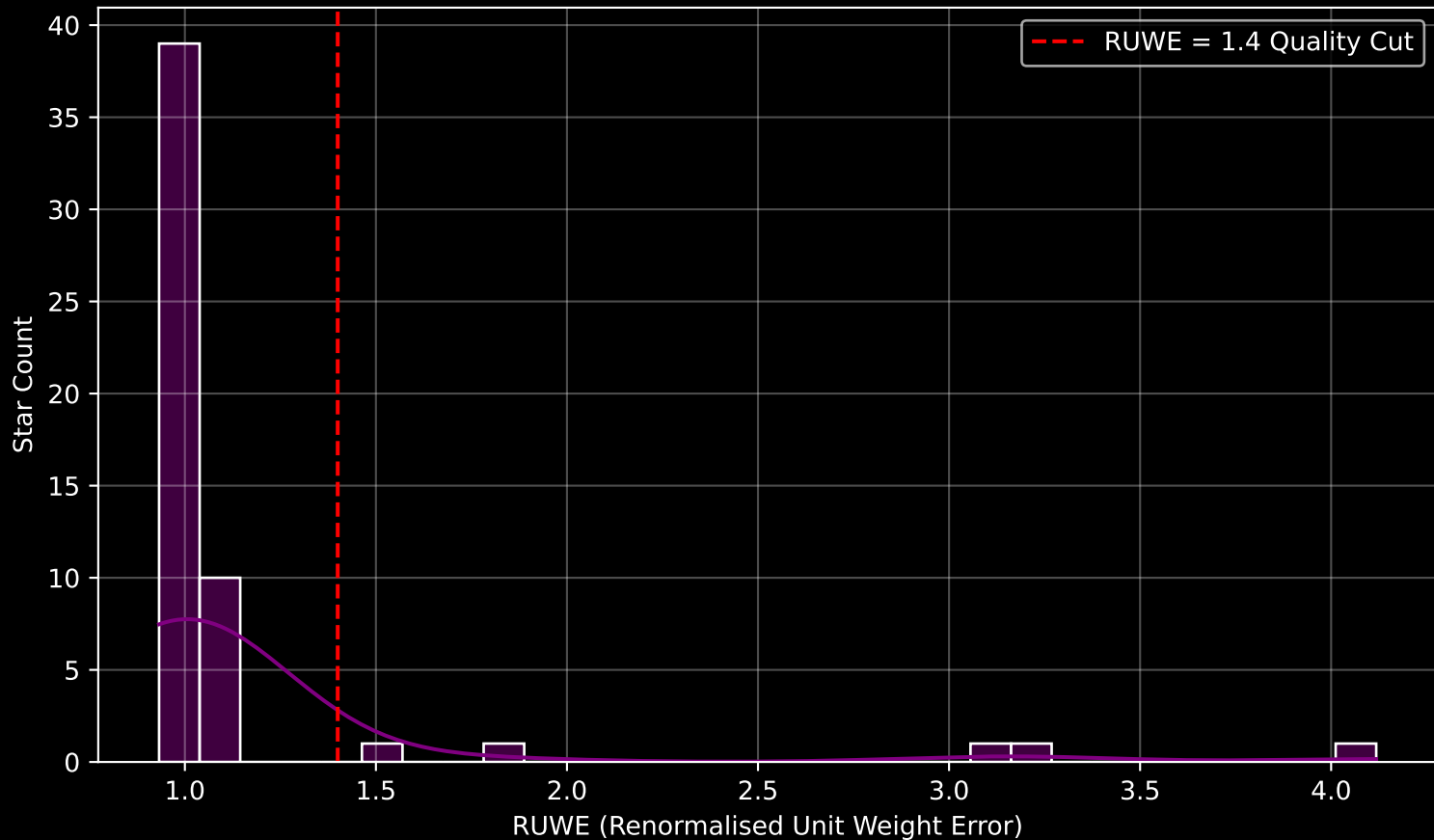
Gaia Cluster: [UPK_99] RUWE Distribution (n= 54)
