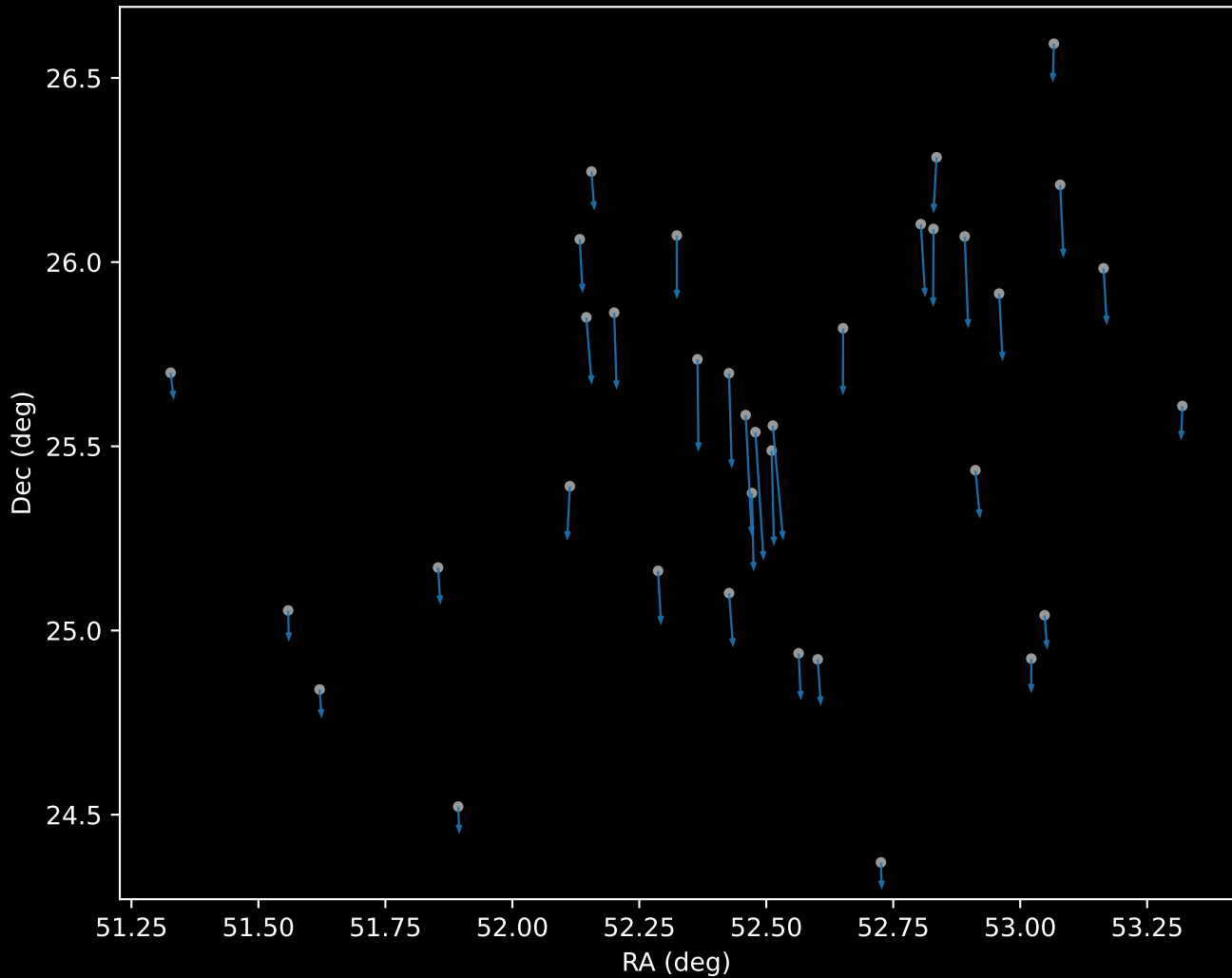
Gaia DR3 Cluster 0 Proper Motion Vectors (n=36)
