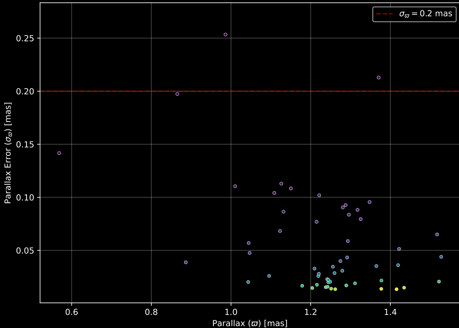
Gaia Cluster: [UPK_99] Parallax Quality (n= 56)
