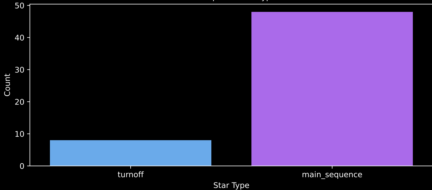
Gaia Cluster: [UPK_99] Count plot of Star Type
