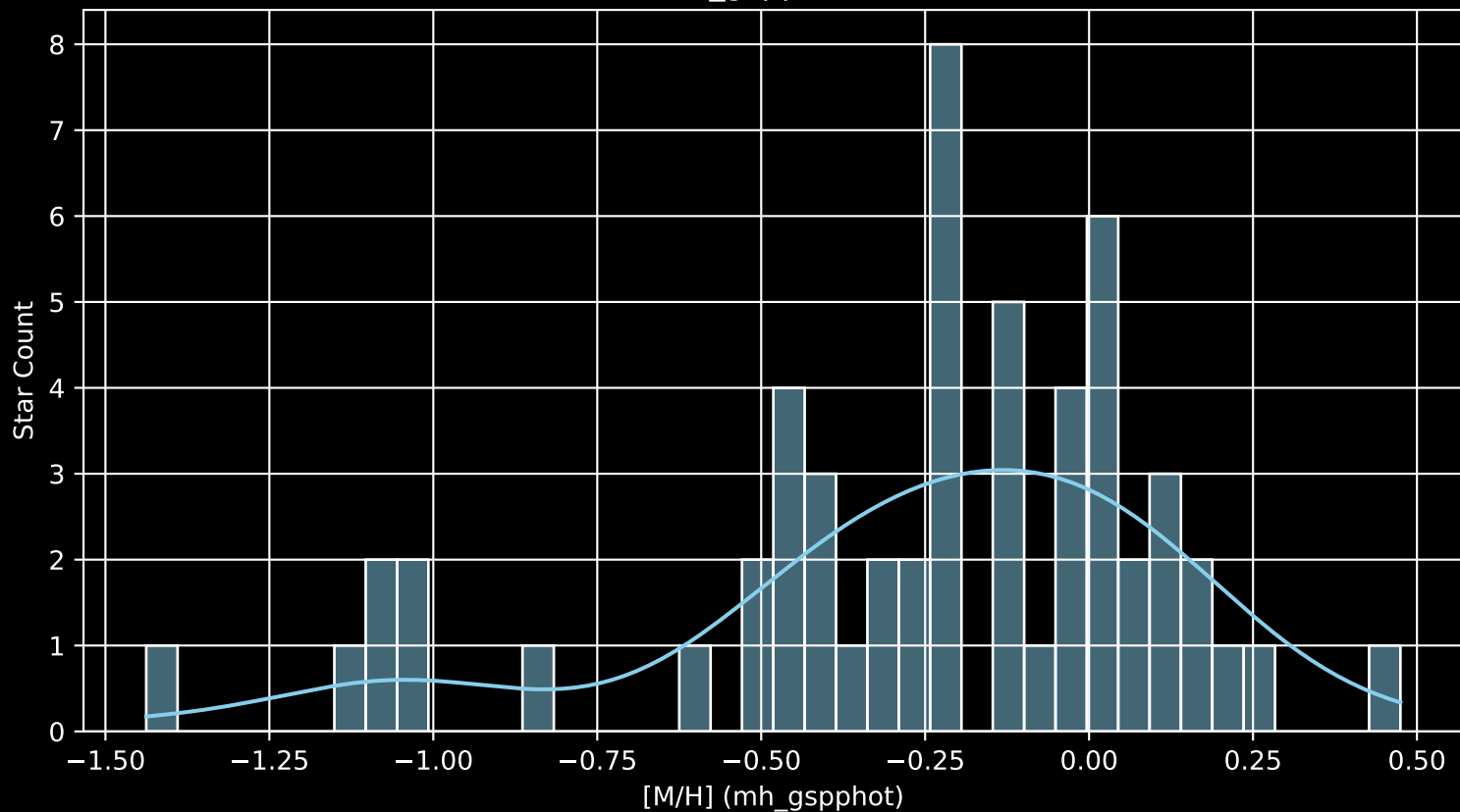
Gaia Cluster: [UPK_99 [M/H] (mh_gspphot) (n= 56)
