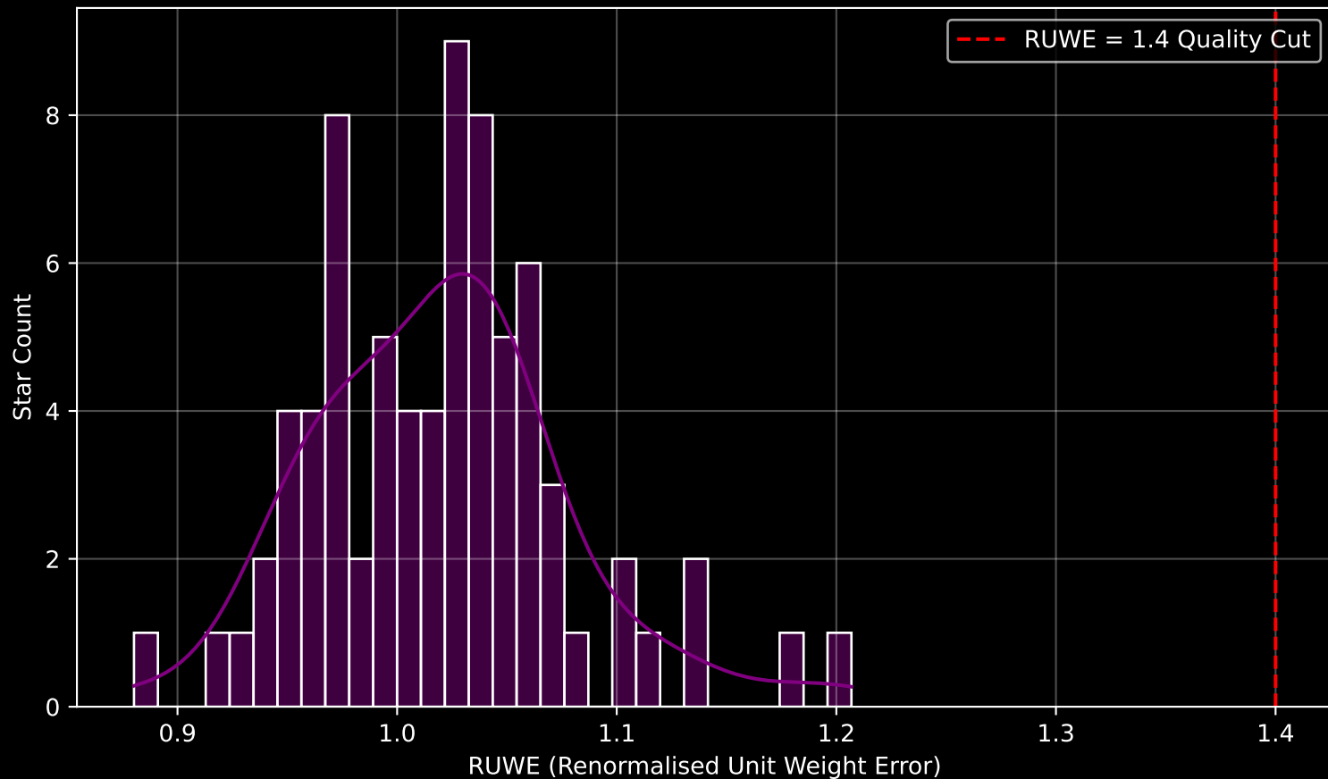
Gaia Cluster: [Waterloo_7] RUWE Distribution (n= 75)
