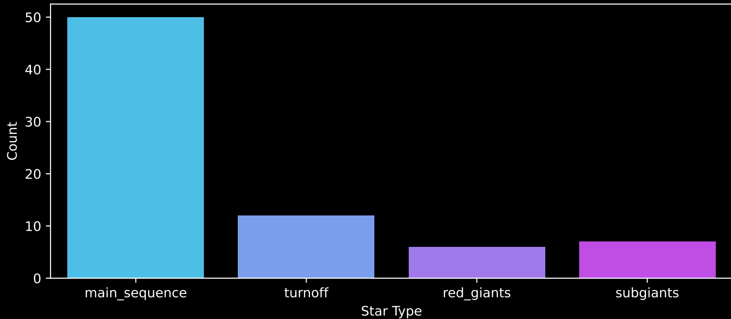
Gaia Cluster: [Waterloo_7] Count plot of Star Type
