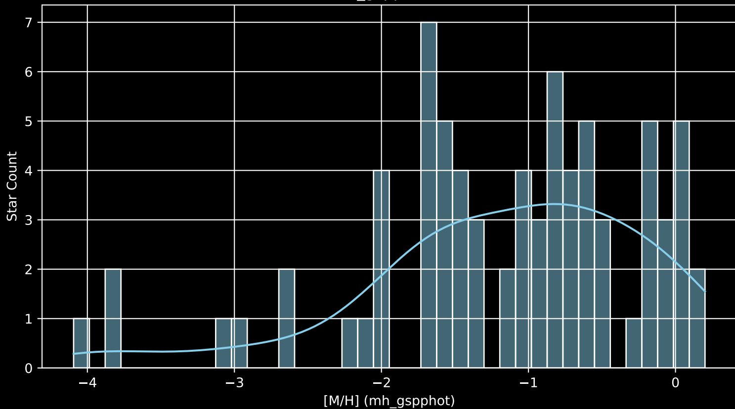
Gaia Cluster: [Waterloo_7 [M/H] (mh_gspphot) (n= 75)
