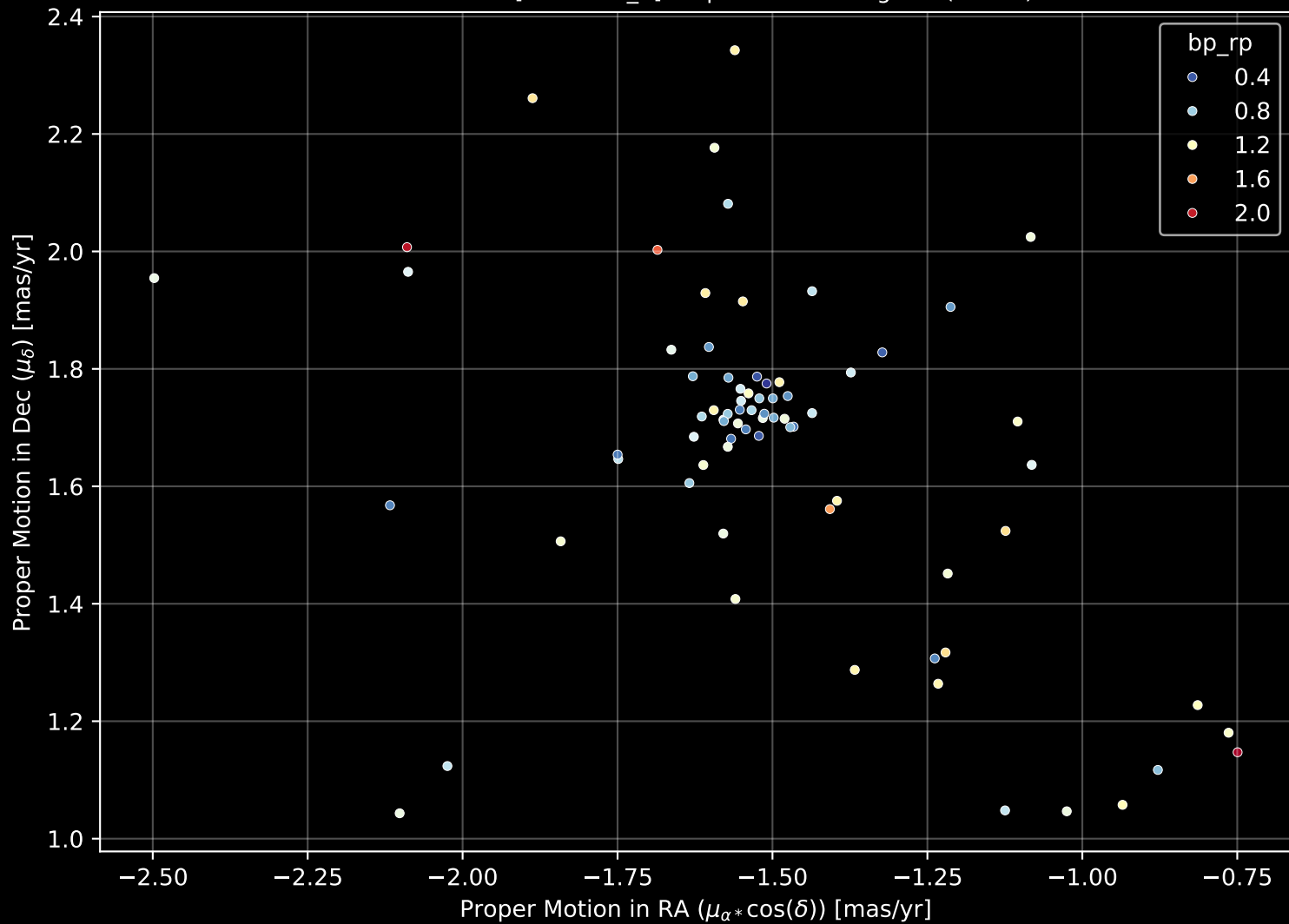
Gaia Cluster: [Waterloo_7] Proper Motion Diagram (n= 75)
