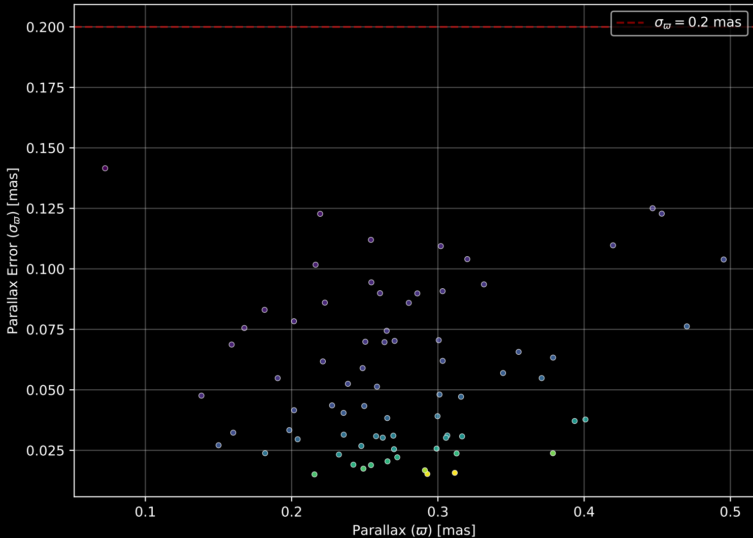
Gaia Cluster: [Waterloo_7] Parallax Quality (n= 75)
