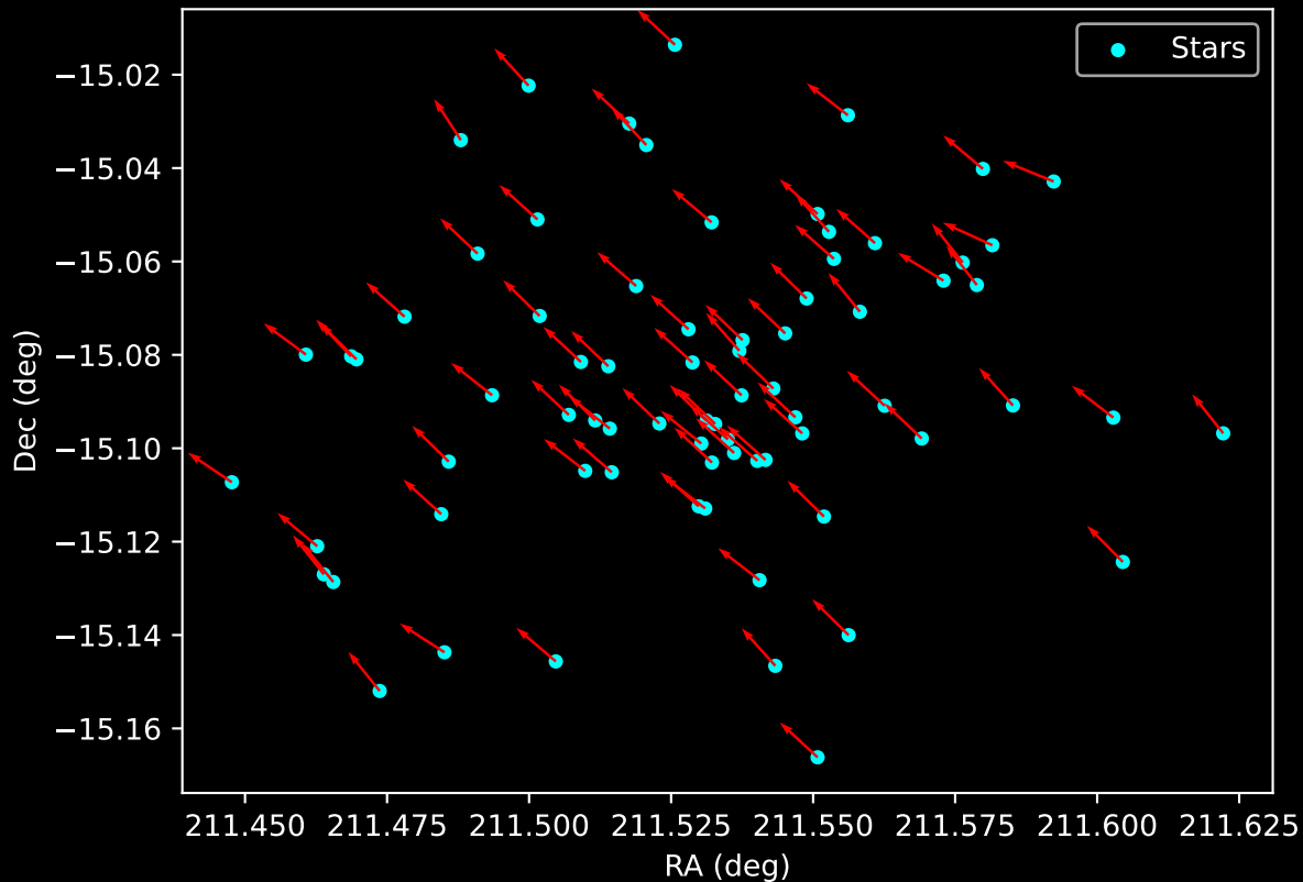
Gaia Cluster: [Waterloo_7] Proper Motion Vectors for Gaia Star Field (n= 75)
