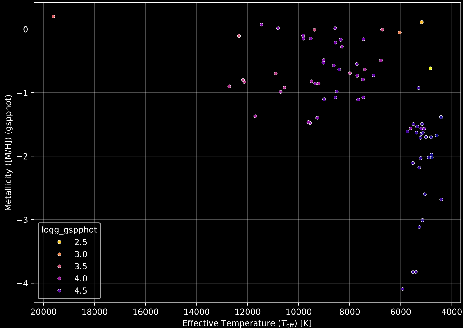
Gaia Cluster: [Waterloo_7] Stellar Population Parameters (n= 75)
