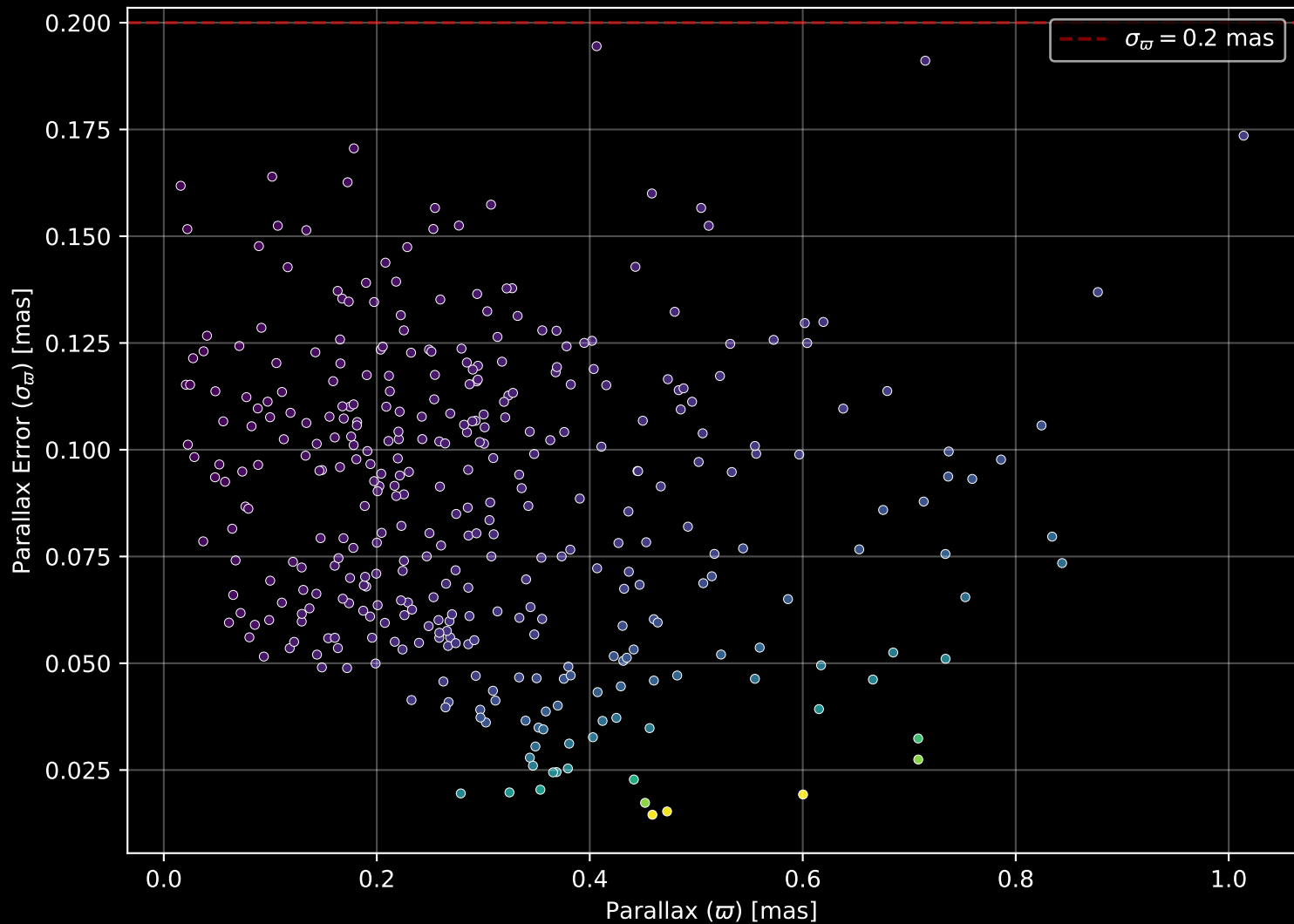
Gaia Cluster: [Westerlund_1] Parallax Quality (n= 364)
