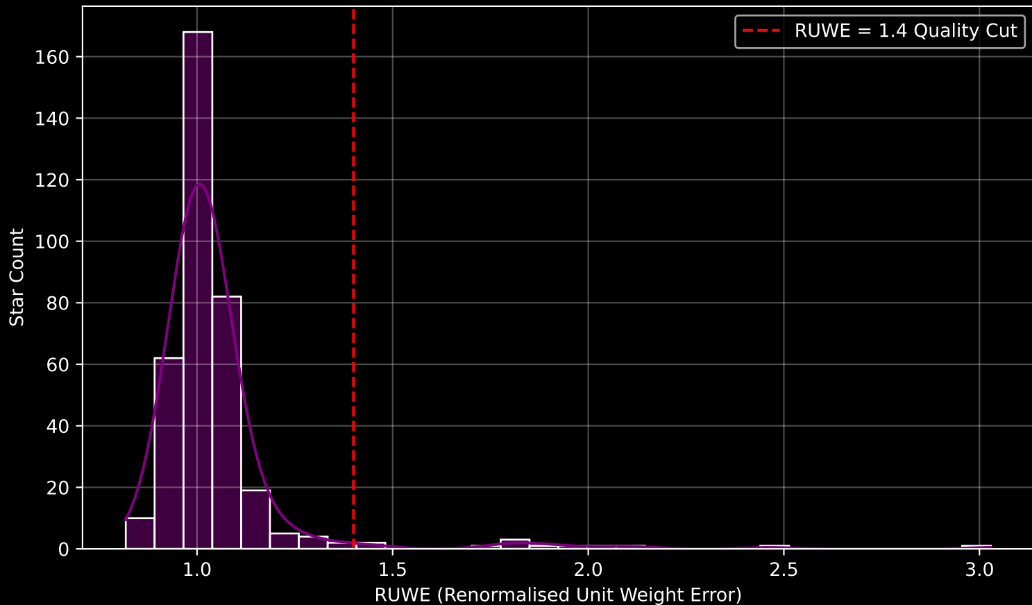
Gaia Cluster: [Westerlund_1] RUWE Distribution (n= 364)
