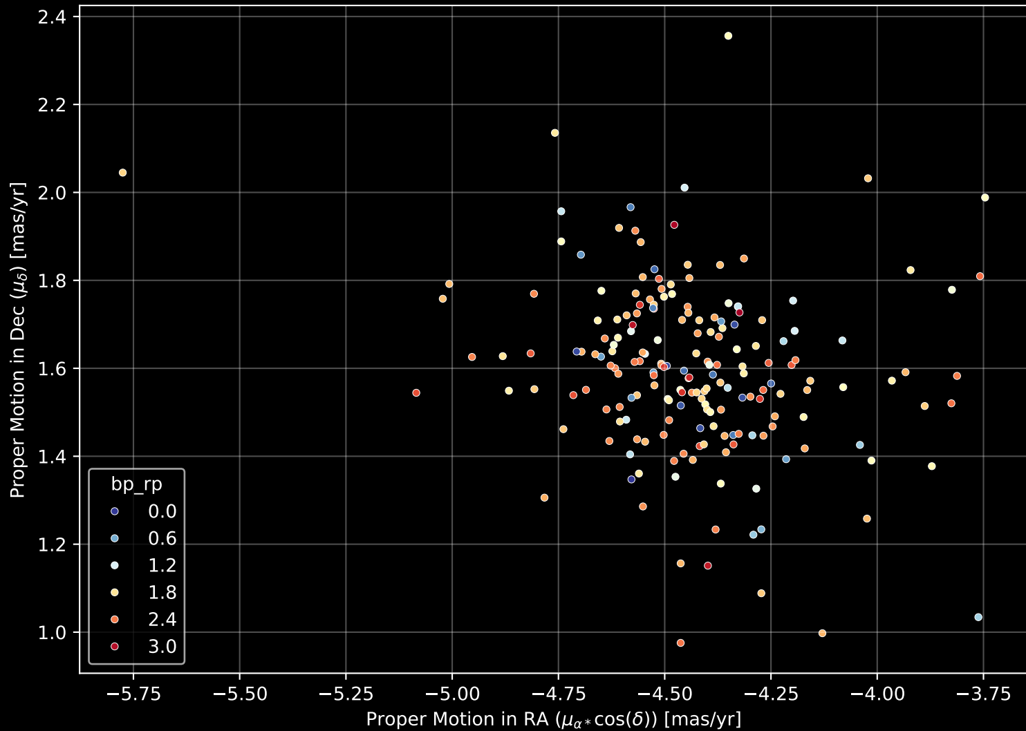
Gaia Cluster: [vdBergh_92] Proper Motion Diagram (n= 192)
