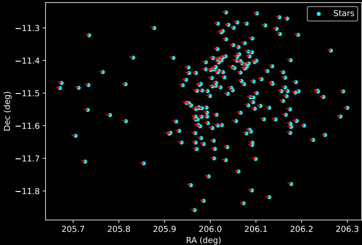
Gaia Cluster: [vdBergh_92] Proper Motion Vectors for Gaia Star Field (n= 192)
