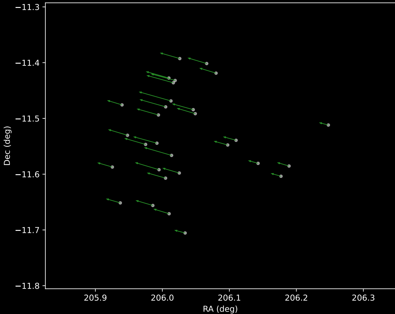
Gaia DR3 Cluster 4 Proper Motion Vectors (n=30)
