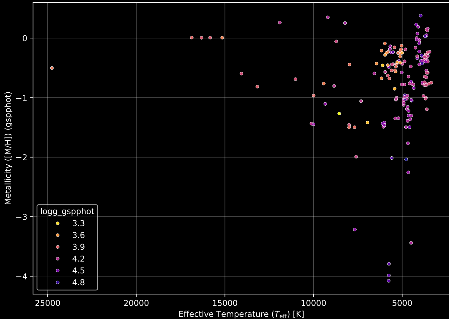
Gaia Cluster: [vdBergh_92] Stellar Population Parameters (n= 192)
