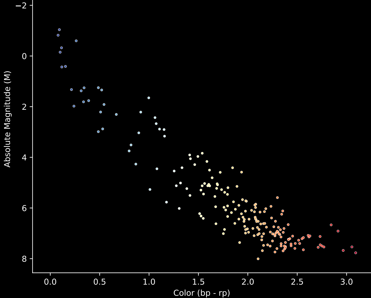
Gaia Cluster: [vdBergh_92] Stars (n= 192) Hertzsprung-Russel Diagram
