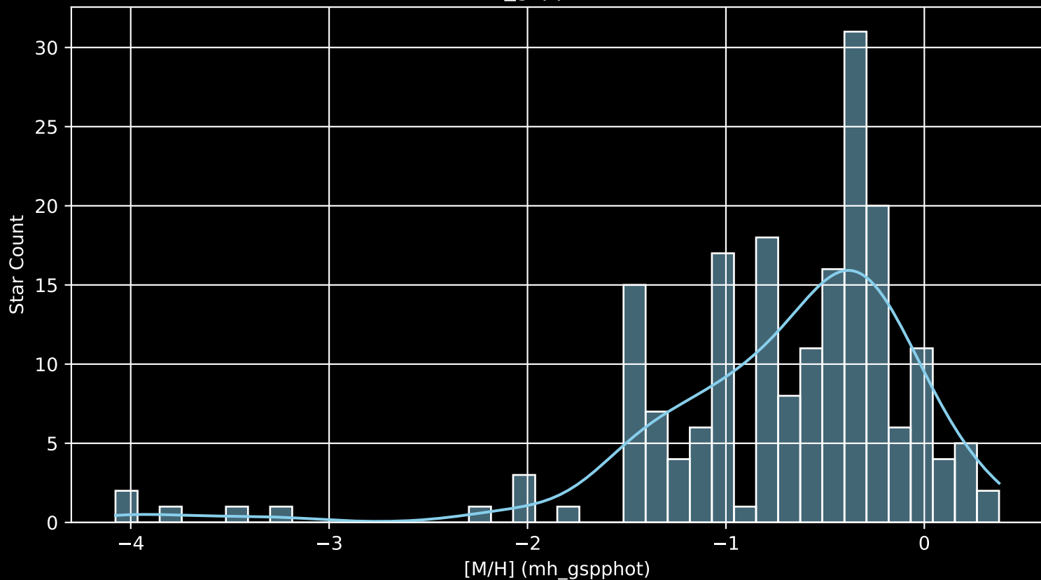
Gaia Cluster: [vdBergh_92 [M/H] (mh_gspphot) (n= 192)
