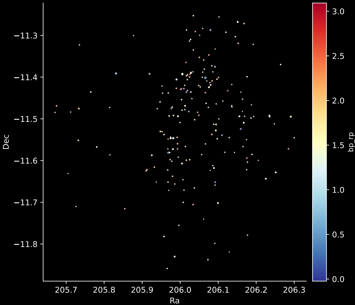
Gaia Cluster: [vdBergh_92] Stars: 192
