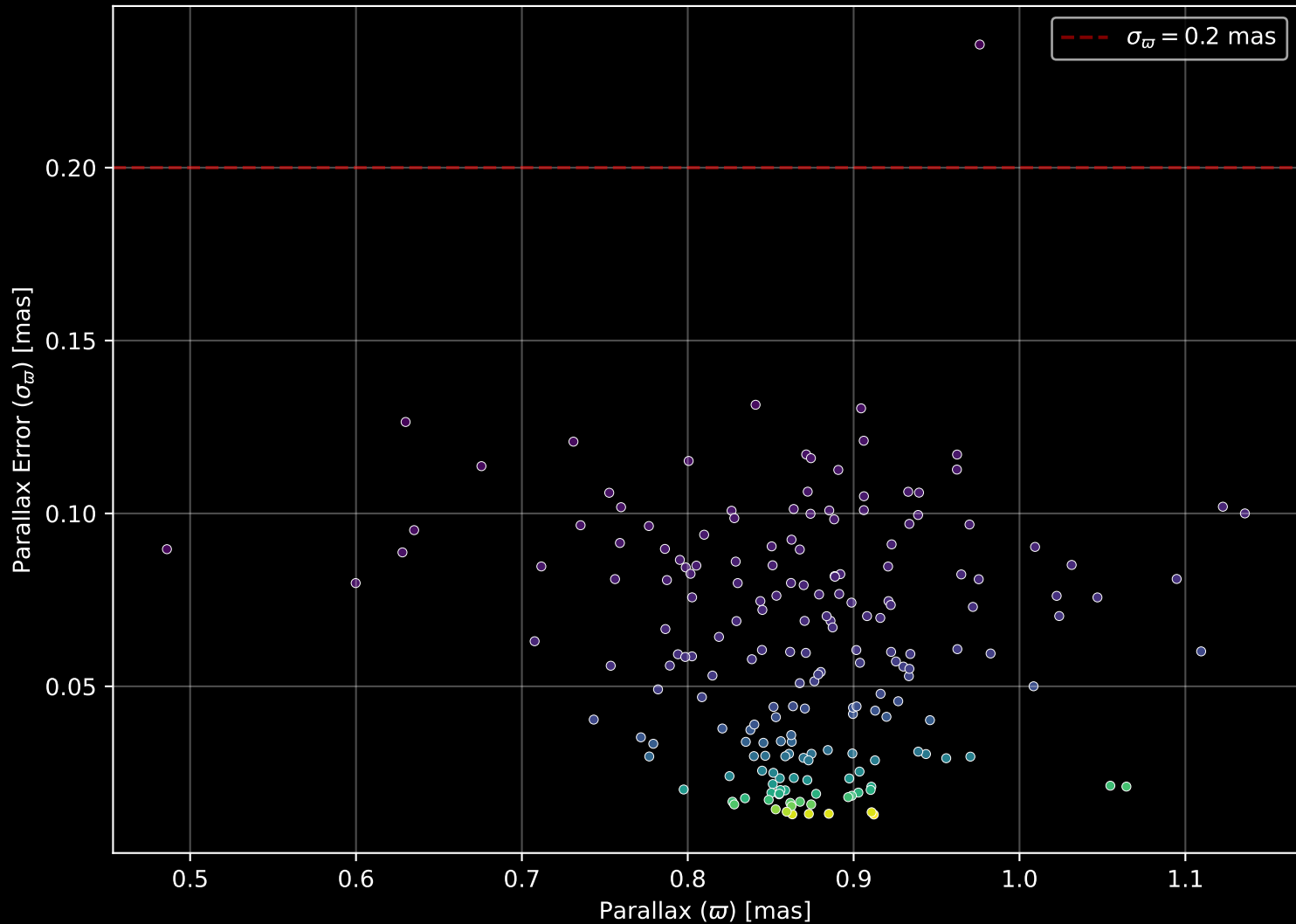
Gaia Cluster: [vdBergh_92] Parallax Quality (n= 192)
