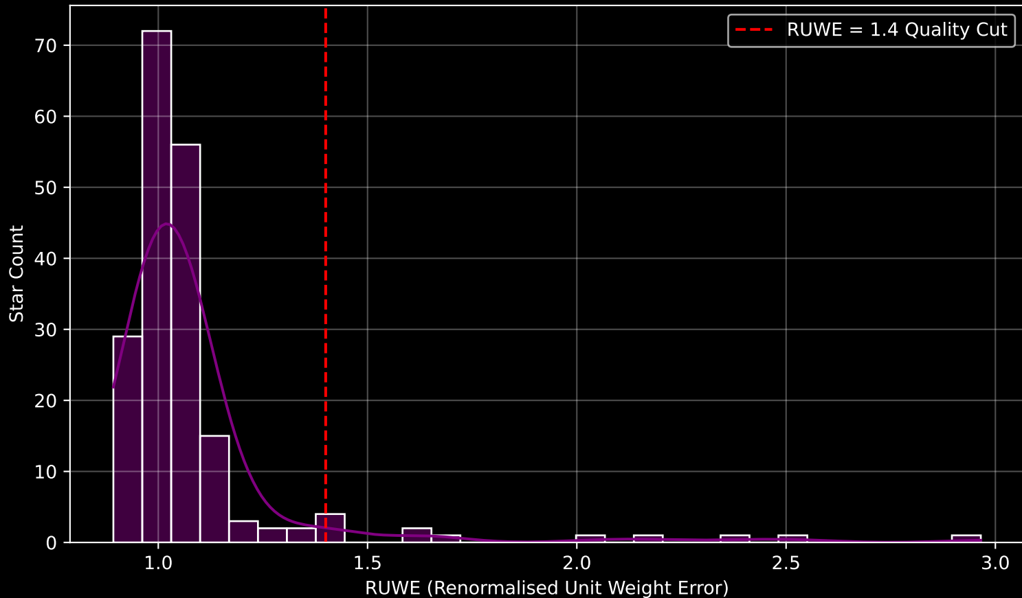
Gaia Cluster: [vdBergh_92] RUWE Distribution (n= 191)
