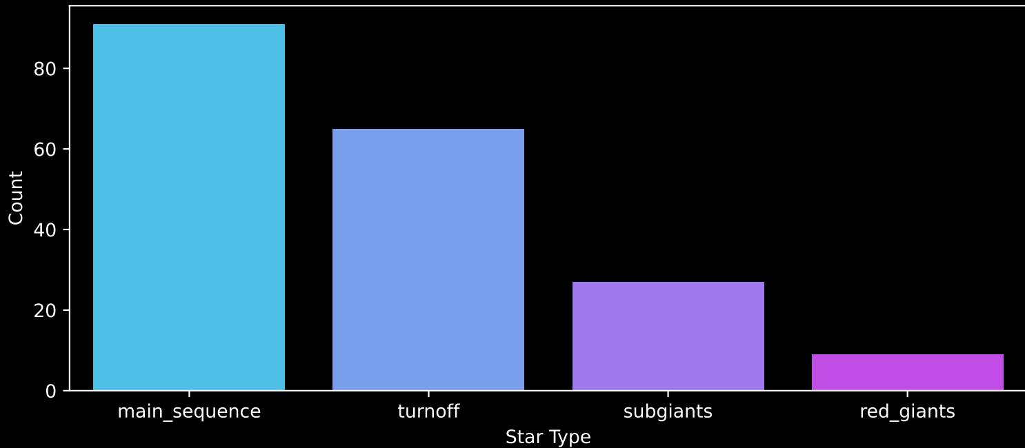
Gaia Cluster: [vdBergh_92] Count plot of Star Type
