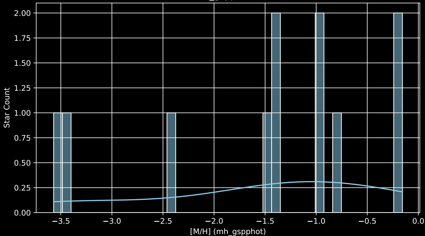
Gaia Stream: [C-19 [M/H] (mh_gspphot) (n= 11)
