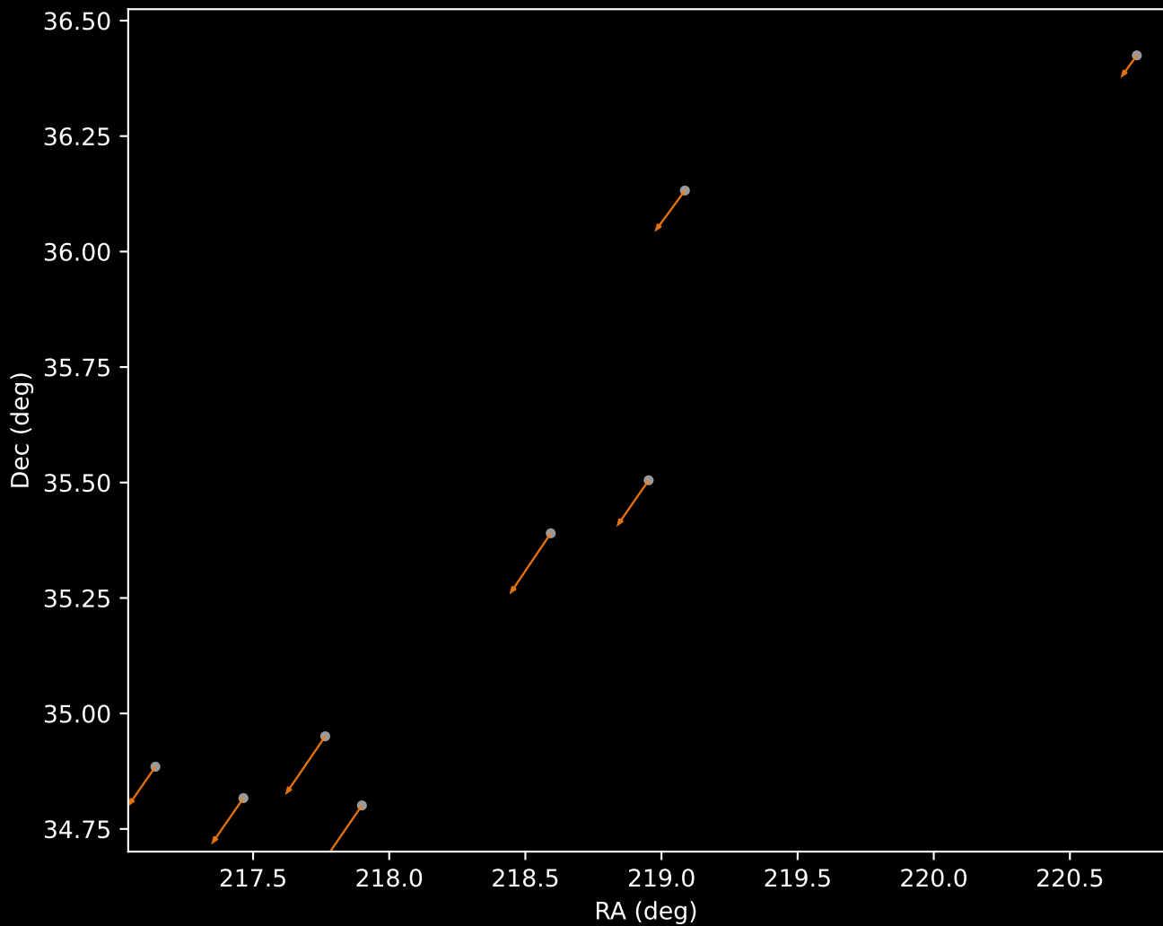
Gaia DR3 Cluster 2 Proper Motion Vectors (n=8)
