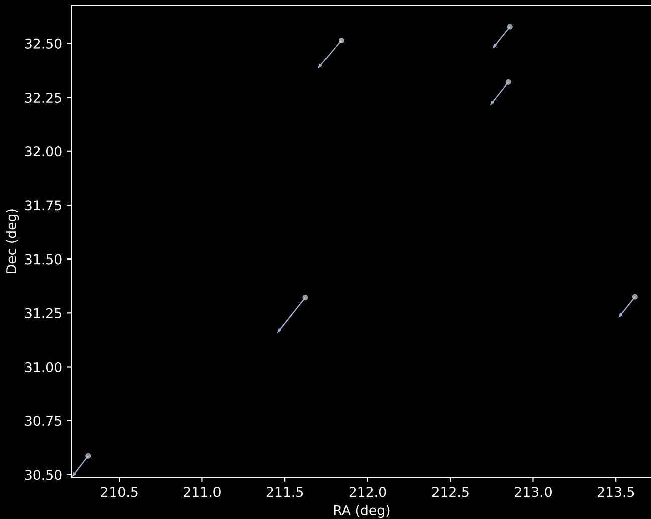
Gaia DR3 Cluster 1 Proper Motion Vectors (n=6)
