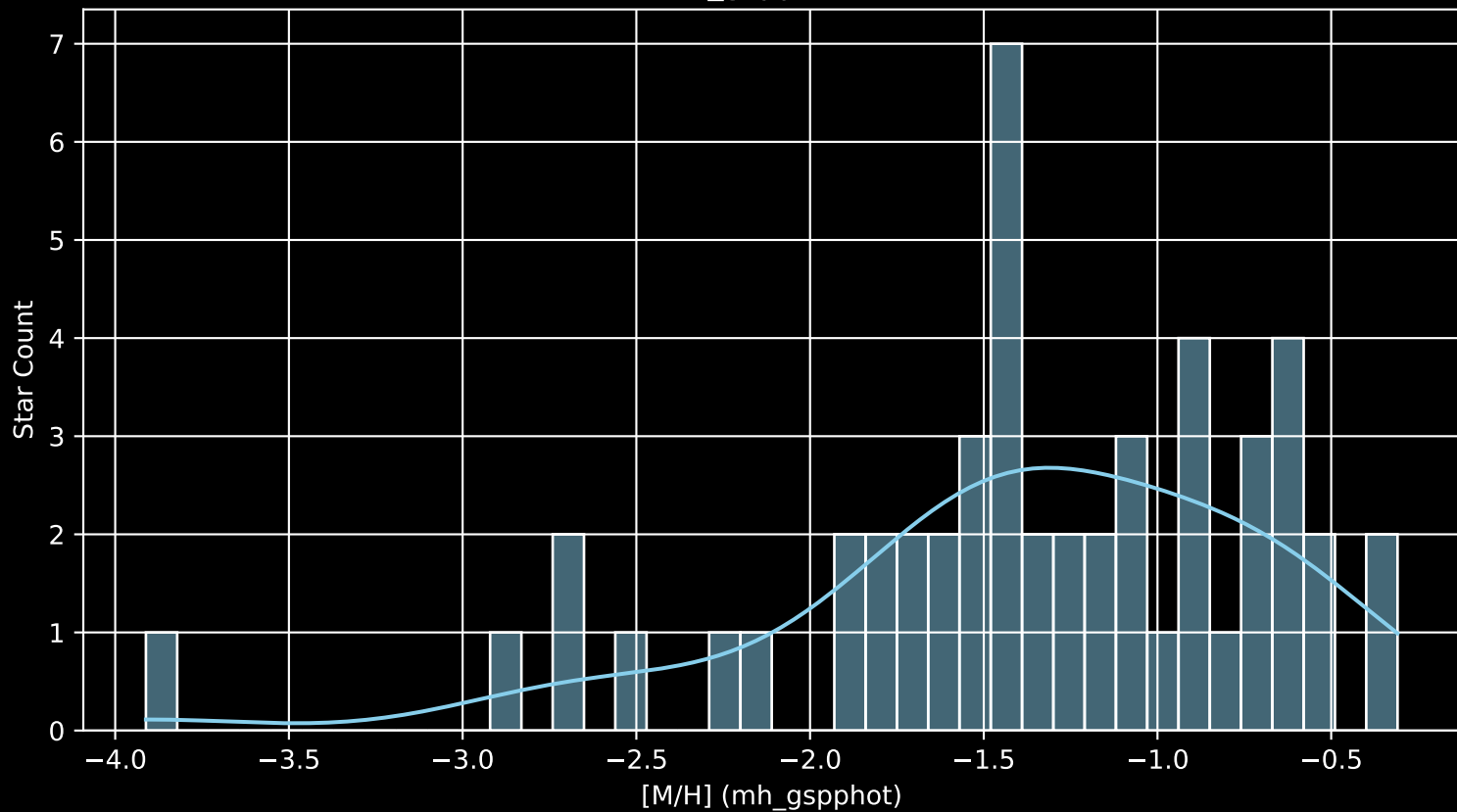
Gaia Stream: [Gaia-6 [M/H] (mh_gspphot) (n= 51)
