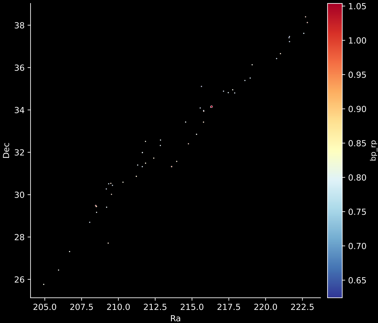
Gaia Stream: [Gaia-6] Stars: 51
