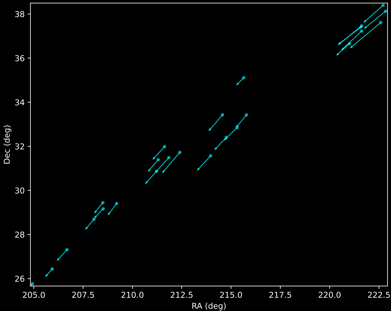
Gaia DR3 Noise Stream Proper Motion Vectors (n=25)
