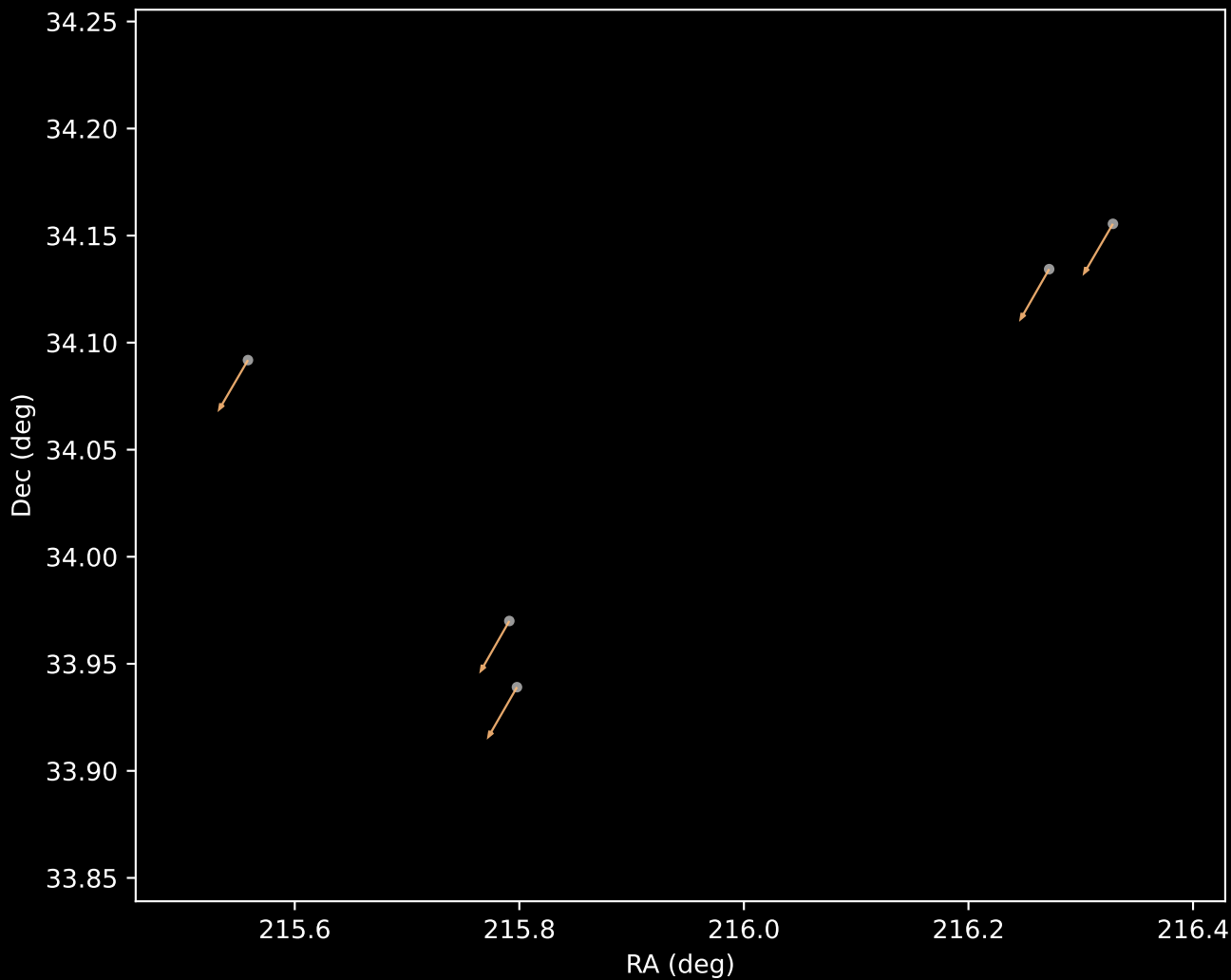
Gaia DR3 Cluster 3 Proper Motion Vectors (n=5)
