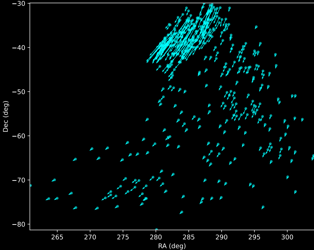
Gaia DR3 Noise Stream Proper Motion Vectors (n=372)
