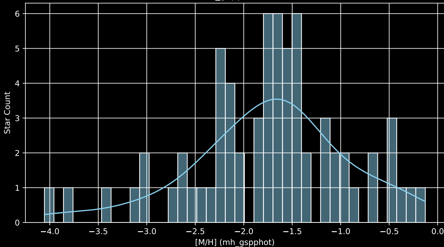
Gaia Stream: [Kshir [M/H] (mh_gspphot) (n= 67)
