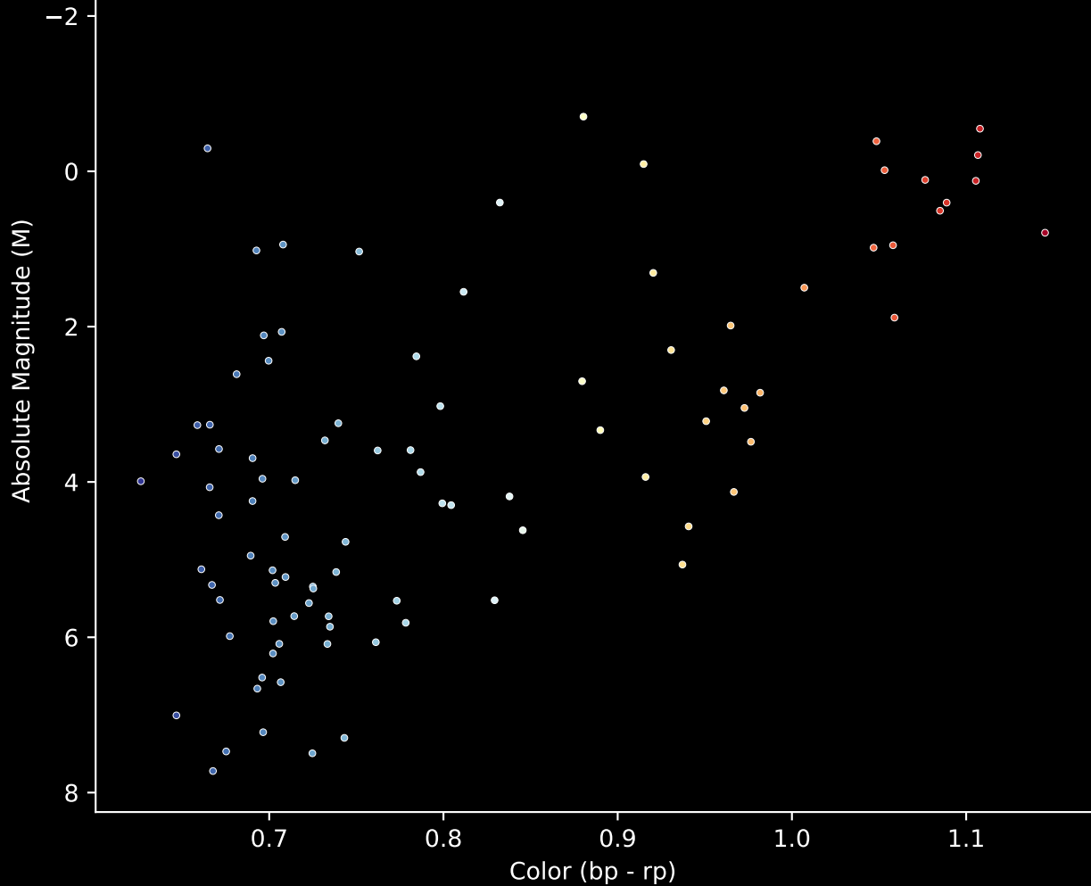
Gaia Stream: [NGC288] Stream (n= 97) Hertzsprung-Russel Diagram
