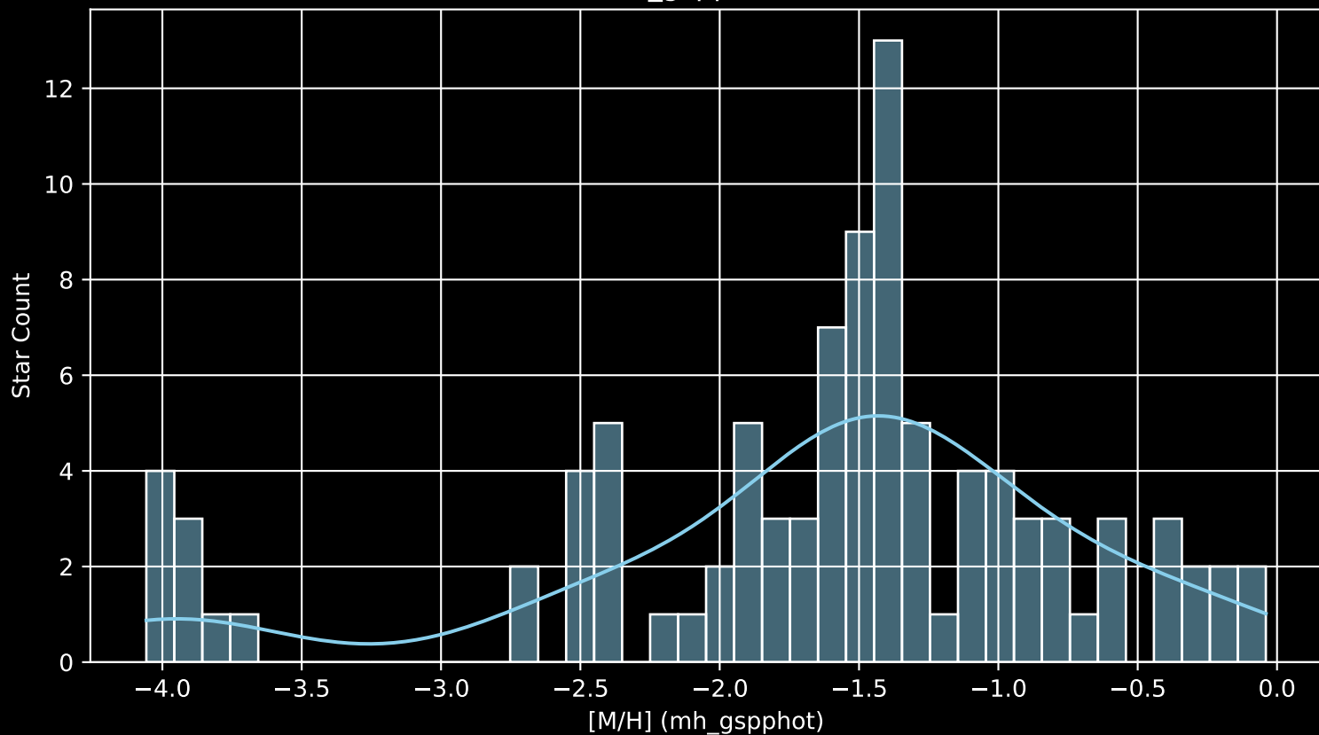
Gaia Stream: [NGC288 [M/H] (mh_gspphot) (n= 97)
