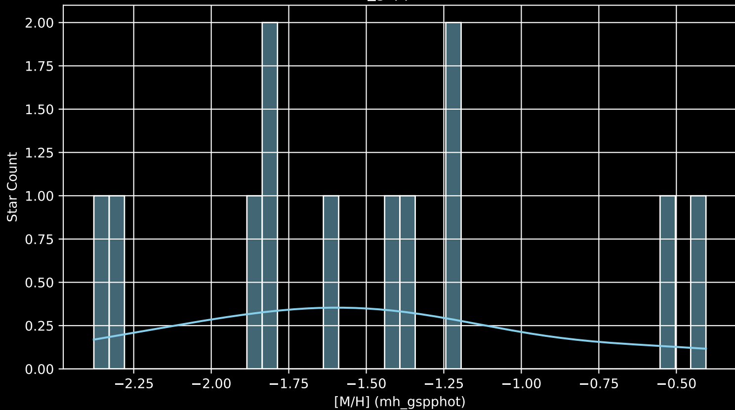
Gaia Stream: [NGC5466 [M/H] (mh_gspphot) (n= 12)
