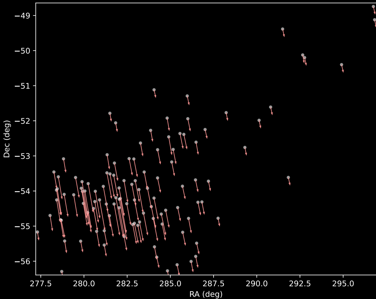
Gaia DR3 Cluster 7 Proper Motion Vectors (n=110)
