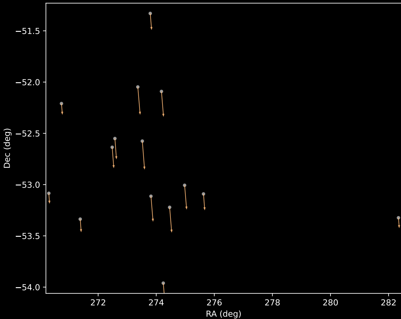
Gaia DR3 Cluster 3 Proper Motion Vectors (n=15)
