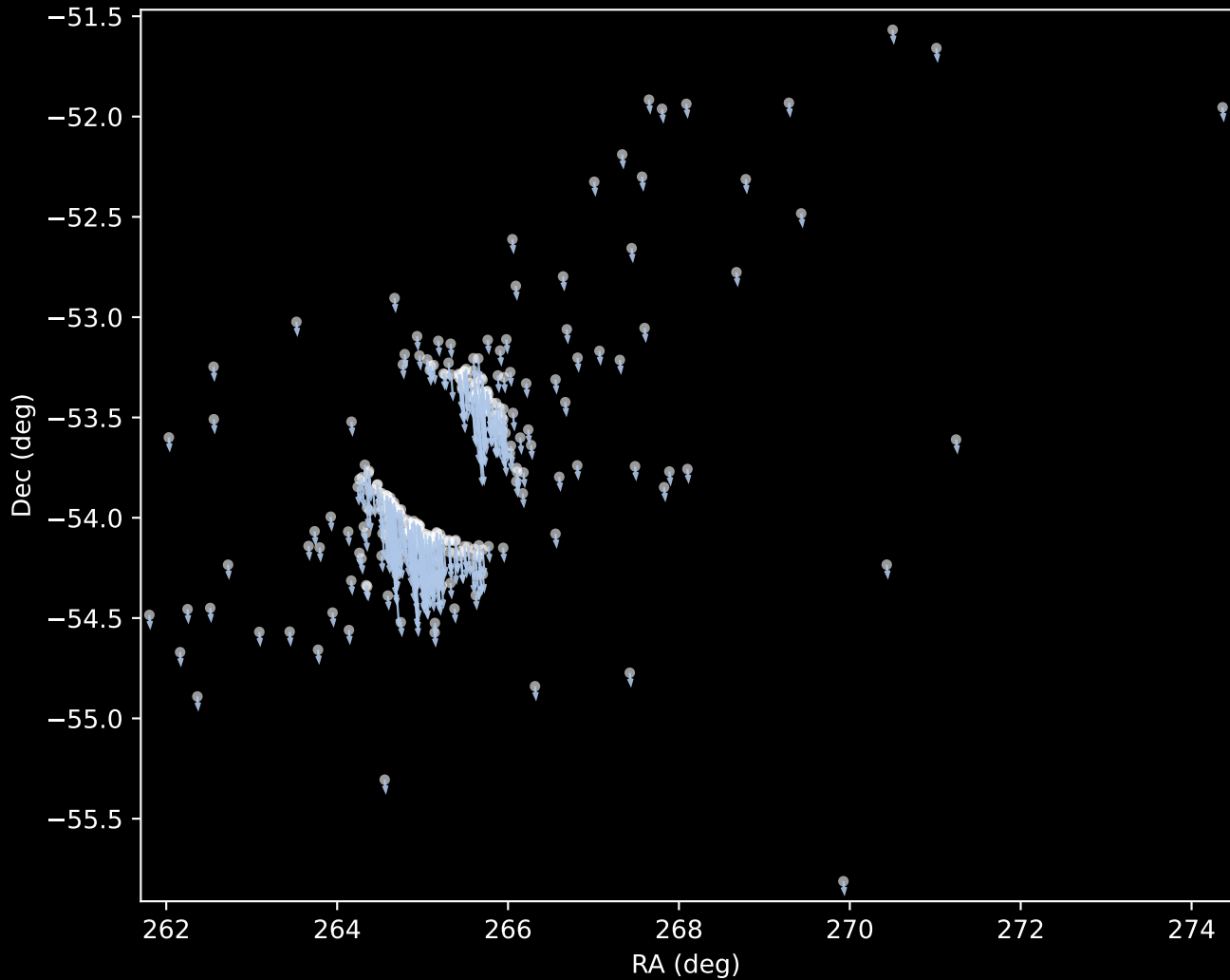
Gaia DR3 Cluster 1 Proper Motion Vectors (n=295)
