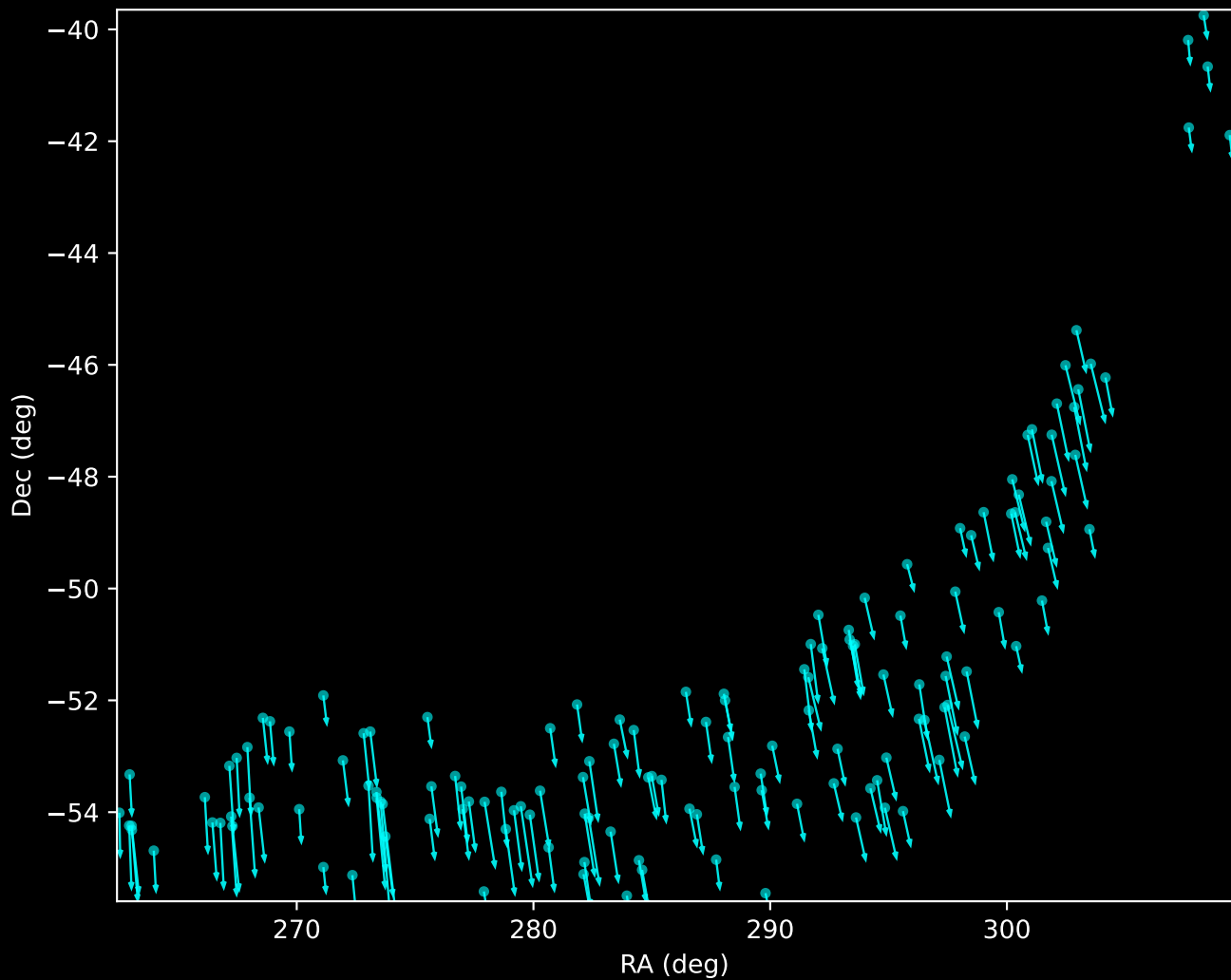
Gaia DR3 Noise Stream Proper Motion Vectors (n=143)
