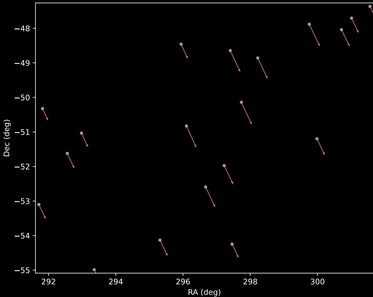
Gaia DR3 Cluster 12 Proper Motion Vectors (n=19)
