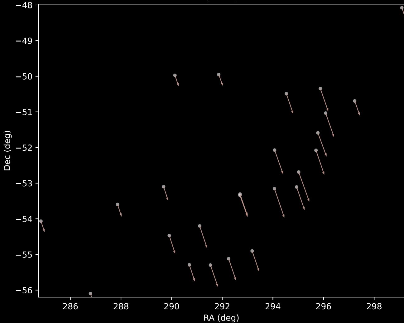
Gaia DR3 Cluster 11 Proper Motion Vectors (n=25)
