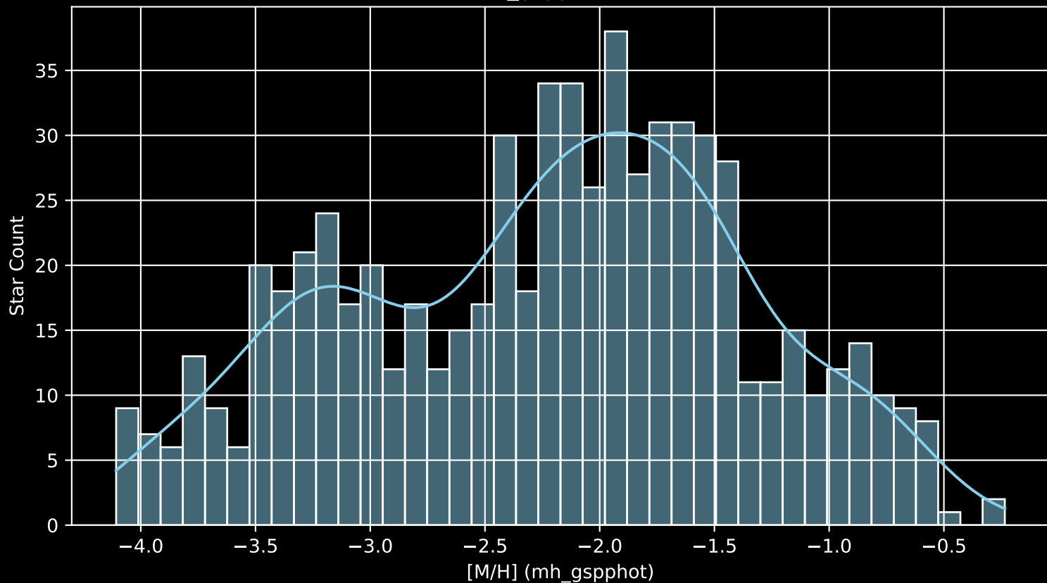
Gaia Stream: [NGC6397 [M/H] (mh_gspphot) (n= 673)
