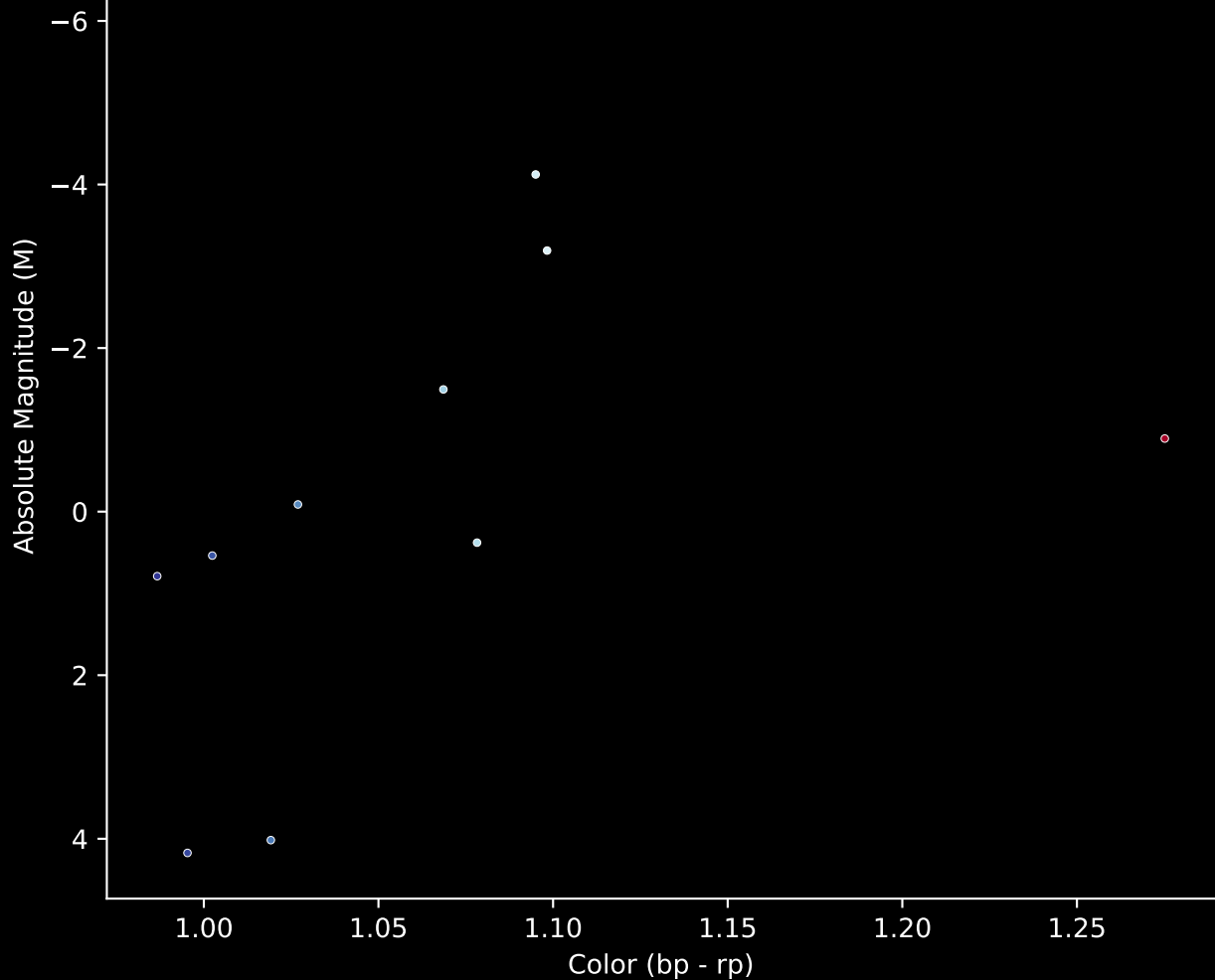
Gaia Stream: [NGC7492] Stream (n= 11) Hertzsprung-Russel Diagram
