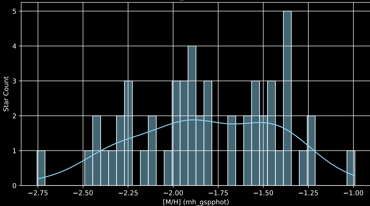
Gaia Stream: [New-2 [M/H] (mh_gspphot) (n= 52)
