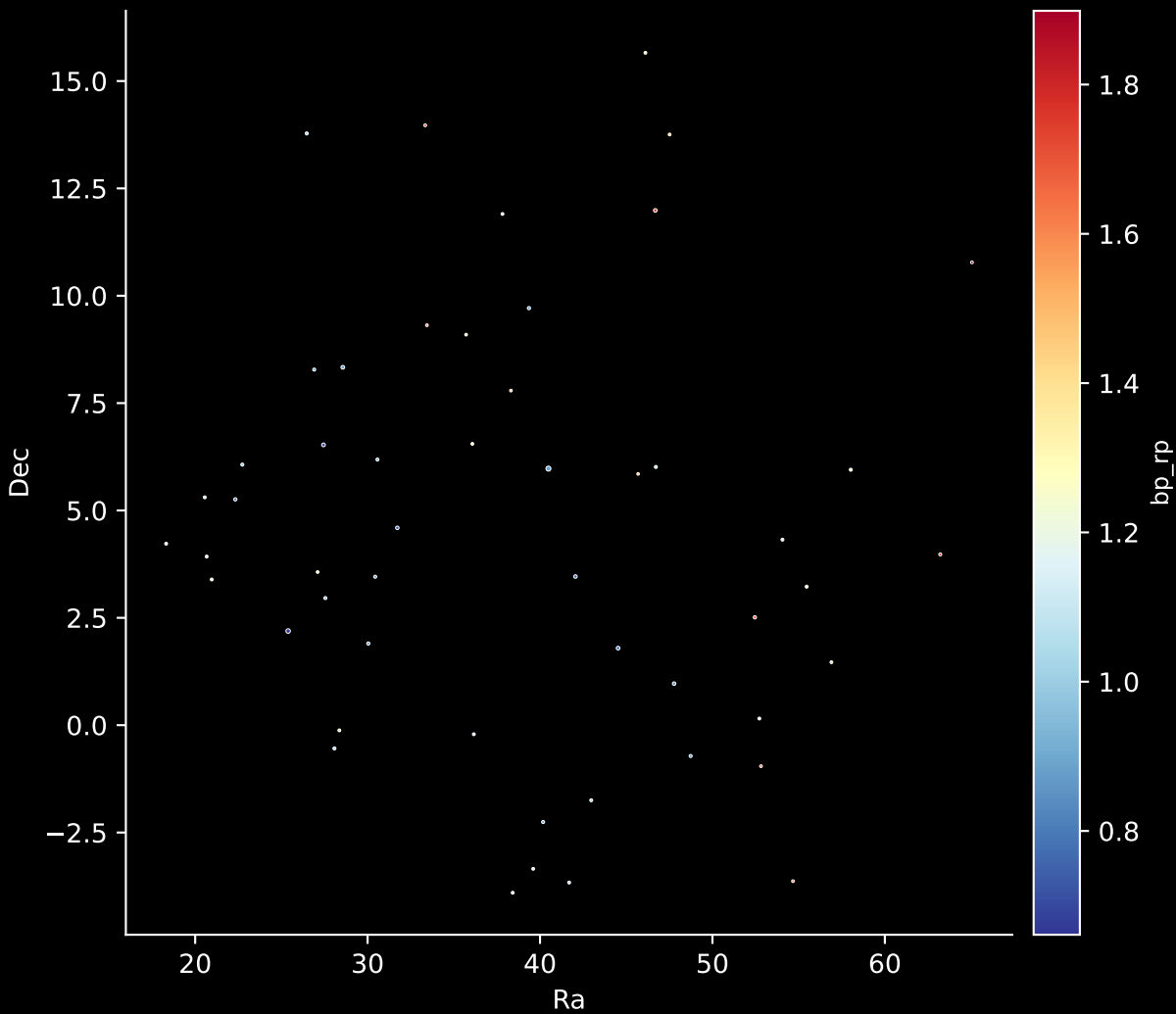
Gaia Stream: [New-2] Stars: 52
