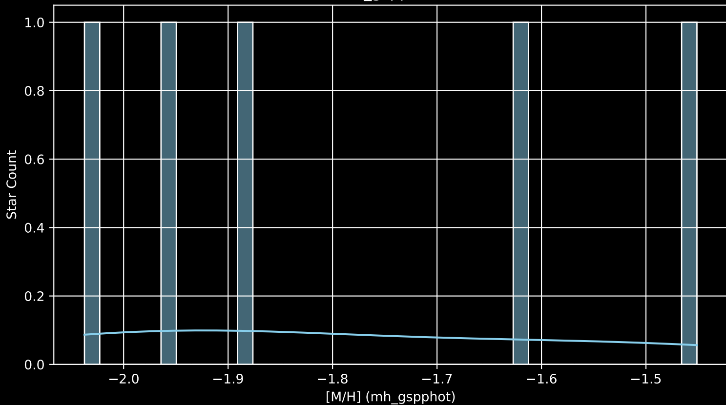
Gaia Stream: [New-20 [M/H] (mh_gspphot) (n= 5)
