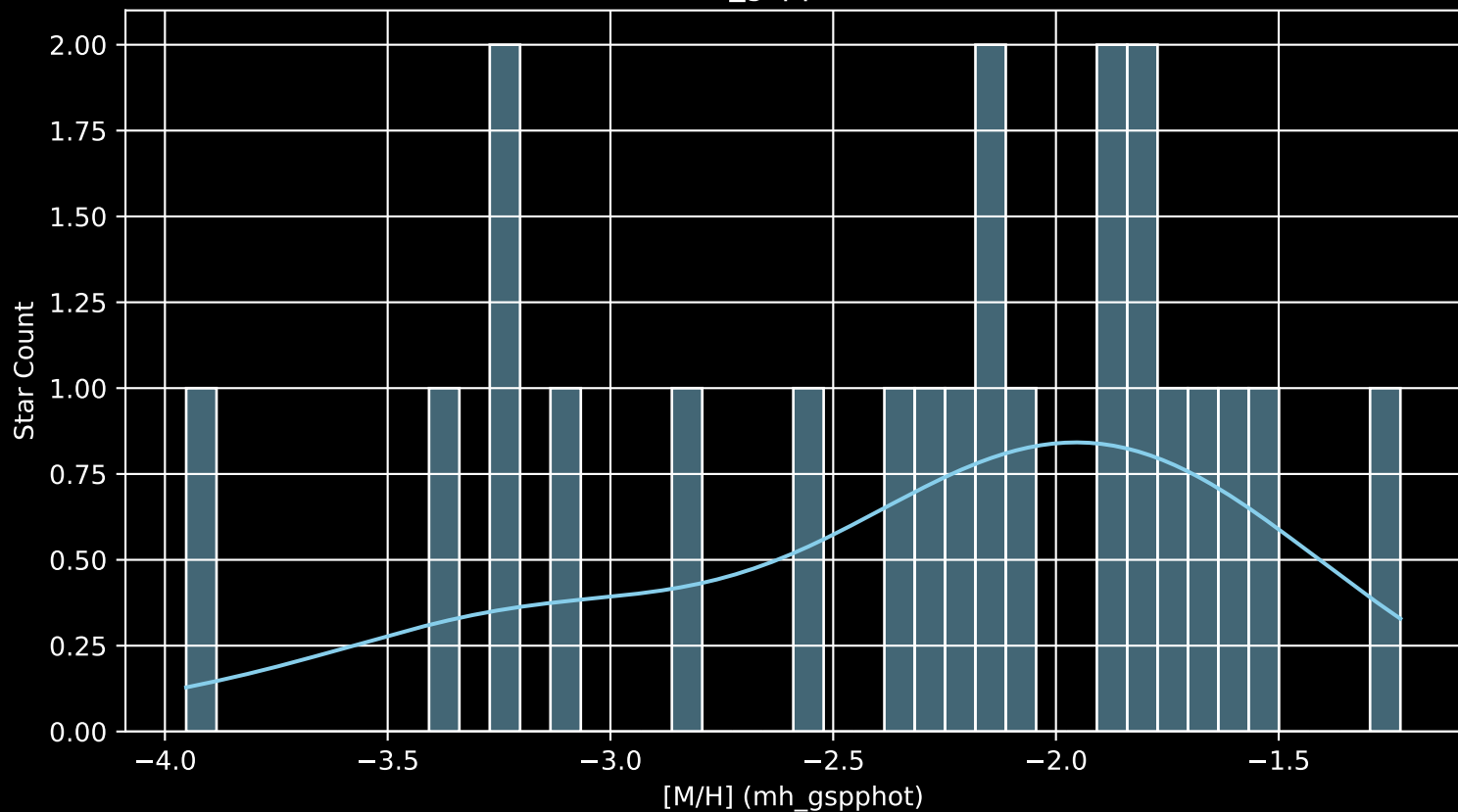
Gaia Stream: [New-7 [M/H] (mh_gspphot) (n= 22)
