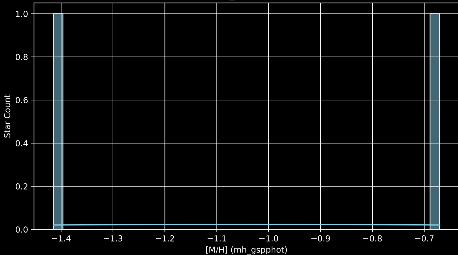
Gaia Stream: [New-8 [M/H] (mh_gspphot) (n= 2)
