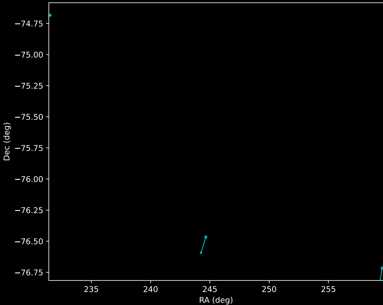
Gaia DR3 Noise Stream Proper Motion Vectors (n=3)
