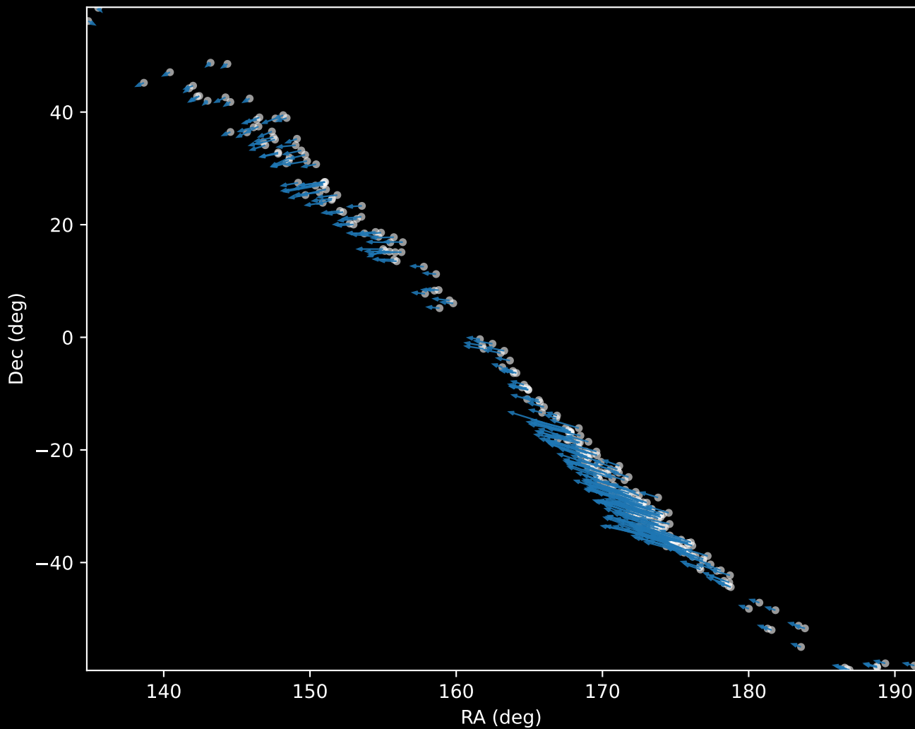
Gaia DR3 Cluster 0 Proper Motion Vectors (n=260)
