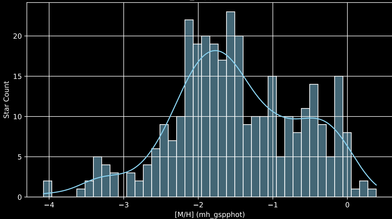
Gaia Stream: [Orphan [M/H] (mh_gspphot) (n= 331)
