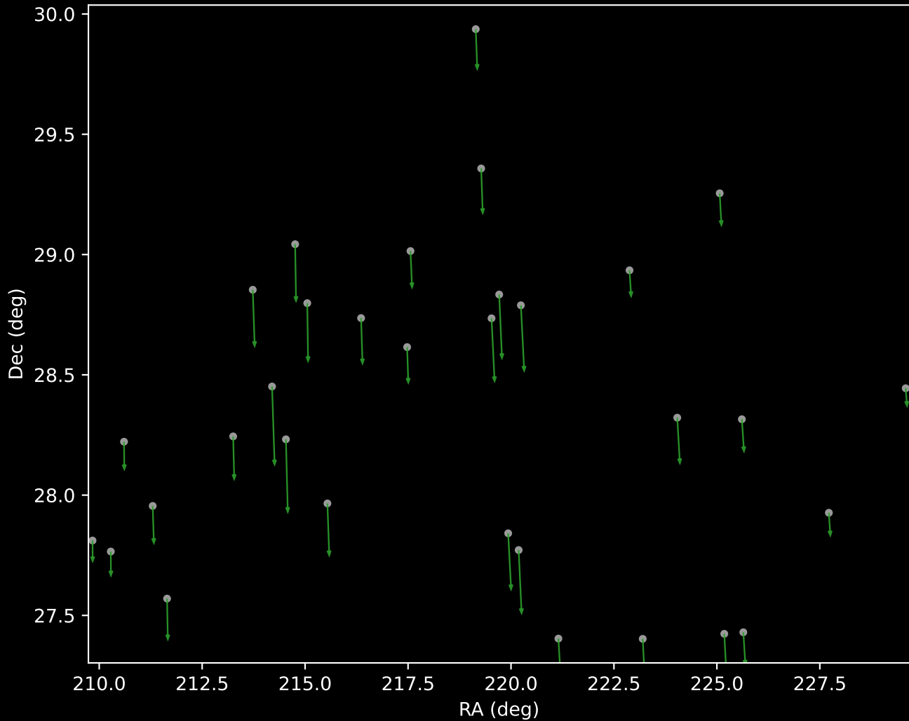
Gaia DR3 Cluster 4 Proper Motion Vectors (n=32)
