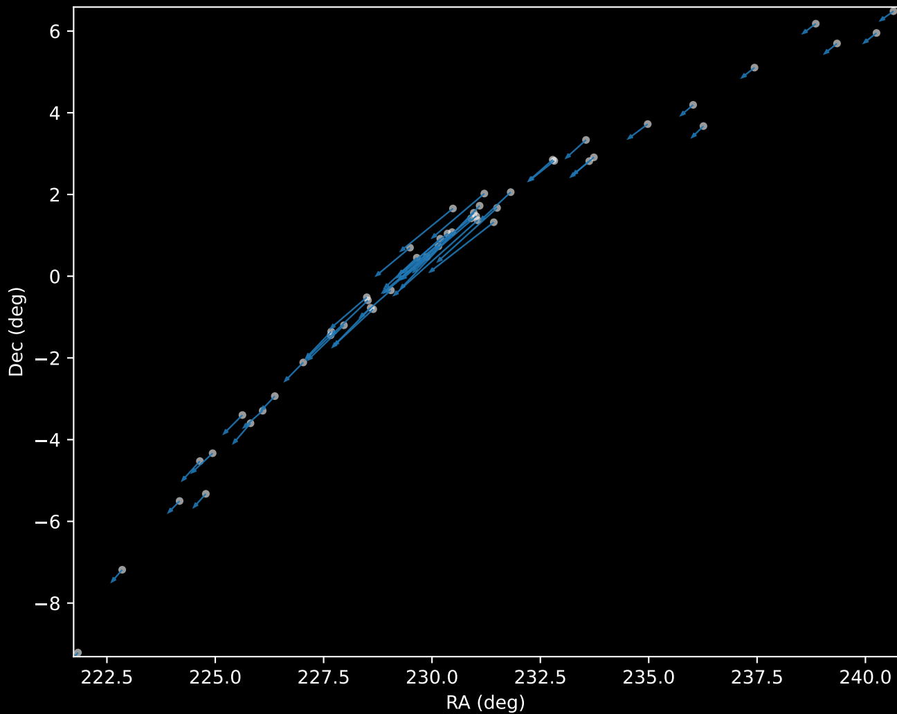
Gaia DR3 Cluster 0 Proper Motion Vectors (n=49)
