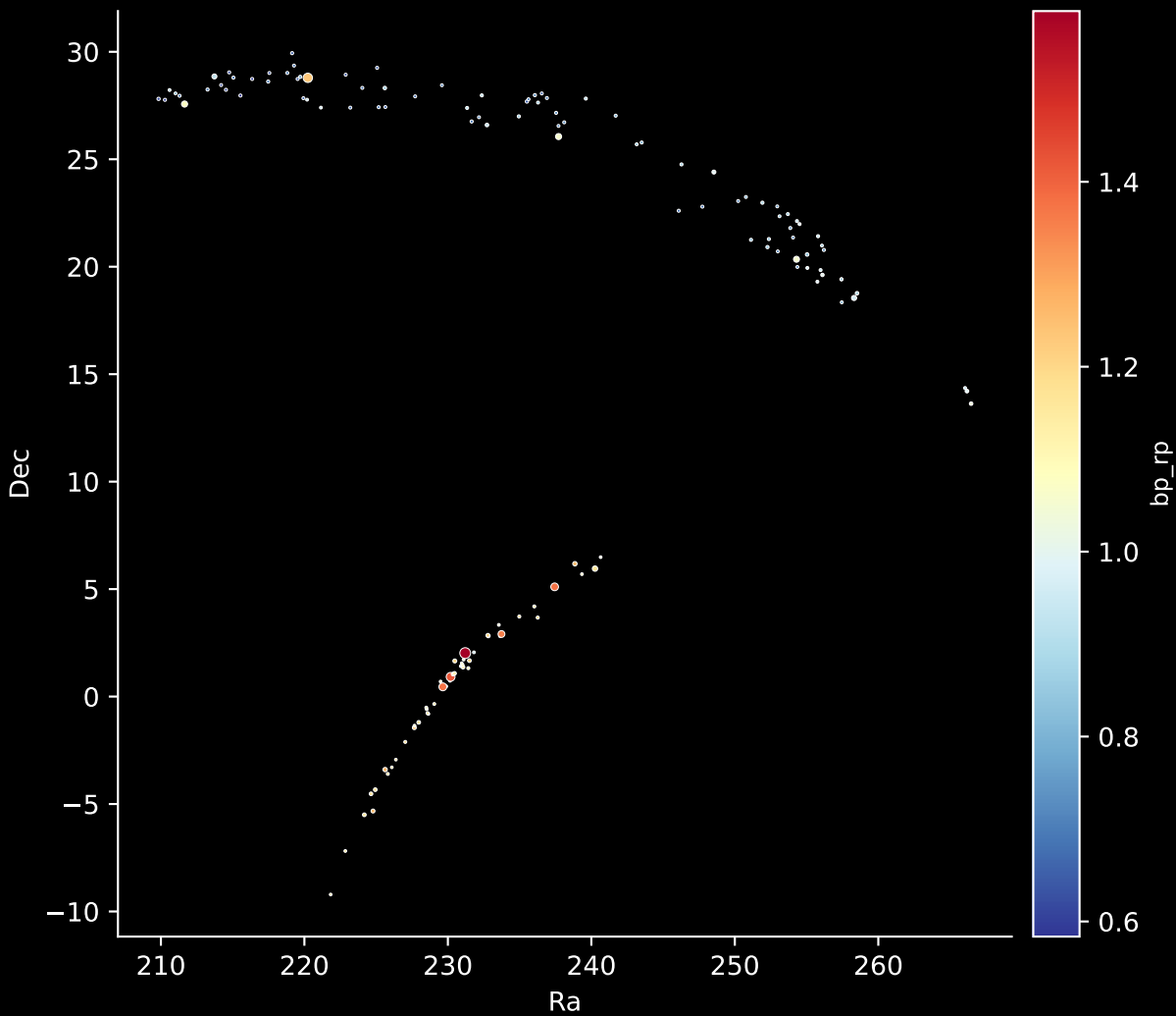
Gaia Stream: [Pal_5] Stars: 139
