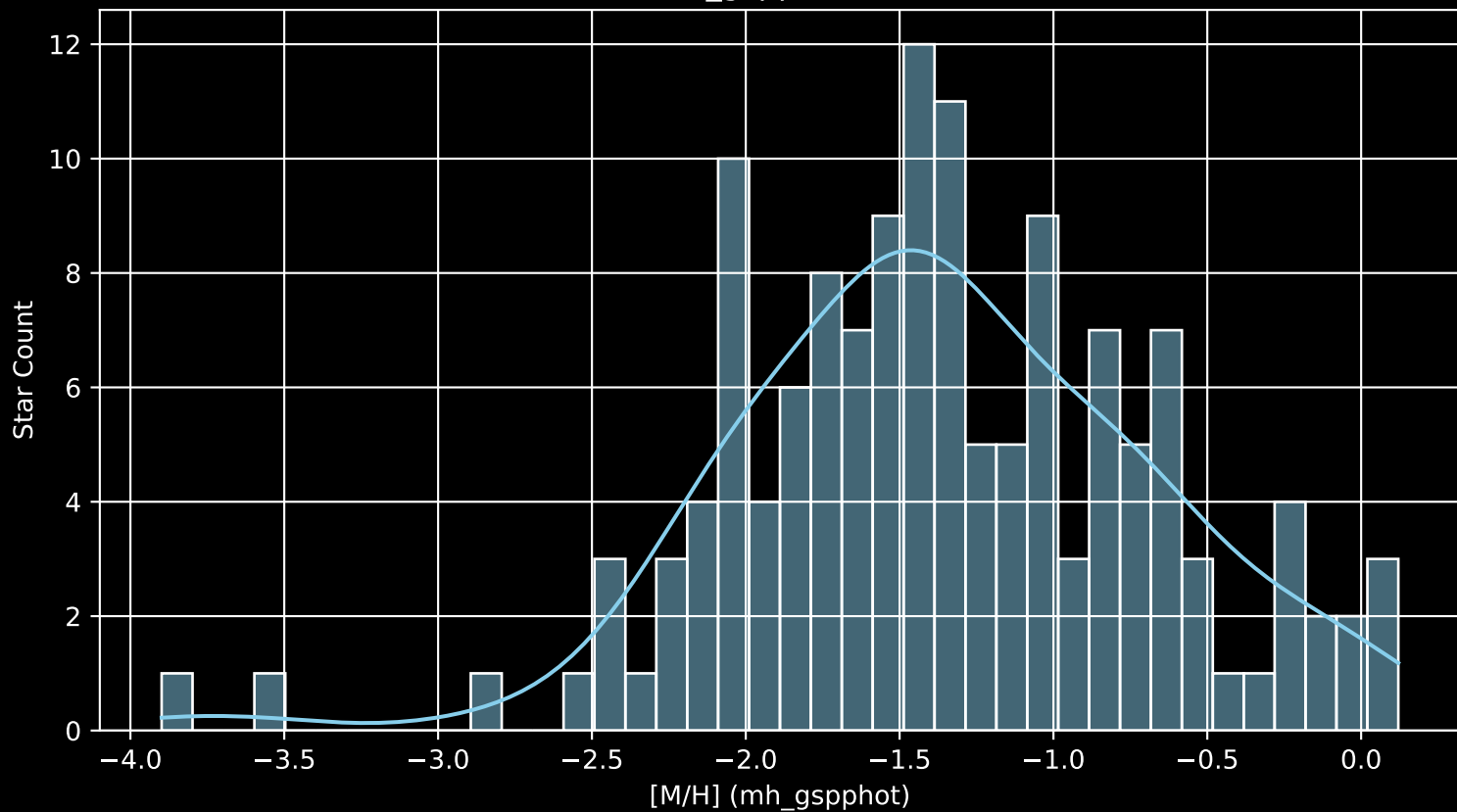
Gaia Stream: [Pal_5 [M/H] (mh_gspphot) (n= 139)
