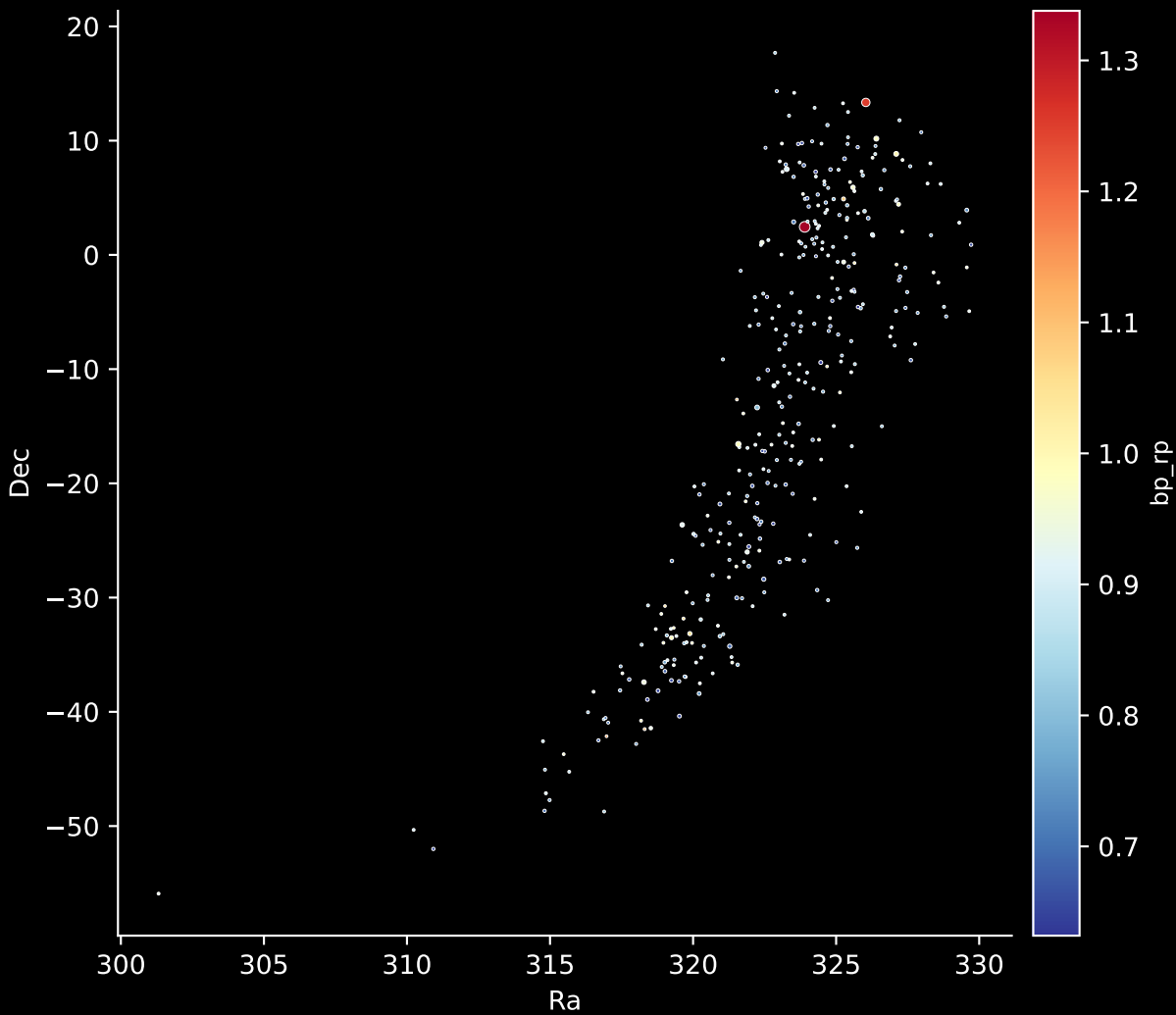
Gaia Stream: [Phlegethon] Stars: 350
