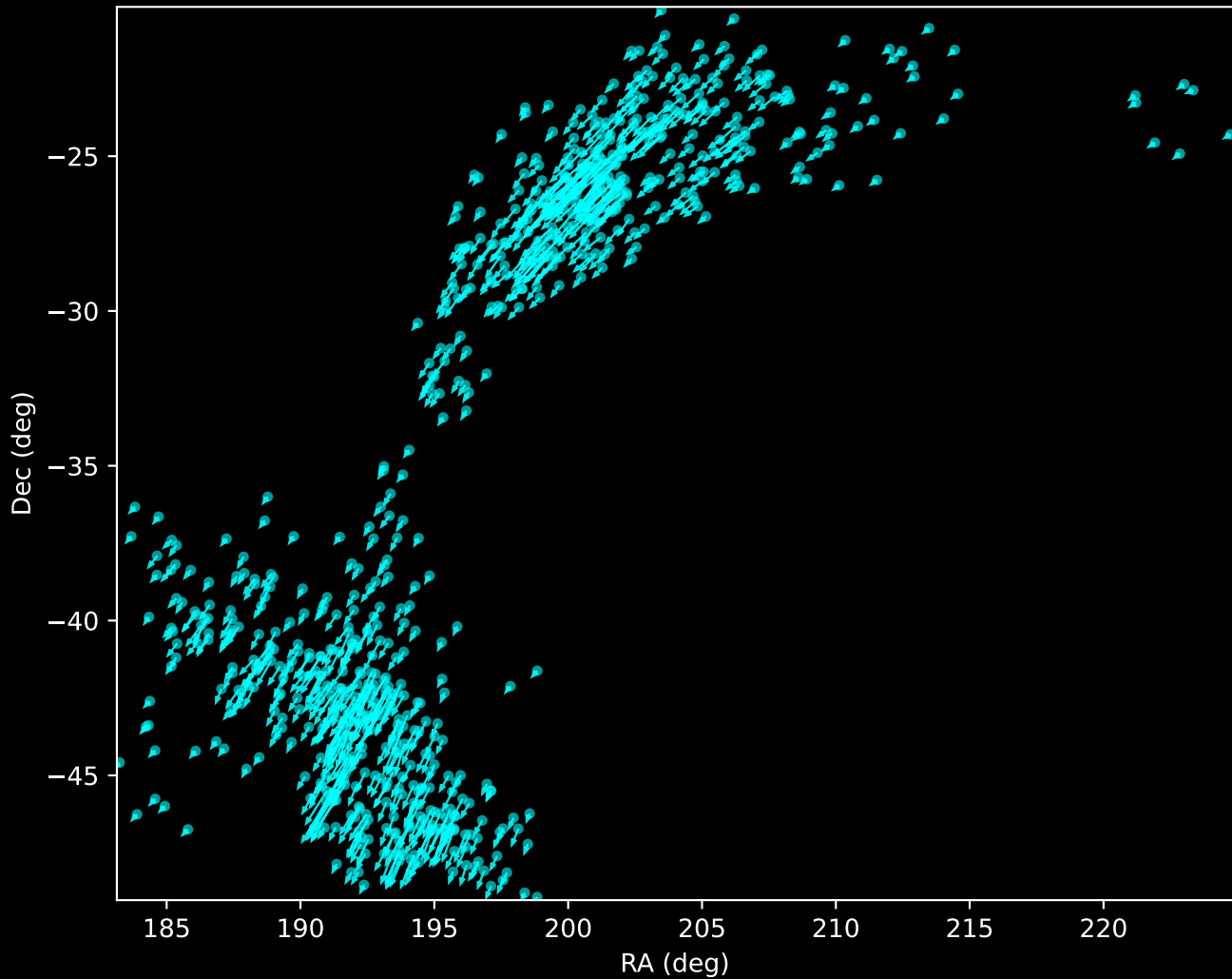
Gaia DR3 Noise Stream Proper Motion Vectors (n=726)
