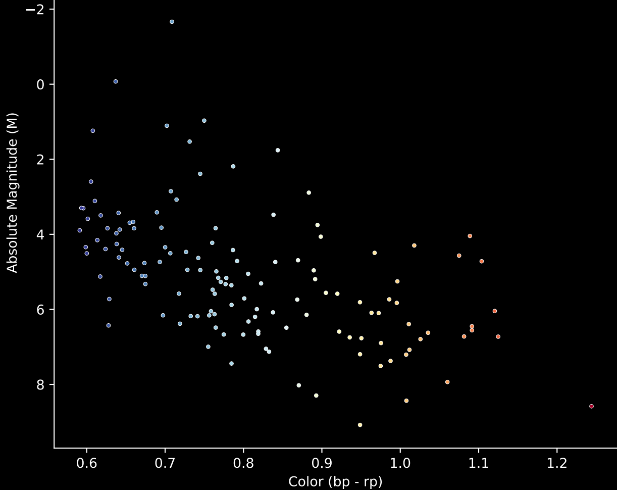
Gaia Stream: [Sylgr] Stream (n= 135) Hertzsprung-Russel Diagram
