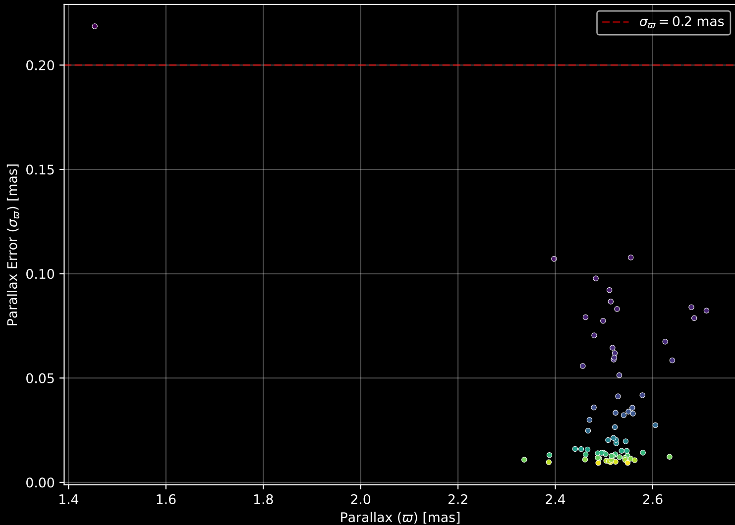
Gaia Cluster: [ASCC_101] Parallax Quality (n= 72)
