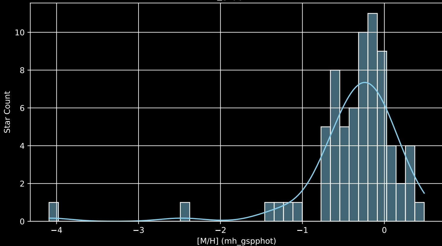
Gaia Cluster: [ASCC_101 [M/H] (mh_gspphot) (n= 71)
