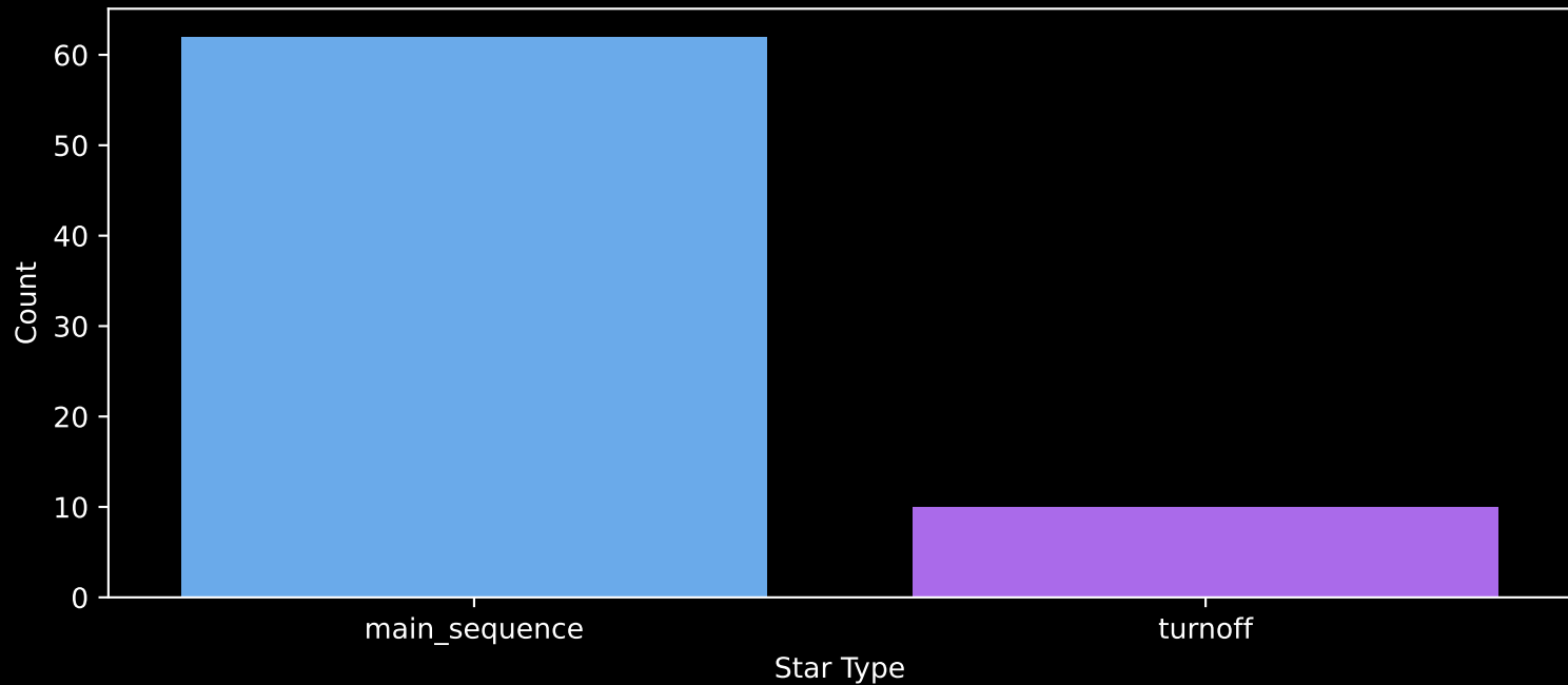
Gaia Cluster: [ASCC_101] Count plot of Star Type
