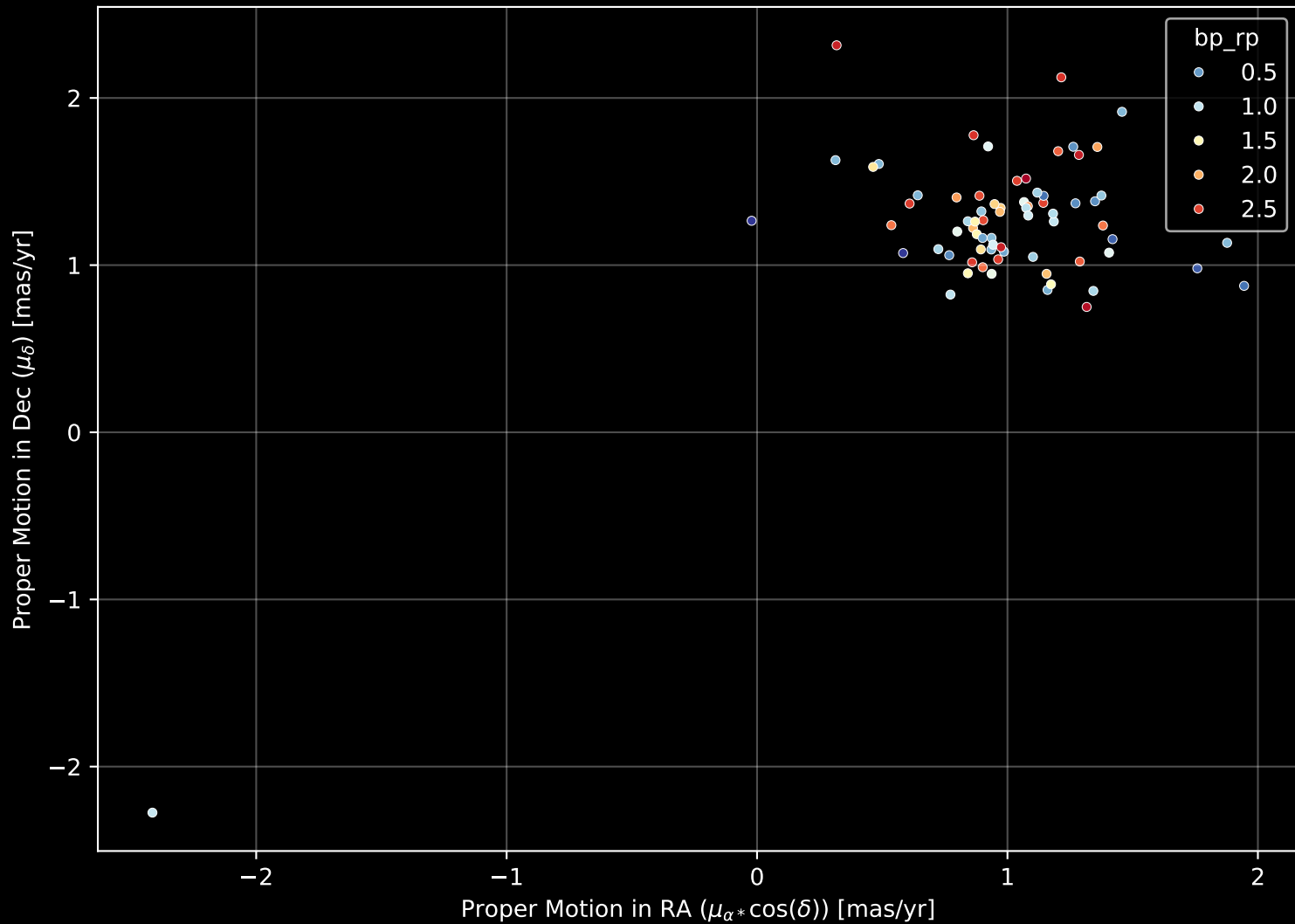
Gaia Cluster: [ASCC_101] Proper Motion Diagram (n= 72)
