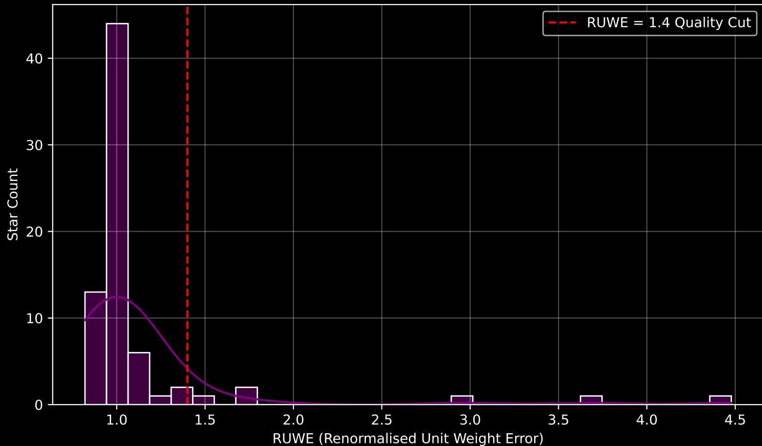
Gaia Cluster: [ASCC_101] RUWE Distribution (n= 72)
