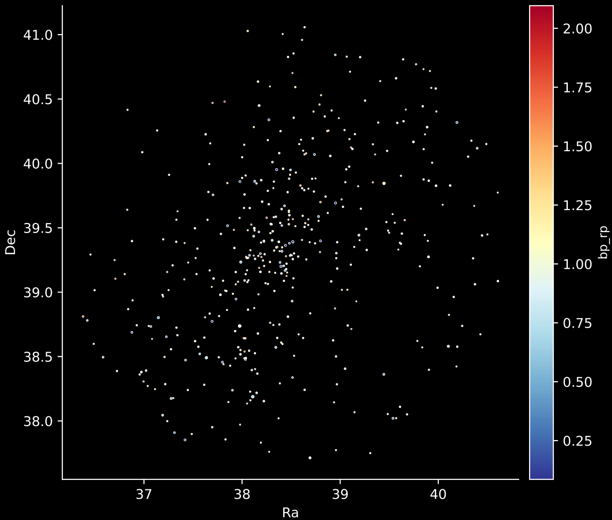
Gaia Cluster: [ASCC_108] Stars: 439
