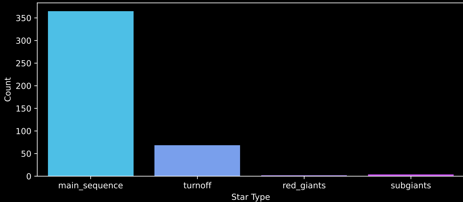
Gaia Cluster: [ASCC_108] Count plot of Star Type
