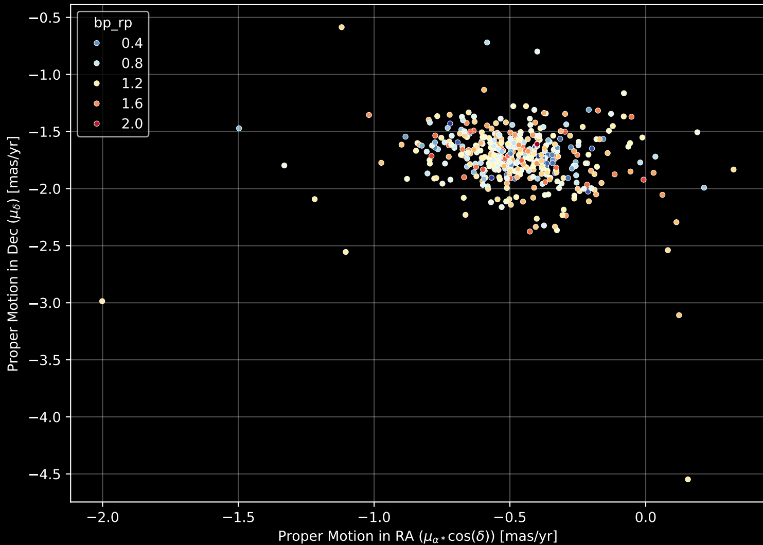
Gaia Cluster: [ASCC_108] Proper Motion Diagram (n= 439)
