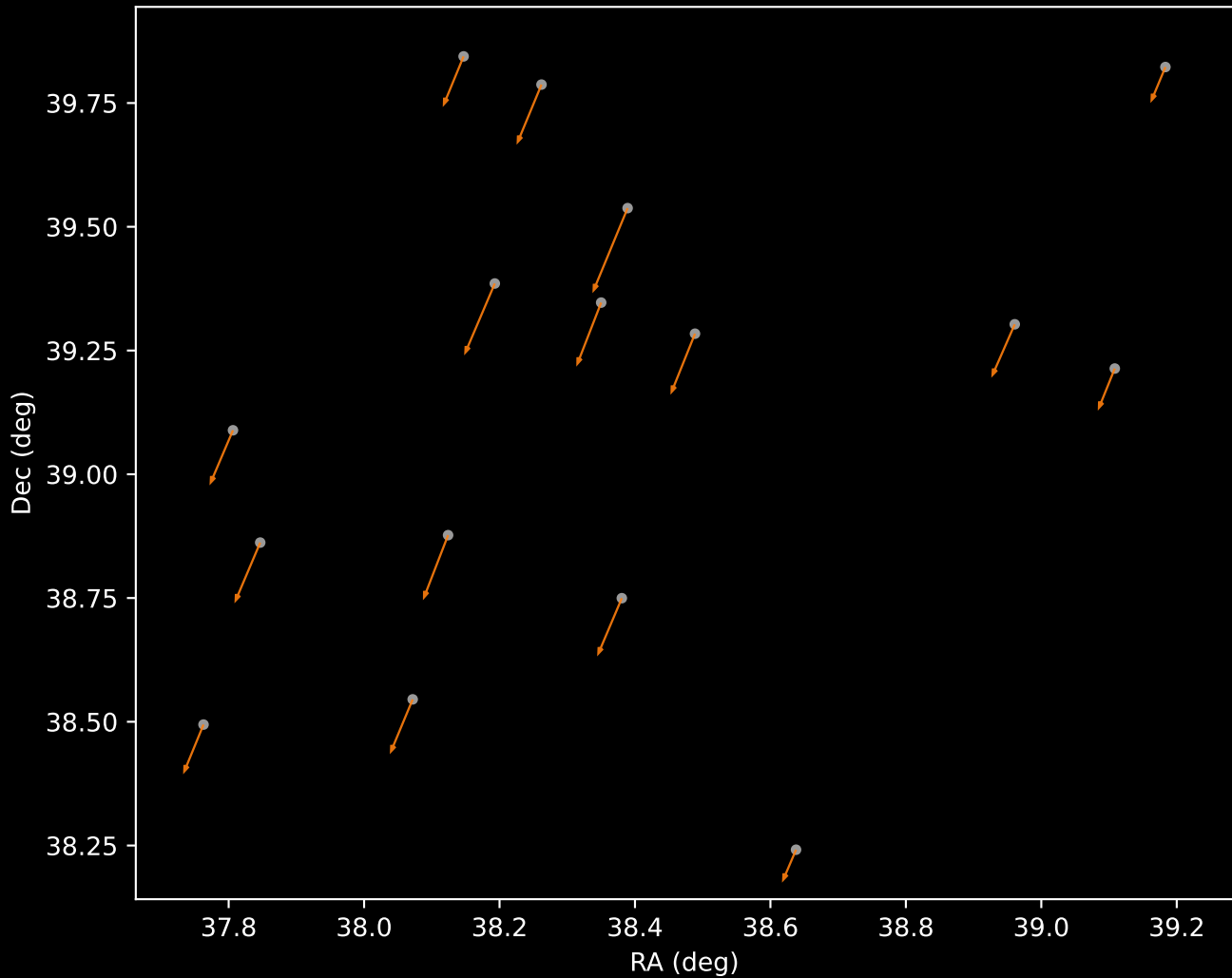
Gaia DR3 Cluster 22 Proper Motion Vectors (n=16)
