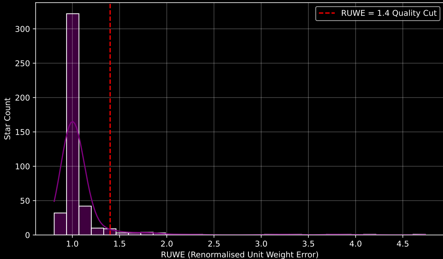
Gaia Cluster: [ASCC_108] RUWE Distribution (n= 438)
