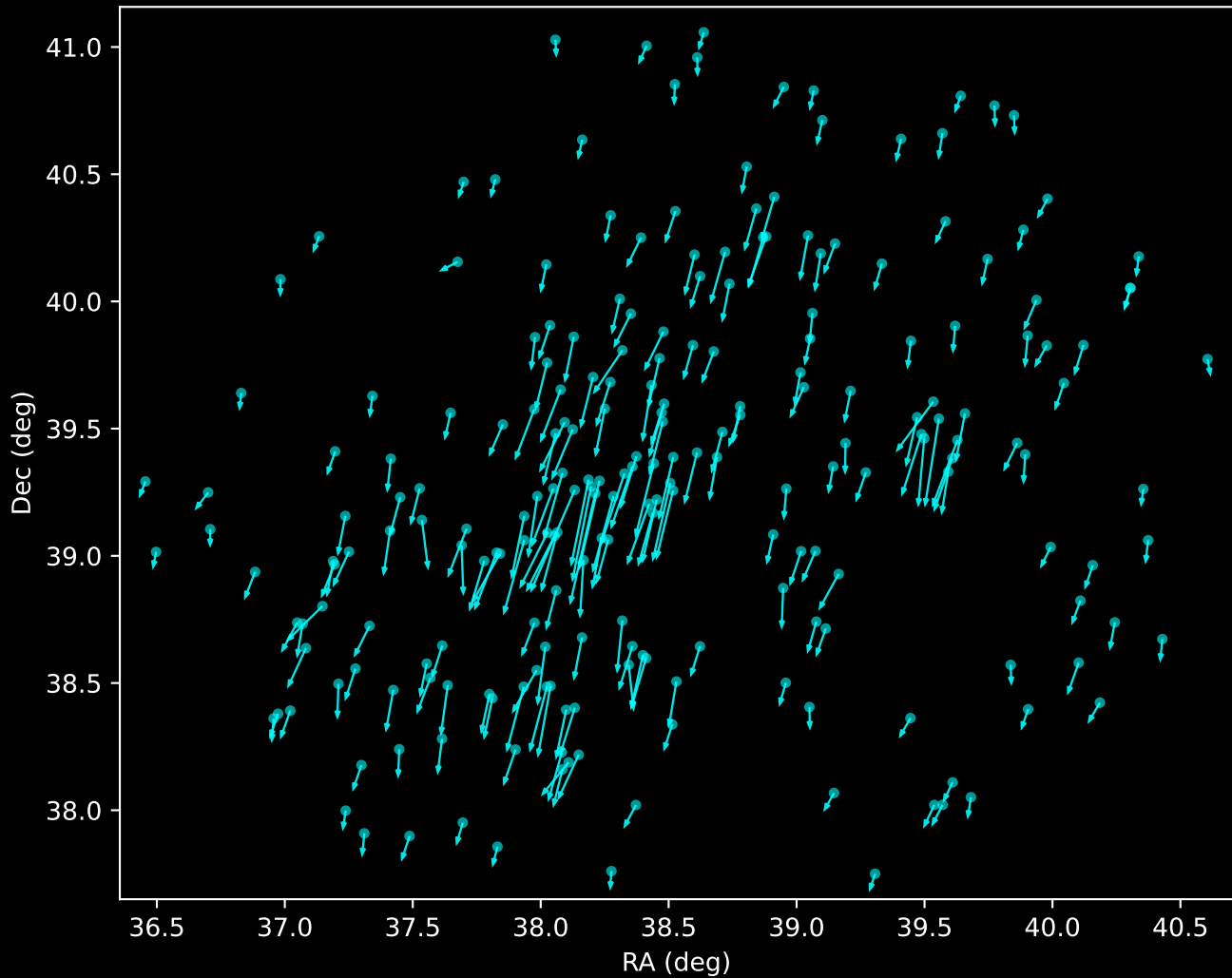
Gaia DR3 Noise Stream Proper Motion Vectors (n=227)
