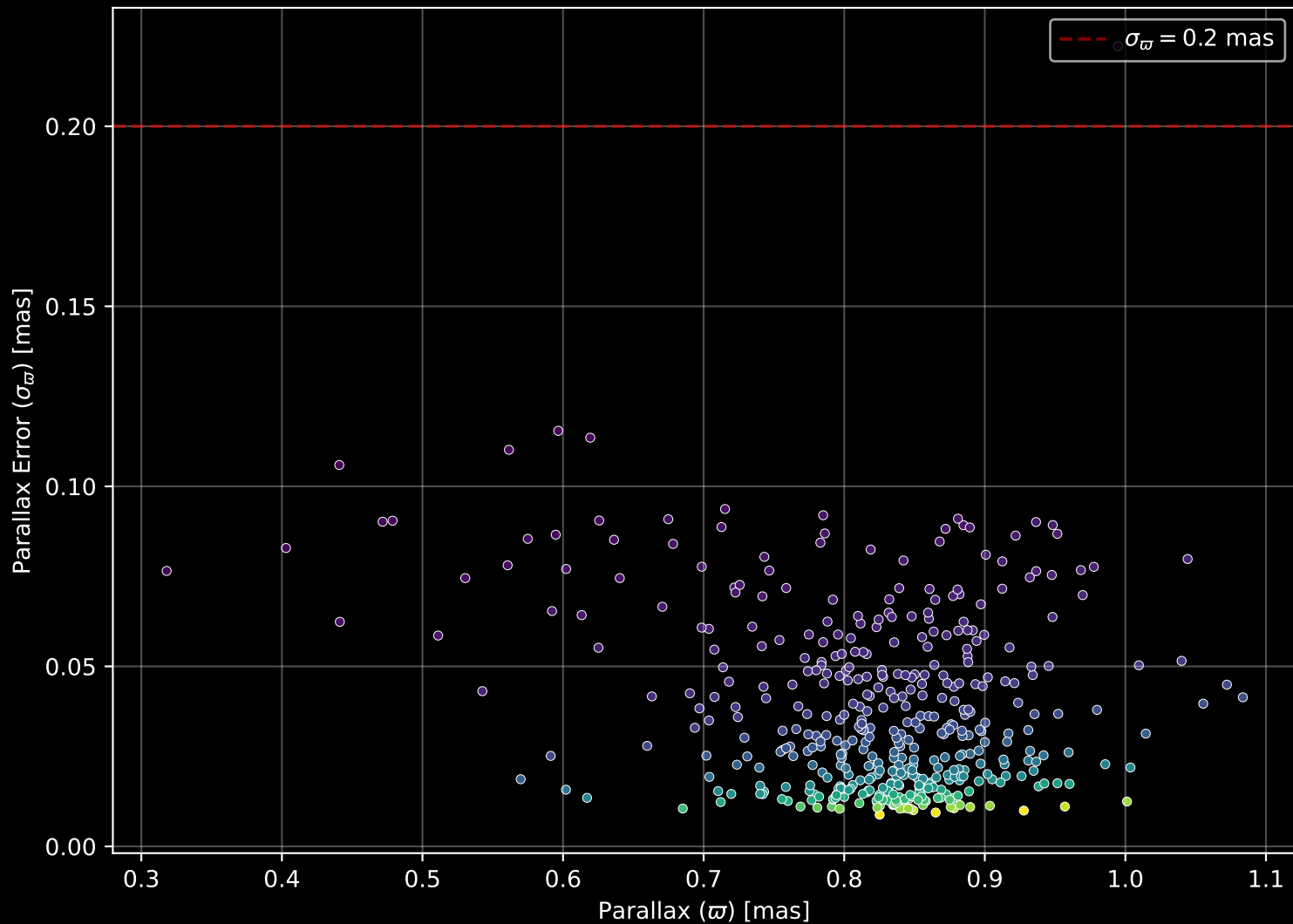
Gaia Cluster: [ASCC_108] Parallax Quality (n= 439)
