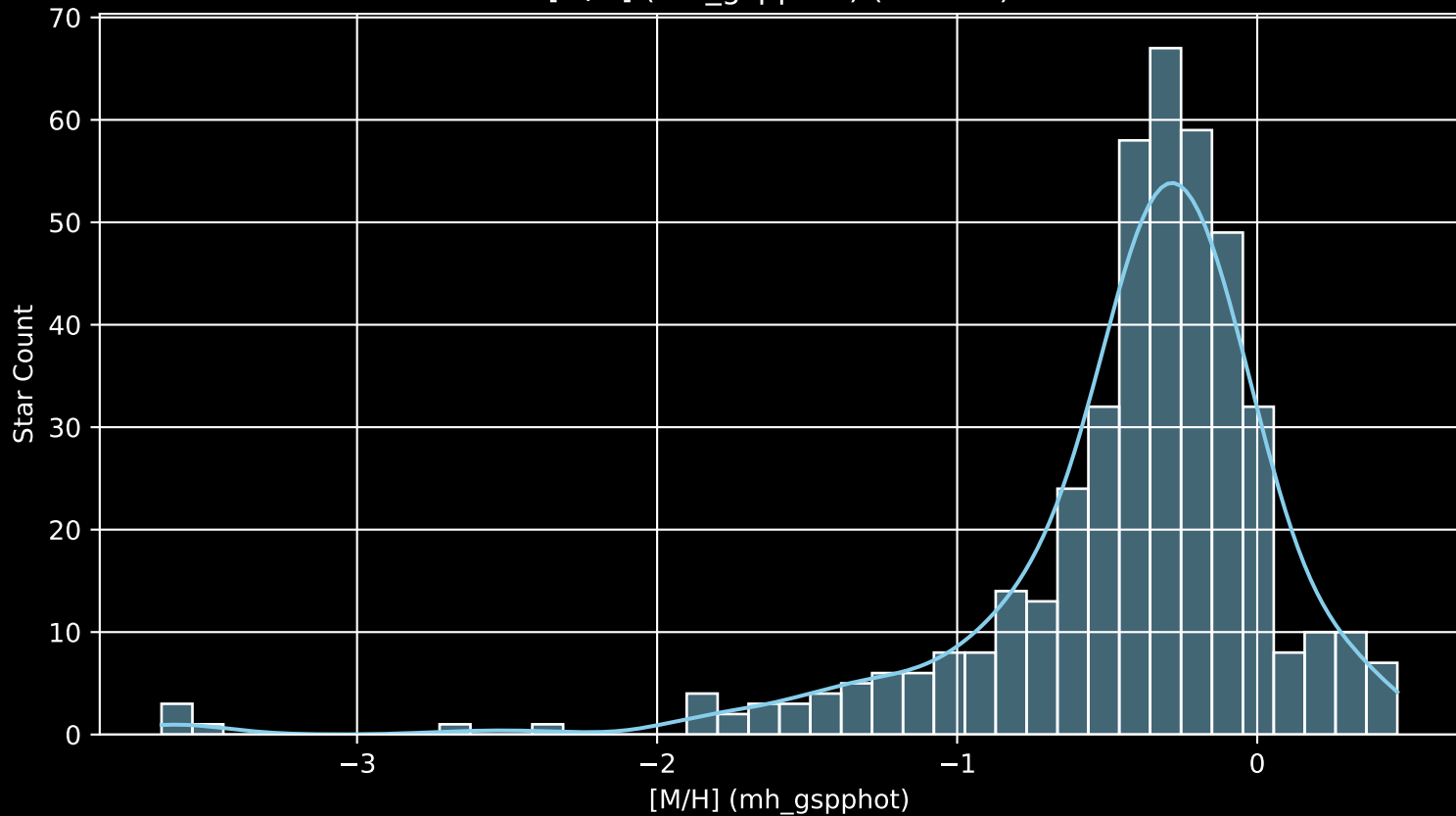
Gaia Cluster: [ASCC_108 [M/H] (mh_gspphot) (n= 438)
