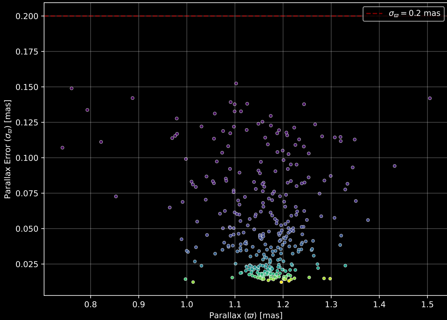
Gaia Cluster: [ASCC_11] Parallax Quality (n= 339)
