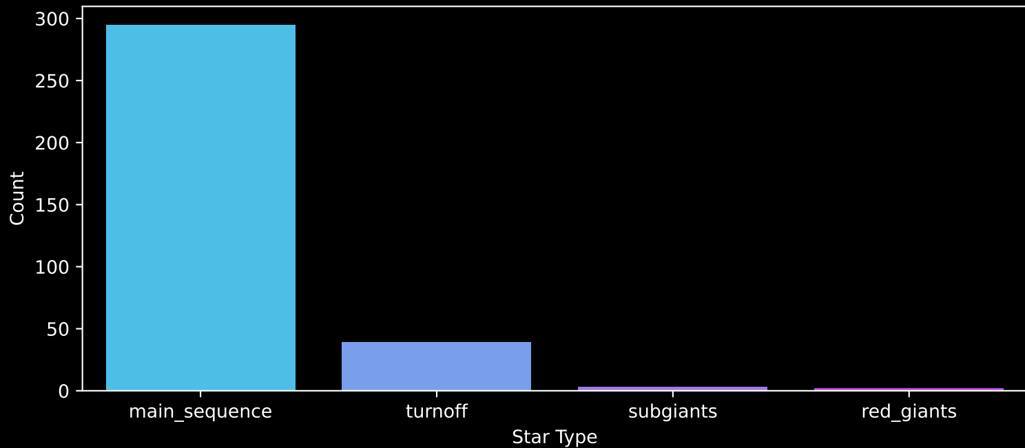
Gaia Cluster: [ASCC_11] Count plot of Star Type
