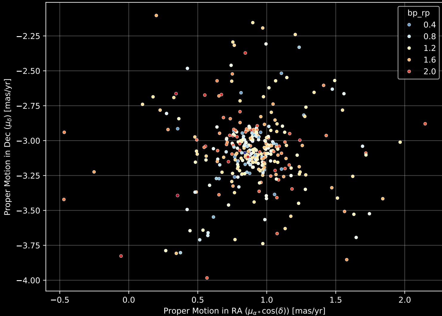
Gaia Cluster: [ASCC_11] Proper Motion Diagram (n= 339)
