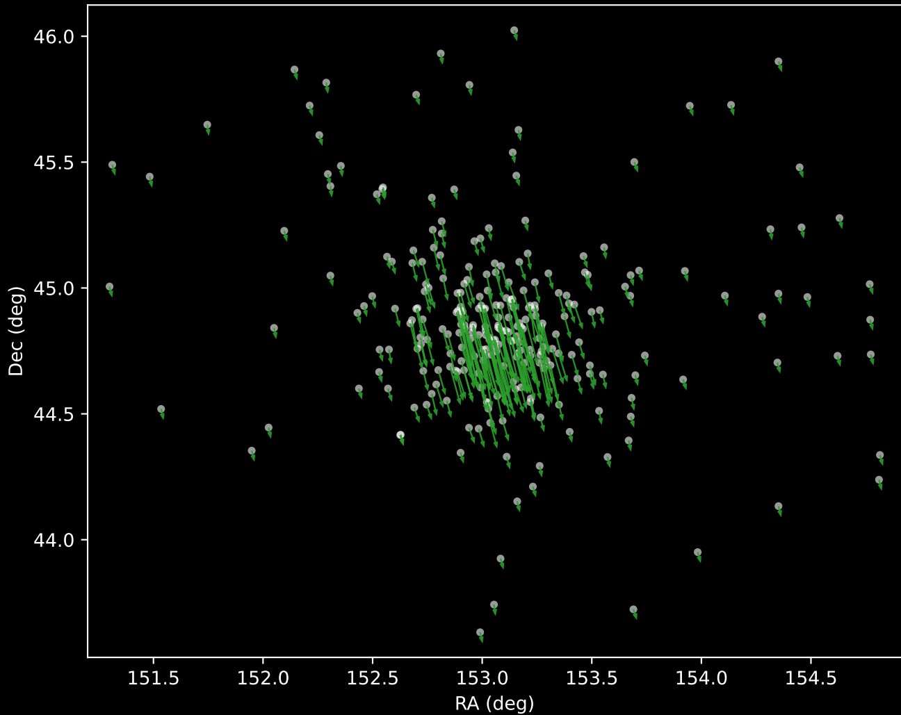
Gaia DR3 Cluster 4 Proper Motion Vectors (n=262)
