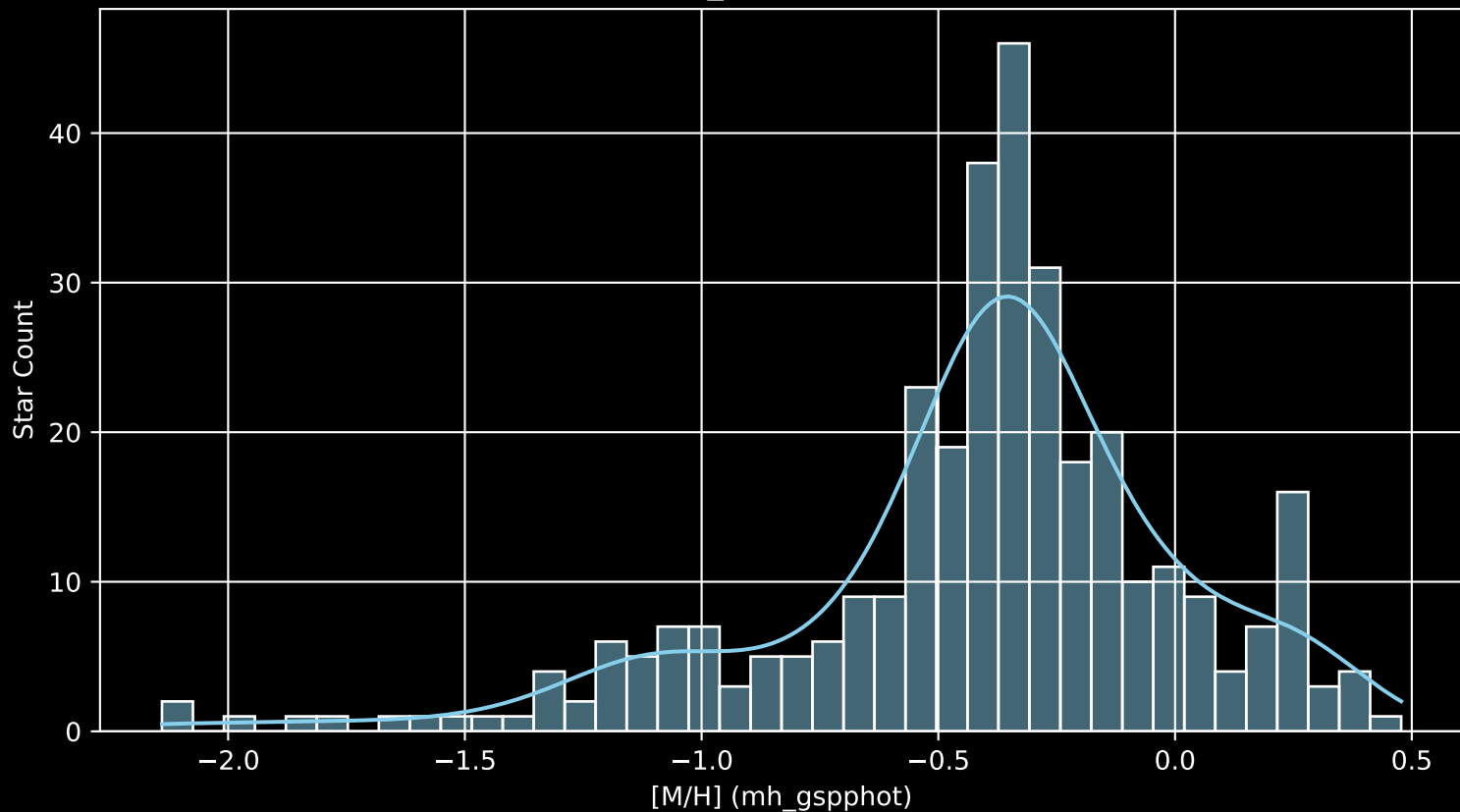
Gaia Cluster: [ASCC_11 [M/H] (mh_gspphot) (n= 338)
