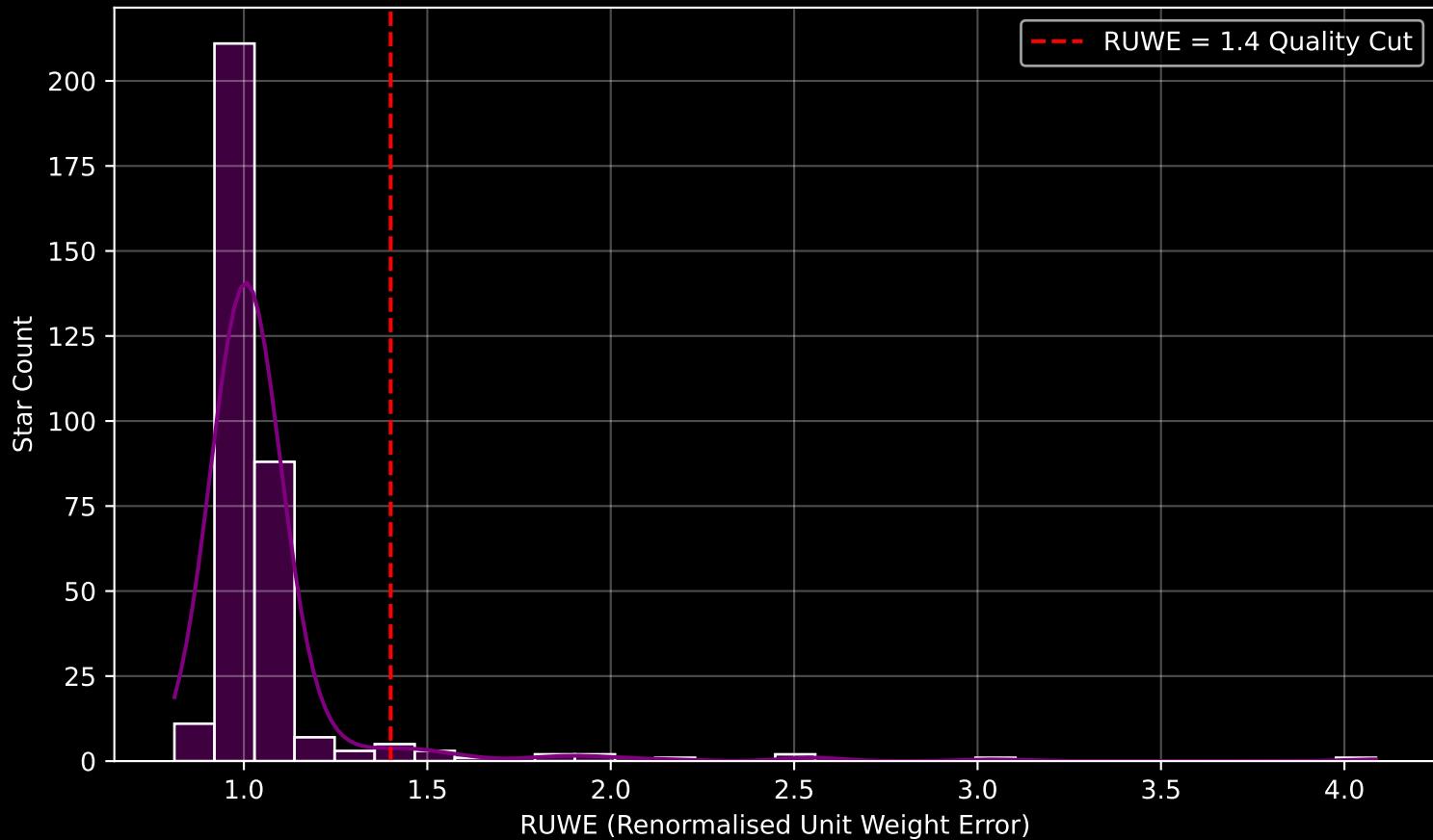
Gaia Cluster: [ASCC_11] RUWE Distribution (n= 338)
