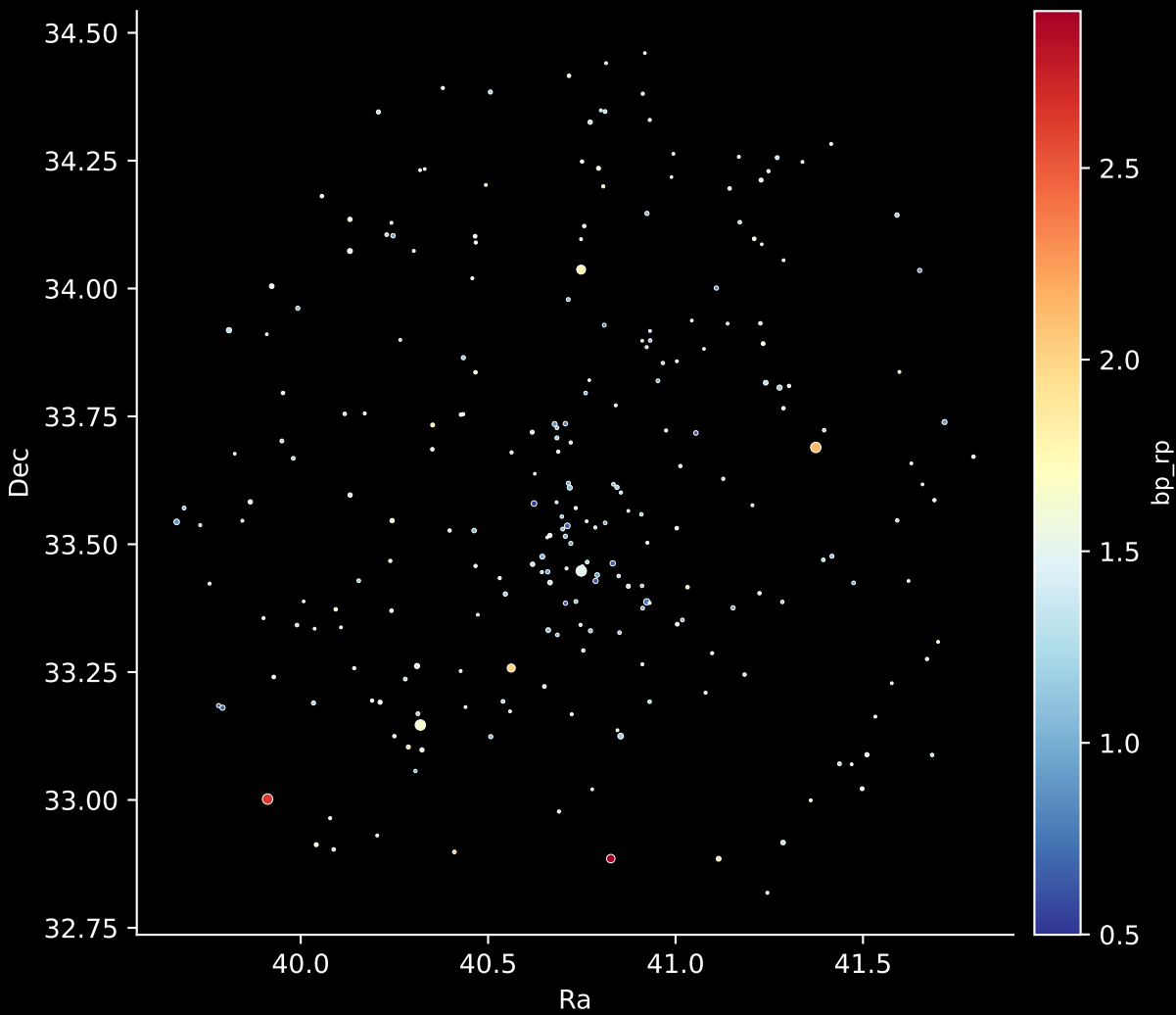
Gaia Cluster: [ASCC_110] Stars: 241
