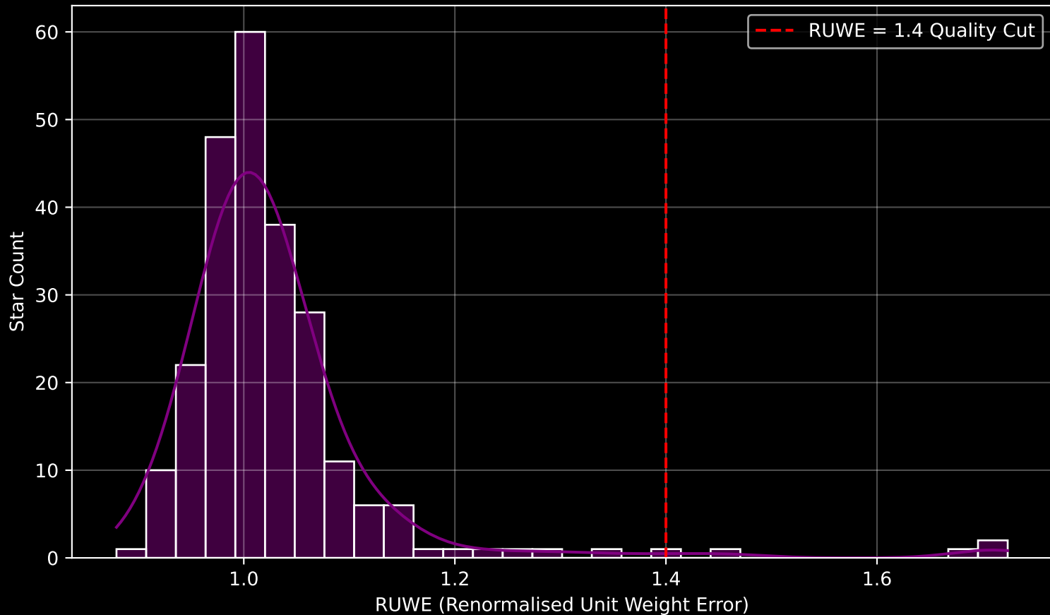
Gaia Cluster: [ASCC_110] RUWE Distribution (n= 241)
