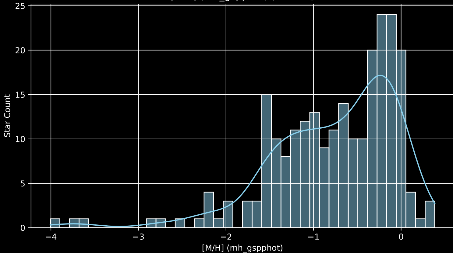
Gaia Cluster: [ASCC_110 [M/H] (mh_gspphot) (n= 240)
