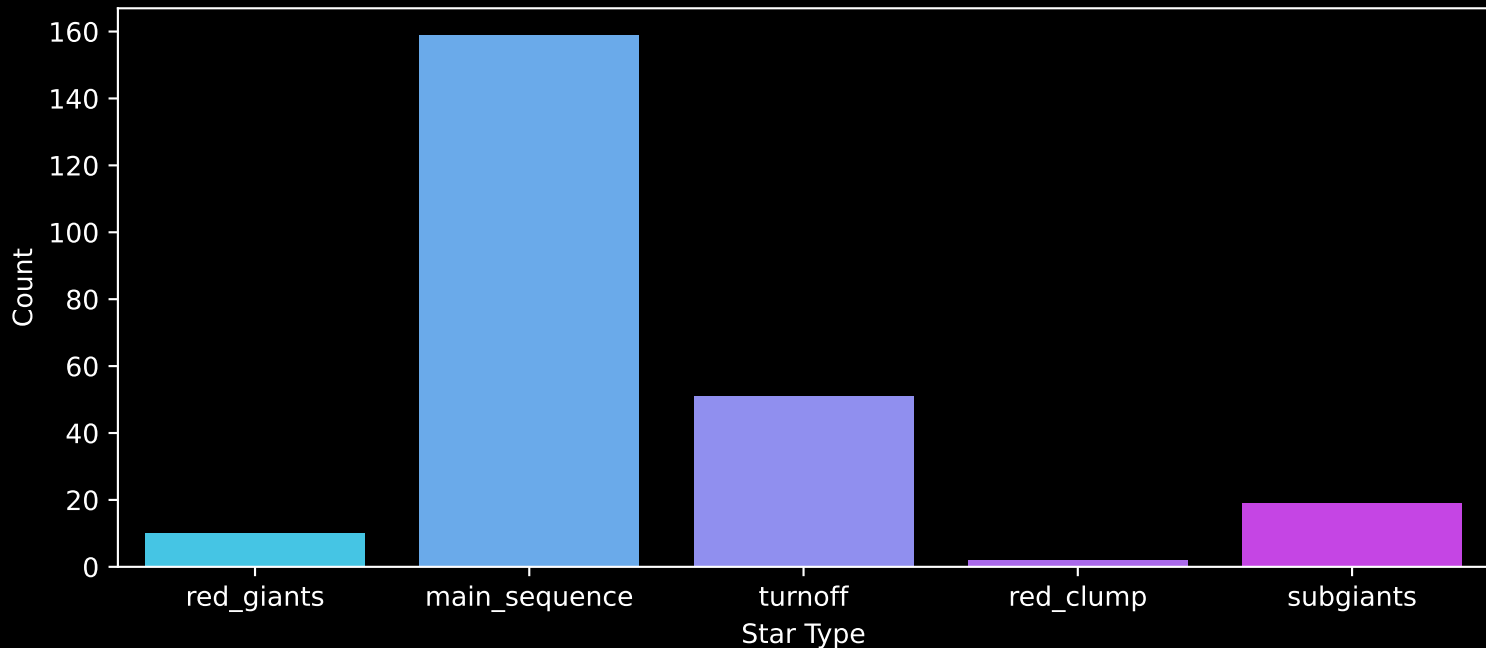
Gaia Cluster: [ASCC_110] Count plot of Star Type
