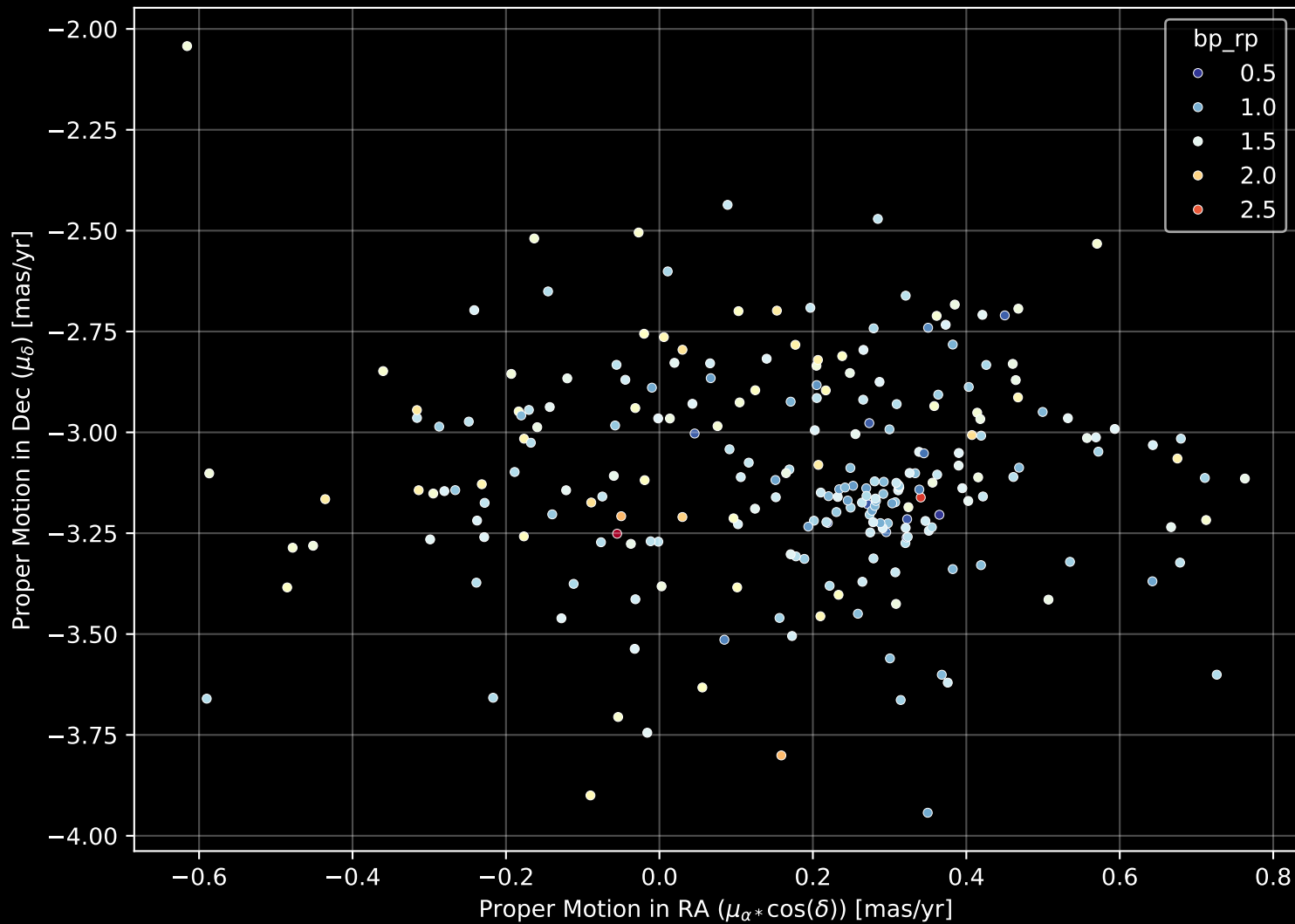
Gaia Cluster: [ASCC_110] Proper Motion Diagram (n= 241)
