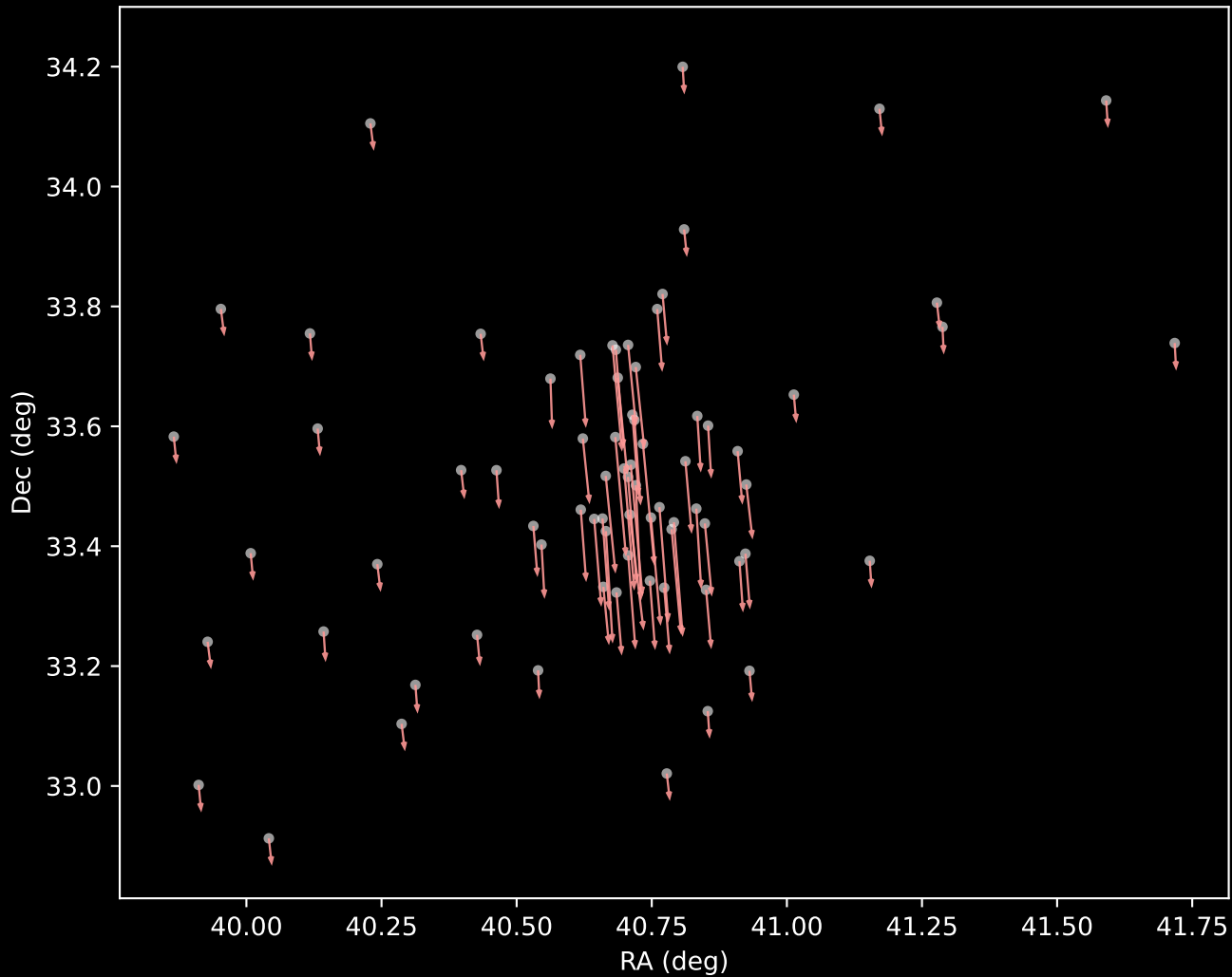
Gaia DR3 Cluster 7 Proper Motion Vectors (n=75)
