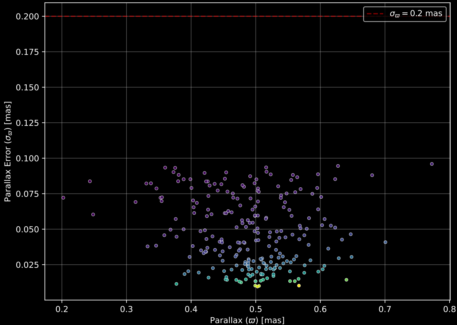
Gaia Cluster: [ASCC_110] Parallax Quality (n= 241)
