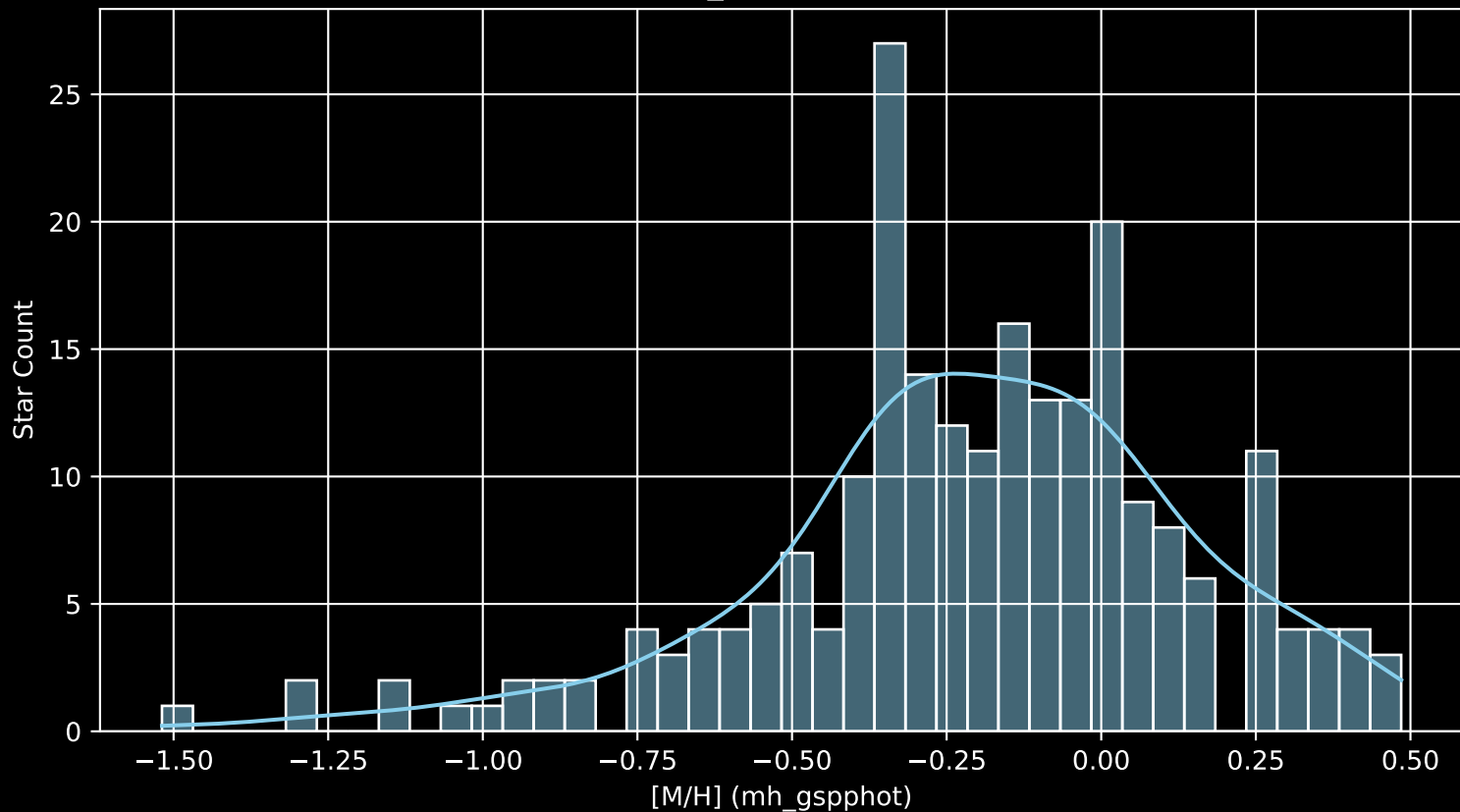
Gaia Cluster: [ASCC_113 [M/H] (mh_gspphot) (n= 229)
