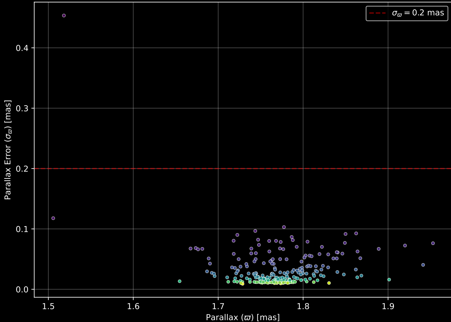
Gaia Cluster: [ASCC_113] Parallax Quality (n= 229)
