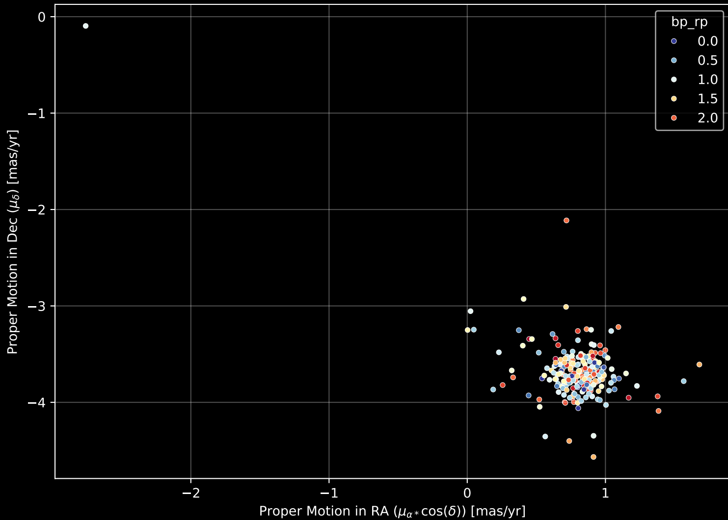
Gaia Cluster: [ASCC_113] Proper Motion Diagram (n= 229)
