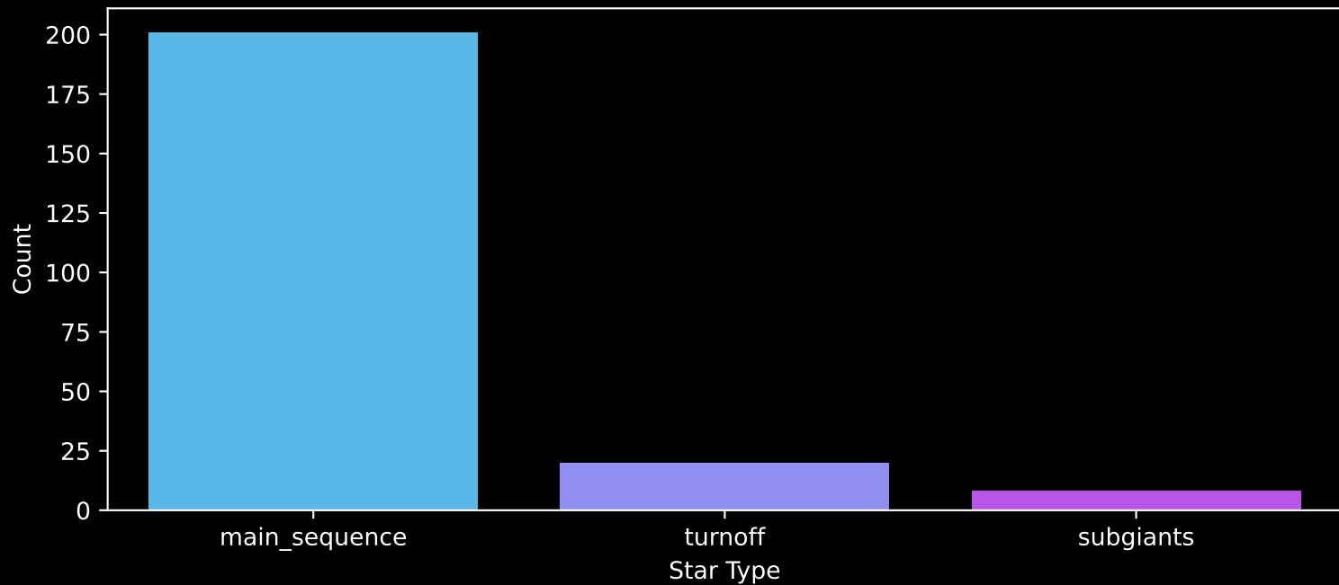
Gaia Cluster: [ASCC_113] Count plot of Star Type
