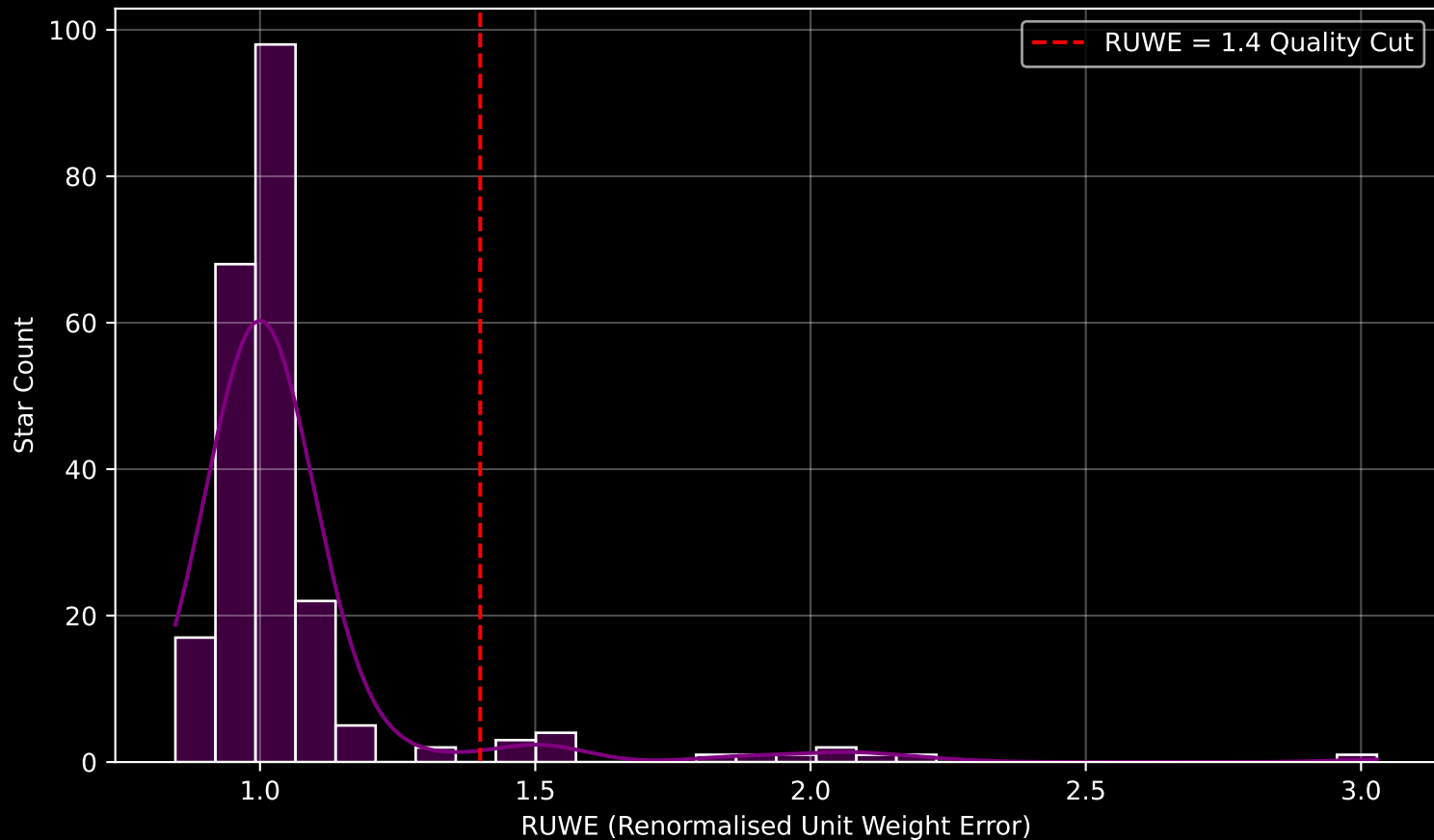
Gaia Cluster: [ASCC_113] RUWE Distribution (n= 227)
