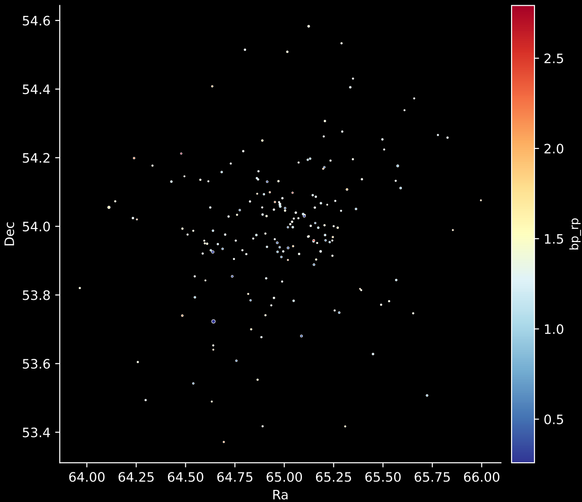
Gaia Cluster: [ASCC_114] Stars: 179
