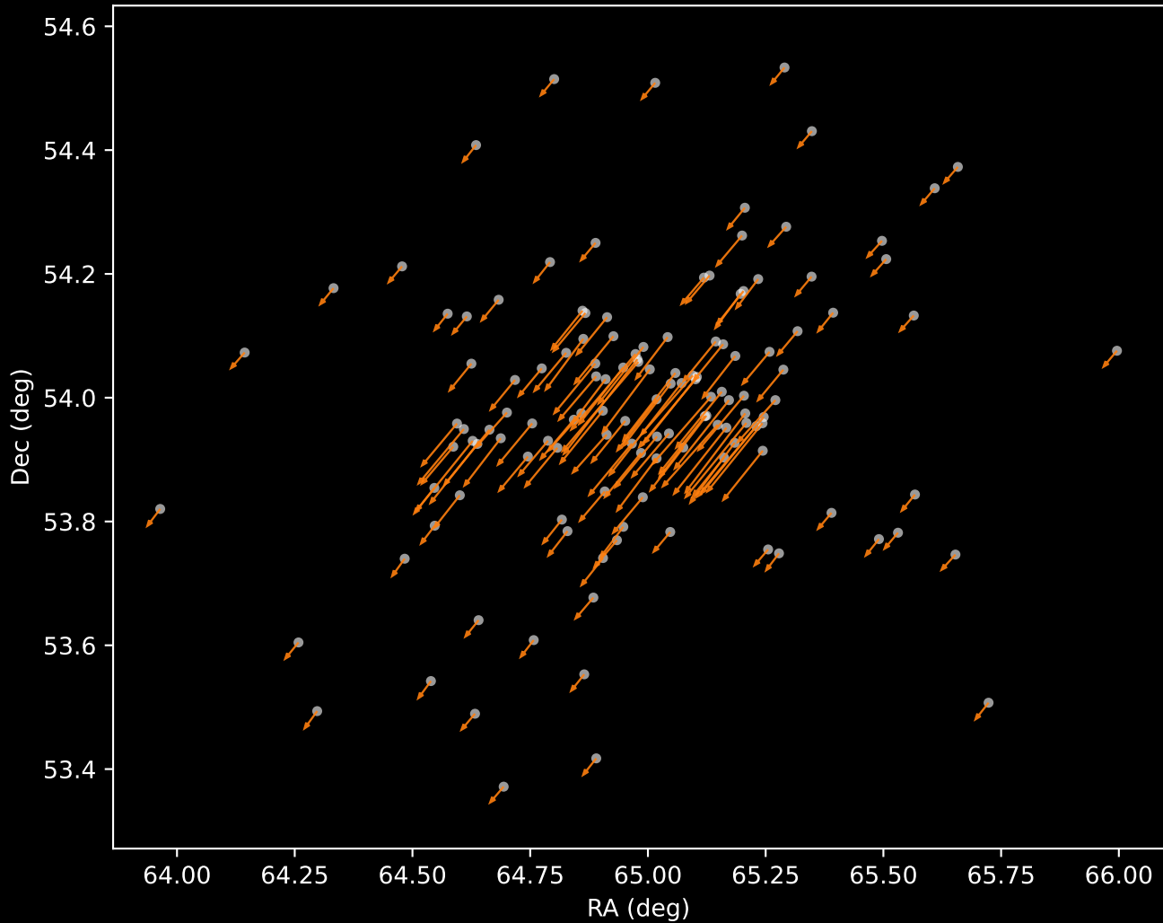
Gaia DR3 Cluster 2 Proper Motion Vectors (n=132)
