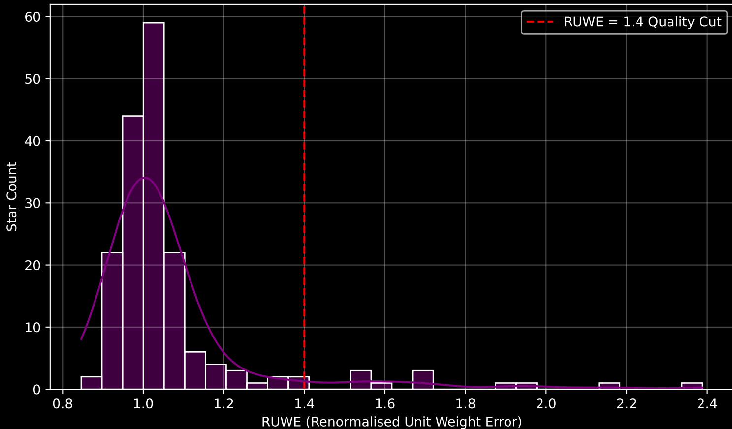
Gaia Cluster: [ASCC_114] RUWE Distribution (n= 178)
