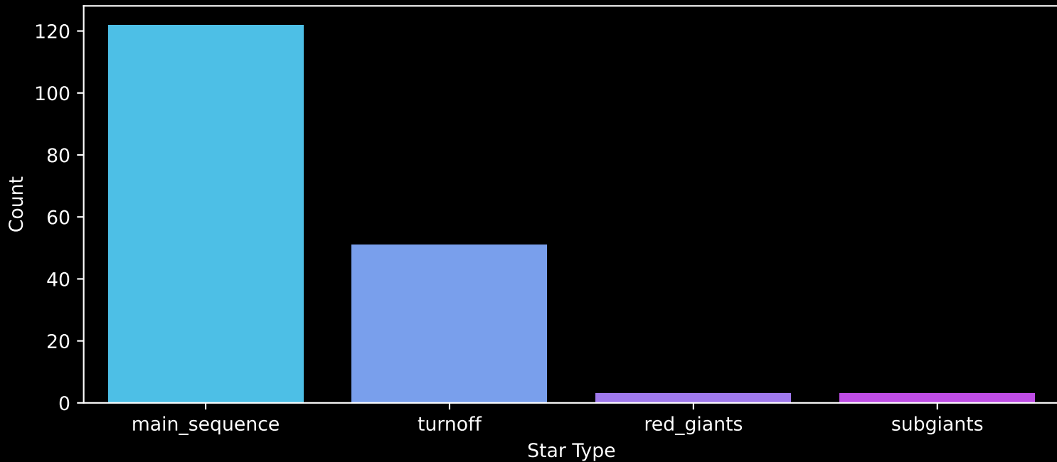
Gaia Cluster: [ASCC_114] Count plot of Star Type
