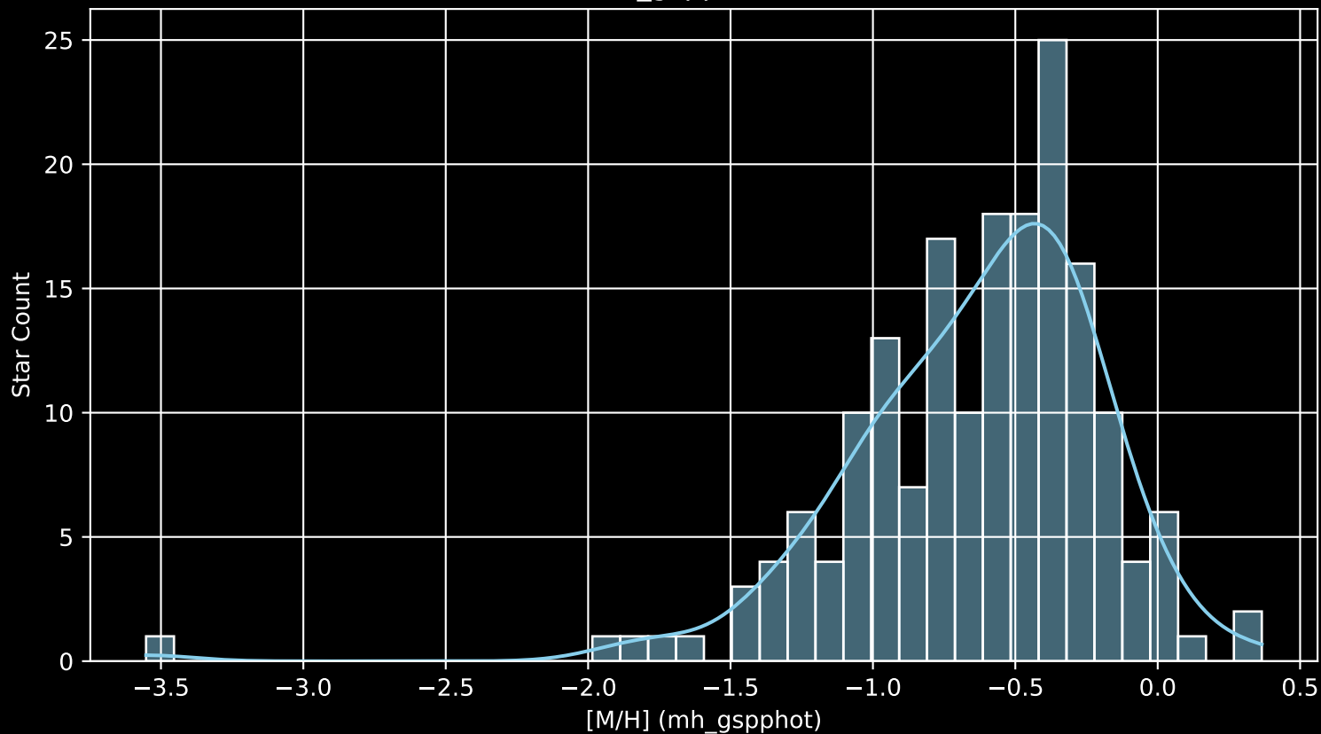
Gaia Cluster: [ASCC_114 [M/H] (mh_gspphot) (n= 179)
