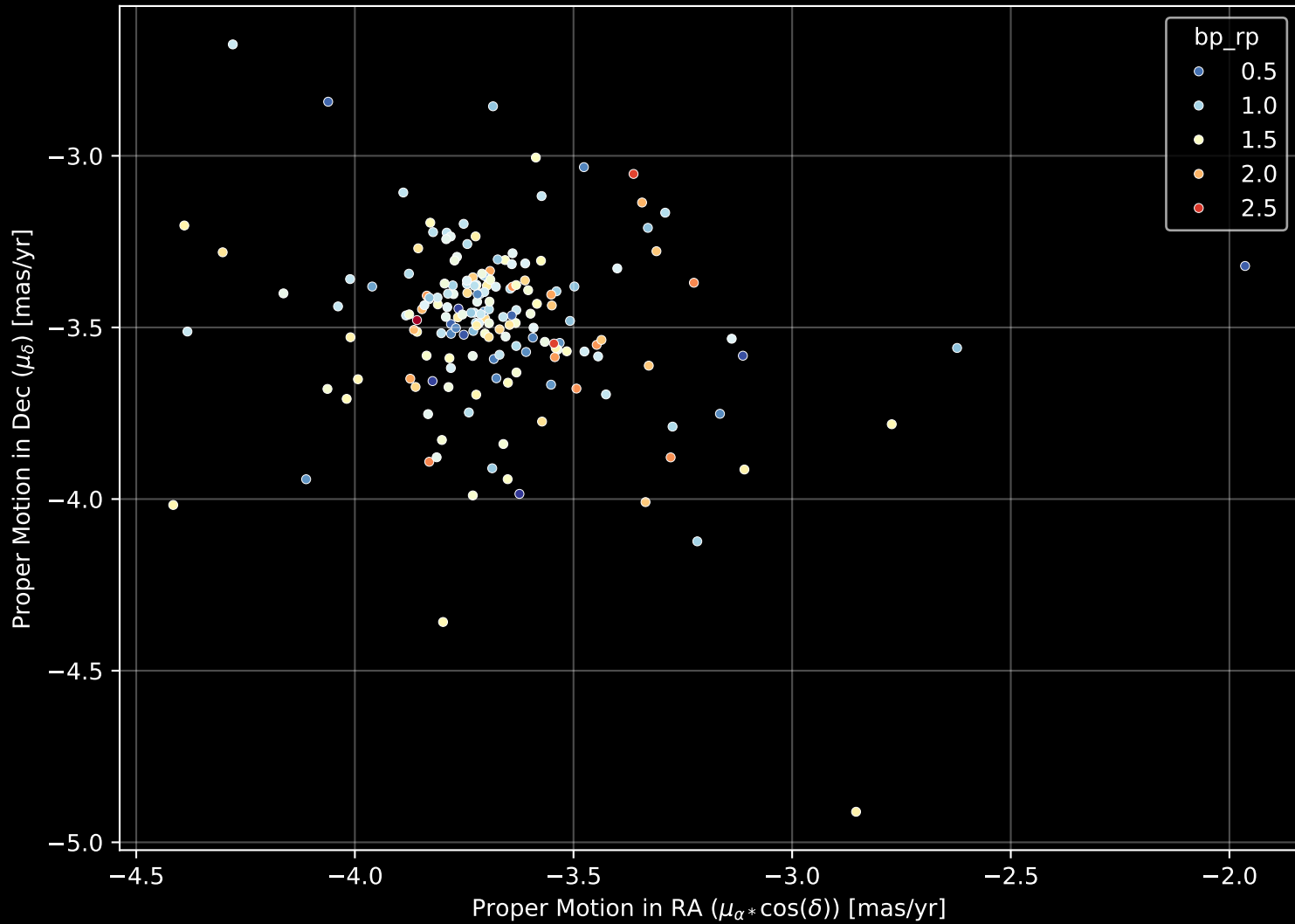
Gaia Cluster: [ASCC_114] Proper Motion Diagram (n= 179)
