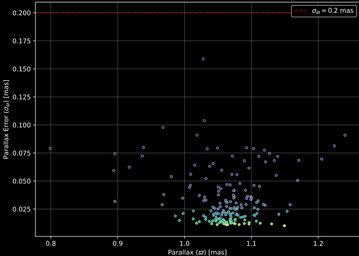
Gaia Cluster: [ASCC_114] Parallax Quality (n= 179)
