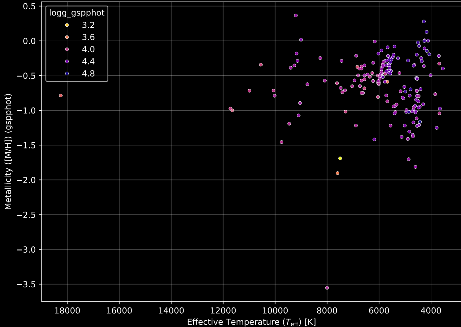
Gaia Cluster: [ASCC_114] Stellar Population Parameters (n= 179)
