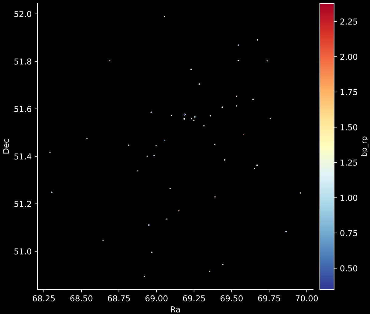
Gaia Cluster: [ASCC_115] Stars: 48
