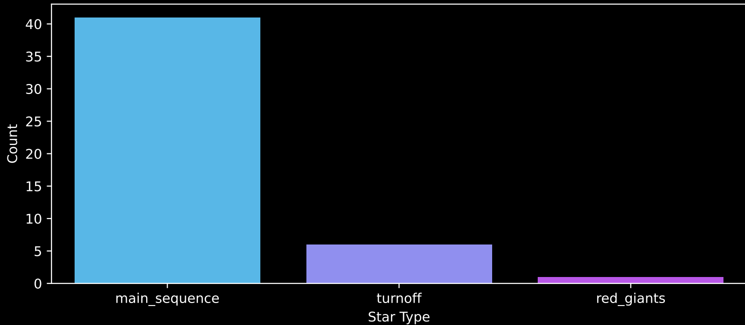
Gaia Cluster: [ASCC_115] Count plot of Star Type
