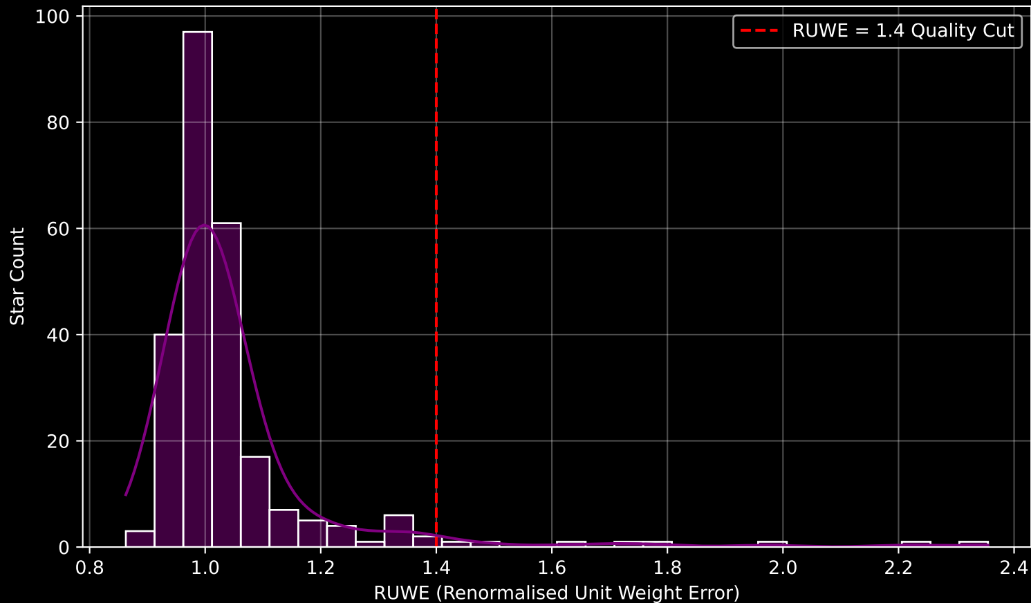
Gaia Cluster: [ASCC_12] RUWE Distribution (n= 251)
