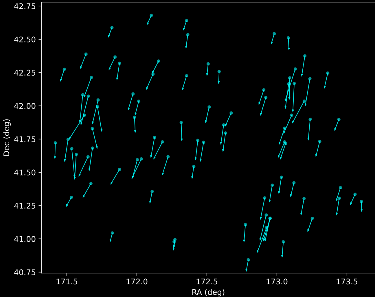
Gaia DR3 Noise Stream Proper Motion Vectors (n=85)
