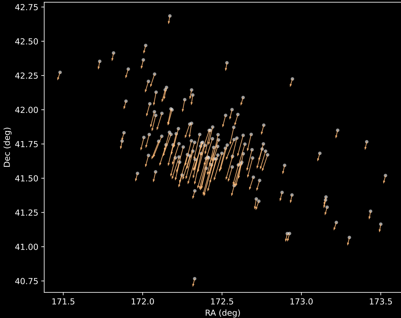
Gaia DR3 Cluster 3 Proper Motion Vectors (n=124)
