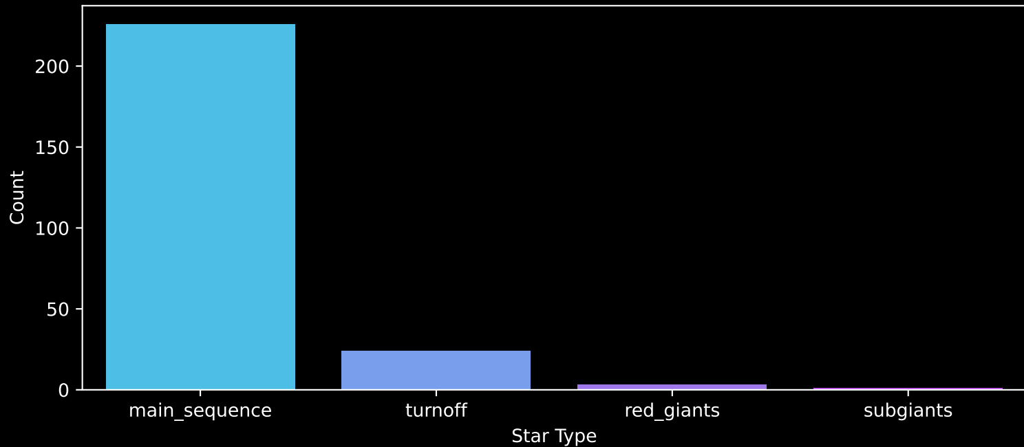
Gaia Cluster: [ASCC_12] Count plot of Star Type
