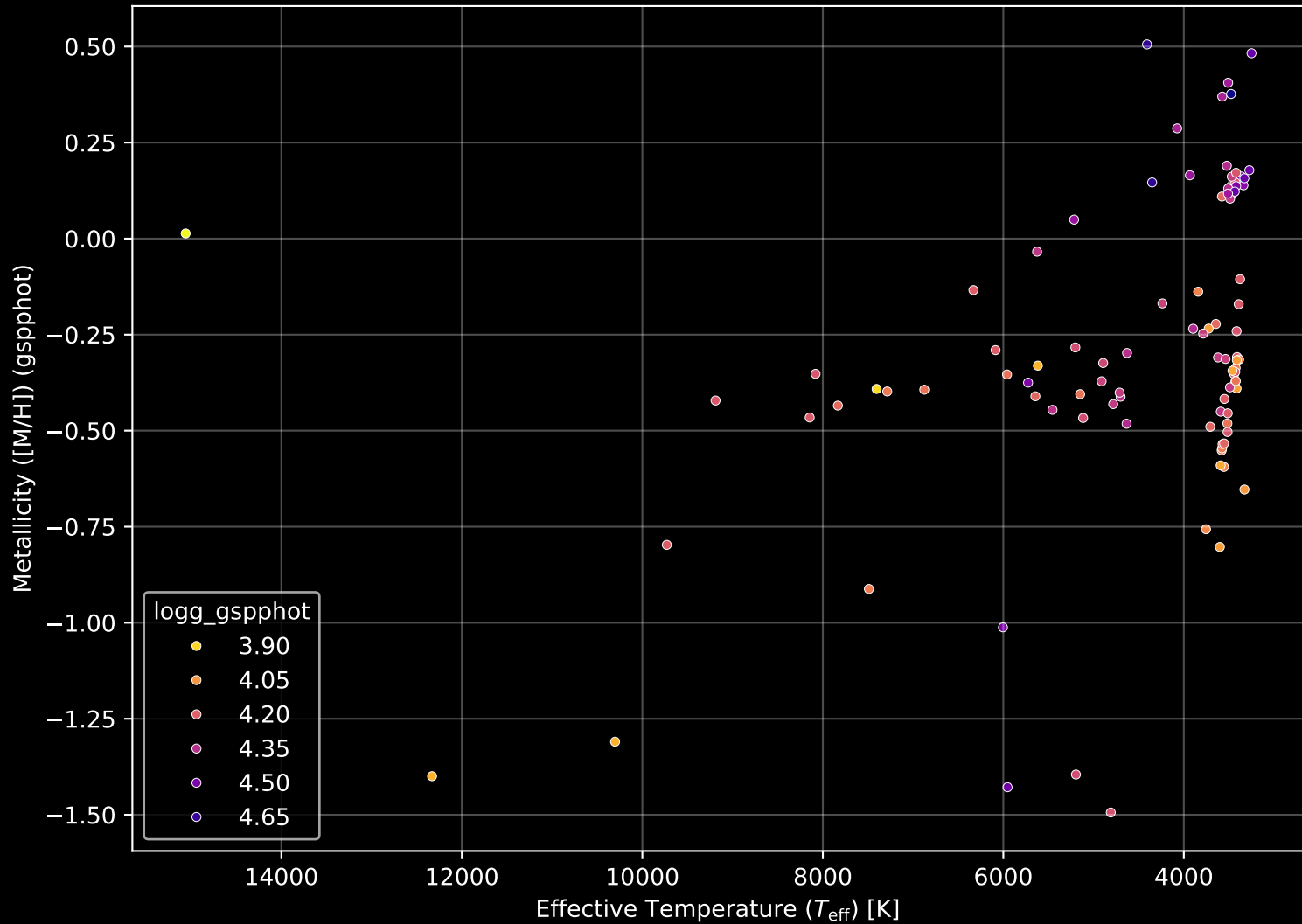
Gaia Cluster: [ASCC_127] Stellar Population Parameters (n= 98)
