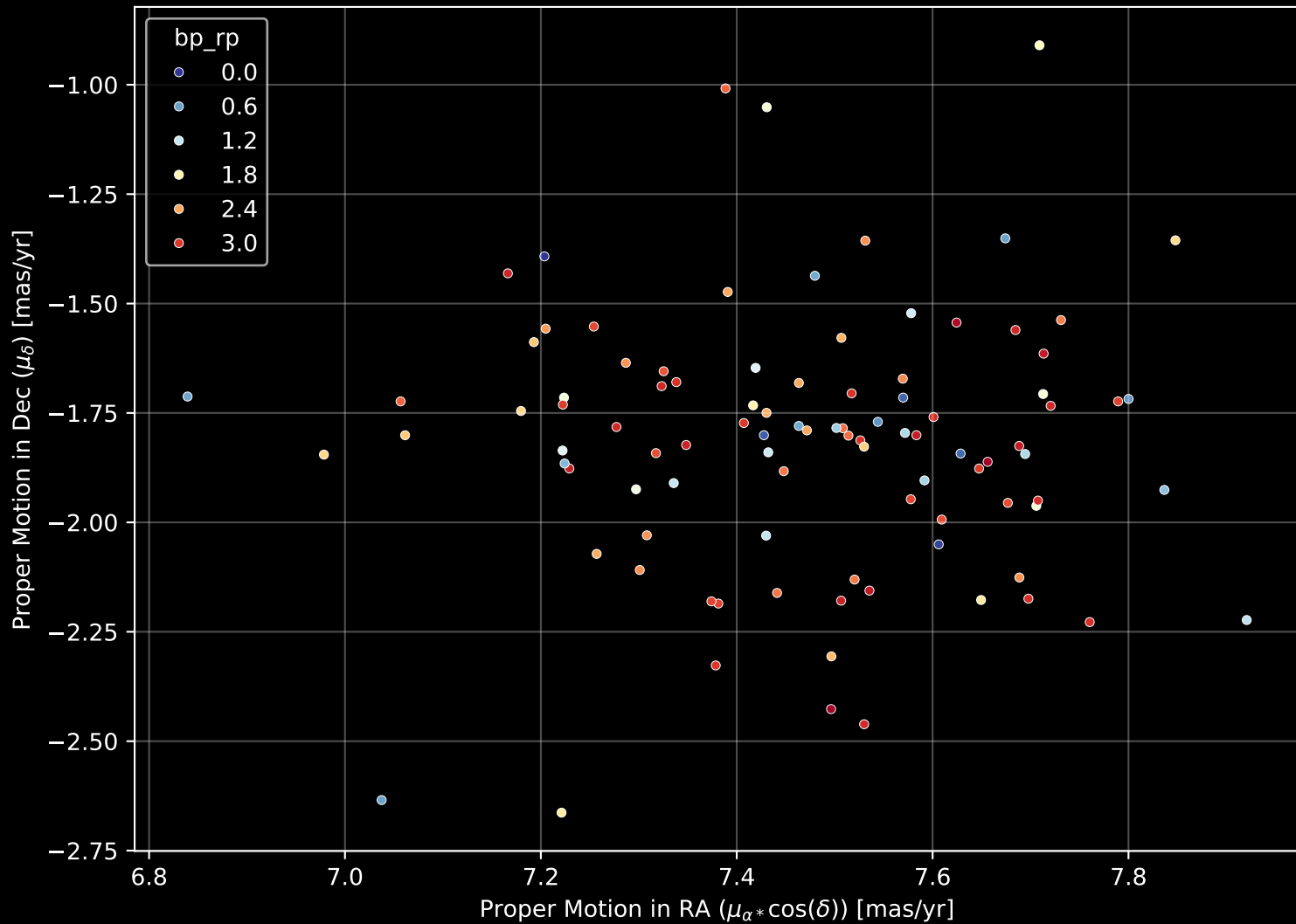
Gaia Cluster: [ASCC_127] Proper Motion Diagram (n= 98)
