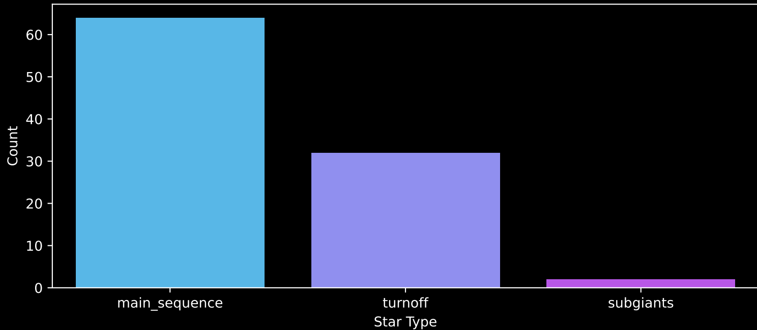
Gaia Cluster: [ASCC_127] Count plot of Star Type
