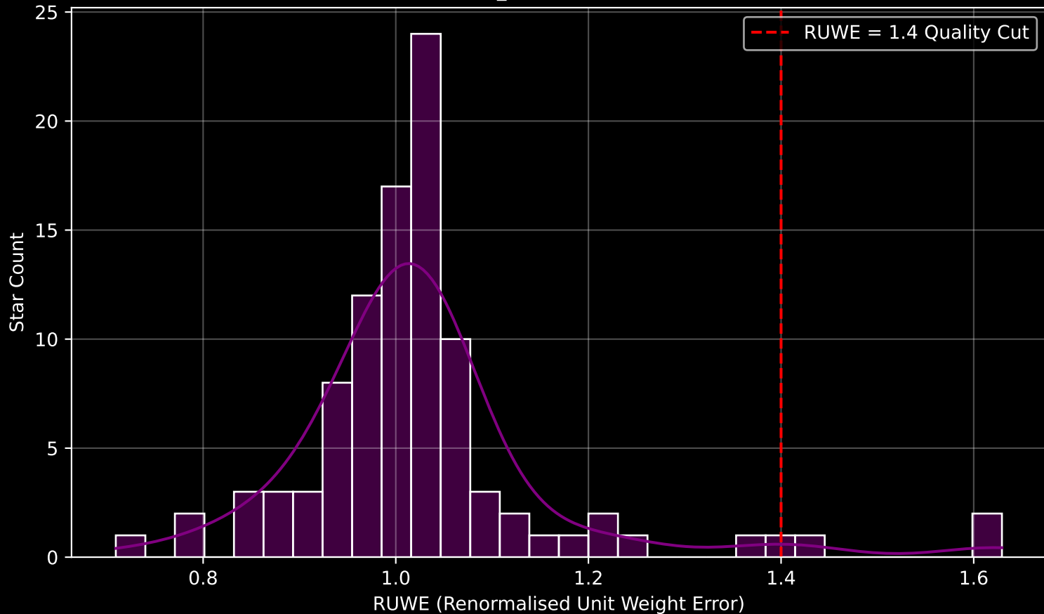
Gaia Cluster: [ASCC_127] RUWE Distribution (n= 98)
