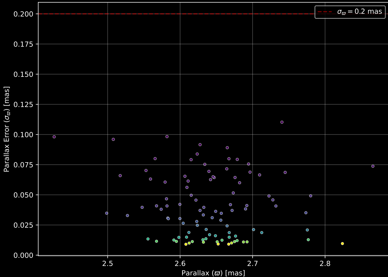
Gaia Cluster: [ASCC_127] Parallax Quality (n= 98)
