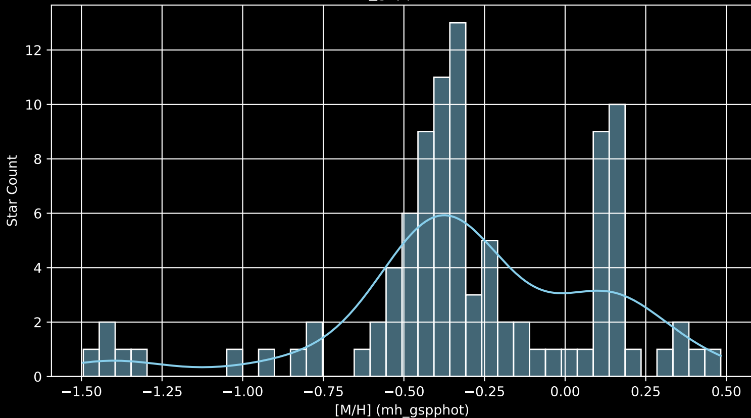
Gaia Cluster: [ASCC_127 [M/H] (mh_gspphot) (n= 97)
