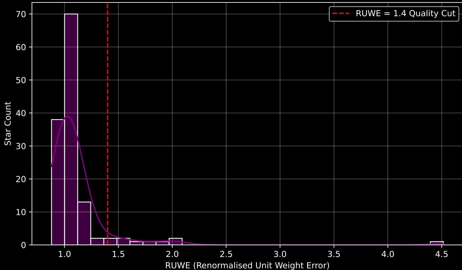
Gaia Cluster: [ASCC_23] RUWE Distribution (n= 133)
