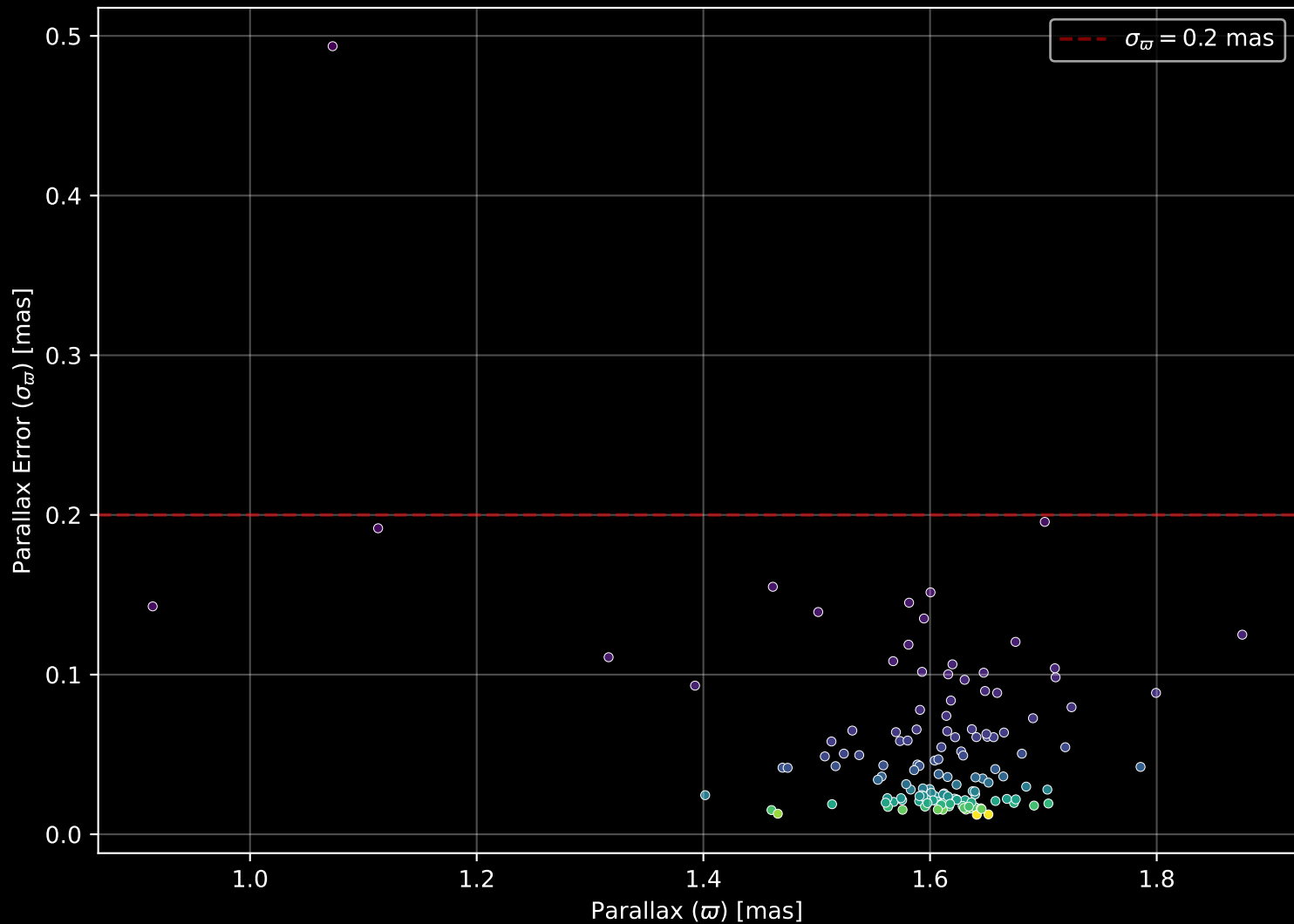
Gaia Cluster: [ASCC_23] Parallax Quality (n= 136)
