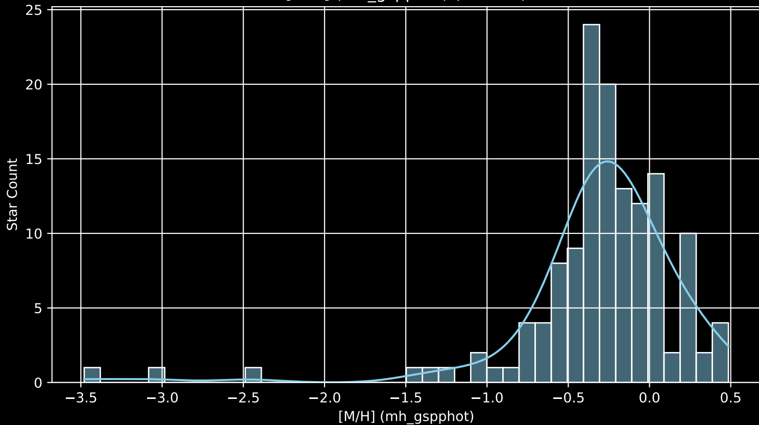
Gaia Cluster: [ASCC_23 [M/H] (mh_gspphot) (n= 136)
