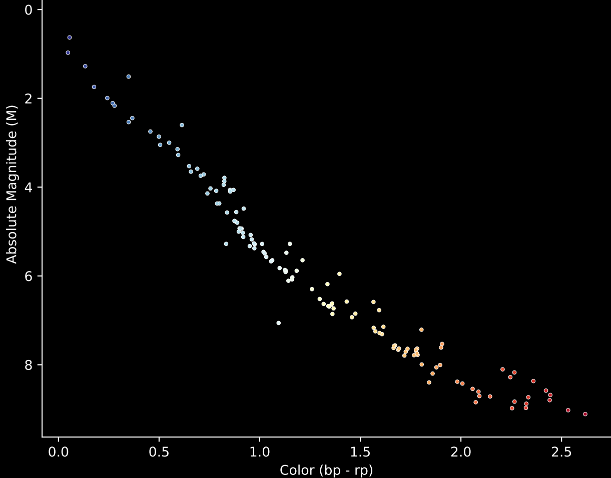
Gaia Cluster: [ASCC_23] Stars (n= 136) Hertzsprung-Russel Diagram
