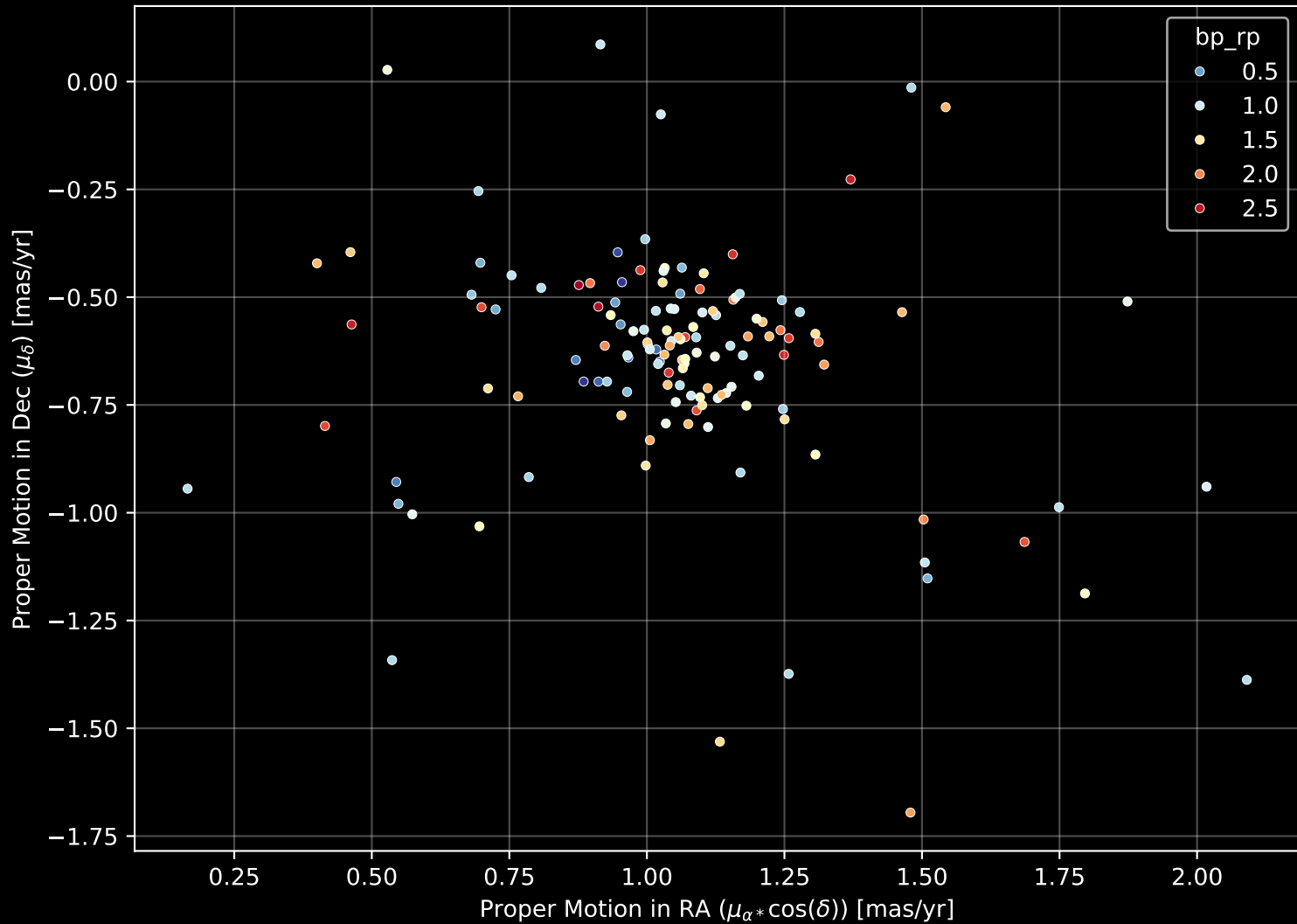
Gaia Cluster: [ASCC_23] Proper Motion Diagram (n= 136)
