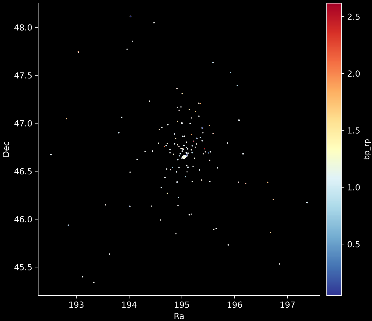
Gaia Cluster: [ASCC_23] Stars: 136
