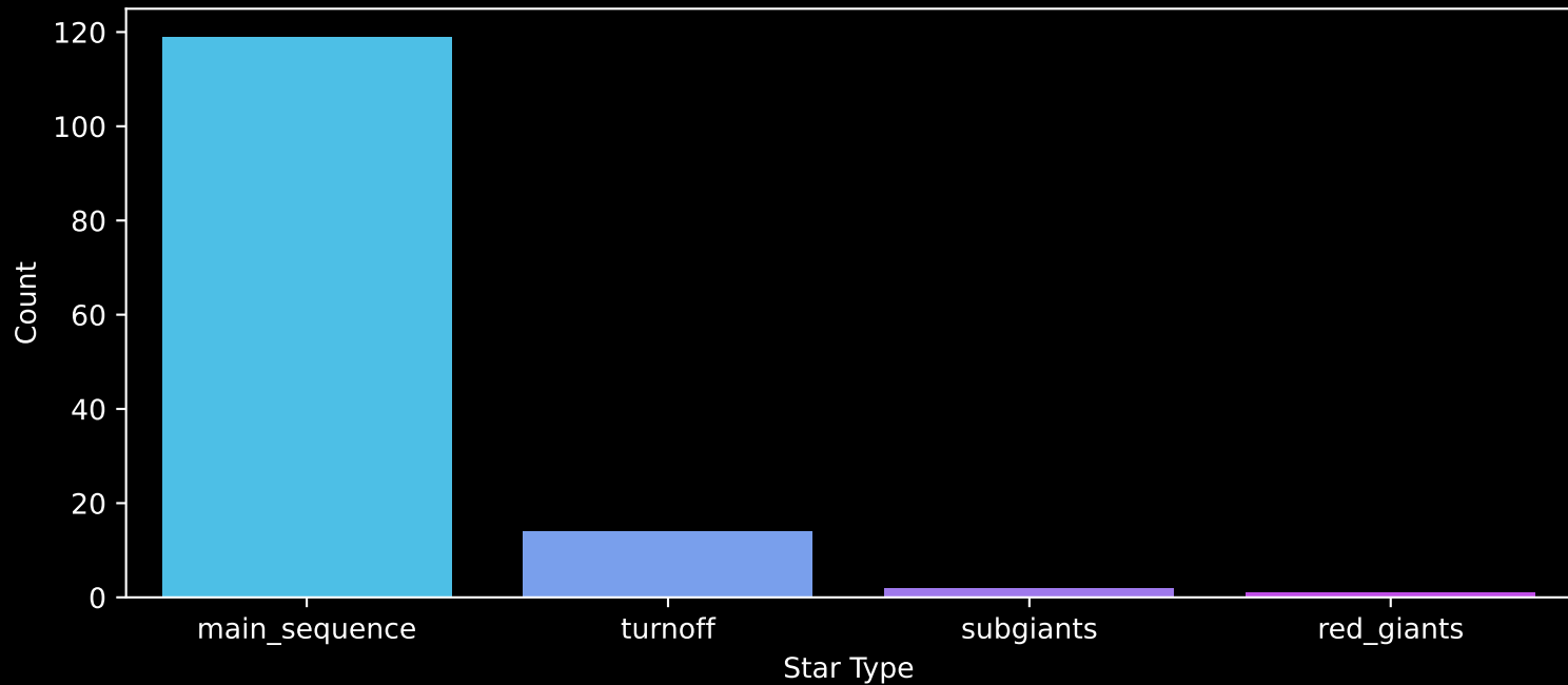
Gaia Cluster: [ASCC_23] Count plot of Star Type
