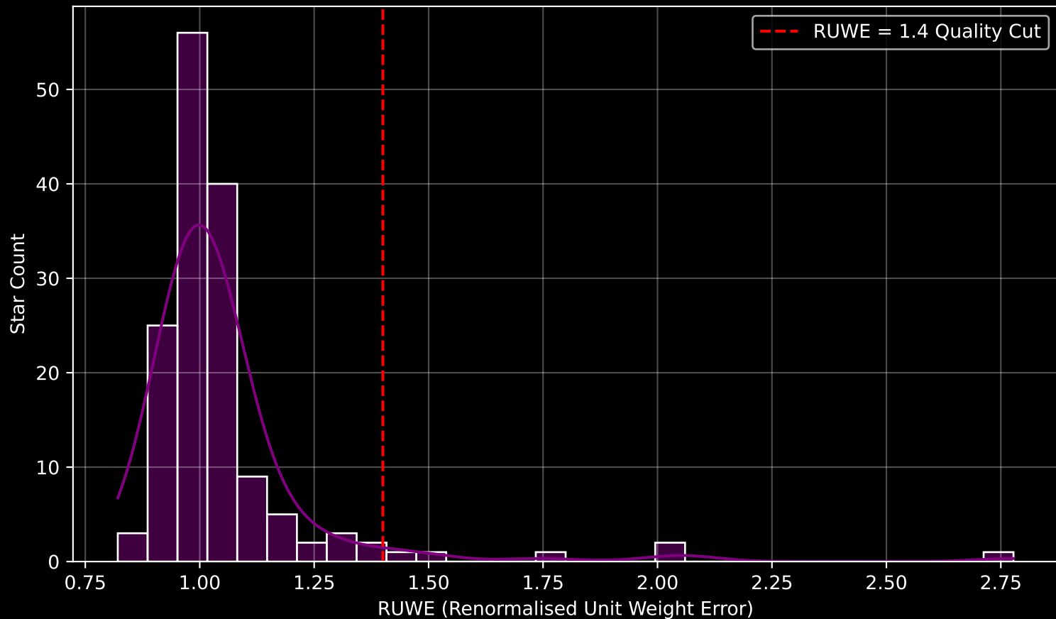
Gaia Cluster: [ASCC_30] RUWE Distribution (n= 151)
