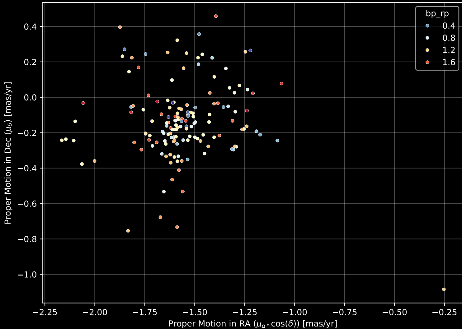
Gaia Cluster: [ASCC_30] Proper Motion Diagram (n= 151)
