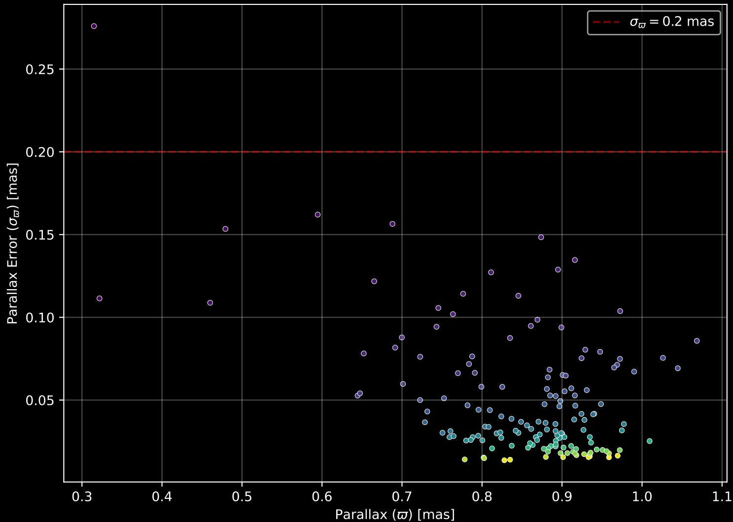
Gaia Cluster: [ASCC 30] Parallax Quality (n= 151)
