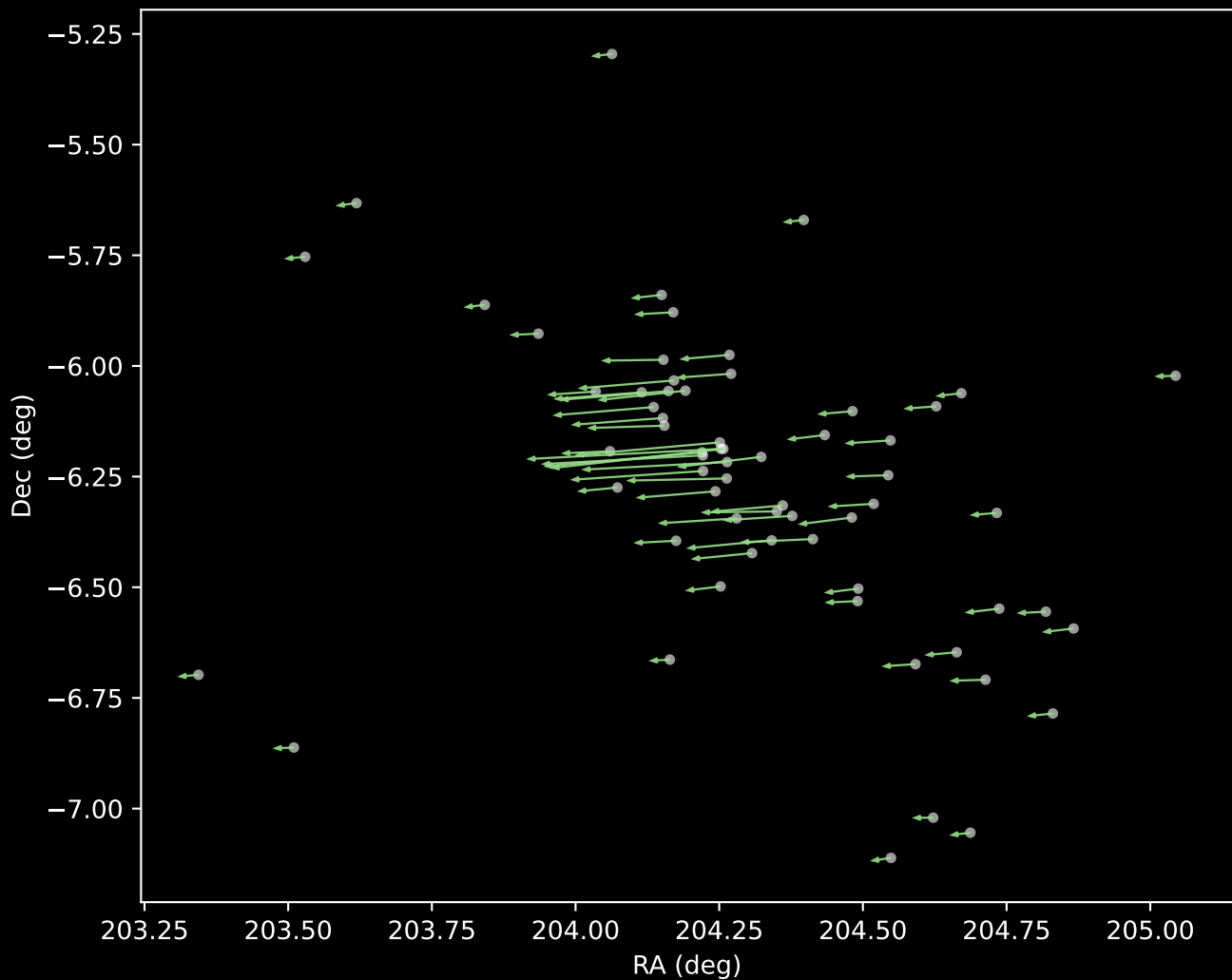
Gaia DR3 Cluster 5 Proper Motion Vectors (n=65)
