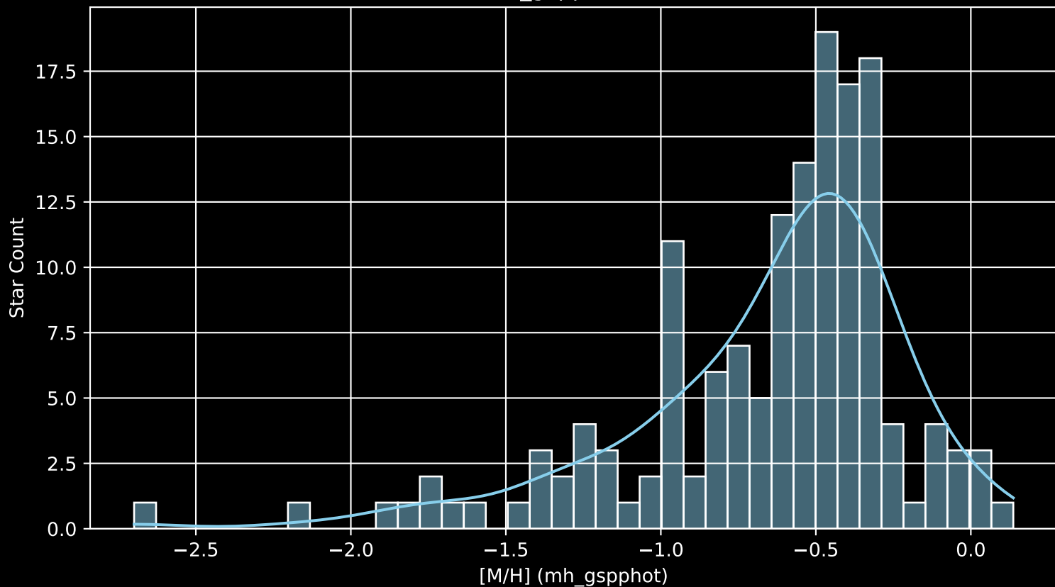
Gaia Cluster: [ASCC_30 [M/H] (mh_gspphot) (n= 151)
