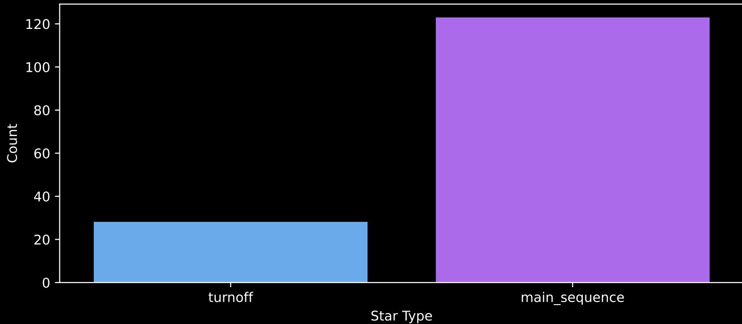
Gaia Cluster: [ASCC_30] Count plot of Star Type
