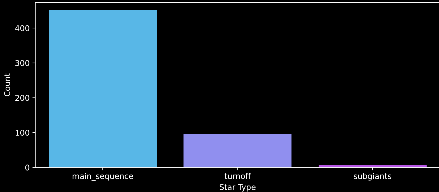
Gaia Cluster: [ASCC_32] Count plot of Star Type
