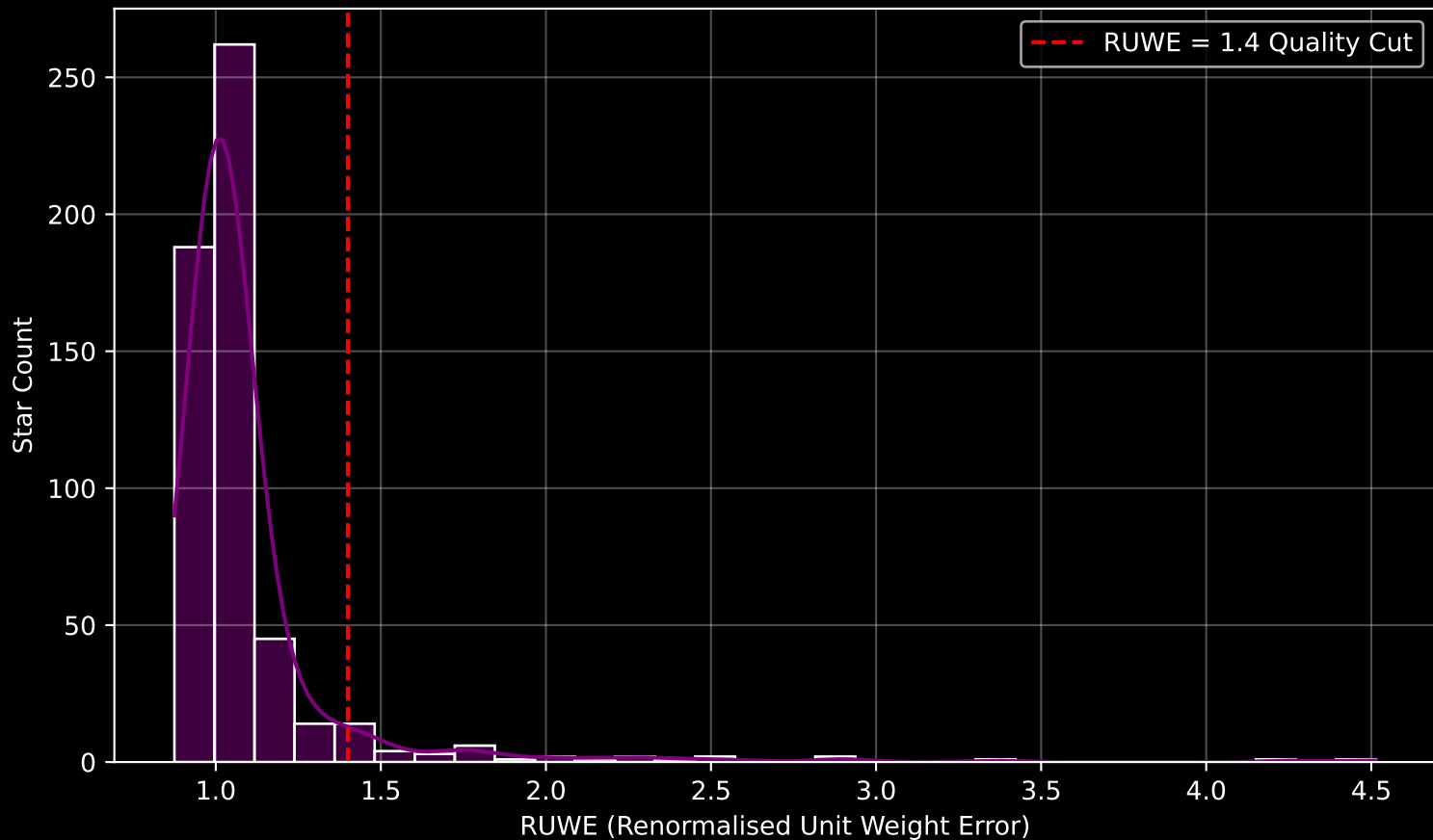
Gaia Cluster: [ASCC_32] RUWE Distribution (n= 550)
