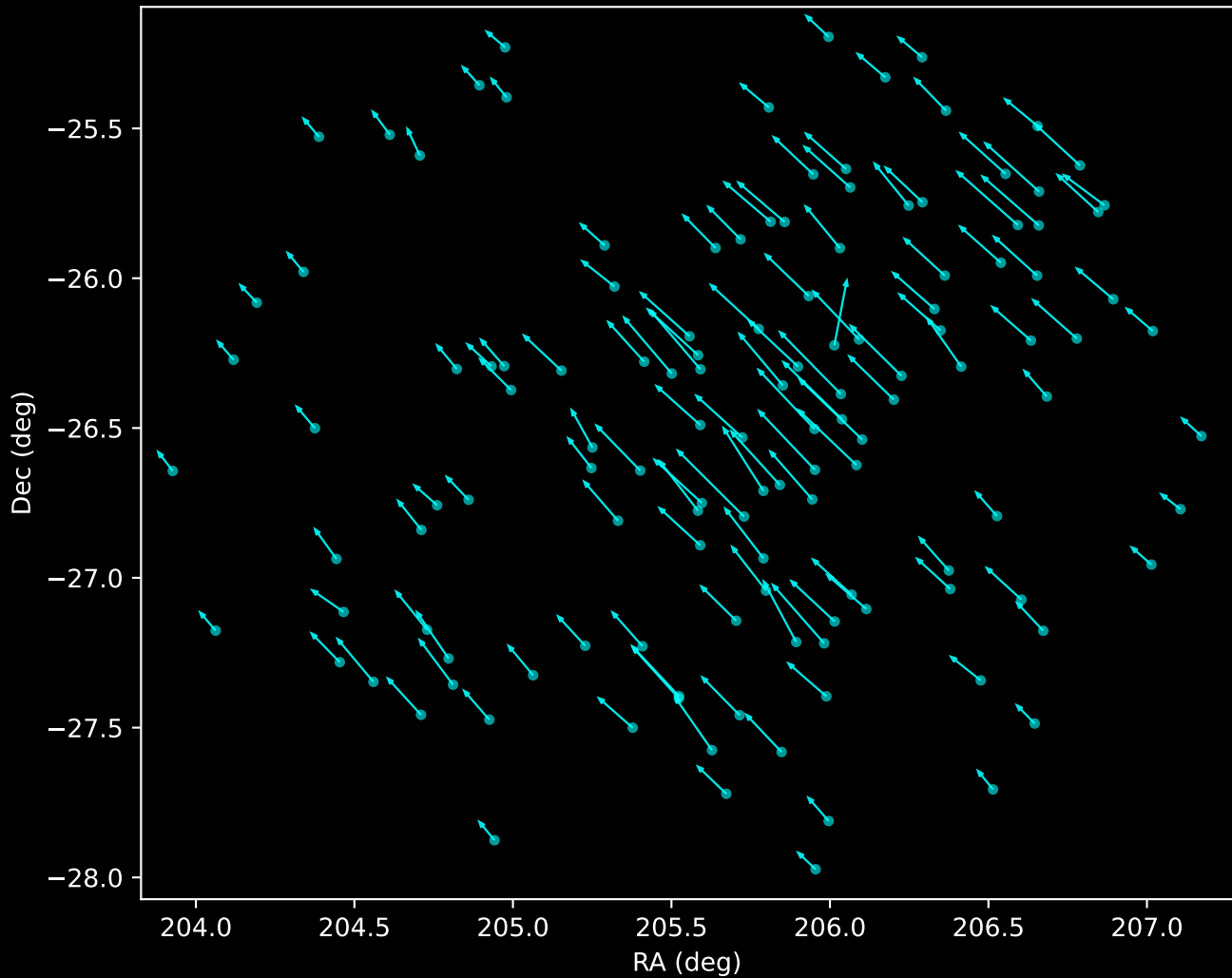
Gaia DR3 Noise Stream Proper Motion Vectors (n=130)
