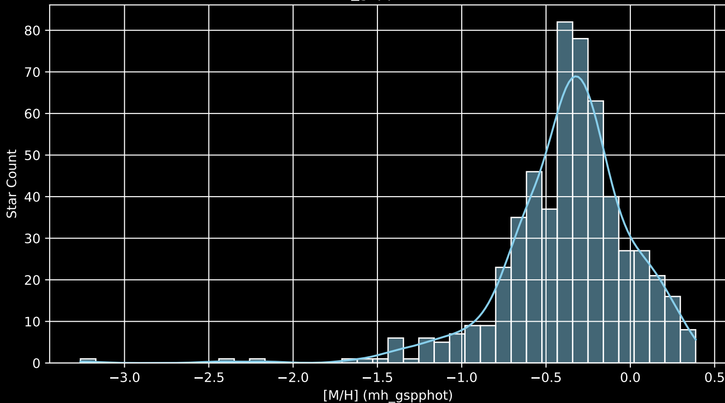
Gaia Cluster: [ASCC_32 [M/H] (mh_gspphot) (n= 552)
