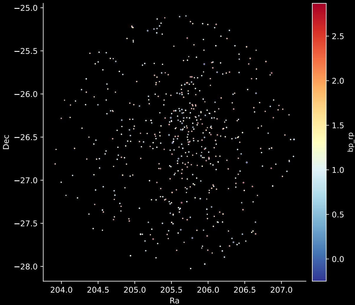
Gaia Cluster: [ASCC_32] Stars: 553
