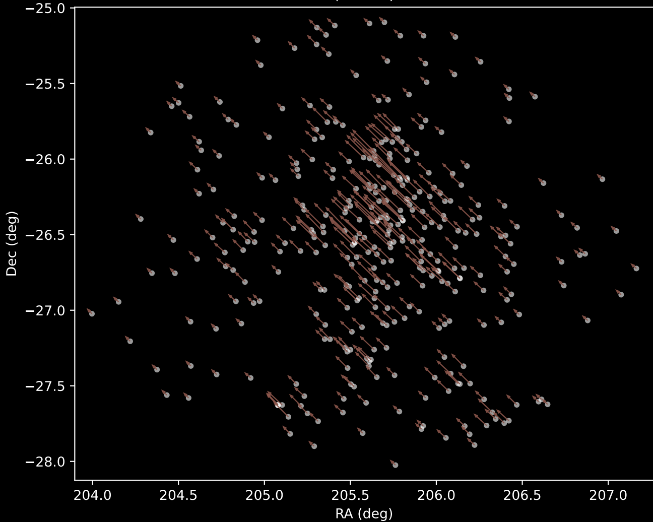
Gaia DR3 Cluster 10 Proper Motion Vectors (n=346)
