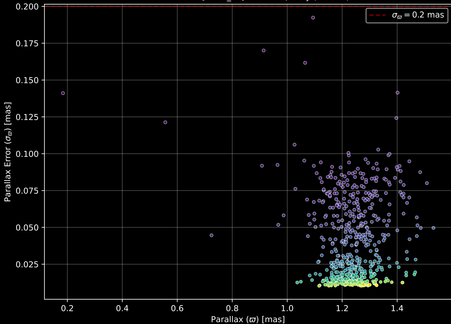
Gaia Cluster: [ASCC_32] Parallax Quality (n= 553)
