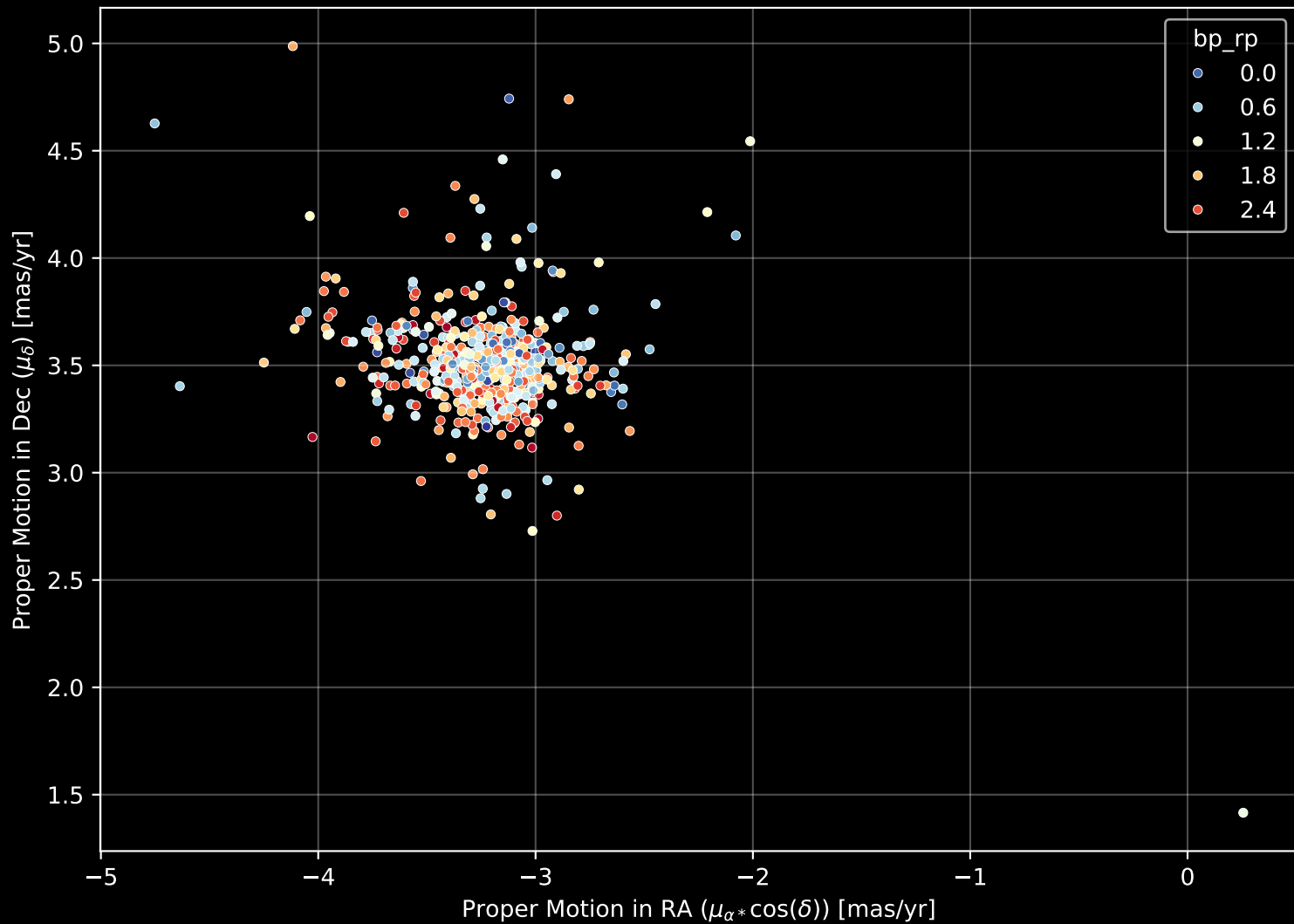
Gaia Cluster: [ASCC_32] Proper Motion Diagram (n= 553)
