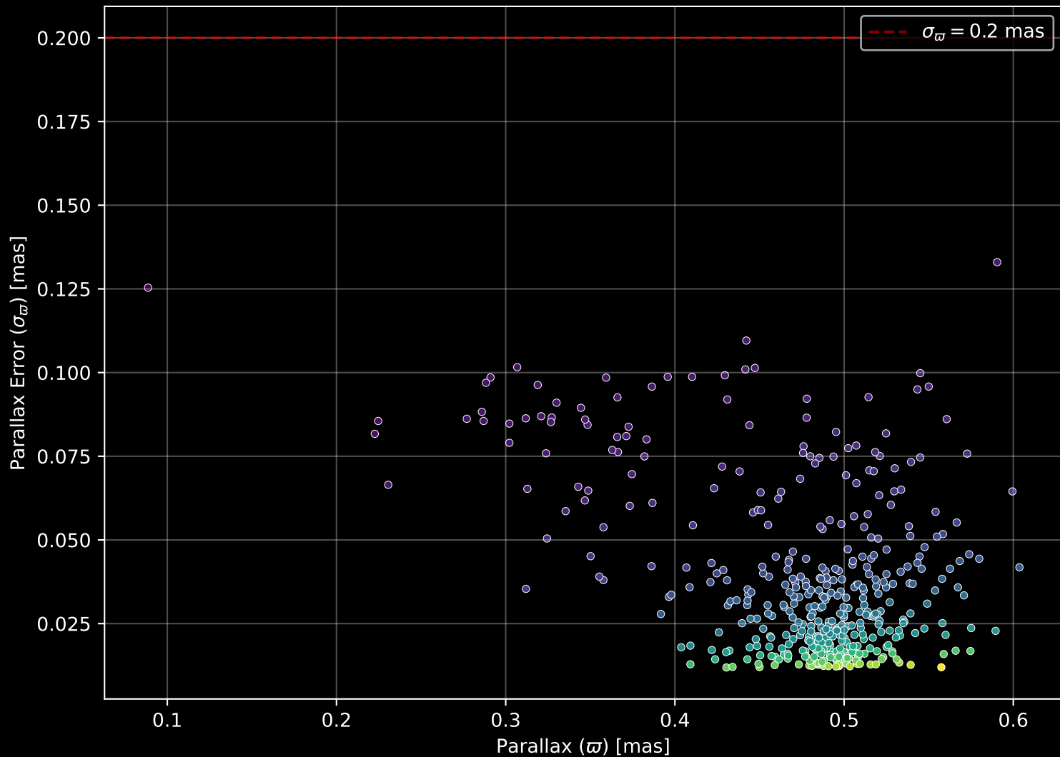
Gaia Cluster: [ASCC_67] Parallax Quality (n= 426)
