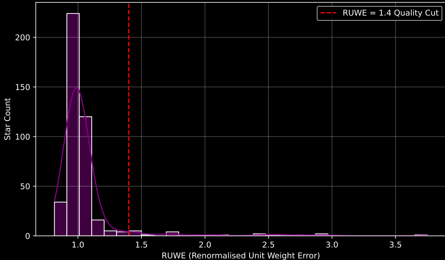
Gaia Cluster: [ASCC_67] RUWE Distribution (n= 424)
