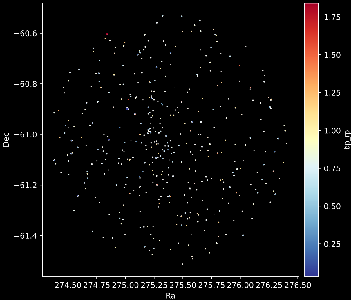
Gaia Cluster: [ASCC_67] Stars: 426
