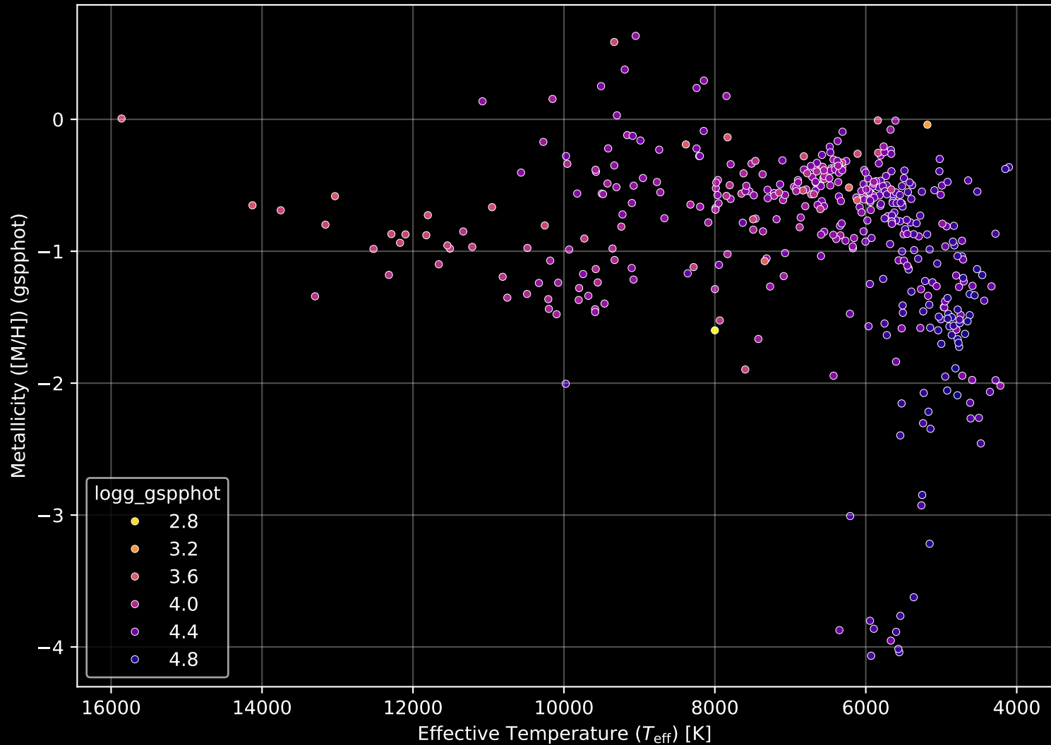
Gaia Cluster: [ASCC_67] Stellar Population Parameters (n= 426)
