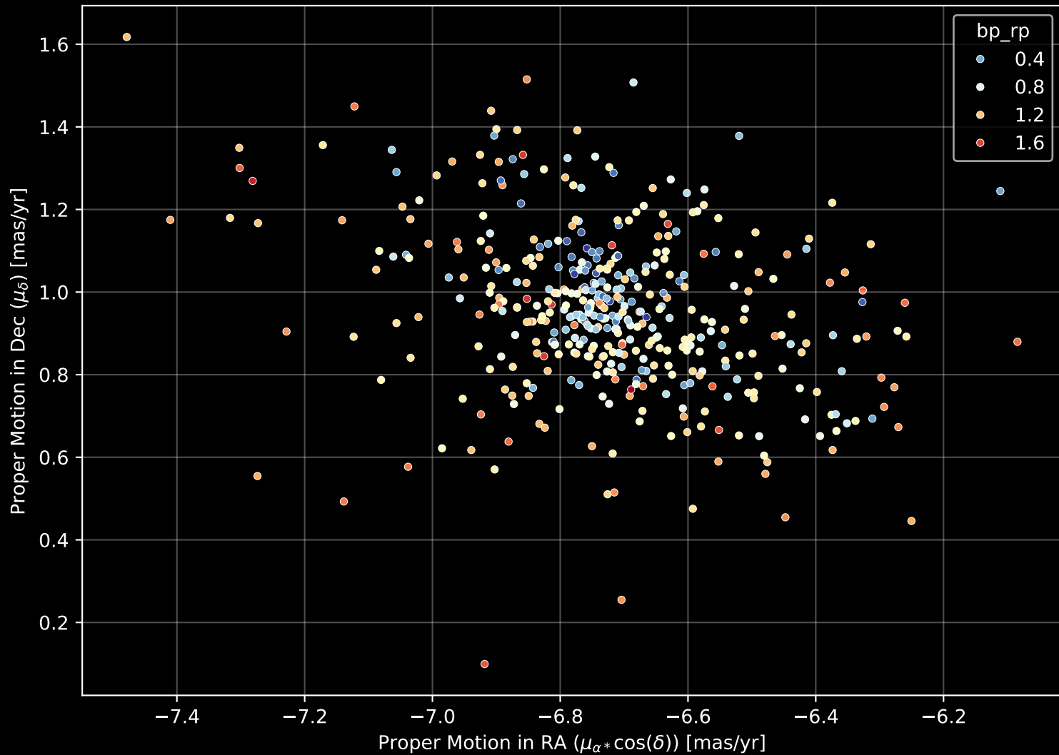
Gaia Cluster: [ASCC_67] Proper Motion Diagram (n= 426)
