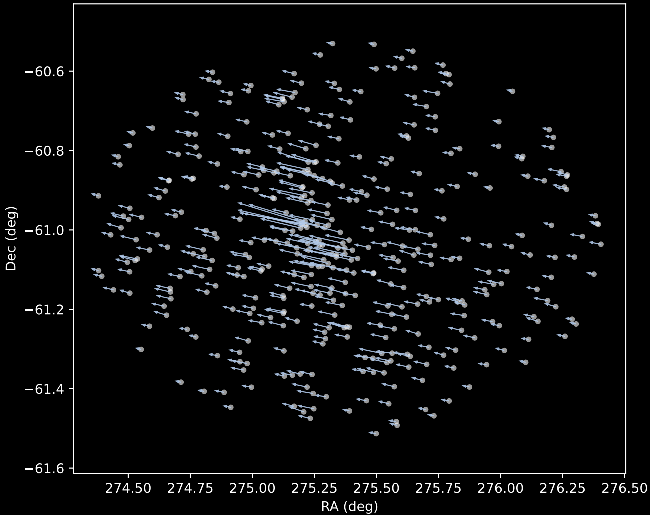
Gaia DR3 Cluster 1 Proper Motion Vectors (n=404)
