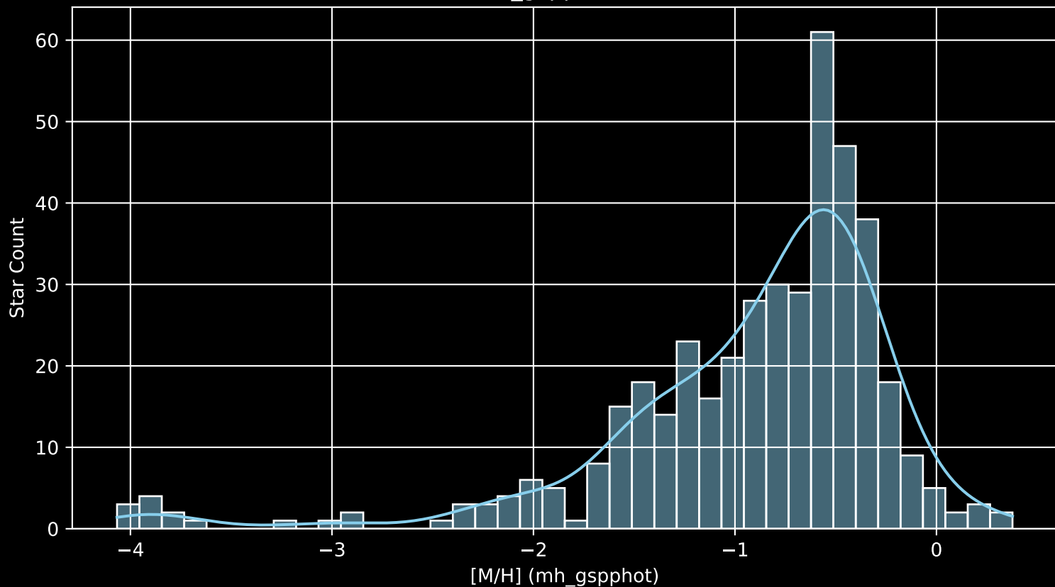
Gaia Cluster: [ASCC_67 [M/H] (mh_gspphot) (n= 424)
