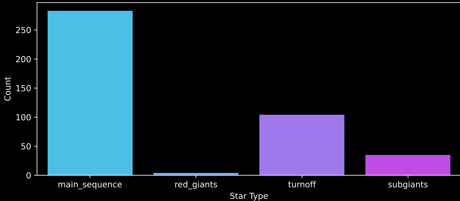
Gaia Cluster: [ASCC_67] Count plot of Star Type
